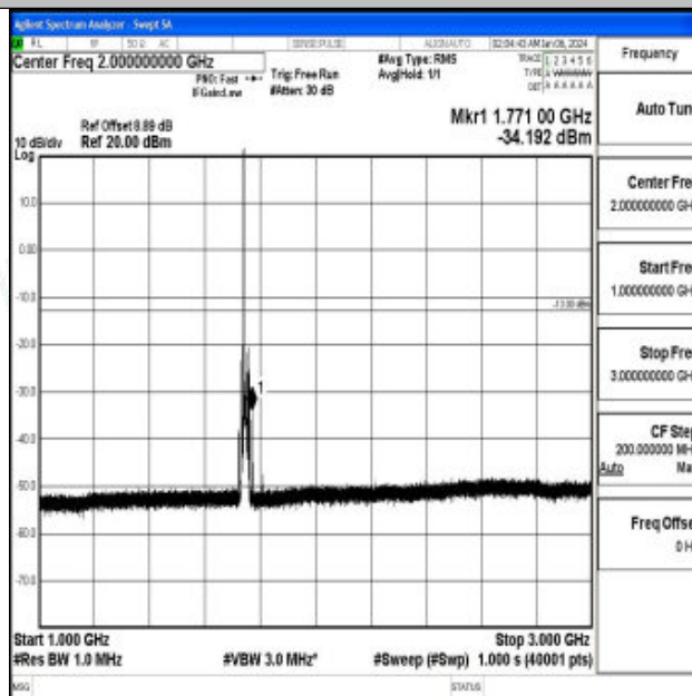
Band66_10MHz_16QAM_132322_1RB#0_1000~3000_1000~3000
