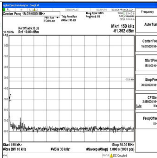
Band66_15MHz_QPSK_132047_1RB#0_0.15~30_0.15~30
