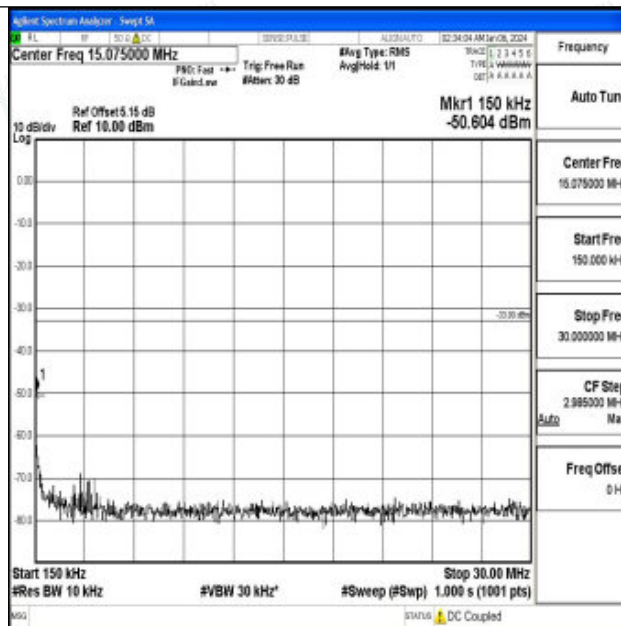
Band66_20MHz_QPSK_132072_1RB#0_0.15~30_0.15~30
