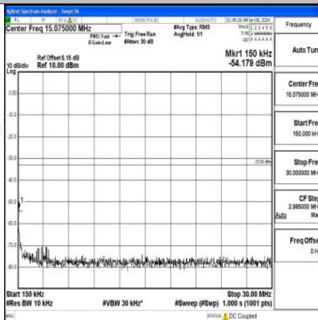
Band66_5MHz_16QAM_132322_1RB#0_0.15~30_0.15~30
