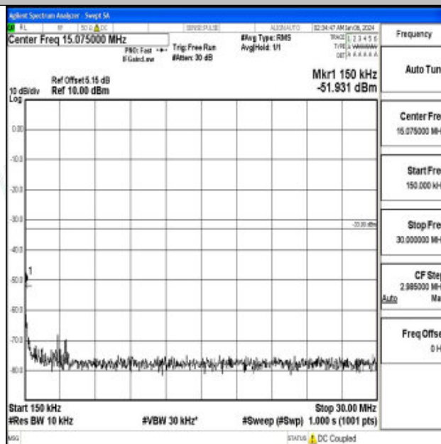
Band66_20MHz_16QAM_132072_1RB#0_0.15~30_0.15~30
