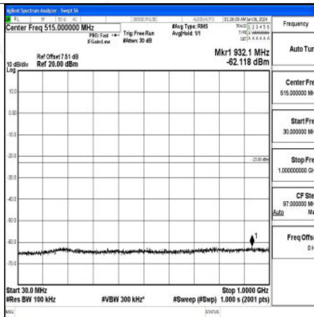
Band66_3MHz_16QAM_132322_1RB#0_30~1000_30~1000
