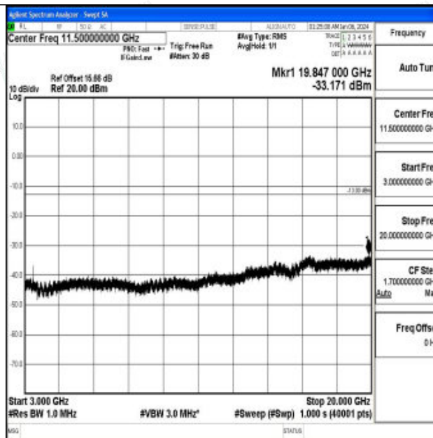
Band66_3MHz_16QAM_131987_1RB#0_3000~20000_3000~20000
