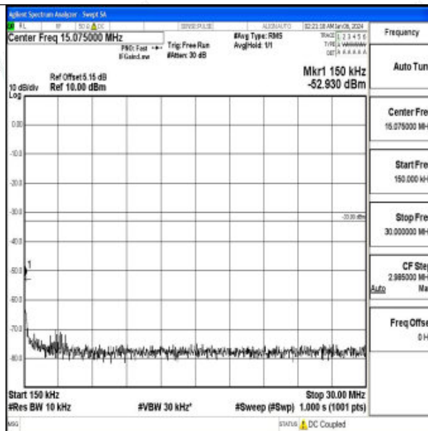
Band66_15MHz_QPSK_132597_1RB#0_0.15~30_0.15~30
