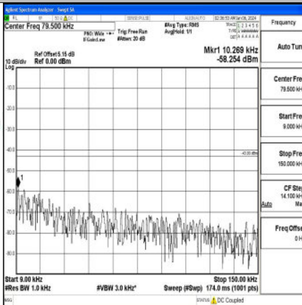
Band66_20MHz_QPSK_132572_1RB#0_0.009~0.15_0.009~0.15
