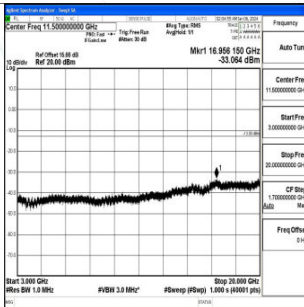
Band66_10MHz_16QAM_132322_1RB#0_3000~20000_3000~20000
