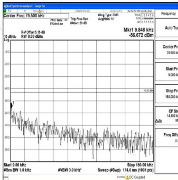
Band66_10MHz_16QAM_132022_1RB#0_0.009~0.15_0.009~0.15
