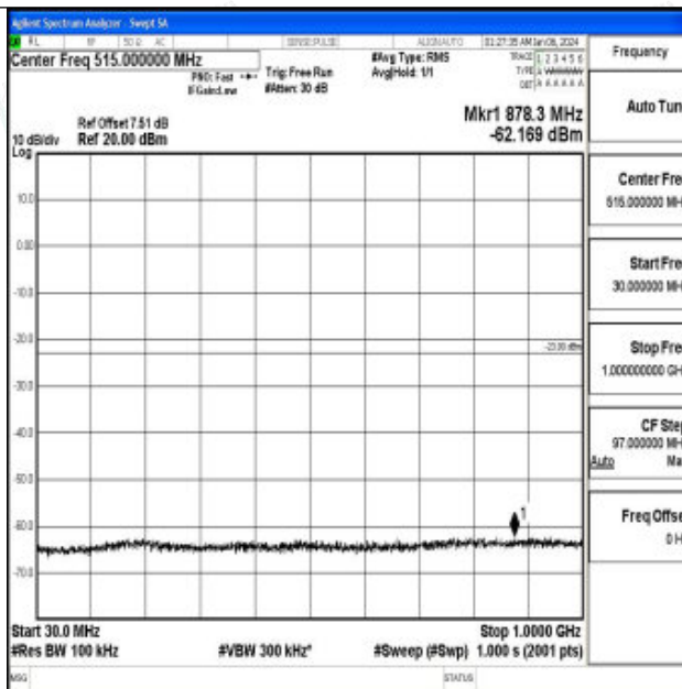
Band66_3MHz_16QAM_132657_1RB#0_30~1000_30~1000
