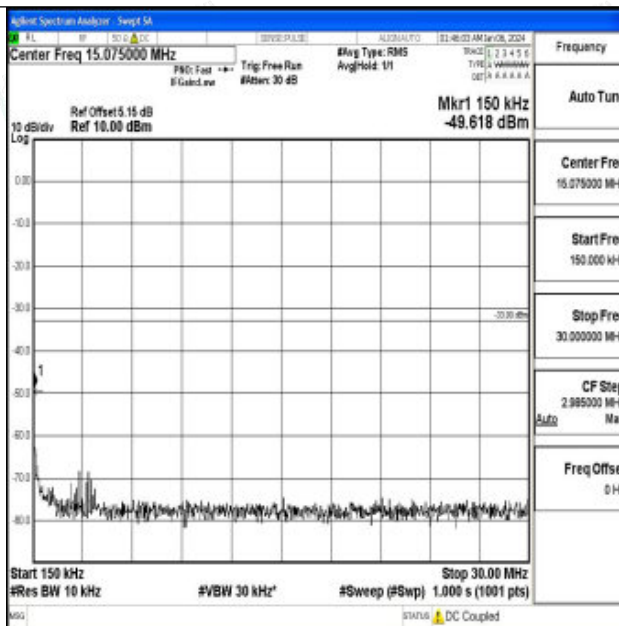
Band66_5MHz_QPSK_132647_1RB#0_0.15~30_0.15~30
