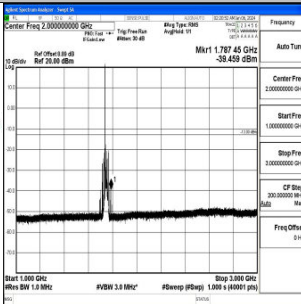
Band66_15MHz_16QAM_132322_1RB#0_1000~3000_1000~3000
