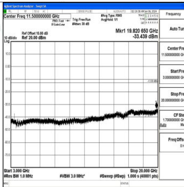
Band66_15MHz_16QAM_132047_1RB#0_3000~20000_3000~20000
