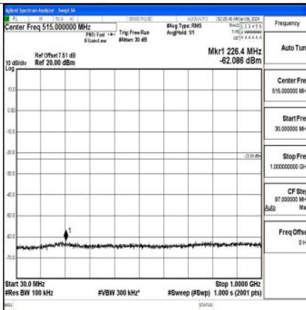
Band66_15MHz_16QAM_132322_1RB#0_30~1000_30~1000
