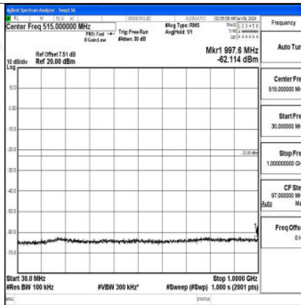
Band66_10MHz_16QAM_132622_1RB#0_30~1000_30~1000
