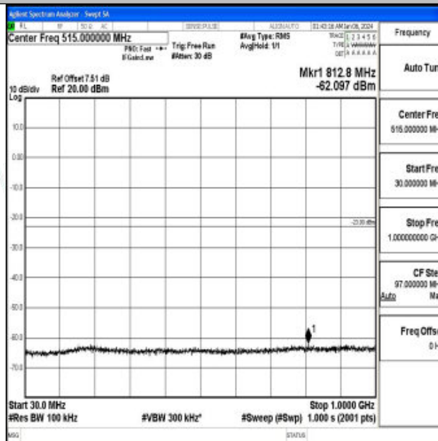
Band66_5MHz_QPSK_131997_1RB#0_30~1000_30~1000
