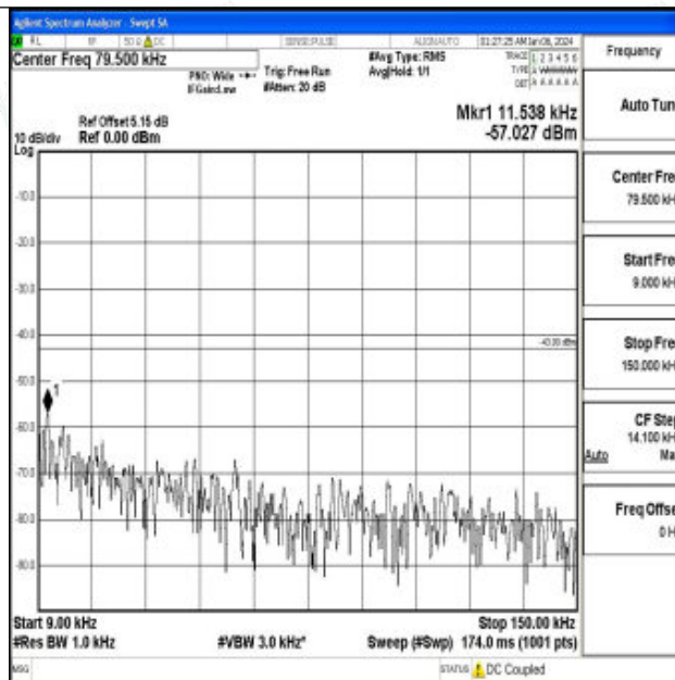
Band66_3MHz_16QAM_132657_1RB#0_0.009~0.15_0.009~0.15
