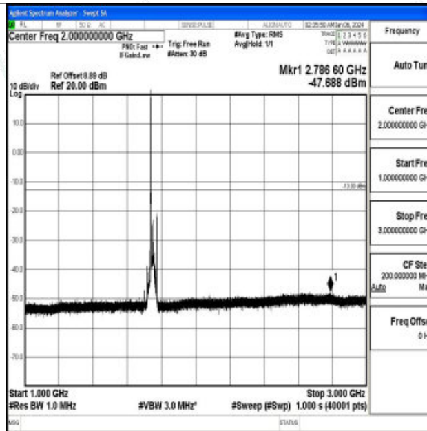
Band66_20MHz_QPSK_132322_1RB#0_1000~3000_1000~3000
