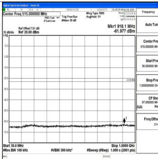
Band66_5MHz_16QAM_132322_1RB#0_30~1000_30~1000
