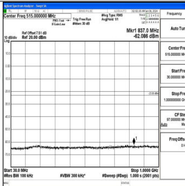
Band66_10MHz_QPSK_132022_1RB#0_30~1000_30~1000
