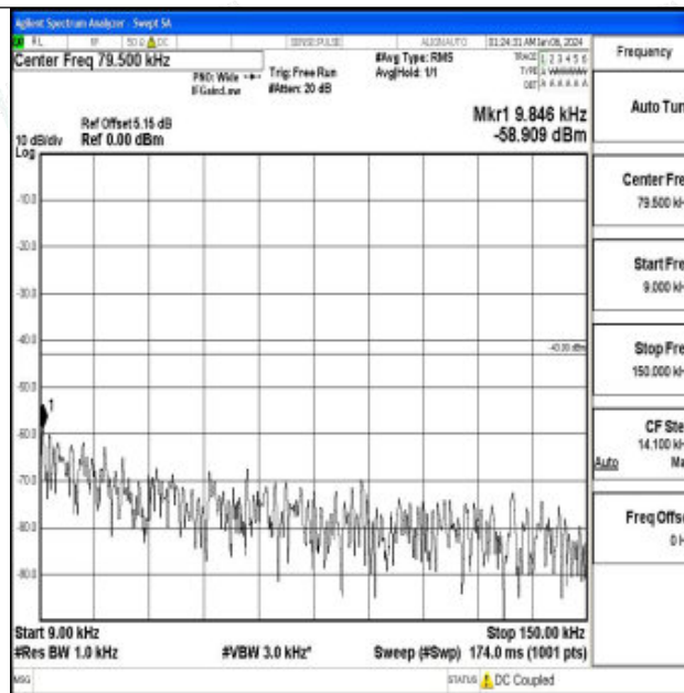
Band66_3MHz_16QAM_131987_1RB#0_0.009~0.15_0.009~0.15
