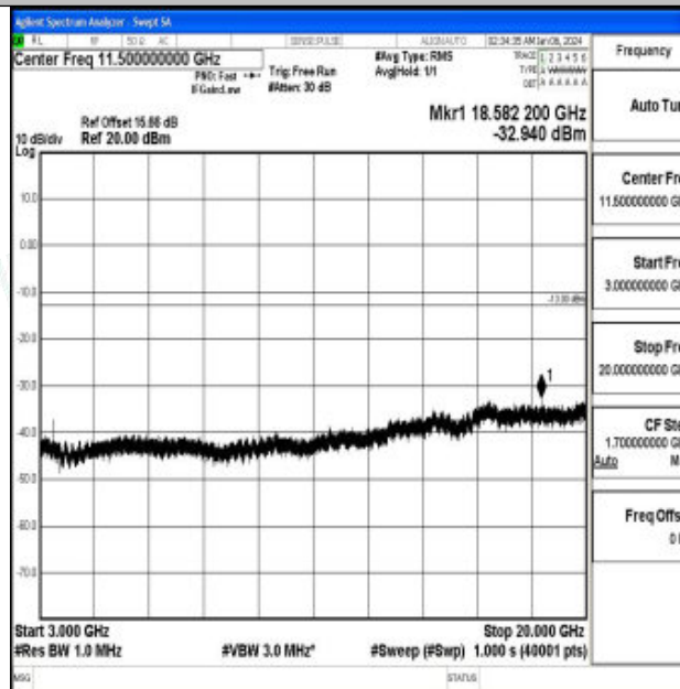
Band66_20MHz_QPSK_132072_1RB#0_3000~20000_3000~20000
