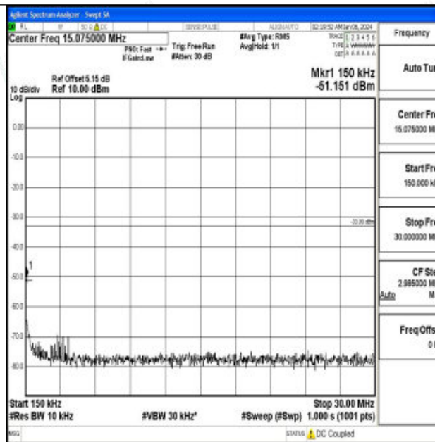
Band66_15MHz_QPSK_132322_1RB#0_0.15~30_0.15~30
