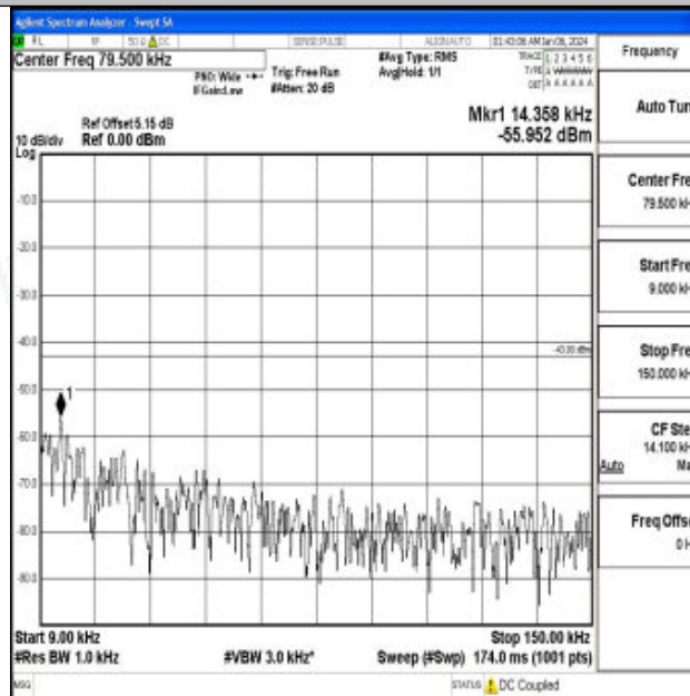
Band66_5MHz_QPSK_131997_1RB#0_0.009~0.15_0.009~0.15
