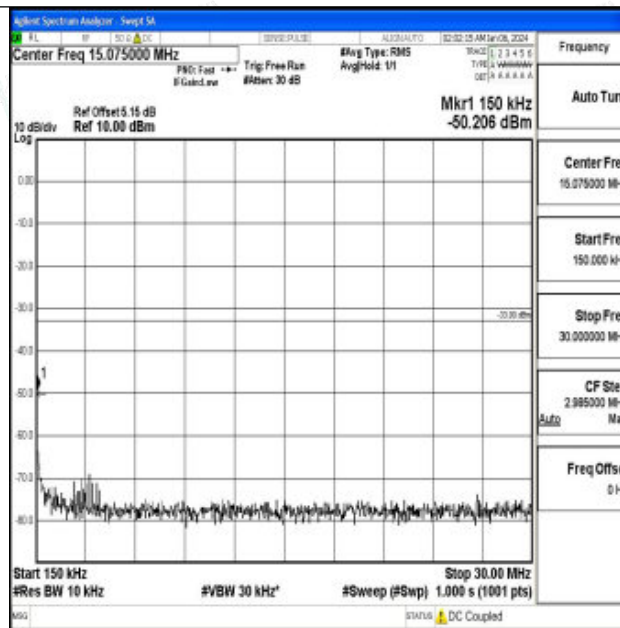
Band66_10MHz_QPSK_132022_1RB#0_0.15~30_0.15~30
