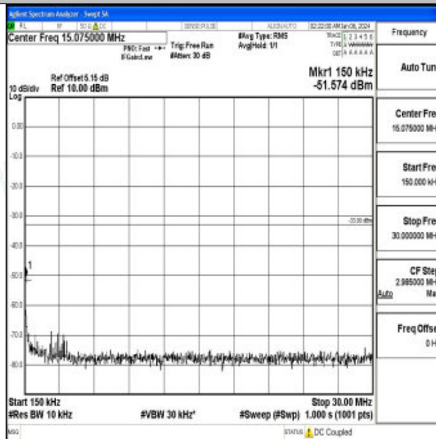
Band66_15MHz_16QAM_132597_1RB#0_0.15~30_0.15~30
