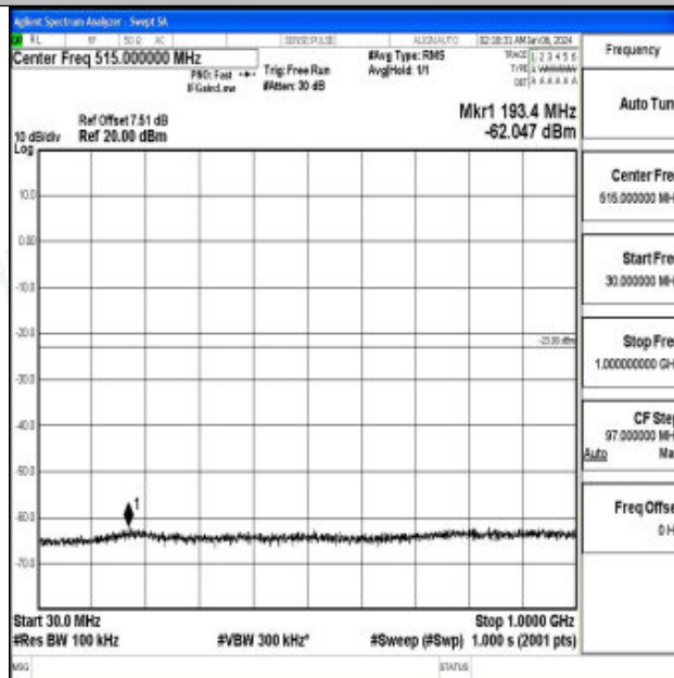
Band66_15MHz_QPSK_132047_1RB#0_30~1000_30~1000
