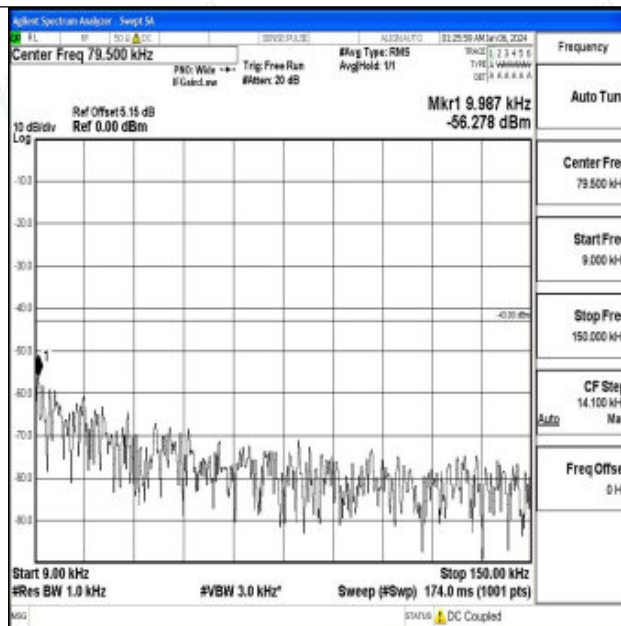
Band66_3MHz_16QAM_132322_1RB#0_0.009~0.15_0.009~0.15
