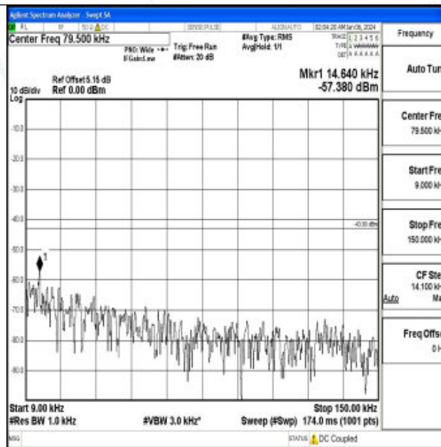
Band66_10MHz_16QAM_132322_1RB#0_0.009~0.15_0.009~0.15
