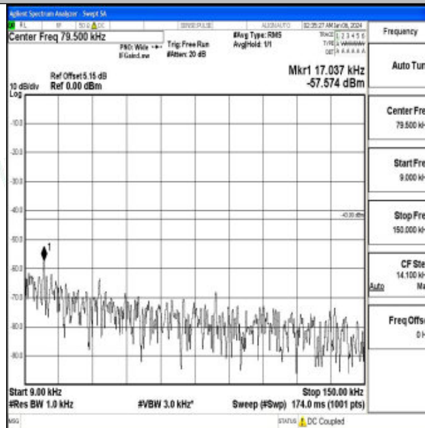
Band66_20MHz_QPSK_132322_1RB#0_0.009~0.15_0.009~0.15
