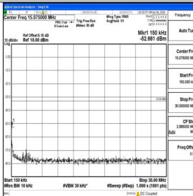
Band66_10MHz_16QAM_132022_1RB#0_0.15~30_0.15~30
