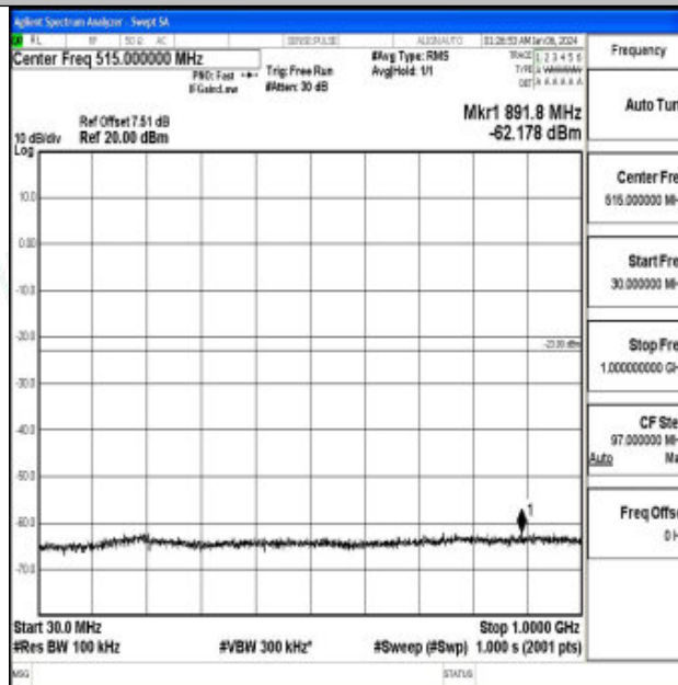
Band66_3MHz_QPSK_132657_1RB#0_30~1000_30~1000
