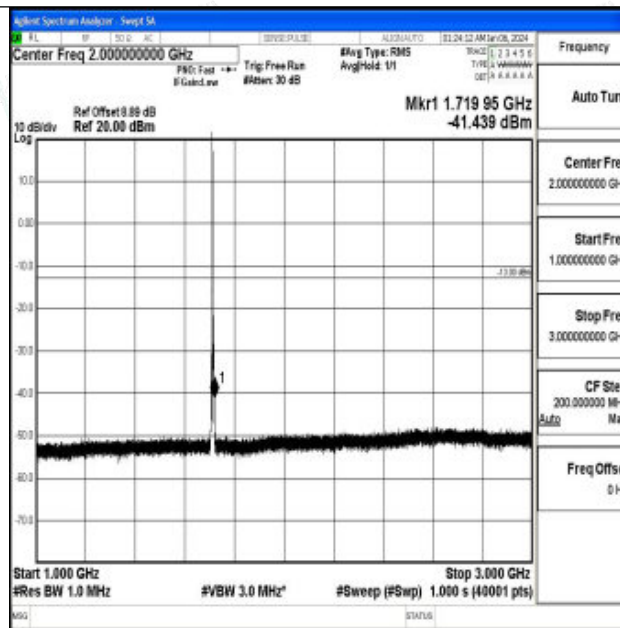
Band66_3MHz_QPSK_131987_1RB#0_1000~3000_1000~3000
