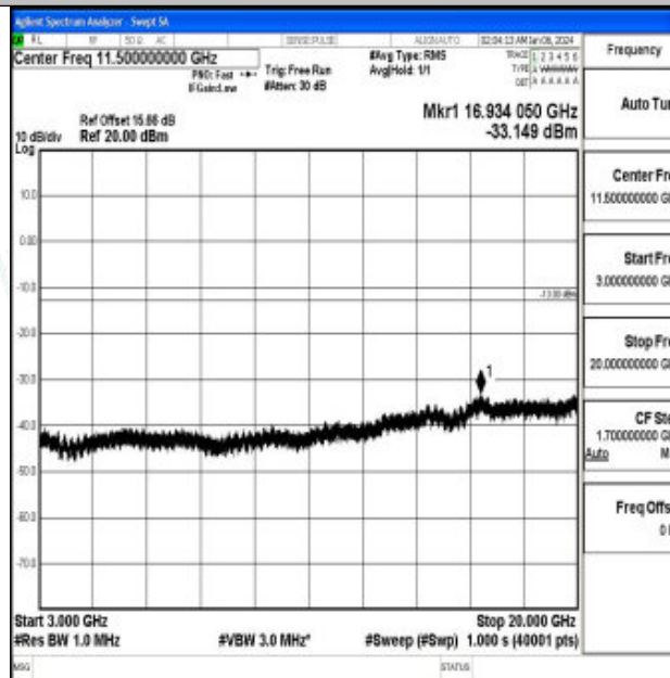
Band66_10MHz_QPSK_132322_1RB#0_3000~20000_3000~20000
