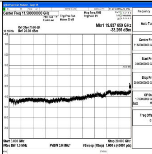
Band66_5MHz_QPSK_132647_1RB#0_3000~20000_3000~20000
