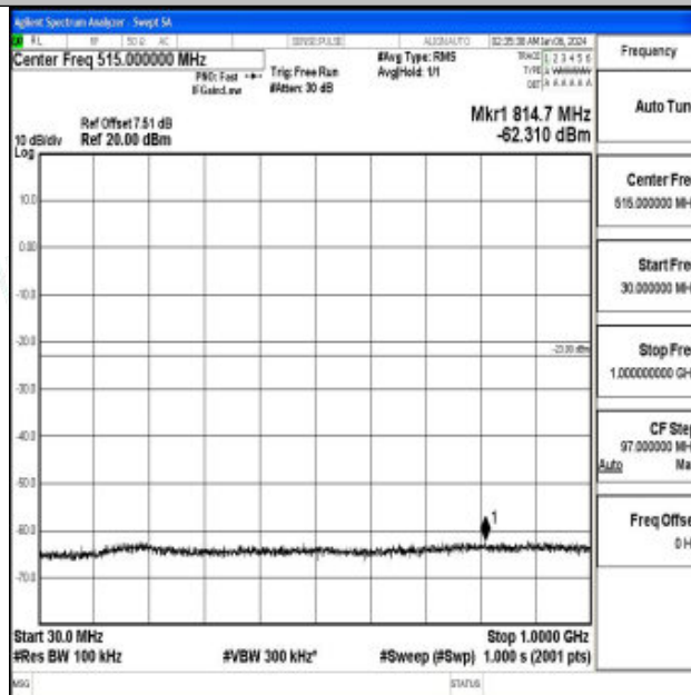
Band66_20MHz_QPSK_132322_1RB#0_30~1000_30~1000
