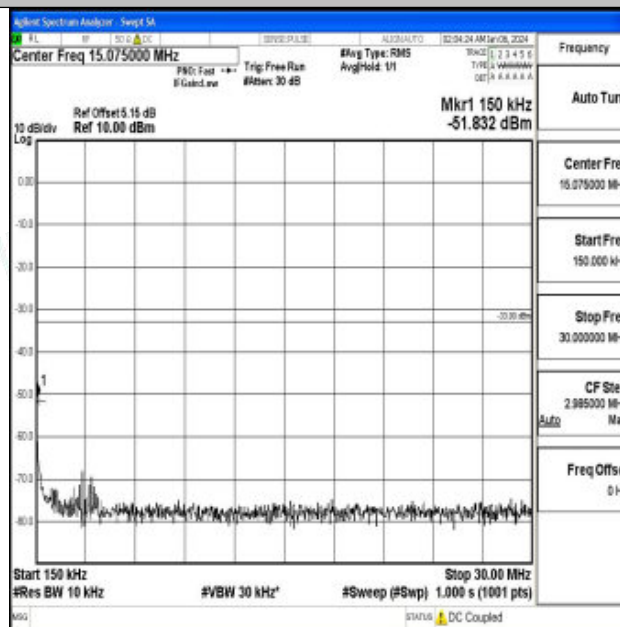
Band66_10MHz_16QAM_132322_1RB#0_0.15~30_0.15~30
