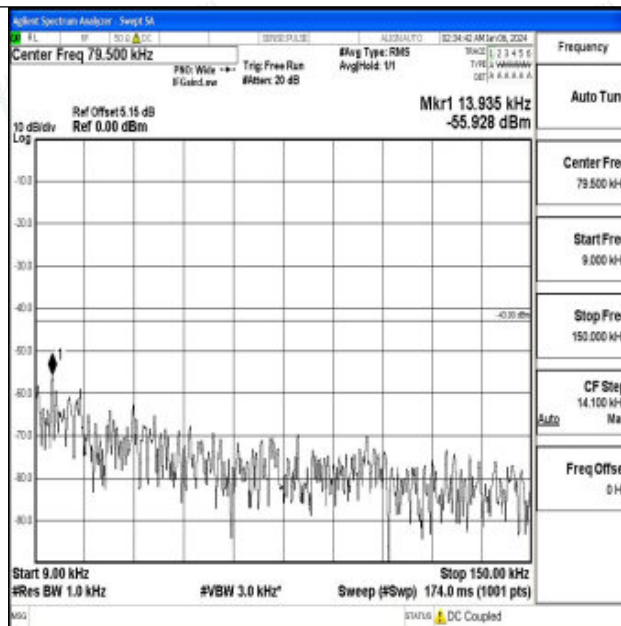
Band66_20MHz_16QAM_132072_1RB#0_0.009~0.15_0.009~0.15
