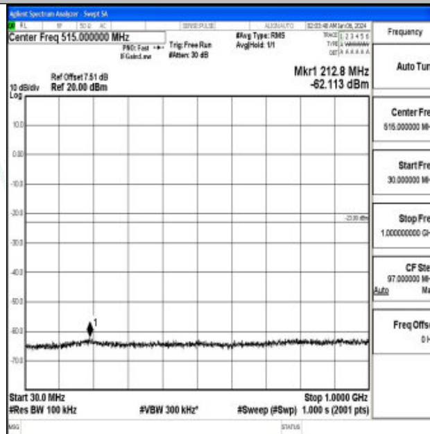
Band66_10MHz_QPSK_132322_1RB#0_30~1000_30~1000
