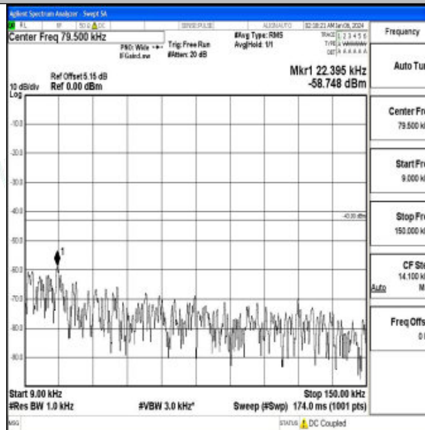
Band66_15MHz_QPSK_132047_1RB#0_0.009~0.15_0.009~0.15
