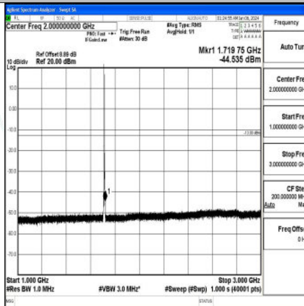
Band66_3MHz_16QAM_131987_1RB#0_1000~3000_1000~3000
