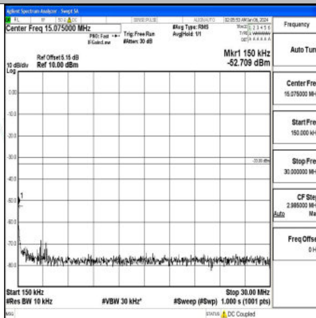
Band66_10MHz_16QAM_132622_1RB#0_0.15~30_0.15~30
