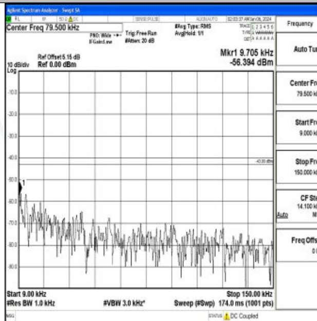
Band66_10MHz_QPSK_132322_1RB#0_0.009~0.15_0.009~0.15
