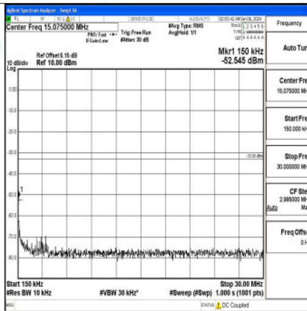
Band66_10MHz_QPSK_132322_1RB#0_0.15~30_0.15~30
