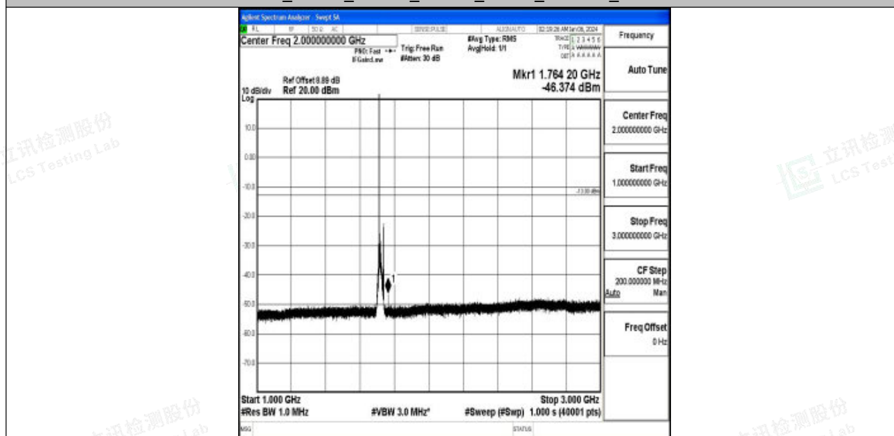
Band66_15MHz_16QAM_132047_1RB#0_1000~3000_1000~3000
