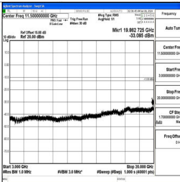
Band66_20MHz_16QAM_132322_1RB#0_3000~20000_3000~20000
