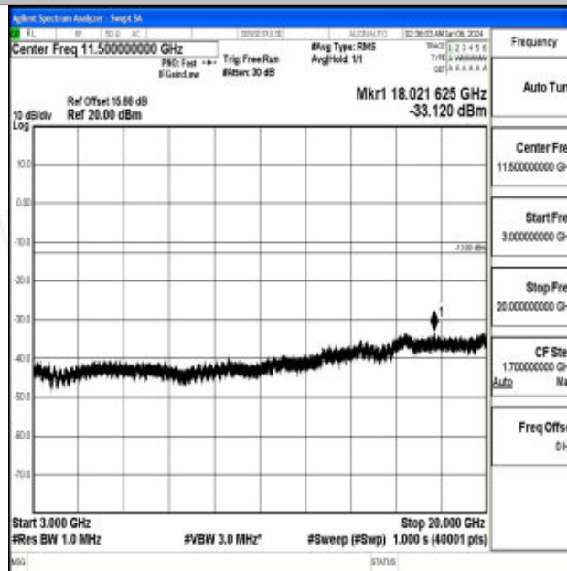
Band66_20MHz_QPSK_132322_1RB#0_3000~20000_3000~20000
