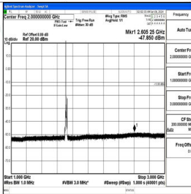
Band66_10MHz_QPSK_132022_1RB#0_1000~3000_1000~3000
