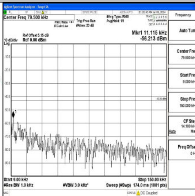
Band66_3MHz_QPSK_132657_1RB#0_0.009~0.15_0.009~0.15
