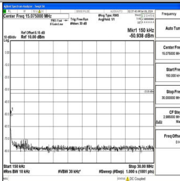
Band66_20MHz_16QAM_132572_1RB#0_0.15~30_0.15~30
