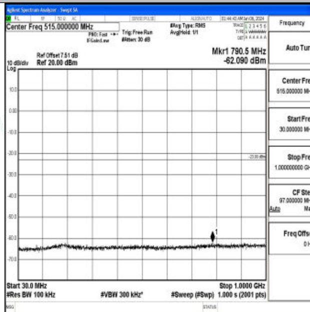
Band66_5MHz_QPSK_132322_1RB#0_30~1000_30~1000
