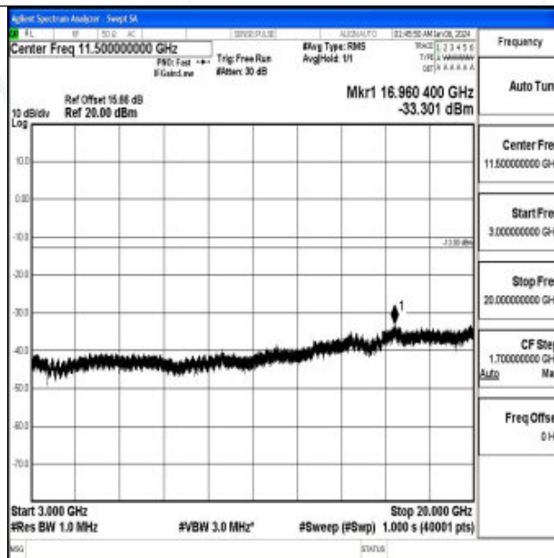
Band66_5MHz_16QAM_132322_1RB#0_3000~20000_3000~20000
