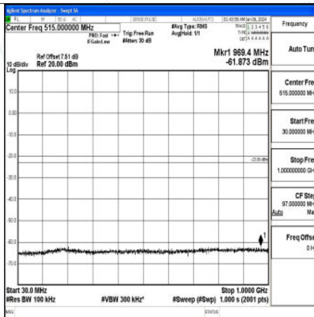
Band66_5MHz_16QAM_131997_1RB#0_30~1000_30~1000
