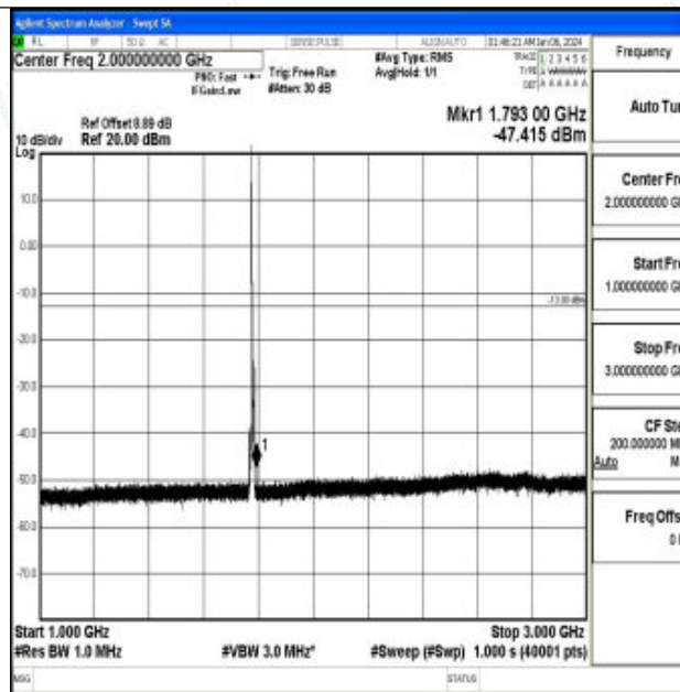
Band66_5MHz_QPSK_132647_1RB#0_1000~3000_1000~3000
