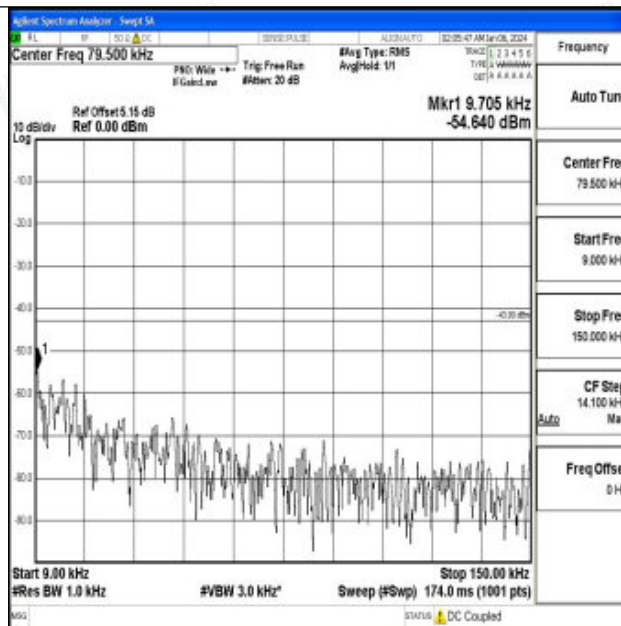
Band66_10MHz_16QAM_132622_1RB#0_0.009~0.15_0.009~0.15
