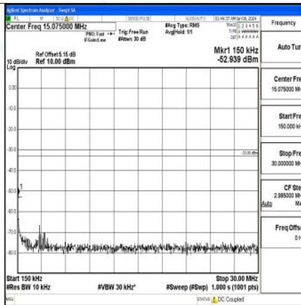
Band66_5MHz_QPSK_132322_1RB#0_0.15~30_0.15~30
