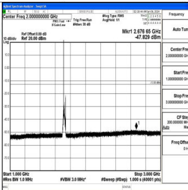
Band66_15MHz_QPSK_132047_1RB#0_1000~3000_1000~3000
