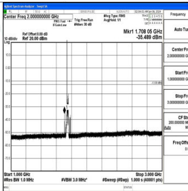
Band66_10MHz_QPSK_132322_1RB#0_1000~3000_1000~3000
