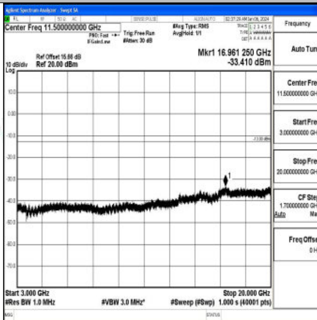
Band66_20MHz_QPSK_132572_1RB#0_3000~20000_3000~20000
