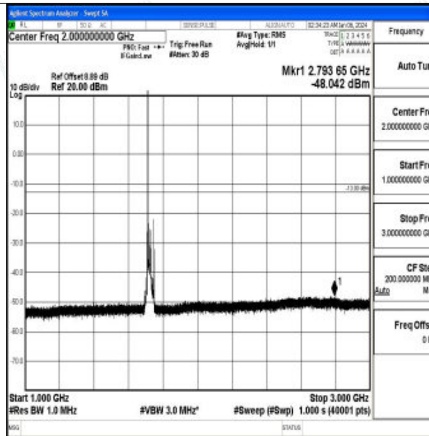
Band66_20MHz_QPSK_132072_1RB#0_1000~3000_1000~3000
