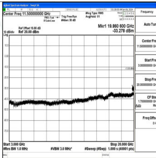
Band66_3MHz_16QAM_132657_1RB#0_3000~20000_3000~20000
