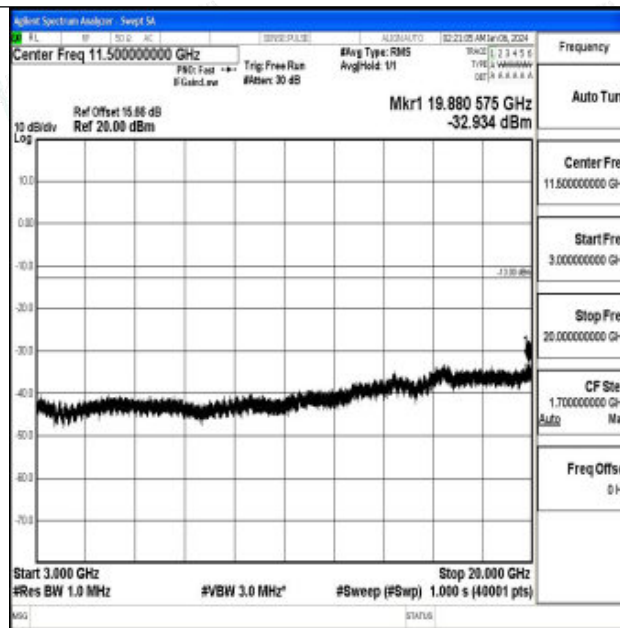
Band66_15MHz_16QAM_132322_1RB#0_3000~20000_3000~20000
