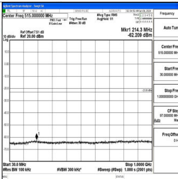
Band66_20MHz_16QAM_132072_1RB#0_30~1000_30~1000
