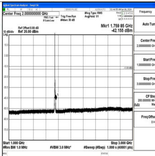
Band66_5MHz_QPSK_132322_1RB#0_1000~3000_1000~3000
