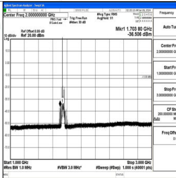
Band66_15MHz_QPSK_132322_1RB#0_1000~3000_1000~3000
