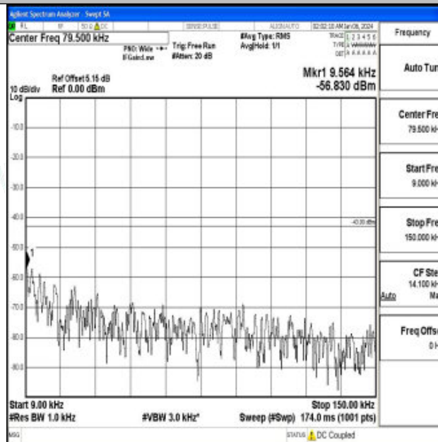
Band66_10MHz_QPSK_132022_1RB#0_0.009~0.15_0.009~0.15
