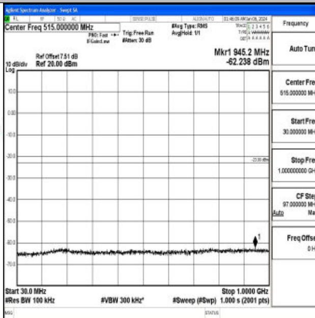
Band66_5MHz_QPSK_132647_1RB#0_30~1000_30~1000
