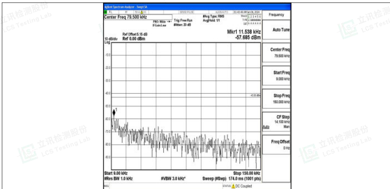
Band66_5MHz_16QAM_131997_1RB#0_0.009~0.15_0.009~0.15
