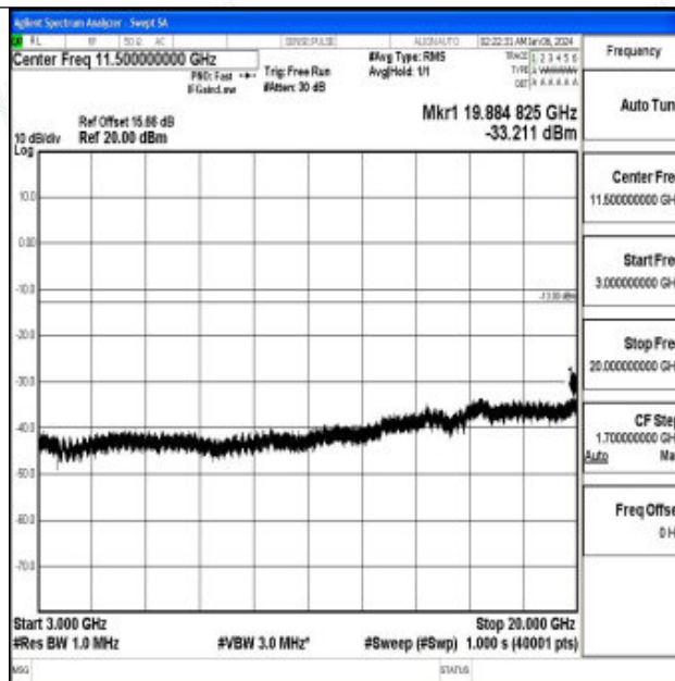
Band66_15MHz_16QAM_132597_1RB#0_3000~20000_3000~20000
