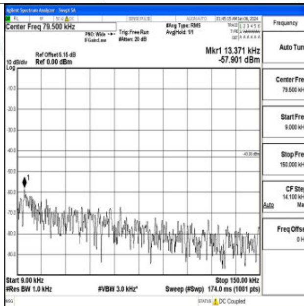
Band66_5MHz_16QAM_132322_1RB#0_0.009~0.15_0.009~0.15
