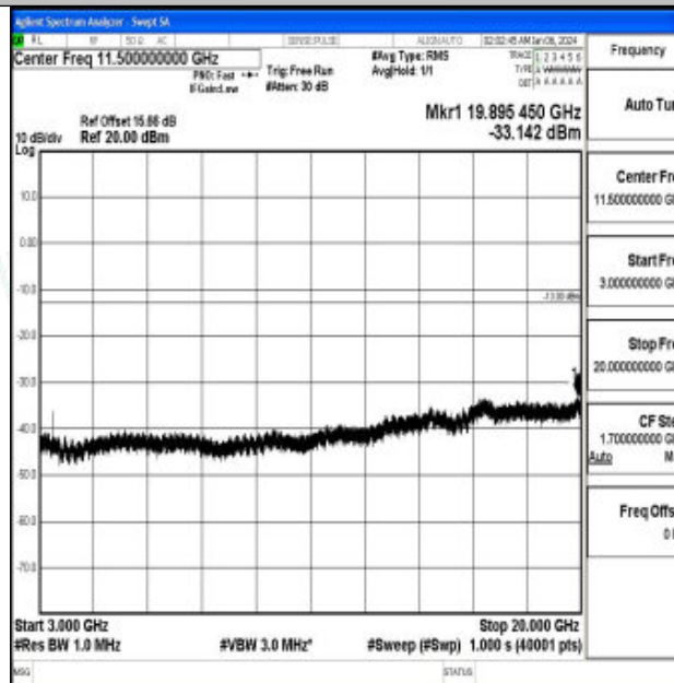
Band66_10MHz_QPSK_132022_1RB#0_3000~20000_3000~20000
