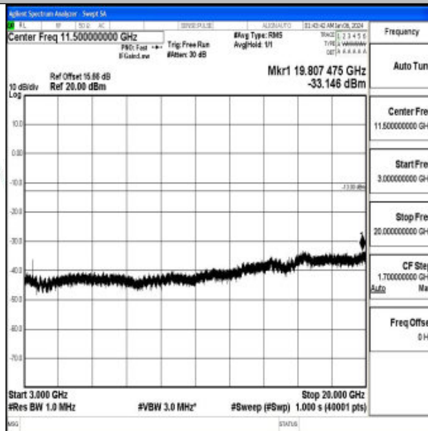
Band66_5MHz_QPSK_131997_1RB#0_3000~20000_3000~20000
