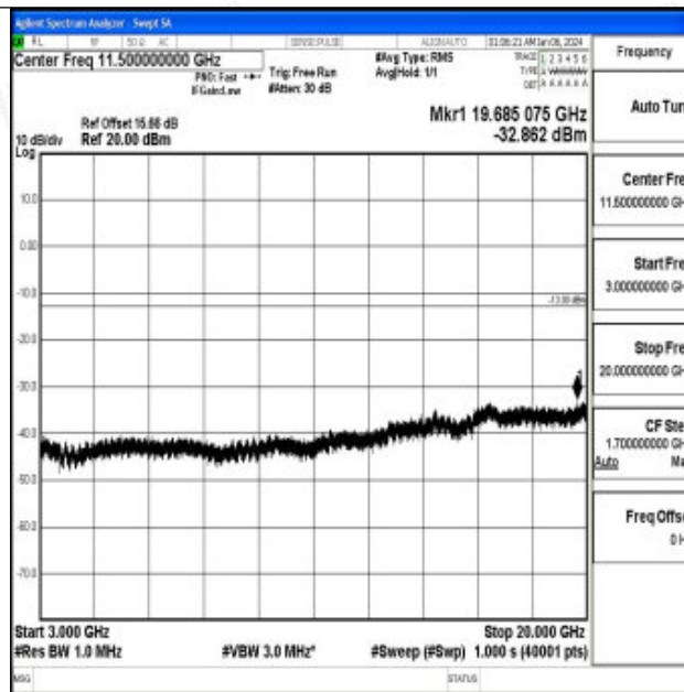
Band66_1.4MHz_16QAM_132665_1RB#0_3000~20000_3000~20000
