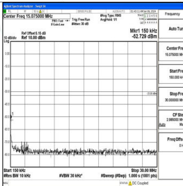
Band66_5MHz_QPSK_131997_1RB#0_0.15~30_0.15~30
