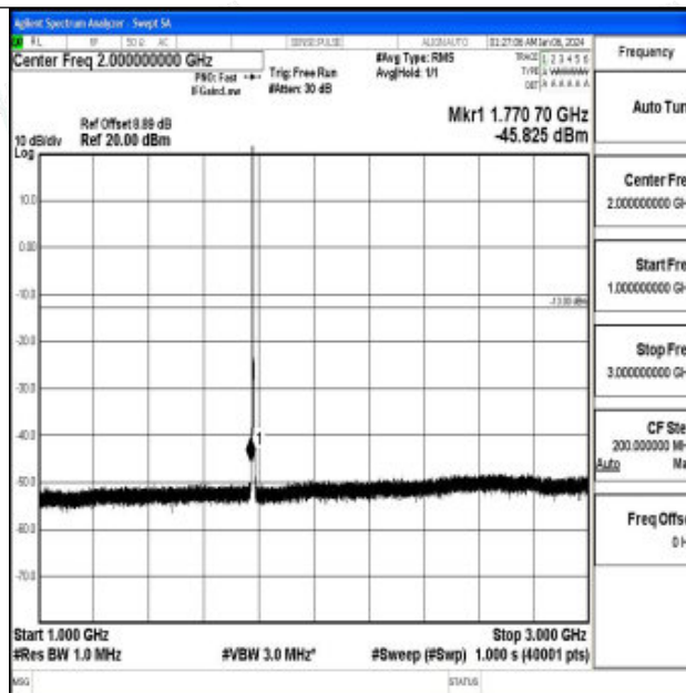
Band66_3MHz_QPSK_132657_1RB#0_1000~3000_1000~3000
