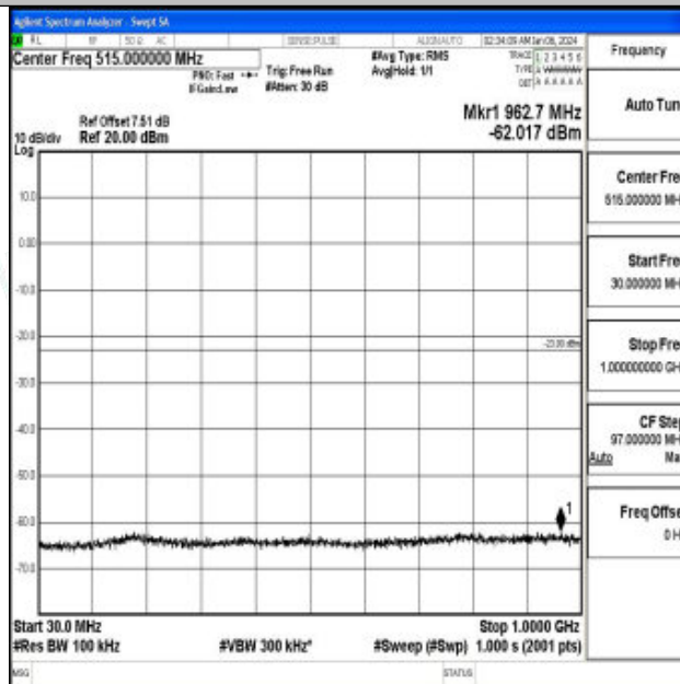
Band66_20MHz_QPSK_132072_1RB#0_30~1000_30~1000
