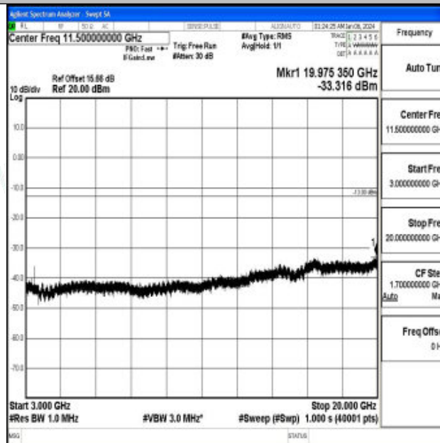
Band66_3MHz_QPSK_131987_1RB#0_3000~20000_3000~20000
