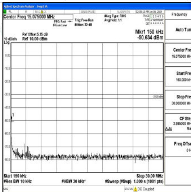
Band66_10MHz_QPSK_132622_1RB#0_0.15~30_0.15~30
