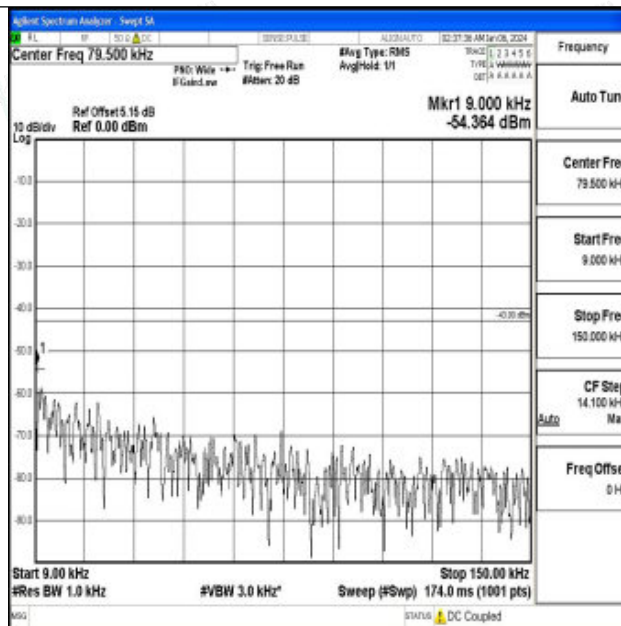
Band66_20MHz_16QAM_132572_1RB#0_0.009~0.15_0.009~0.15
