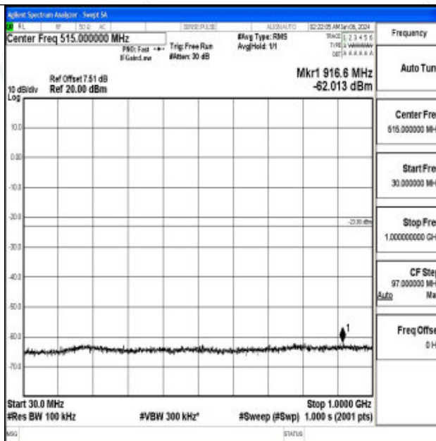
Band66_15MHz_16QAM_132597_1RB#0_30~1000_30~1000
