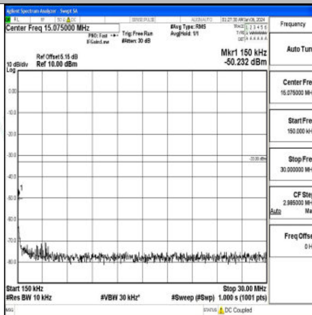
Band66_3MHz_16QAM_132657_1RB#0_0.15~30_0.15~30
