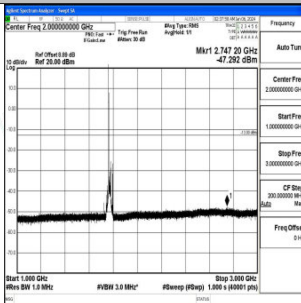
Band66_20MHz_16QAM_132572_1RB#0_1000~3000_1000~3000
