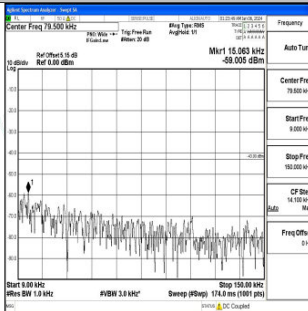
Band66_3MHz_QPSK_131987_1RB#0_0.009~0.15_0.009~0.15
