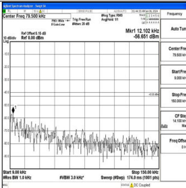
Band66_5MHz_QPSK_132322_1RB#0_0.009~0.15_0.009~0.15
