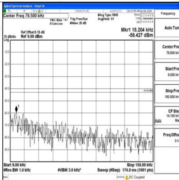
Band66_15MHz_16QAM_132597_1RB#0_0.009~0.15_0.009~0.15
