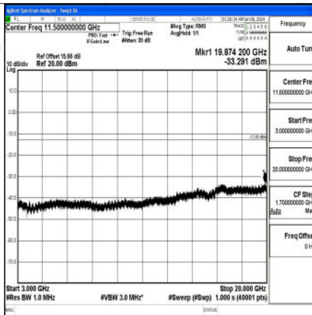
Band66_3MHz_16QAM_132322_1RB#0_3000~20000_3000~20000
