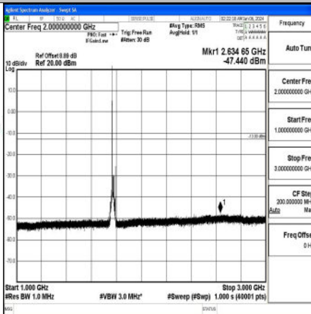
Band66_15MHz_16QAM_132597_1RB#0_1000~3000_1000~3000
