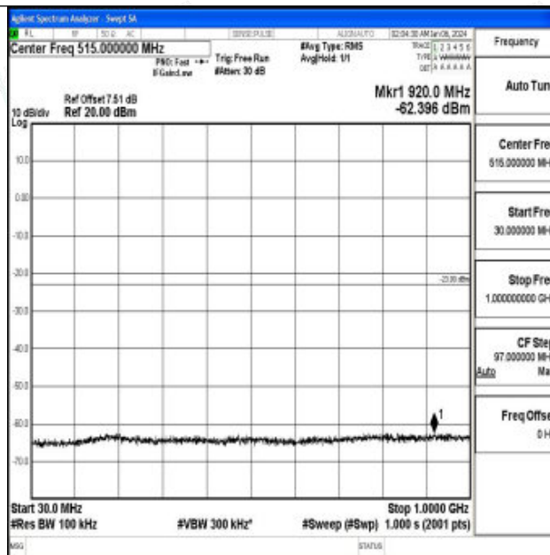
Band66_10MHz_16QAM_132322_1RB#0_30~1000_30~1000
