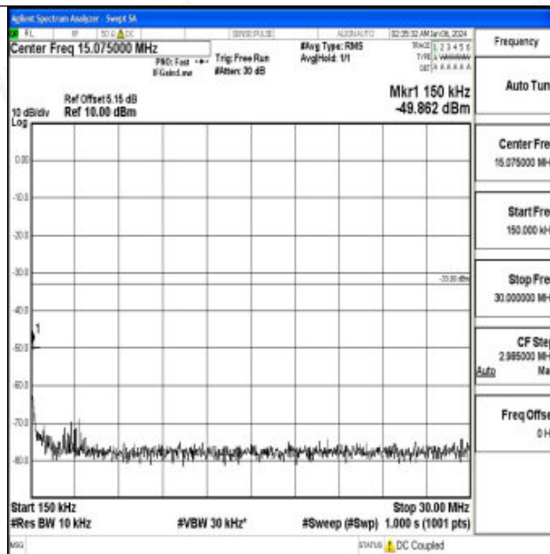
Band66_20MHz_QPSK_132322_1RB#0_0.15~30_0.15~30
