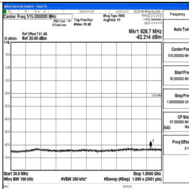
Band66_20MHz_16QAM_132572_1RB#0_30~1000_30~1000
