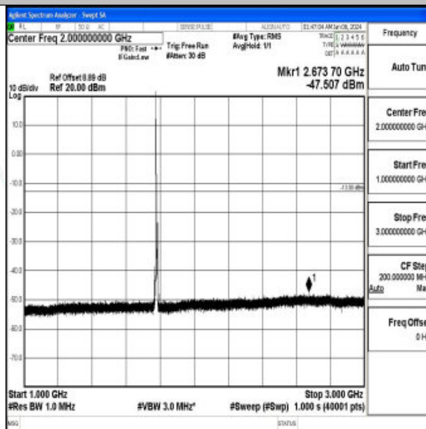
Band66_5MHz_16QAM_132647_1RB#0_1000~3000_1000~3000
