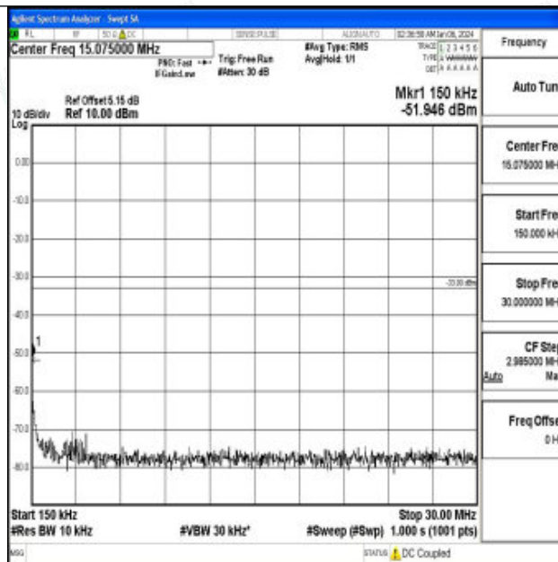
Band66_20MHz_QPSK_132572_1RB#0_0.15~30_0.15~30
