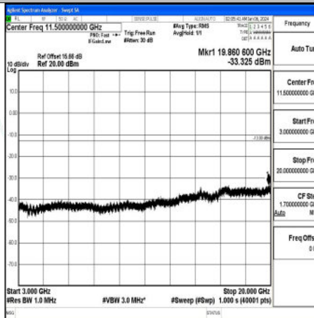
Band66_10MHz_QPSK_132622_1RB#0_3000~20000_3000~20000
