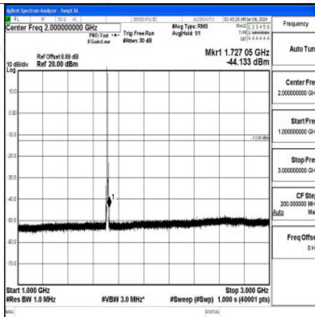
Band66_5MHz_QPSK_131997_1RB#0_1000~3000_1000~3000
