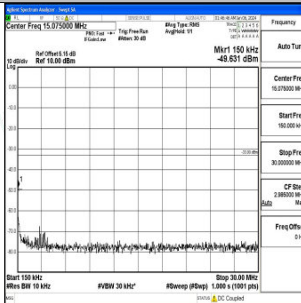
Band66_5MHz_16QAM_132647_1RB#0_0.15~30_0.15~30
