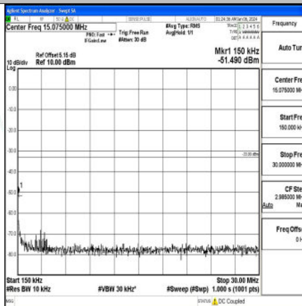
Band66_3MHz_16QAM_131987_1RB#0_0.15~30_0.15~30
