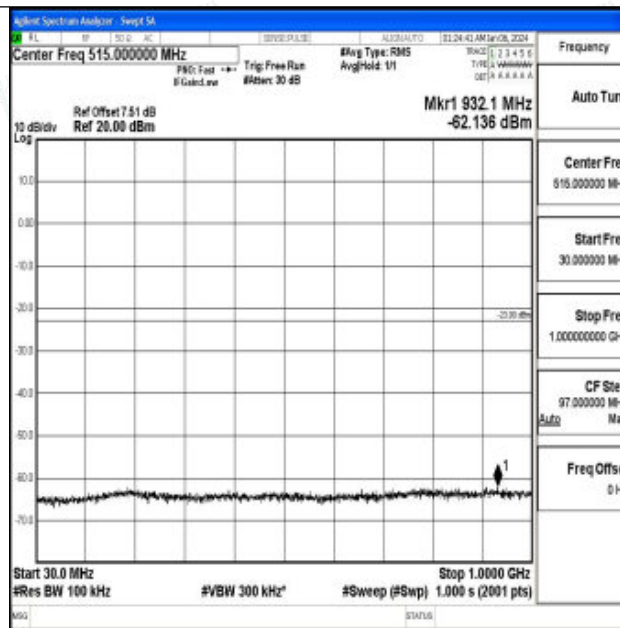
Band66_3MHz_16QAM_131987_1RB#0_30~1000_30~1000
