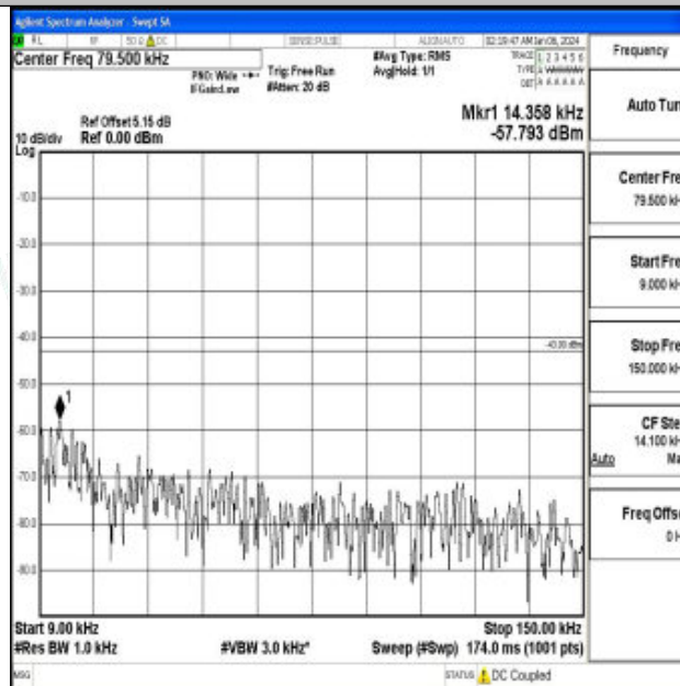
Band66_15MHz_QPSK_132322_1RB#0_0.009~0.15_0.009~0.15
