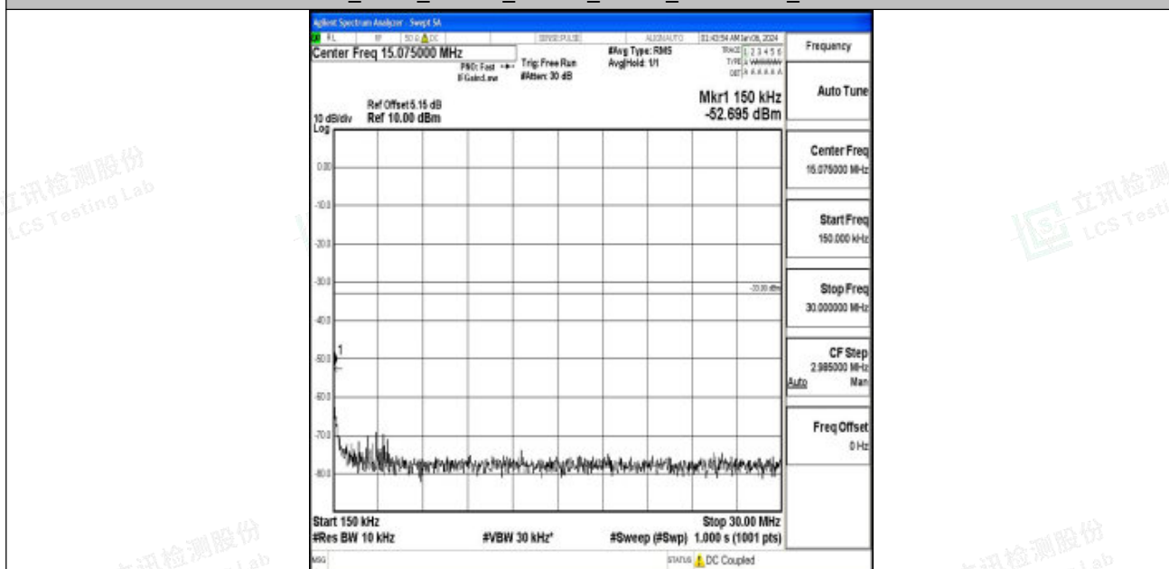
Band66_5MHz_16QAM_131997_1RB#0_0.15~30_0.15~30
