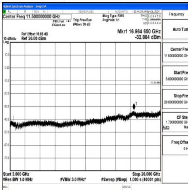
Band66_5MHz_16QAM_131997_1RB#0_3000~20000_3000~20000
