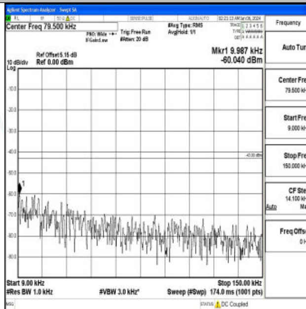
Band66_15MHz_QPSK_132597_1RB#0_0.009~0.15_0.009~0.15
