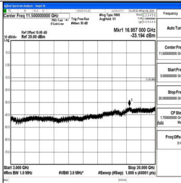
Band66_3MHz_QPSK_132322_1RB#0_3000~20000_3000~20000
