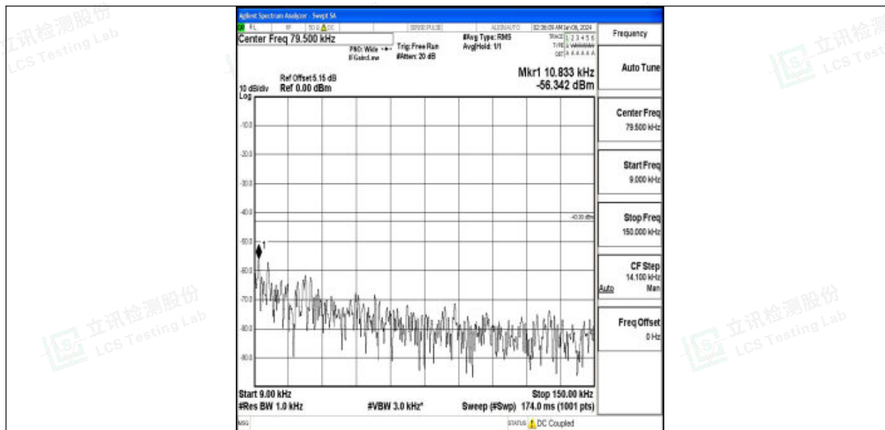
Band66_20MHz_16QAM_132322_1RB#0_0.009~0.15_0.009~0.15
