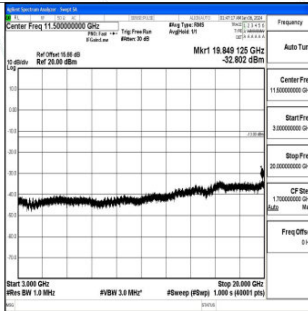
Band66_5MHz_16QAM_132647_1RB#0_3000~20000_3000~20000
