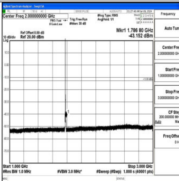
Band66_3MHz_16QAM_132657_1RB#0_1000~3000_1000~3000
