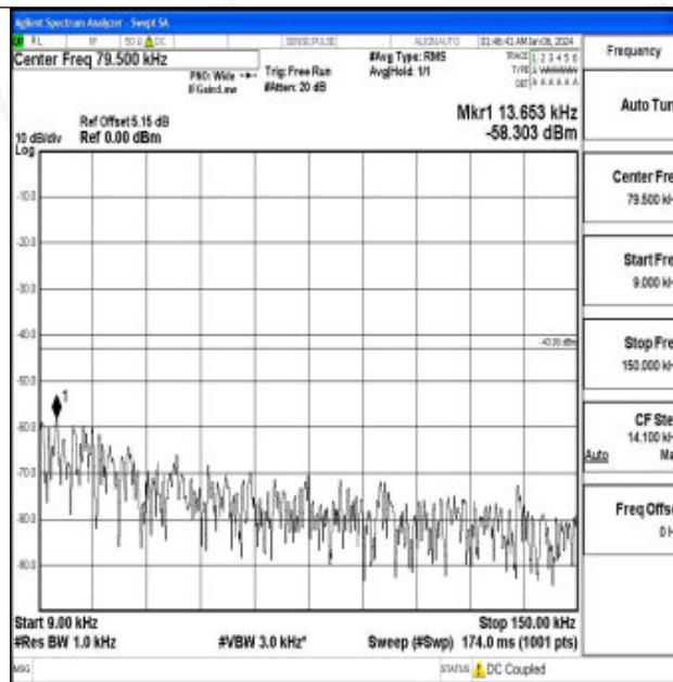
Band66_5MHz_16QAM_132647_1RB#0_0.009~0.15_0.009~0.15
