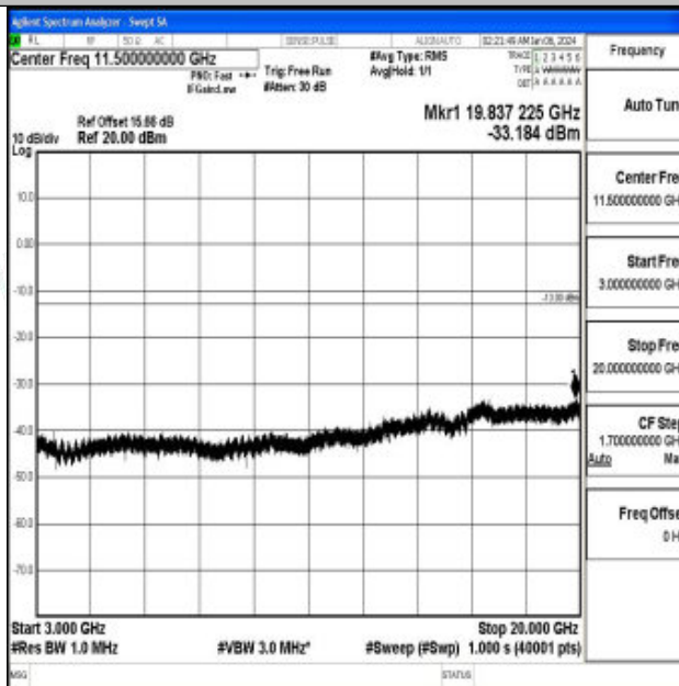
Band66_15MHz_QPSK_132597_1RB#0_3000~20000_3000~20000
