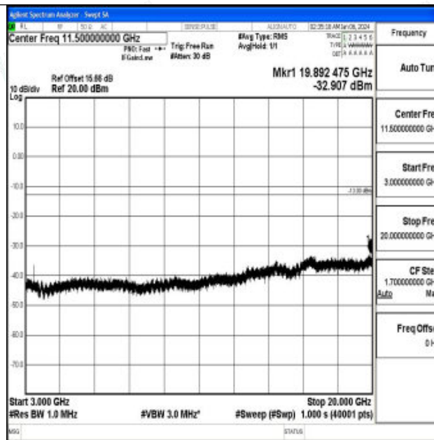
Band66_20MHz_16QAM_132072_1RB#0_3000~20000_3000~20000
