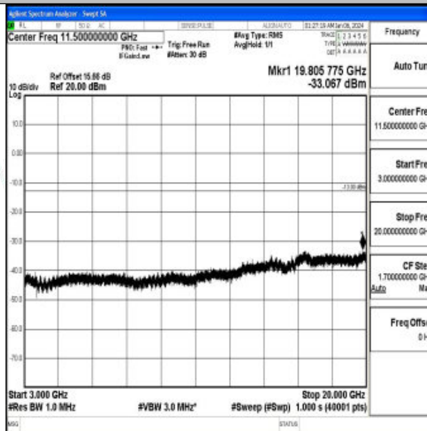
Band66_3MHz_QPSK_132657_1RB#0_3000~20000_3000~20000
