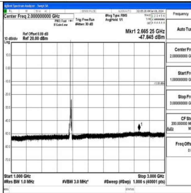
Band66_10MHz_QPSK_132622_1RB#0_1000~3000_1000~3000
