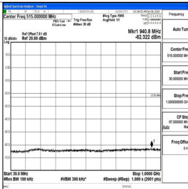
Band66_5MHz_16QAM_132647_1RB#0_30~1000_30~1000
