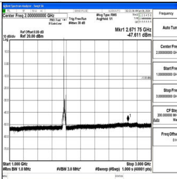
Band66_15MHz_QPSK_132597_1RB#0_1000~3000_1000~3000
