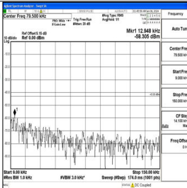
Band66_5MHz_QPSK_132647_1RB#0_0.009~0.15_0.009~0.15
