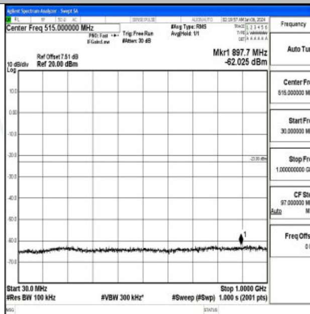
Band66_15MHz_QPSK_132322_1RB#0_30~1000_30~1000
