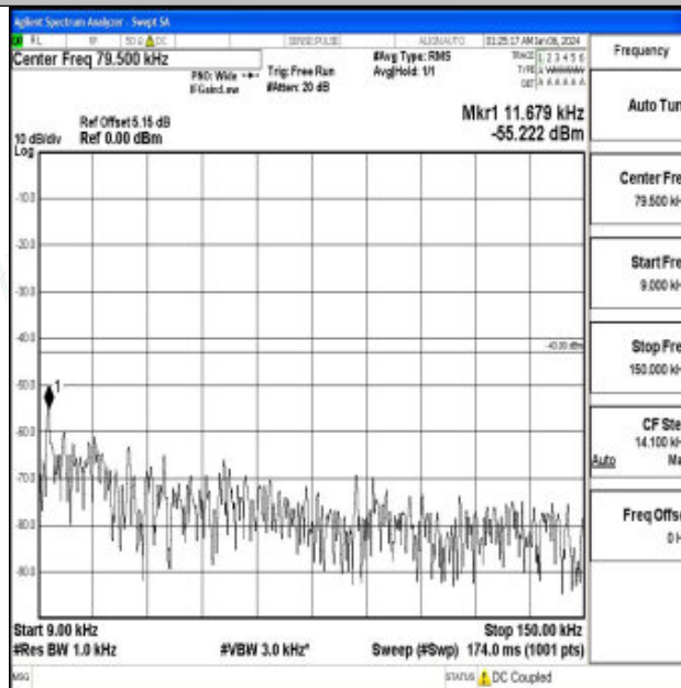
Band66_3MHz_QPSK_132322_1RB#0_0.009~0.15_0.009~0.15
