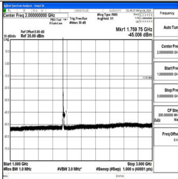
Band66_5MHz_16QAM_132322_1RB#0_1000~3000_1000~3000
