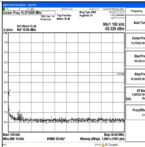
Band66_3MHz_QPSK_132657_1RB#0_0.15~30_0.15~30
