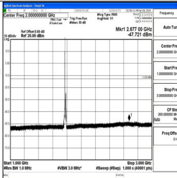
Band66_10MHz_16QAM_132622_1RB#0_1000~3000_1000~3000
