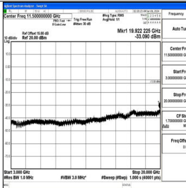
Band66_15MHz_QPSK_132322_1RB#0_3000~20000_3000~20000
