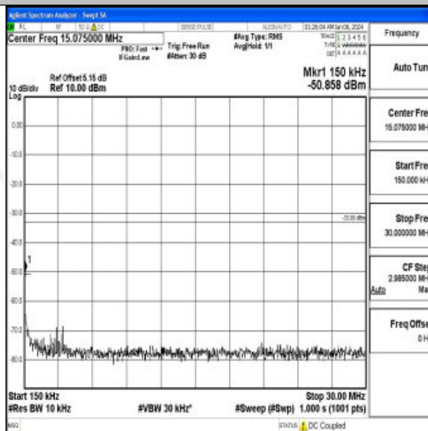
Band66_3MHz_16QAM_132322_1RB#0_0.15~30_0.15~30
