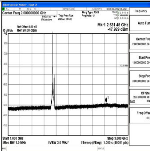
Band66_20MHz_16QAM_132322_1RB#0_1000~3000_1000~3000
