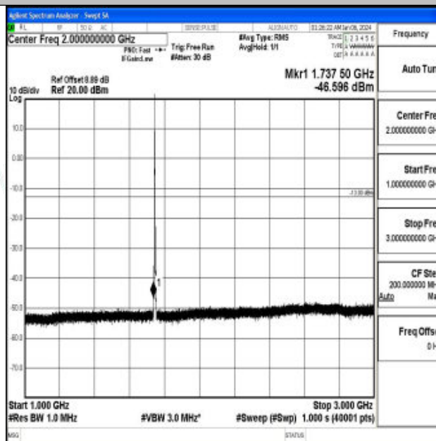
Band66_3MHz_16QAM_132322_1RB#0_1000~3000_1000~3000
