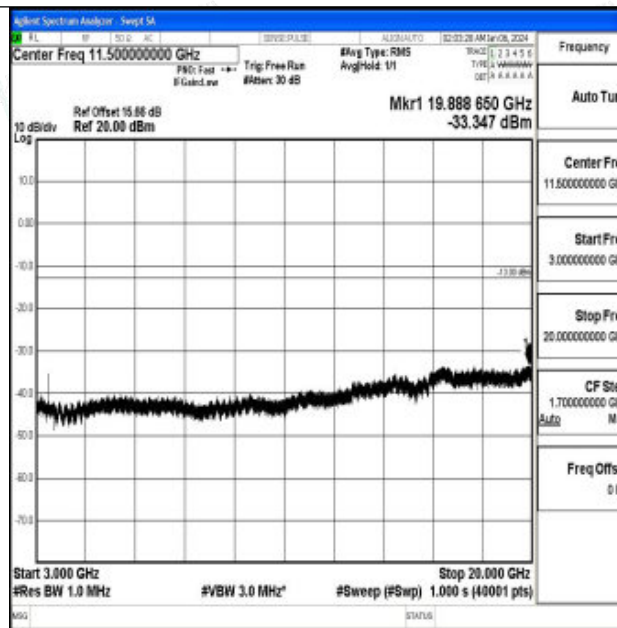
Band66_10MHz_16QAM_132022_1RB#0_3000~20000_3000~20000
