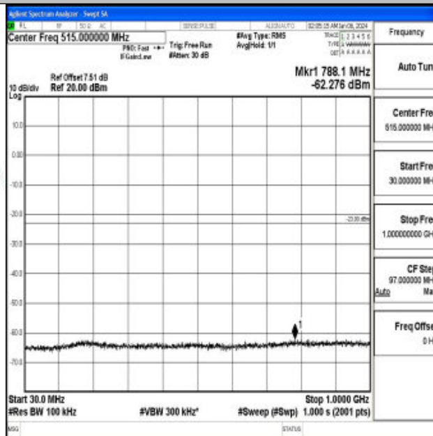
Band66_10MHz_QPSK_132622_1RB#0_30~1000_30~1000
