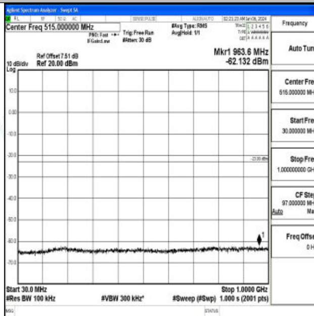
Band66_15MHz_QPSK_132597_1RB#0_30~1000_30~1000
