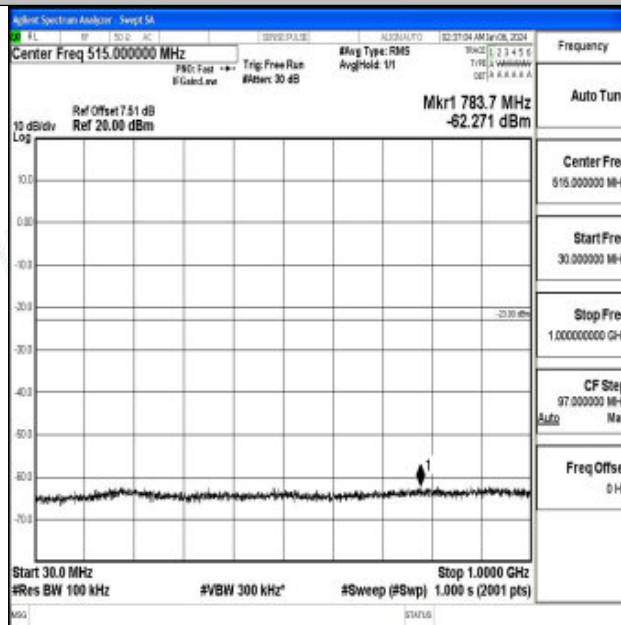
Band66_20MHz_QPSK_132572_1RB#0_30~1000_30~1000
