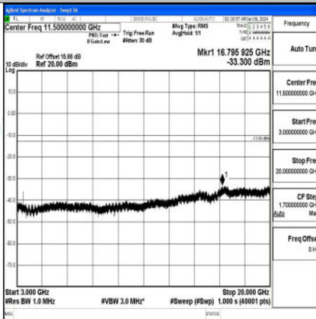
Band66_15MHz_QPSK_132047_1RB#0_3000~20000_3000~20000
