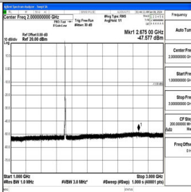
Band66_5MHz_16QAM_131997_1RB#0_1000~3000_1000~3000
