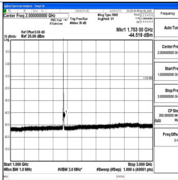
Band66_3MHz_QPSK_132322_1RB#0_1000~3000_1000~3000
