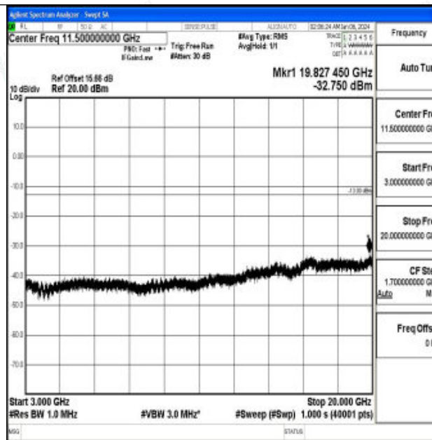
Band66_10MHz_16QAM_132622_1RB#0_3000~20000_3000~20000
