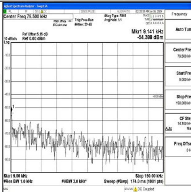
Band66_20MHz_QPSK_132072_1RB#0_0.009~0.15_0.009~0.15
