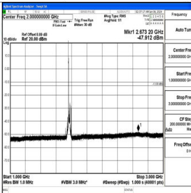
Band66_20MHz_QPSK_132572_1RB#0_1000~3000_1000~3000
