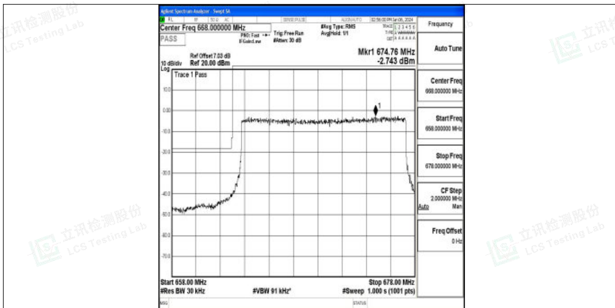
Band71_15MHz_16QAM_133197_75RB#0
