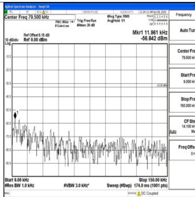
Band71_5MHz_QPSK_133297_1RB#0_0.009~0.15_0.009~0.15
