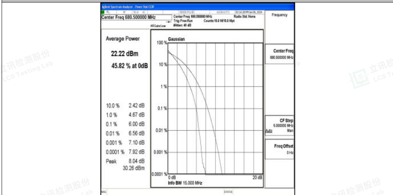
Band71-15MHz-QPSK-133297-75RB#0-PASS
