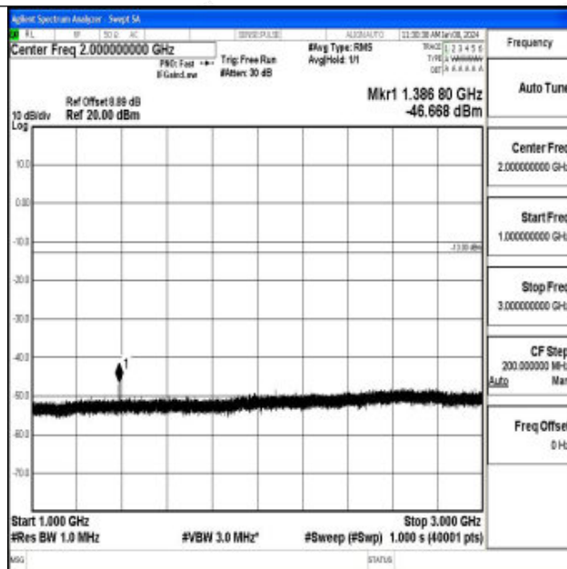
Band71_5MHz_16QAM_133447_1RB#0_1000~3000_1000~3000
