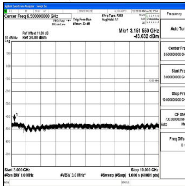
Band71_5MHz_QPSK_133447_1RB#0_3000~10000_3000~10000
