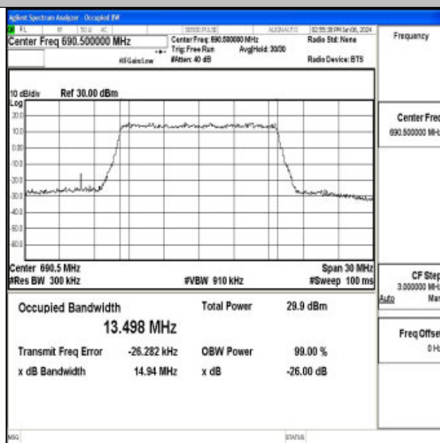
Band71-15MHz-16QAM-133397-75RB#0-PASS
