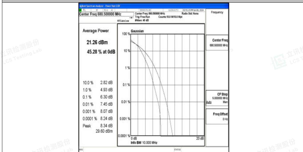
Band71-10MHz-16QAM-133297-50RB#0-PASS
