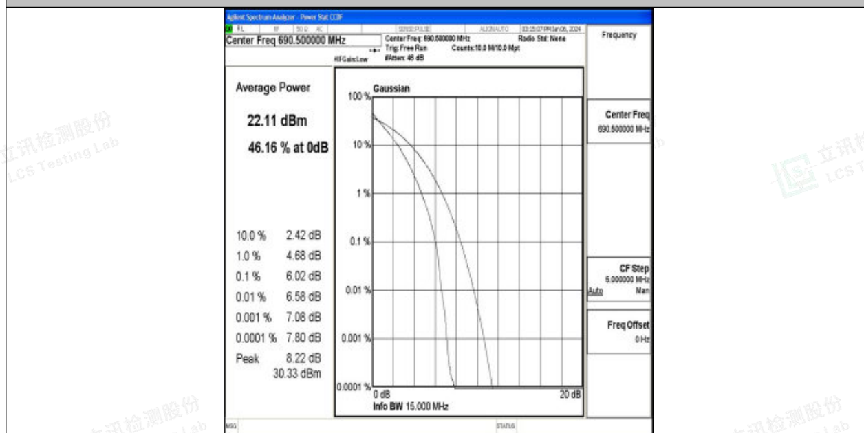
Band71-15MHz-QPSK-133397-75RB#0-PASS
