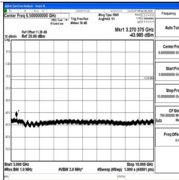
Band71_5MHz_QPSK_133147_1RB#0_3000~10000_3000~10000
