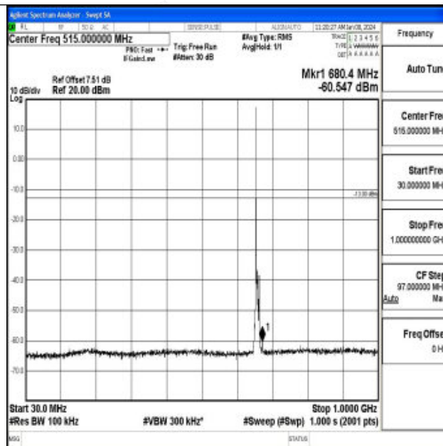
Band71_5MHz_QPSK_133147_1RB#0_30~1000_30~1000
