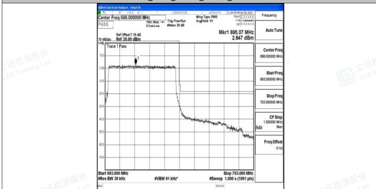
Band71_5MHz_QPSK_133447_25RB#0
