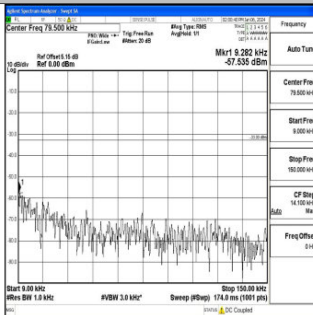
Band71_10MHz_QPSK_133297_1RB#0_0.009~0.15_0.009~0.15
