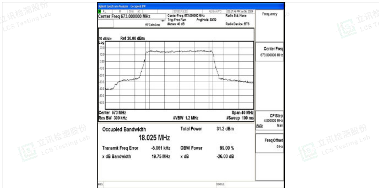
Band71-20MHz-QPSK-133222-100RB#0-PASS
