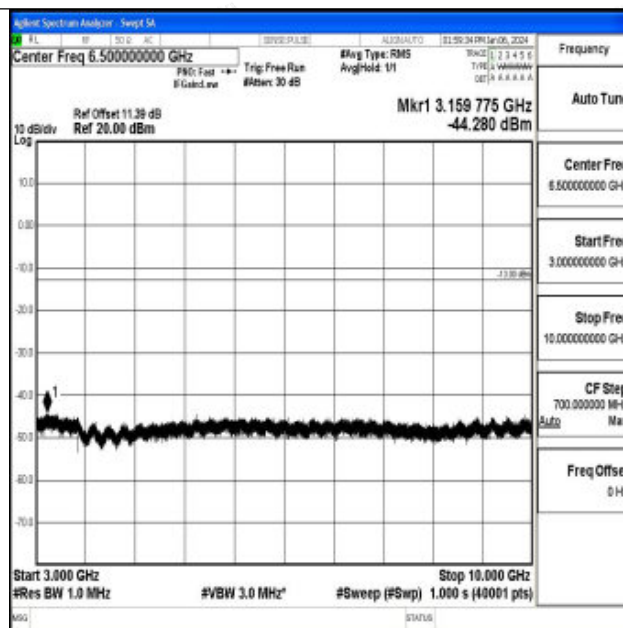
Band71_10MHz_16QAM_133172_1RB#0_3000~10000_3000~10000
