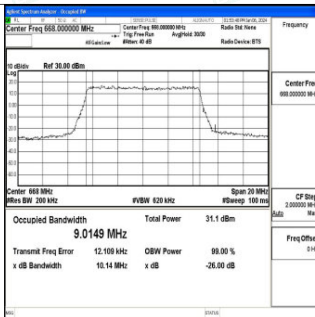
Band71-10MHz-QPSK-133172-50RB#0-PASS
