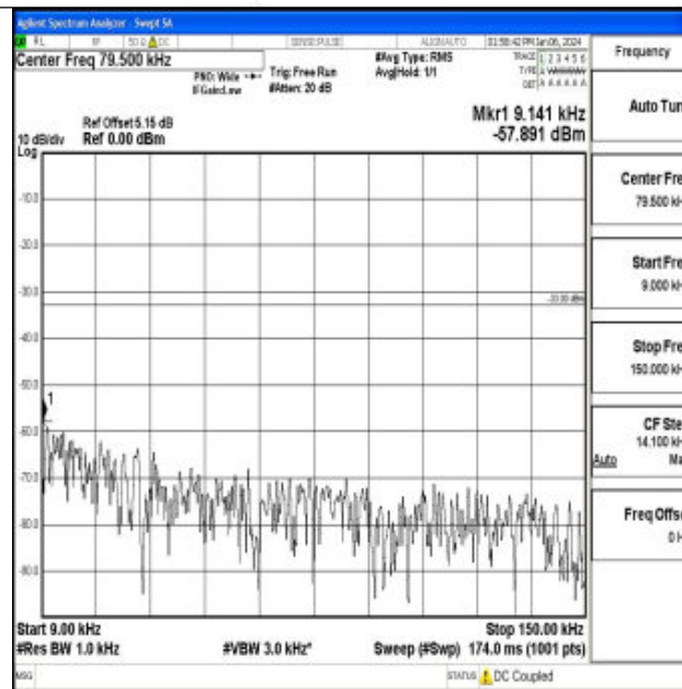
Band71_10MHz_16QAM_133172_1RB#0_0.009~0.15_0.009~0.15
