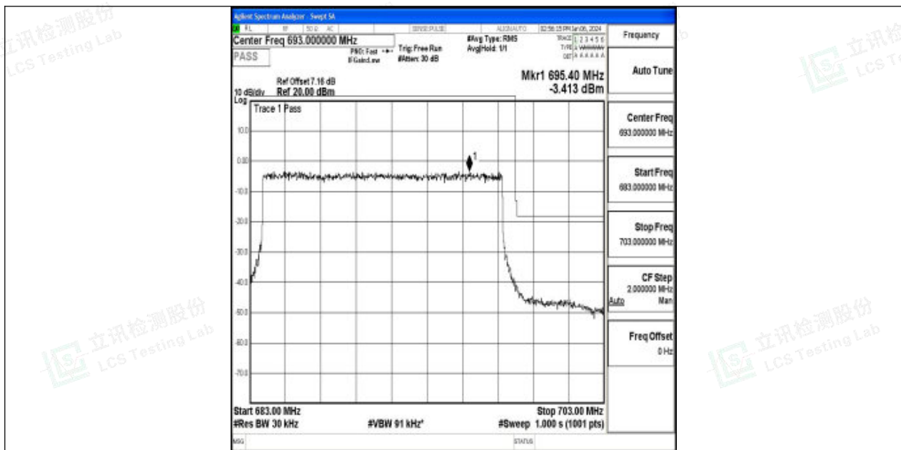
Band71_15MHz_16QAM_133397_75RB#0
