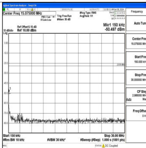
Band71_5MHz_16QAM_133447_1RB#0_0.15~30_0.15~30
