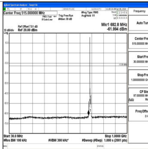
Band71_5MHz_QPSK_133447_1RB#0_30~1000_30~1000
