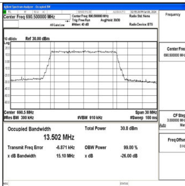
Band71-15MHz-QPSK-133397-75RB#0-PASS
