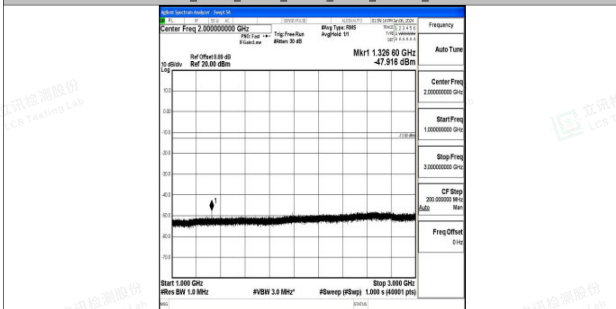
Band71_10MHz_16QAM_133172_1RB#0_1000~3000_1000~3000
