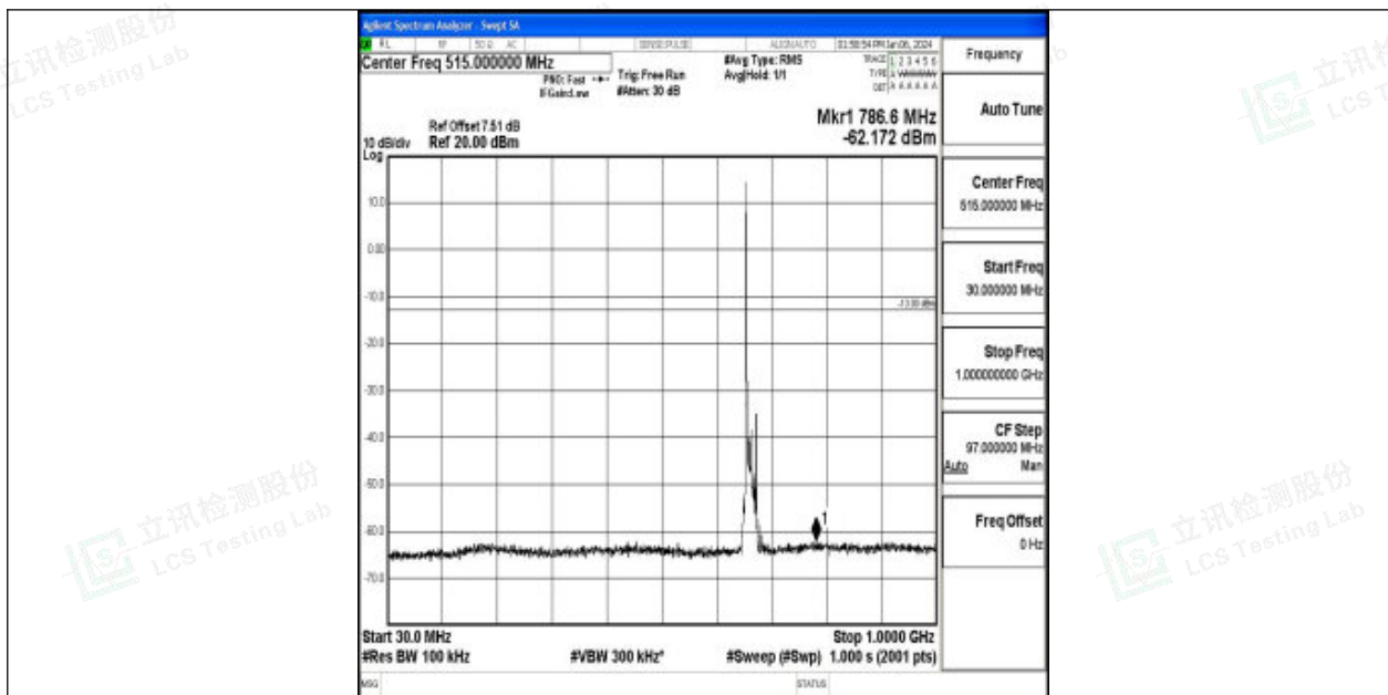
Band71_10MHz_16QAM_133172_1RB#0_30~1000_30~1000
