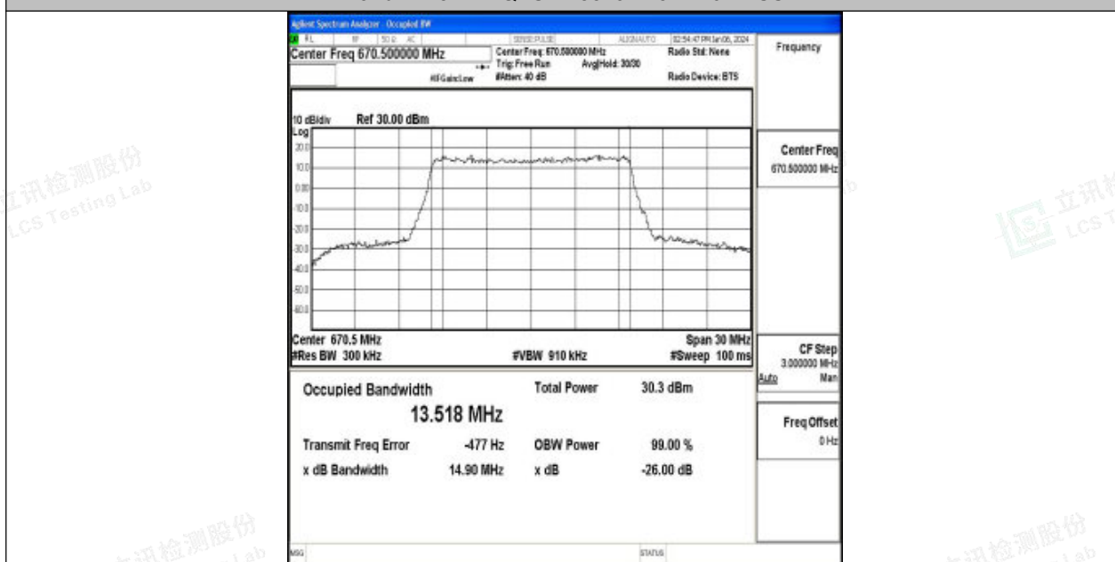
Band71-15MHz-16QAM-133197-75RB#0-PASS
