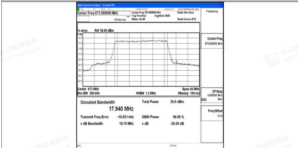
Band71-20MHz-16QAM-133222-100RB#0-PASS
