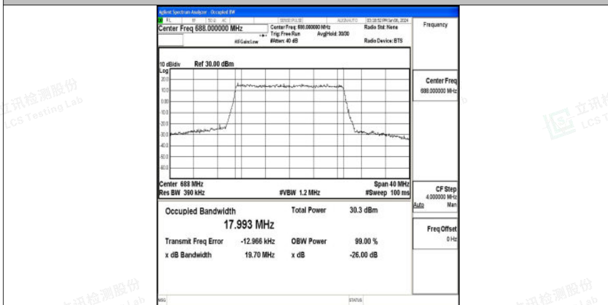
Band71-20MHz-16QAM-133372-100RB#0-PASS
