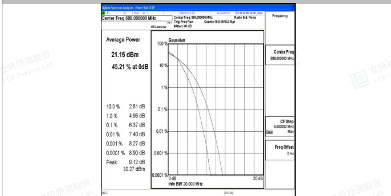
Band71-20MHz-QPSK-133372-100RB#0-PASS
