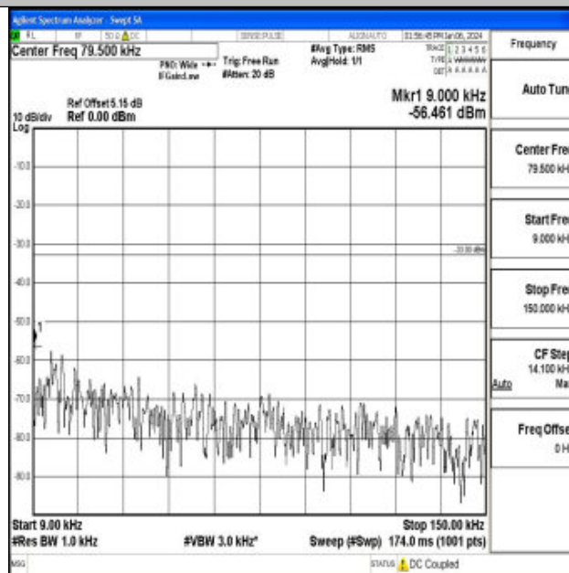
Band71_10MHz_QPSK_133172_1RB#0_0.009~0.15_0.009~0.15
