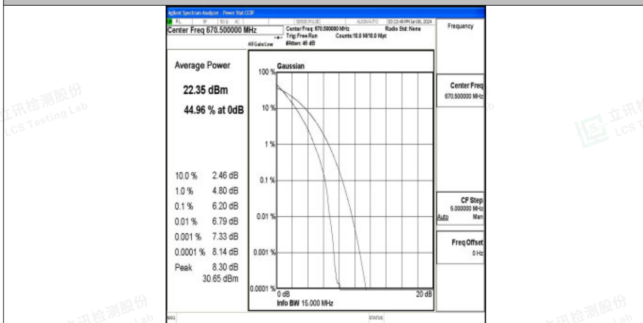
Band71-15MHz-QPSK-133197-75RB#0-PASS
