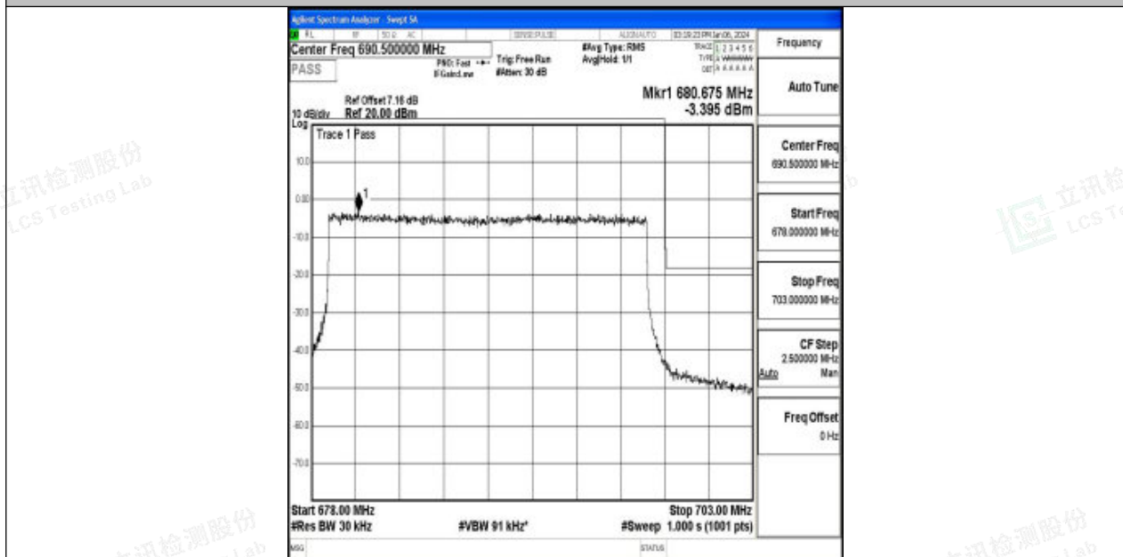
Band71_20MHz_QPSK_133372_100RB#0
