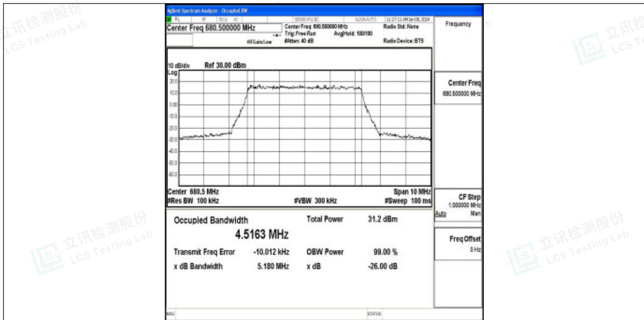
Band71-5MHz-QPSK-133297-25RB#0-PASS
