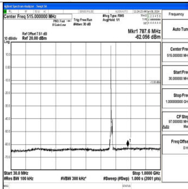
Band71_5MHz_QPSK_133297_1RB#0_30~1000_30~1000
