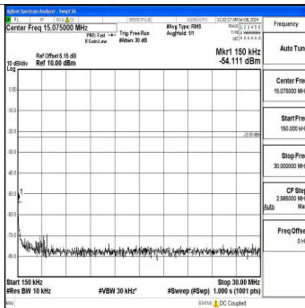
Band71_5MHz_16QAM_133147_1RB#0_0.15~30_0.15~30
