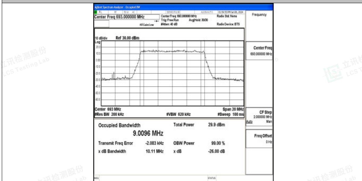
Band71-10MHz-16QAM-133422-50RB#0-PASS
