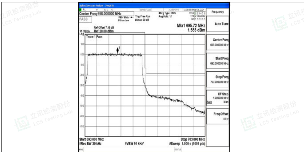
Band71_5MHz_16QAM_133447_25RB#0
