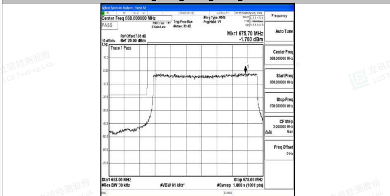
Band71_15MHz_QPSK_133197_75RB#0
