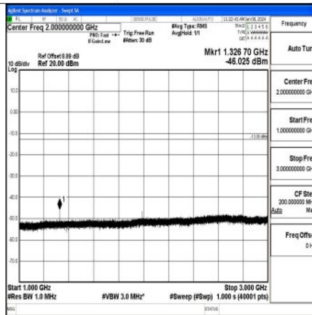
Band71_5MHz_16QAM_133147_1RB#0_1000~3000_1000~3000
