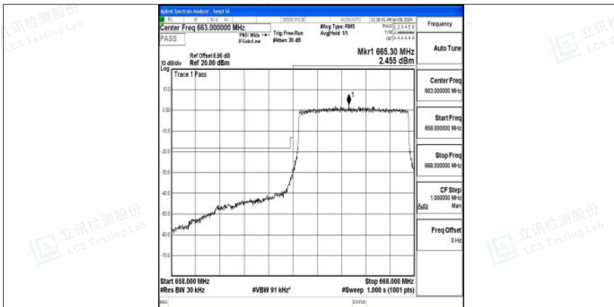
Band71_5MHz_16QAM_133147_25RB#0
