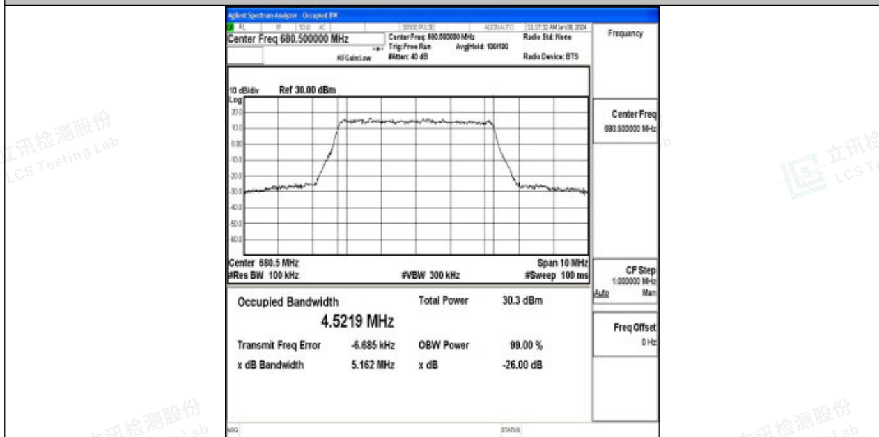
Band71-5MHz-16QAM-133297-25RB#0-PASS
