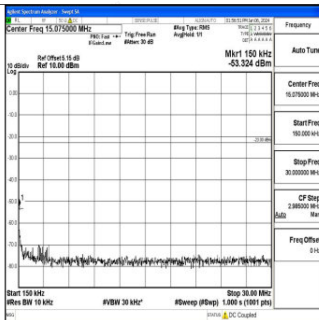
Band71_10MHz_QPSK_133172_1RB#0_0.15~30_0.15~30
