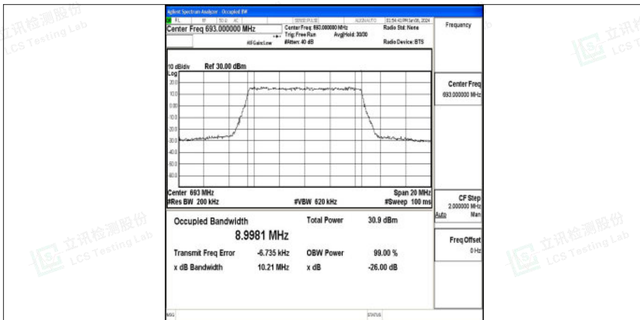
Band71-10MHz-QPSK-133422-50RB#0-PASS
