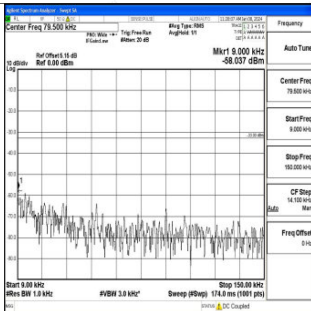
Band71_5MHz_QPSK_133447_1RB#0_0.009~0.15_0.009~0.15
