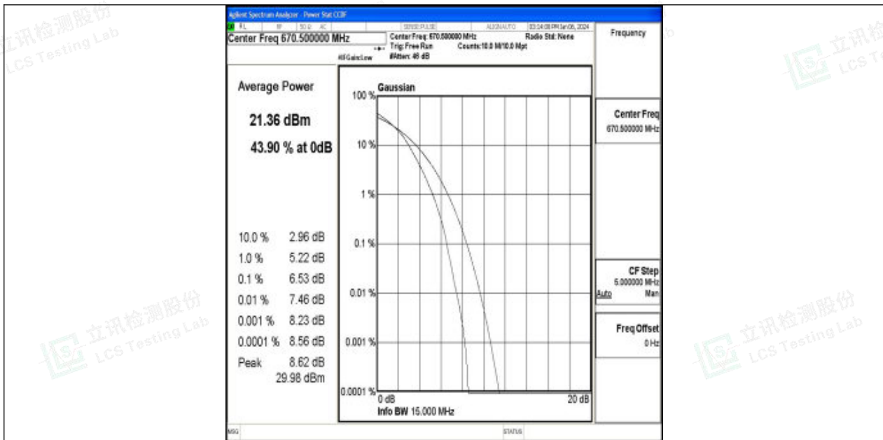
Band71-15MHz-16QAM-133197-75RB#0-PASS
