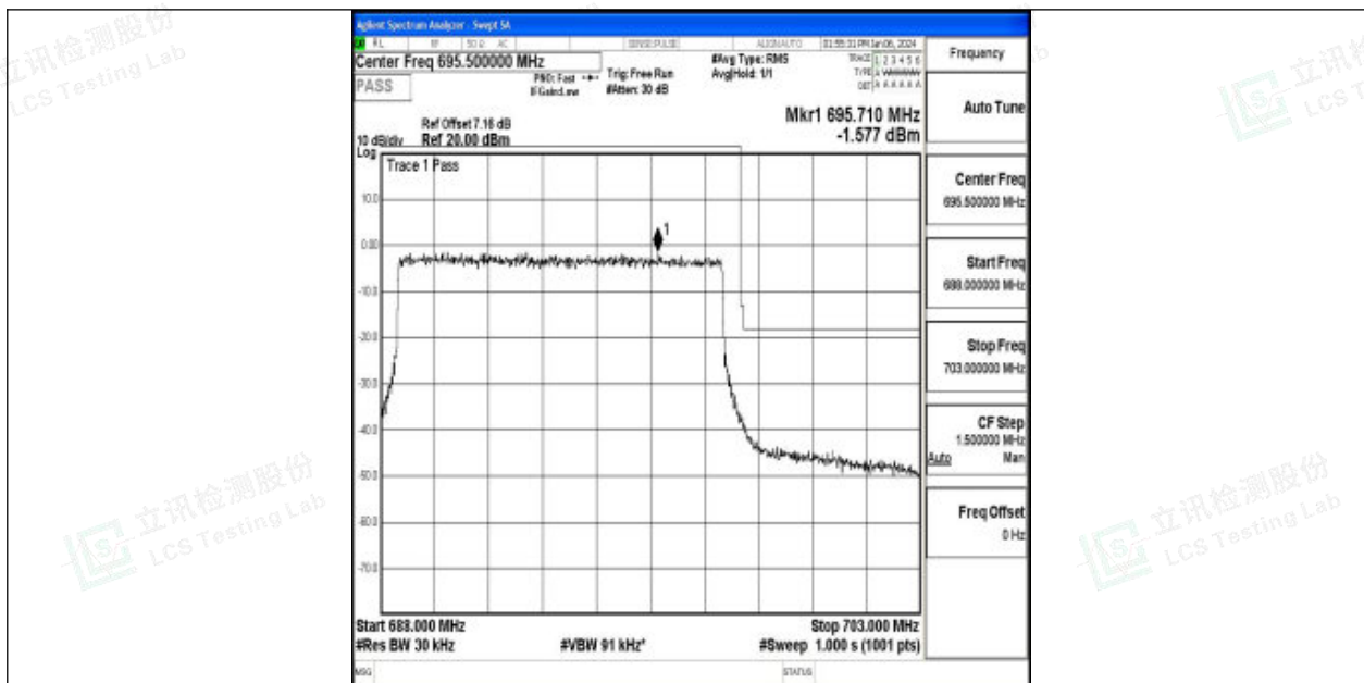
Band71_10MHz_16QAM_133422_50RB#0
