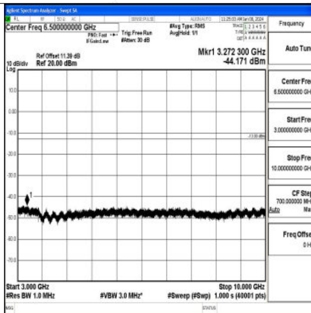
Band71_5MHz_QPSK_133297_1RB#0_3000~10000_3000~10000
