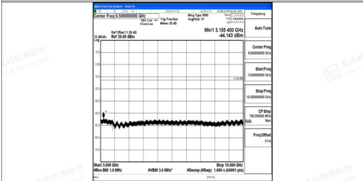
Band71_15MHz_QPSK_133197_1RB#0_3000~10000_3000~10000
