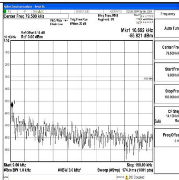
Band71_10MHz_16QAM_133422_1RB#0_0.009~0.15_0.009~0.15
