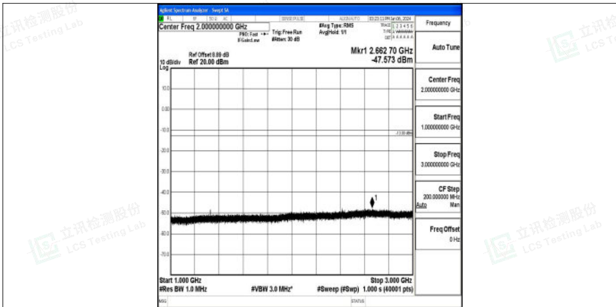
Band71_20MHz_16QAM_133222_1RB#0_1000~3000_1000~3000
