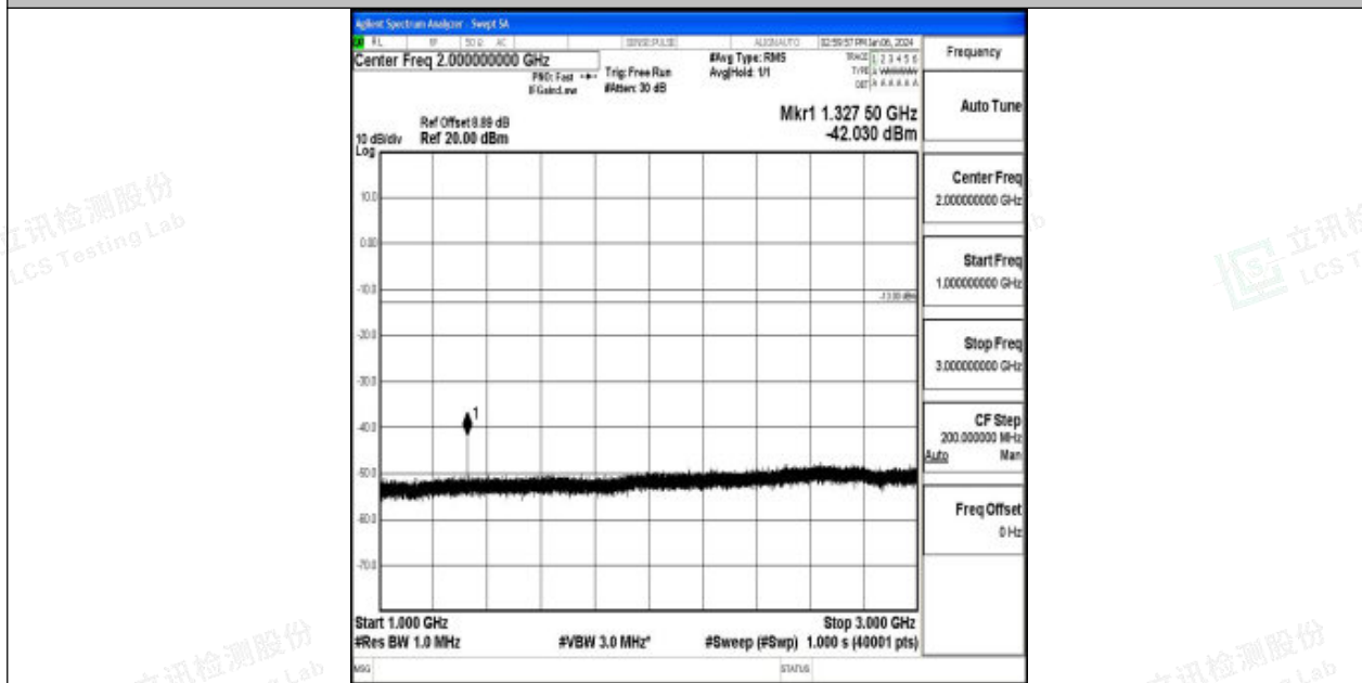
Band71_15MHz_16QAM_133197_1RB#0_1000~3000_1000~3000
