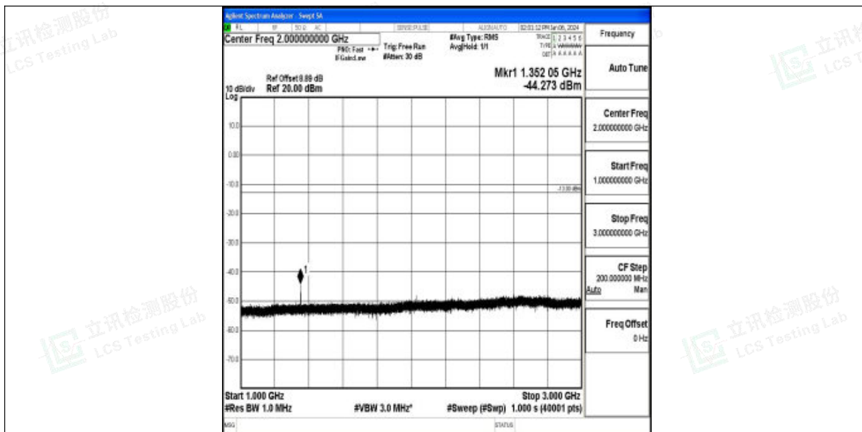
Band71_10MHz_QPSK_133297_1RB#0_1000~3000_1000~3000
