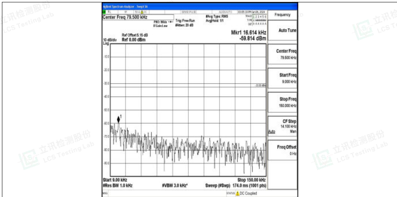
Band71_15MHz_QPSK_133397_1RB#0_0.009~0.15_0.009~0.15
