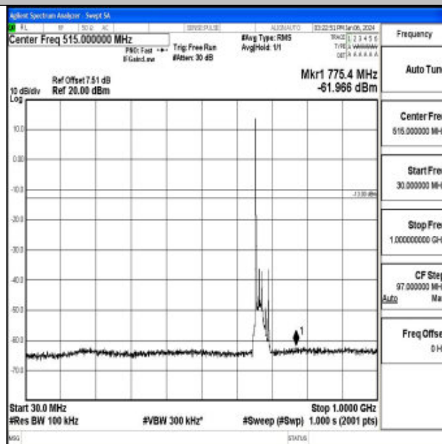
Band71_20MHz_16QAM_133222_1RB#0_30~1000_30~1000
