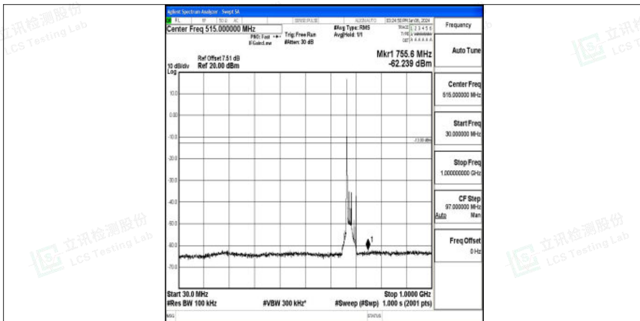
Band71_20MHz_QPSK_133322_1RB#0_30~1000_30~1000
