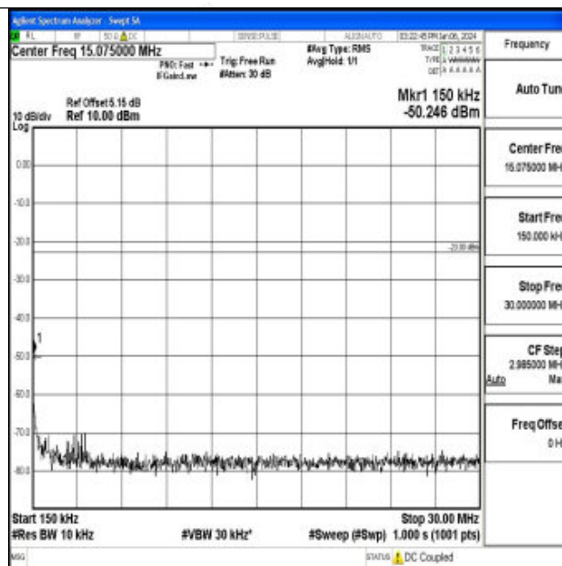
Band71_20MHz_16QAM_133222_1RB#0_0.15~30_0.15~30
