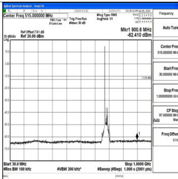
Band71_20MHz_16QAM_133372_1RB#0_30~1000_30~1000
