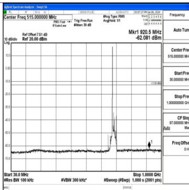
Band71_15MHz_16QAM_133397_1RB#0_30~1000_30~1000
