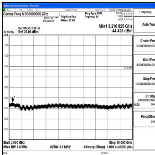
Band71_15MHz_16QAM_133197_1RB#0_3000~10000_3000~10000
