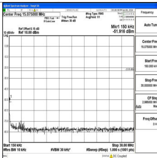
Band71_20MHz_QPSK_133372_1RB#0_0.15~30_0.15~30
