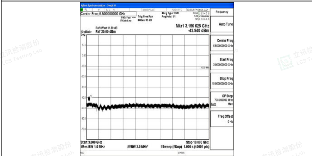
Band71_20MHz_QPSK_133372_1RB#0_3000~10000_3000~10000
