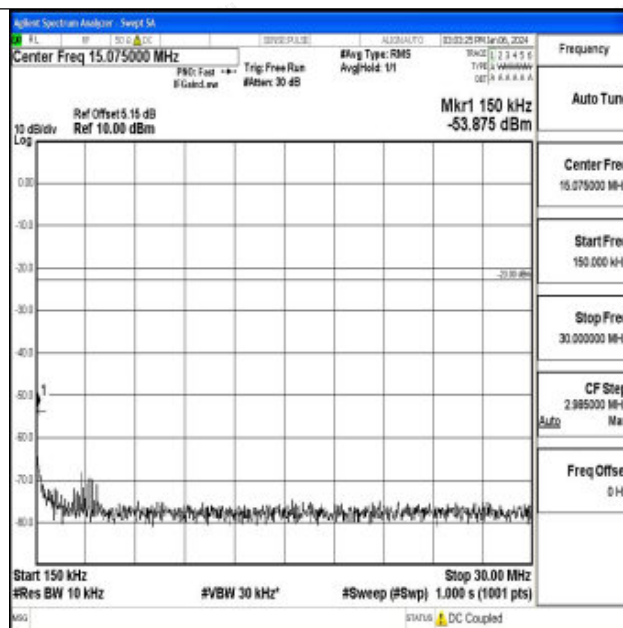
Band71_15MHz_16QAM_133297_1RB#0_0.15~30_0.15~30
