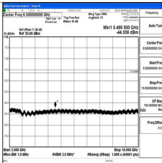
Band71_20MHz_16QAM_133372_1RB#0_3000~10000_3000~10000
