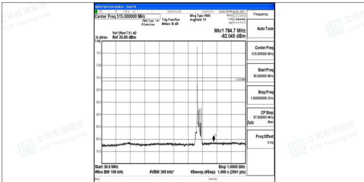
Band71_15MHz_QPSK_133297_1RB#0_30~1000_30~1000
