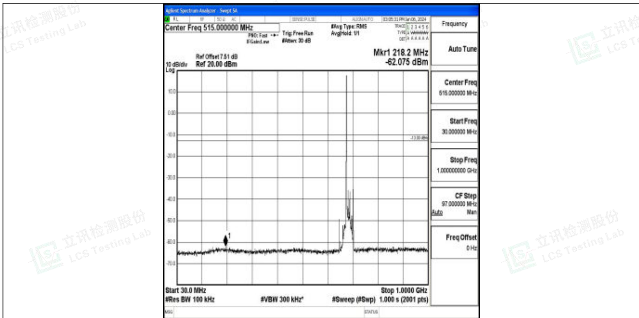
Band71_15MHz_QPSK_133397_1RB#0_30~1000_30~1000
