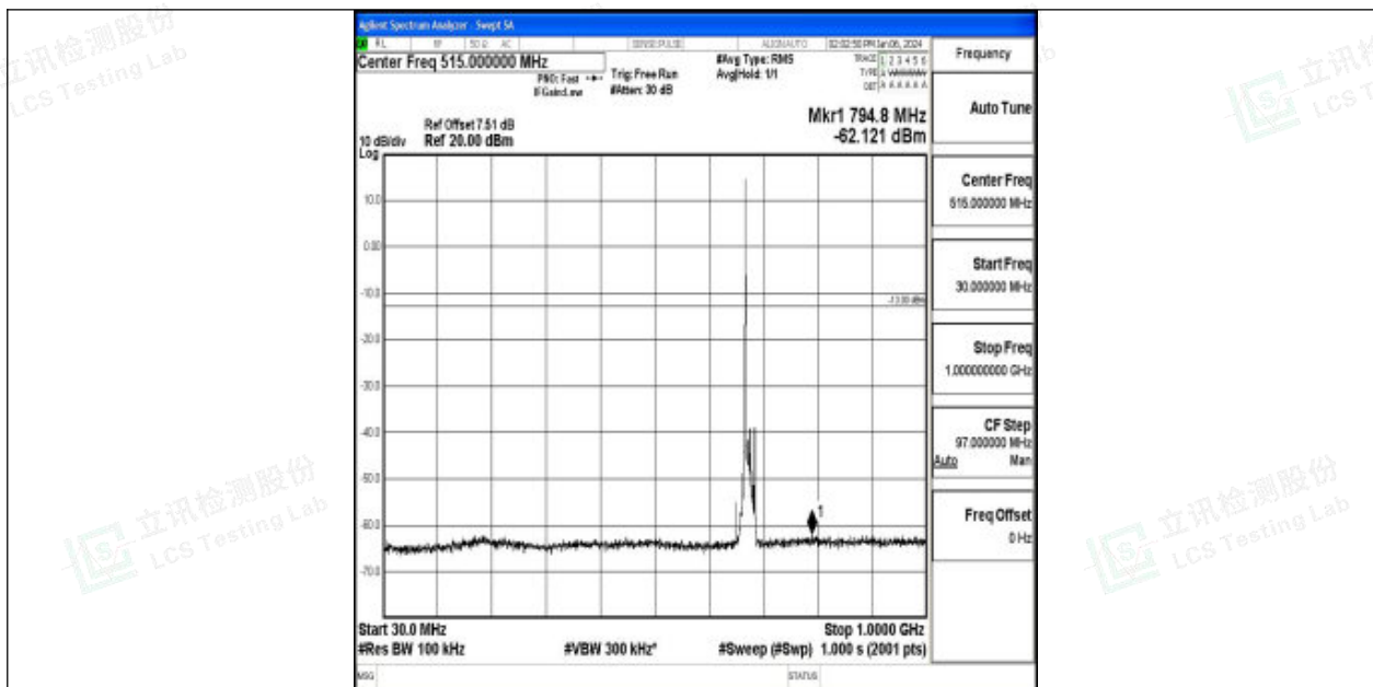
Band71_10MHz_16QAM_133297_1RB#0_30~1000_30~1000
