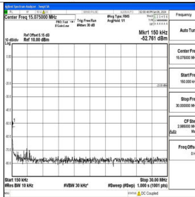
Band71_10MHz_QPSK_133297_1RB#0_0.15~30_0.15~30
