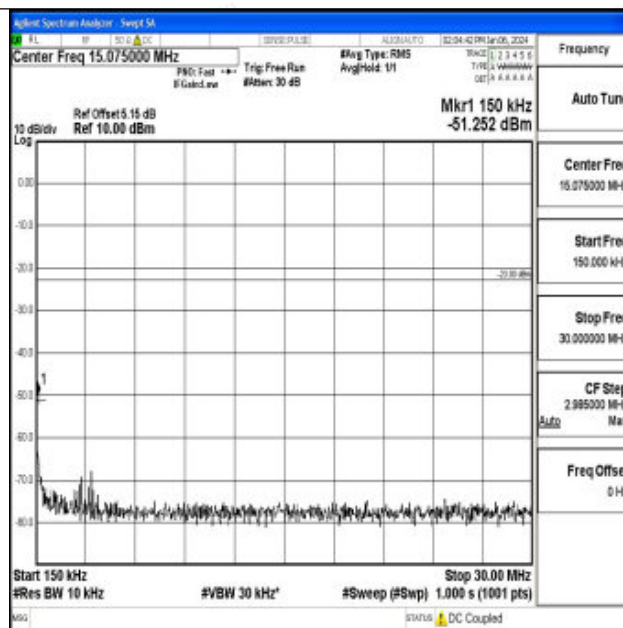
Band71_10MHz_QPSK_133422_1RB#0_0.15~30_0.15~30
