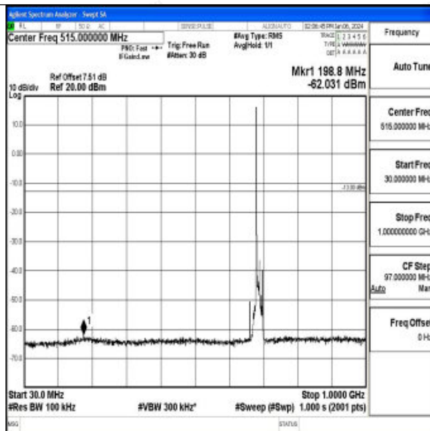
Band71_10MHz_16QAM_133422_1RB#0_30~1000_30~1000
