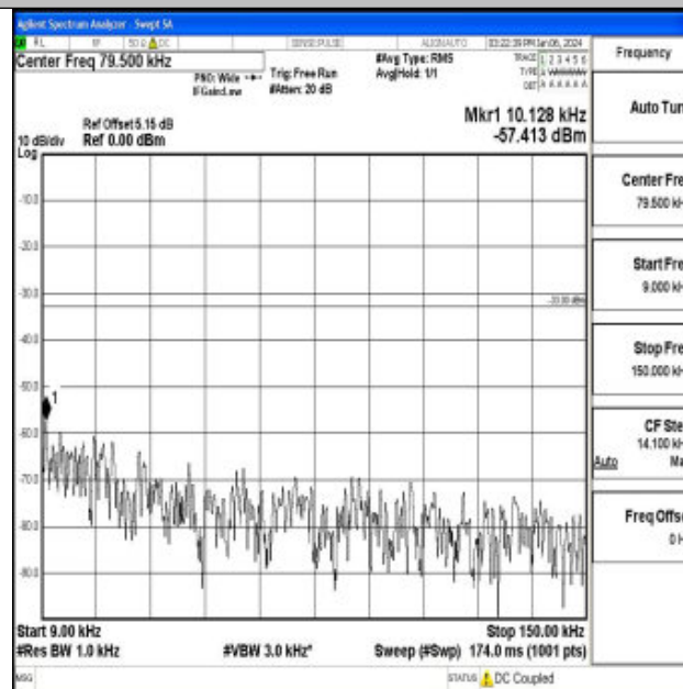
Band71_20MHz_16QAM_133222_1RB#0_0.009~0.15_0.009~0.15
