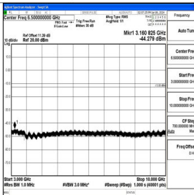
Band71_10MHz_16QAM_133422_1RB#0_3000~10000_3000~10000
