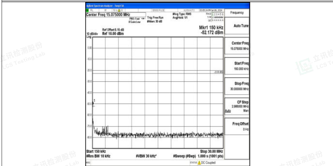
Band71_15MHz_QPSK_133397_1RB#0_0.15~30_0.15~30
