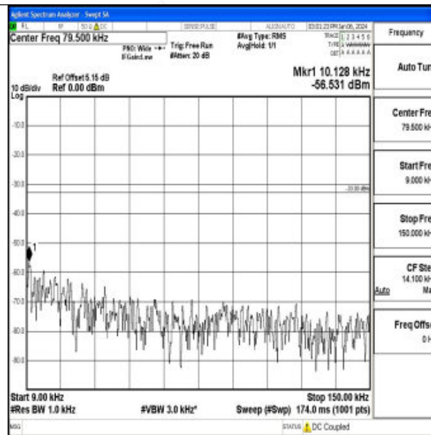
Band71_15MHz_QPSK_133297_1RB#0_0.009~0.15_0.009~0.15
