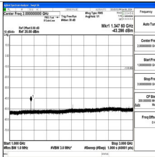
Band71_15MHz_16QAM_133297_1RB#0_1000~3000_1000~3000
