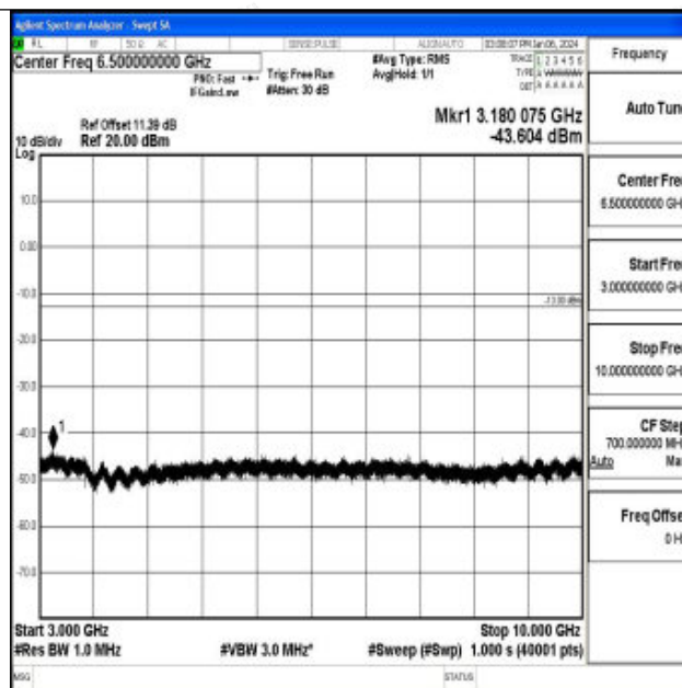
Band71_15MHz_16QAM_133397_1RB#0_3000~10000_3000~10000
