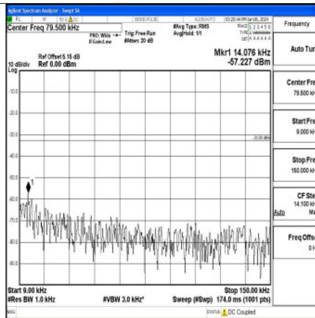
Band71_20MHz_QPSK_133222_1RB#0_0.009~0.15_0.009~0.15
