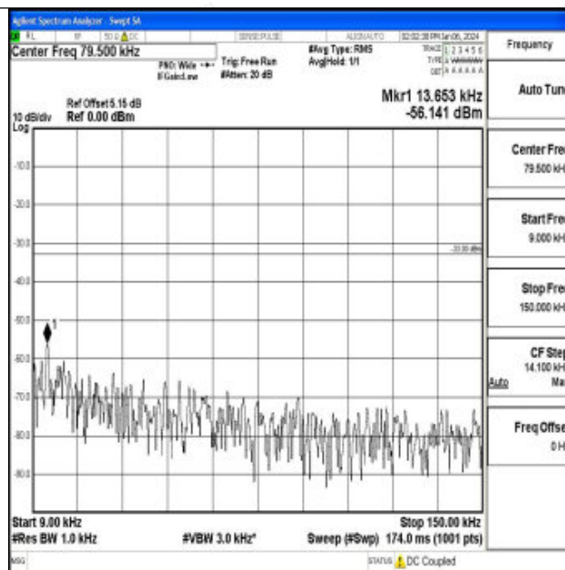
Band71_10MHz_16QAM_133297_1RB#0_0.009~0.15_0.009~0.15
