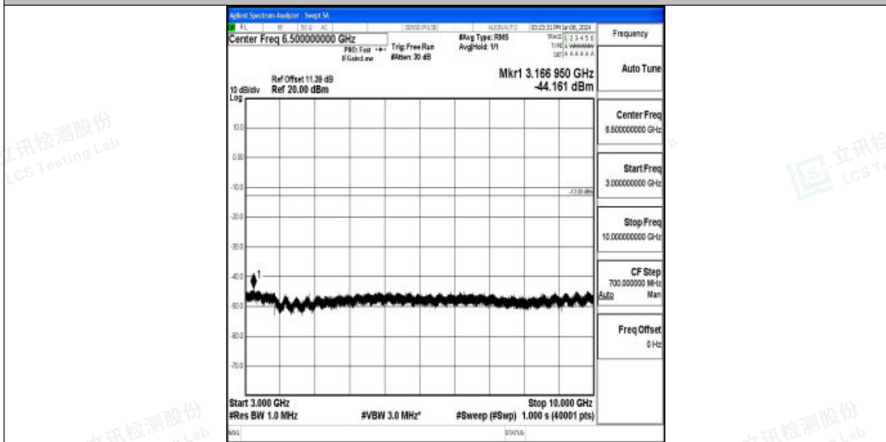
Band71_20MHz_16QAM_133222_1RB#0_3000~10000_3000~10000
