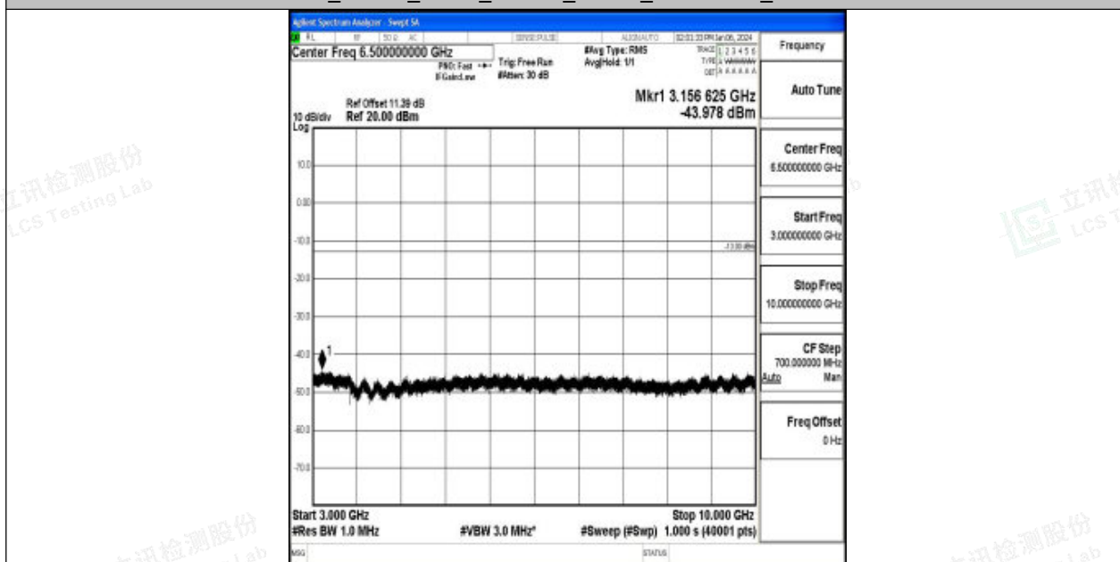
Band71_10MHz_QPSK_133297_1RB#0_3000~10000_3000~10000
