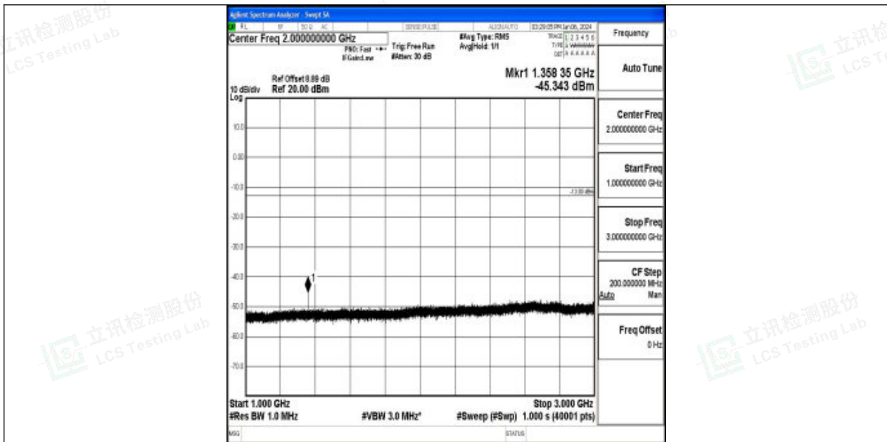
Band71_20MHz_QPSK_133372_1RB#0_1000~3000_1000~3000
