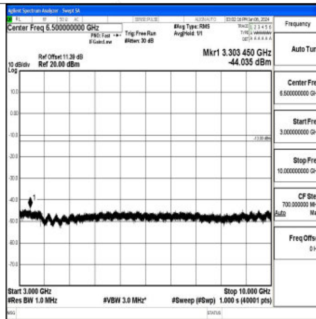
Band71_15MHz_QPSK_133297_1RB#0_3000~10000_3000~10000
