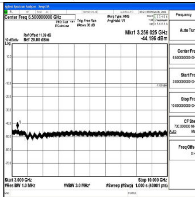
Band71_20MHz_QPSK_133222_1RB#0_3000~10000_3000~10000
