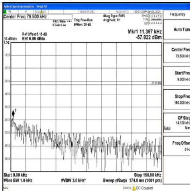
Band71_15MHz_16QAM_133397_1RB#0_0.009~0.15_0.009~0.15
