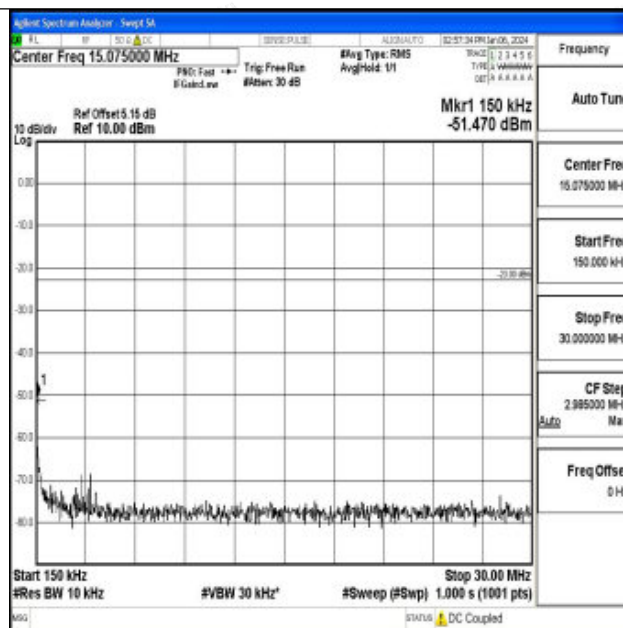
Band71_15MHz_QPSK_133197_1RB#0_0.15~30_0.15~30
