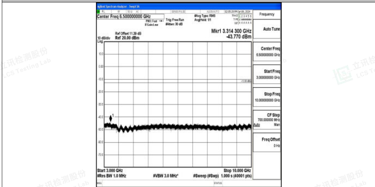
Band71_10MHz_QPSK_133422_1RB#0_3000~10000_3000~10000
