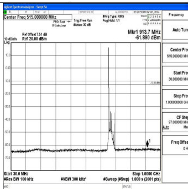
Band71_20MHz_QPSK_133222_1RB#0_30~1000_30~1000
