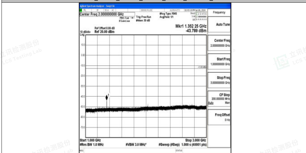
Band71_10MHz_16QAM_133297_1RB#0_1000~3000_1000~3000
