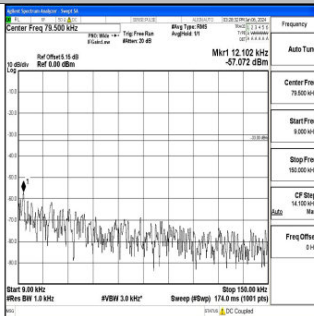
Band71_20MHz_QPSK_133372_1RB#0_0.009~0.15_0.009~0.15
