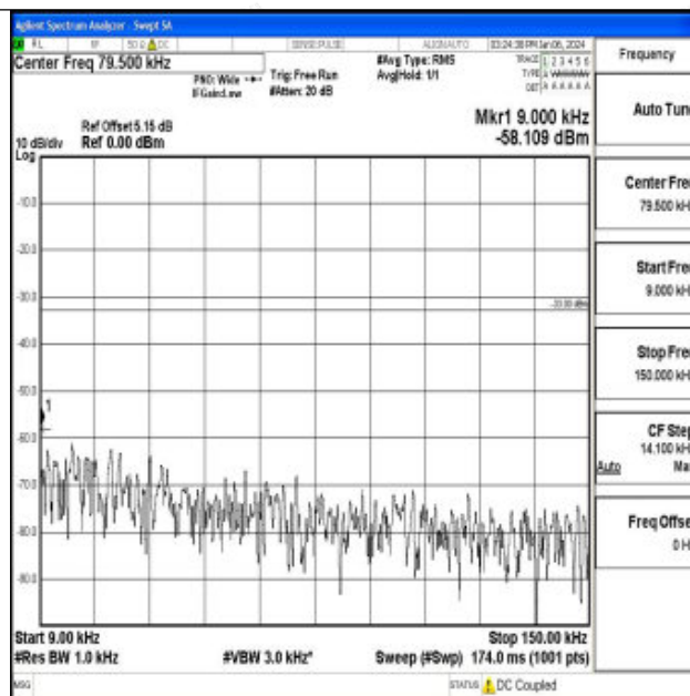
Band71_20MHz_QPSK_133322_1RB#0_0.009~0.15_0.009~0.15
