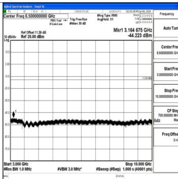
Band71_10MHz_16QAM_133297_1RB#0_3000~10000_3000~10000
