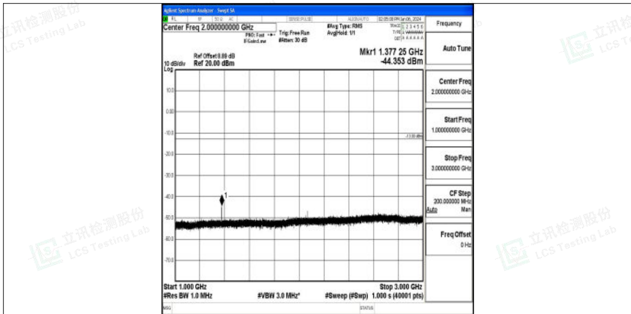
Band71_10MHz_QPSK_133422_1RB#0_1000~3000_1000~3000
