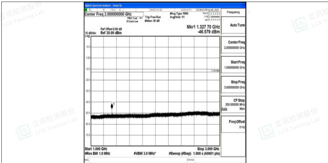
Band71_15MHz_QPSK_133197_1RB#0_1000~3000_1000~3000
