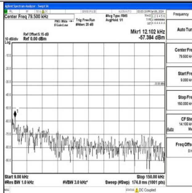
Band71_15MHz_16QAM_133297_1RB#0_0.009~0.15_0.009~0.15
