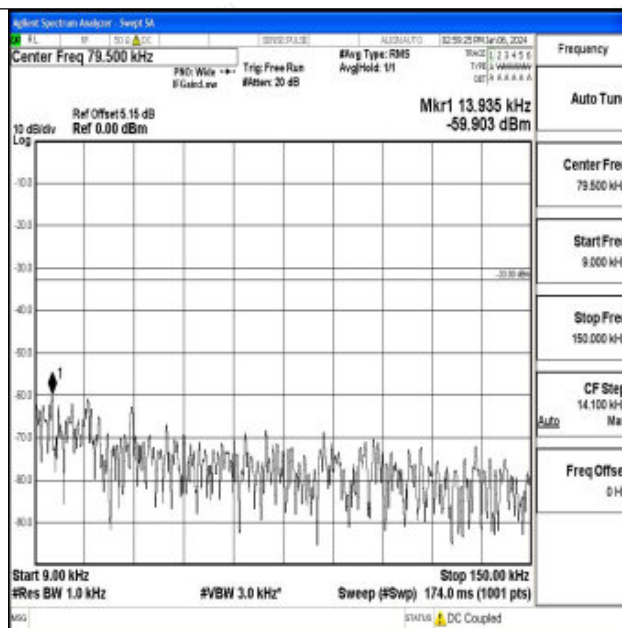
Band71_15MHz_16QAM_133197_1RB#0_0.009~0.15_0.009~0.15
