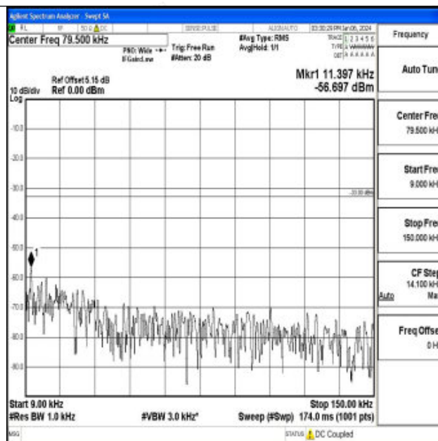
Band71_20MHz_16QAM_133372_1RB#0_0.009~0.15_0.009~0.15
