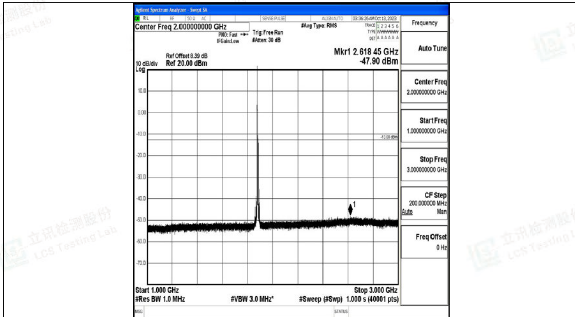
Band2_10MHz_16QAM_18900_1RB#0_1000~3000_1000~3000
