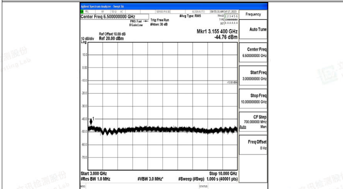
Band26_3MHz_16QAM_26705_1RB#0_3000~10000_3000~10000
