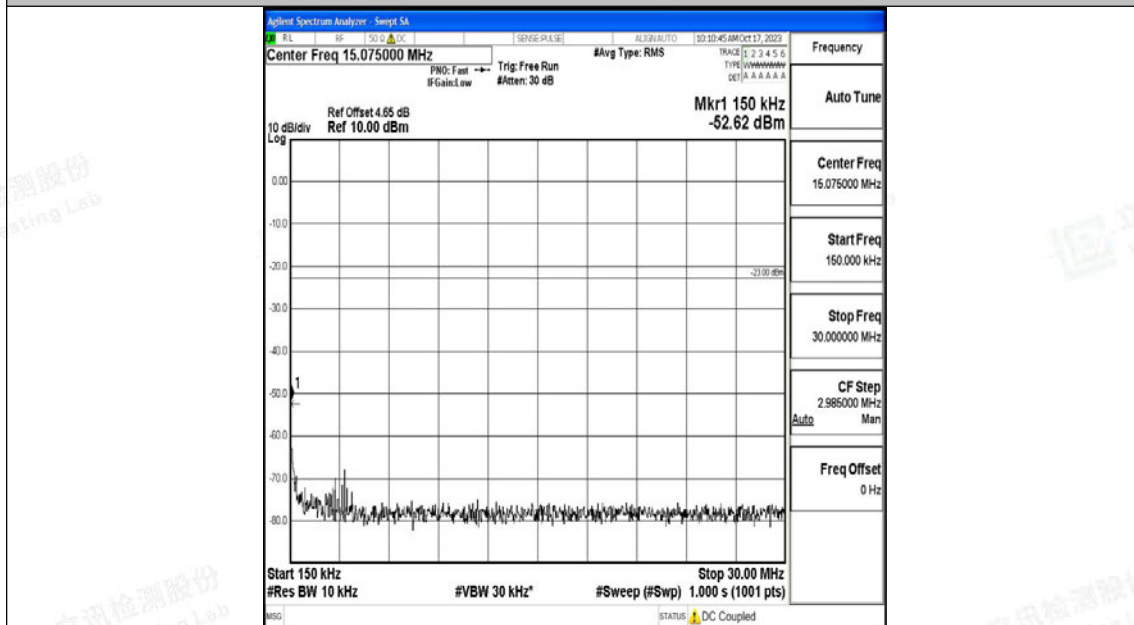
Band26_5MHz_QPSK_26740_1RB#0_0.15~30_0.15~30
