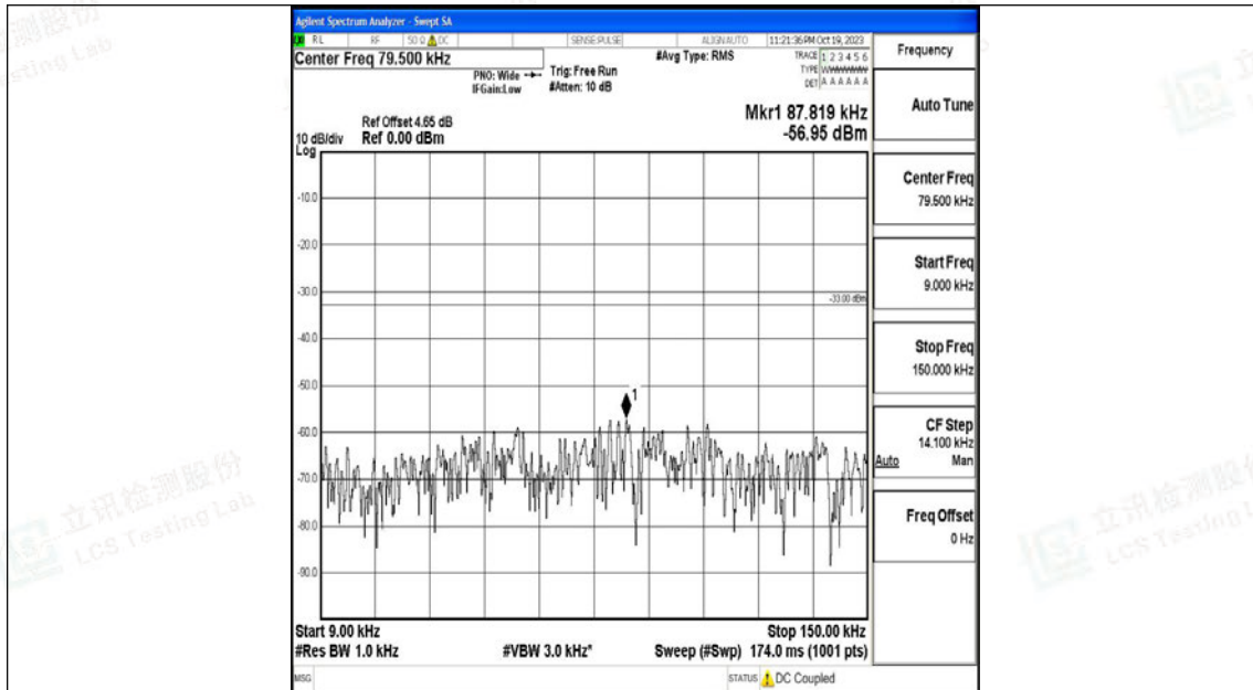
Band26_10MHz_QPSK_26990_1RB#0_0.009~0.15_0.009~0.15
