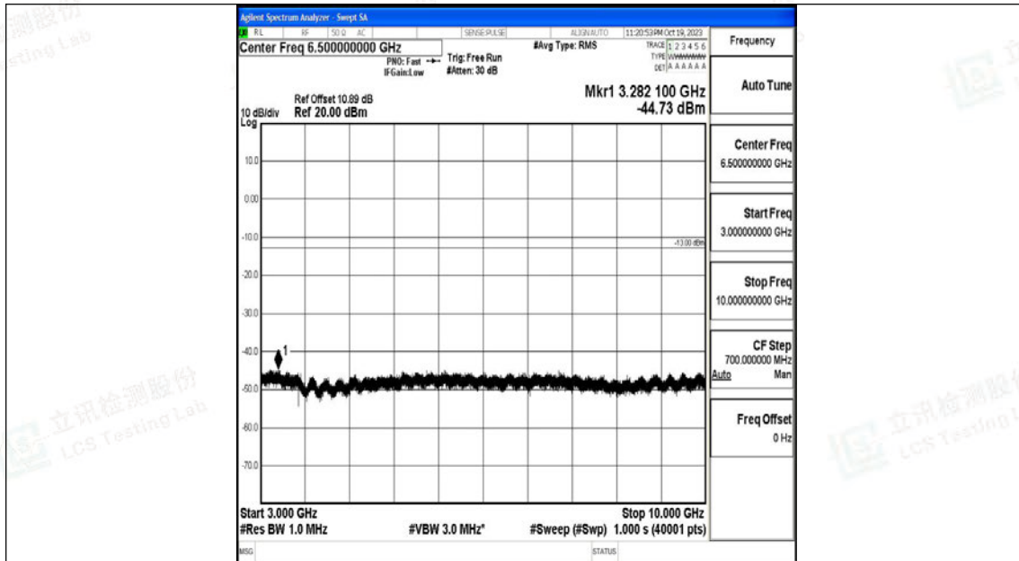
Band26_10MHz_QPSK_26915_1RB#0_3000~10000_3000~10000
