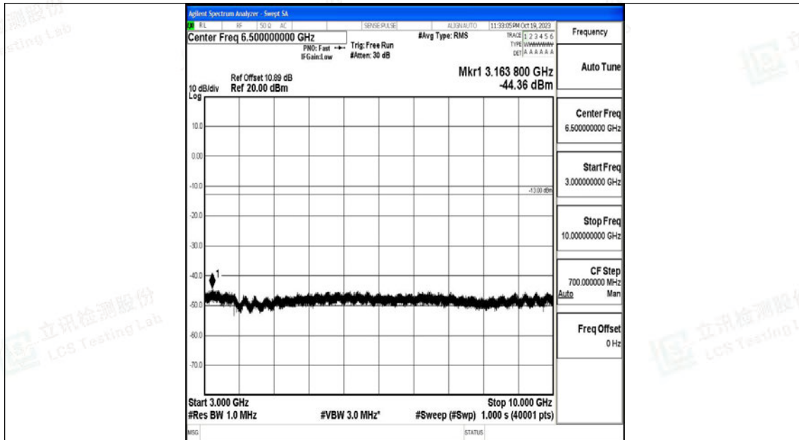
Band26_15MHz_QPSK_26865_1RB#0_3000~10000_3000~10000
