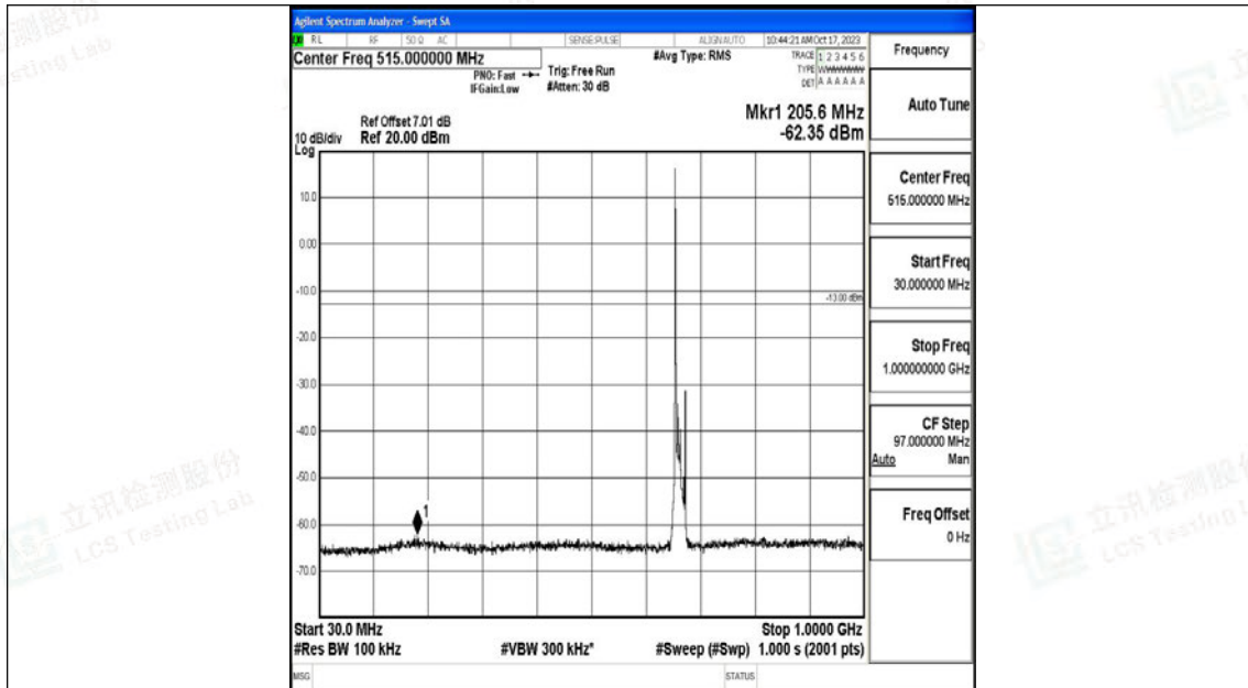
Band71_10MHz_QPSK_133172_1RB#0_30~1000_30~1000
