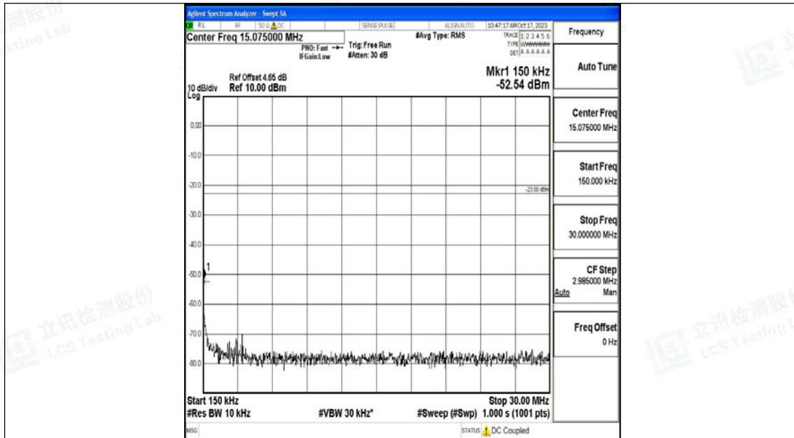
Band71_10MHz_16QAM_133422_1RB#0_0.15~30_0.15~30
