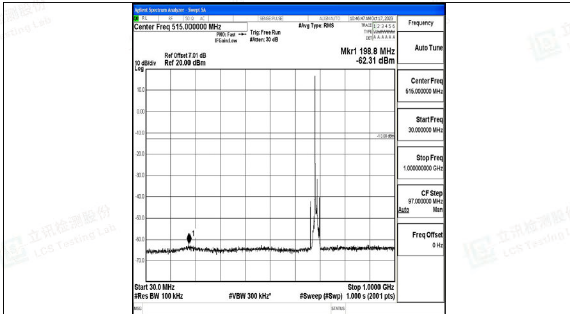
Band71_10MHz_QPSK_133422_1RB#0_30~1000_30~1000
