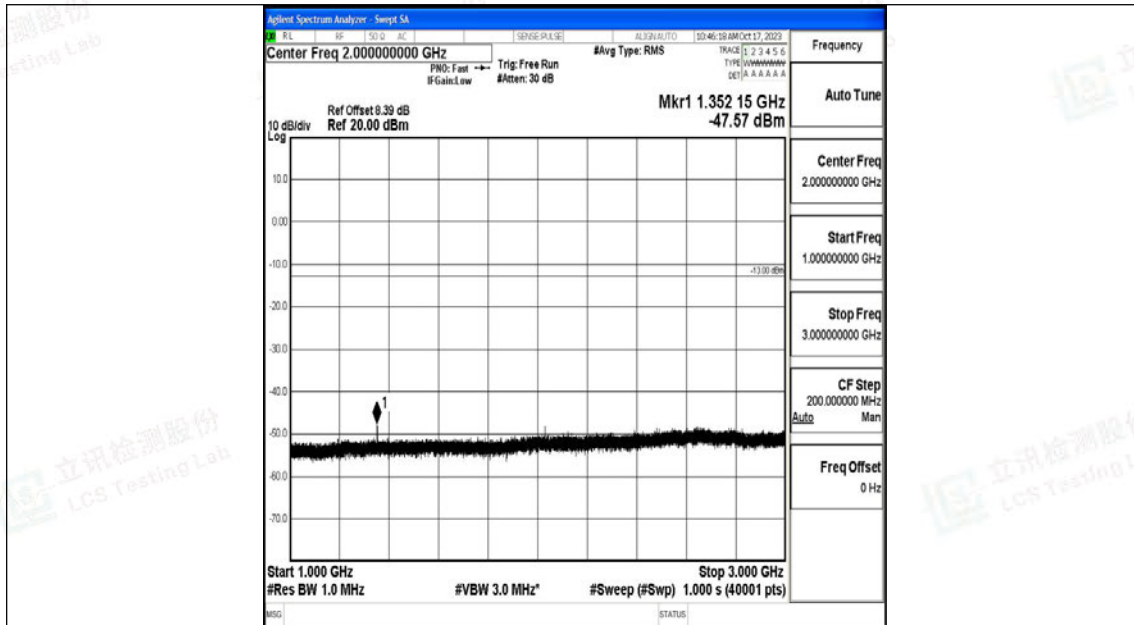
Band71_10MHz_16QAM_133297_1RB#0_1000~3000_1000~3000
