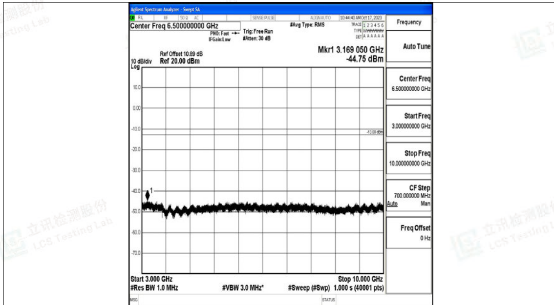
Band71_10MHz_QPSK_133172_1RB#0_3000~10000_3000~10000
