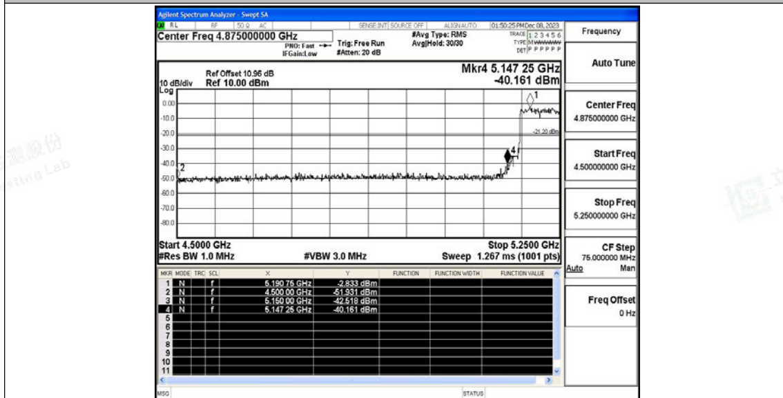
11AC80SISO_Ant1_High_5210_AV
