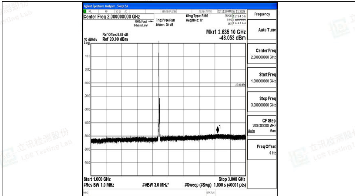
Band2_5MHz_16QAM_18900_1RB#0_1000~3000_1000~3000
