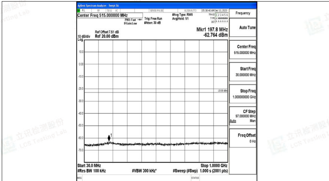
Band25_20MHz_QPSK_26140_1RB#0_30~1000_30~1000
