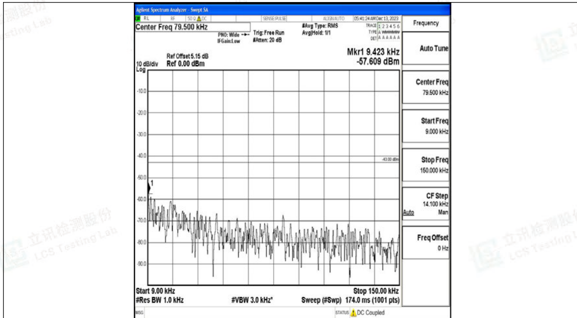
Band25_20MHz_QPSK_26590_1RB#0_0.009~0.15_0.009~0.15
