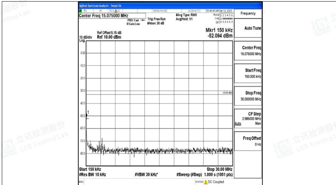
Band25_20MHz_16QAM_26365_1RB#0_0.15~30_0.15~30
