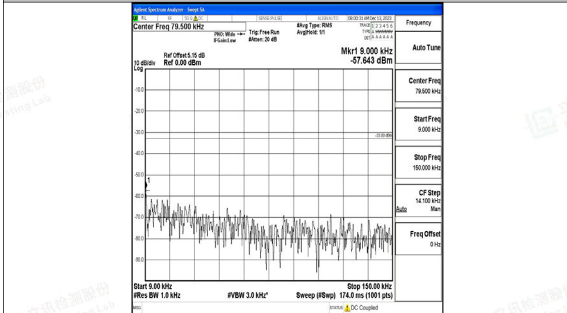
Band26_3MHz_16QAM_26740_1RB#0_0.009~0.15_0.009~0.15
