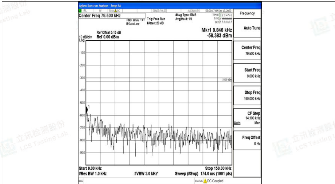
Band26_5MHz_QPSK_26740_1RB#0_0.009~0.15_0.009~0.15
