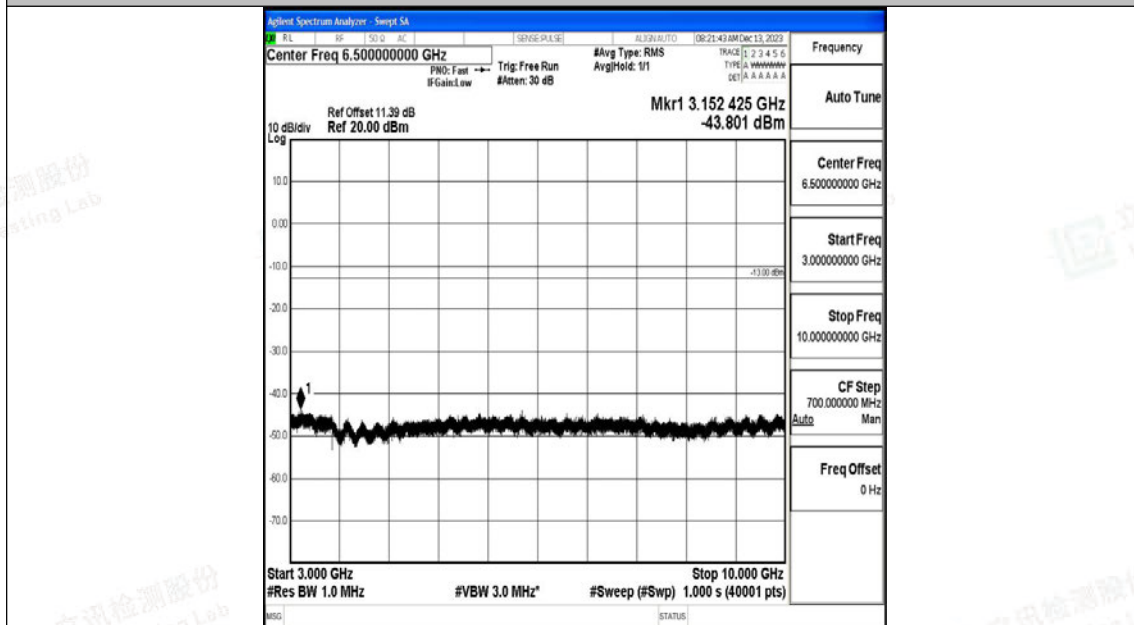
Band26_5MHz_16QAM_26740_1RB#0_3000~10000_3000~10000
