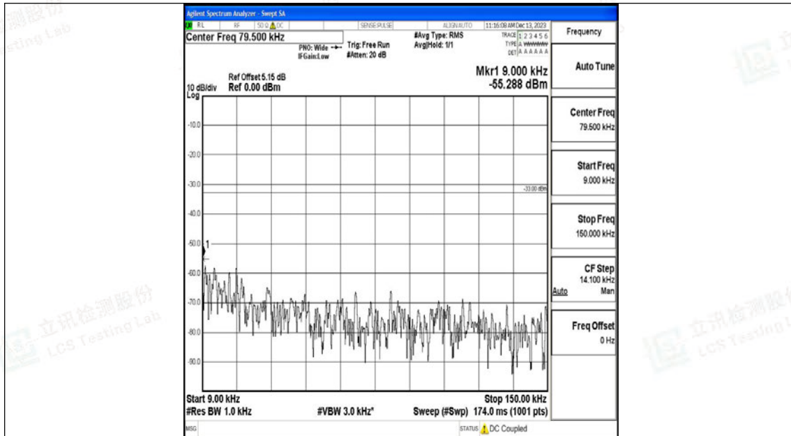
Band26_15MHz_QPSK_26915_1RB#0_0.009~0.15_0.009~0.15
