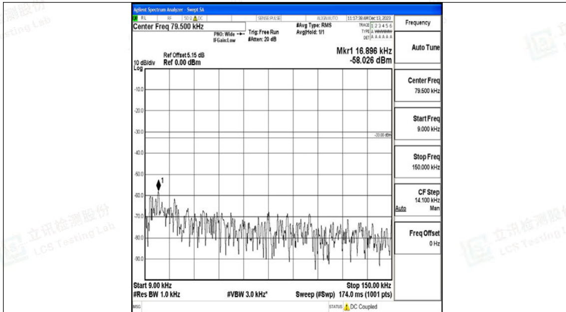
Band26_15MHz_QPSK_26965_1RB#0_0.009~0.15_0.009~0.15
