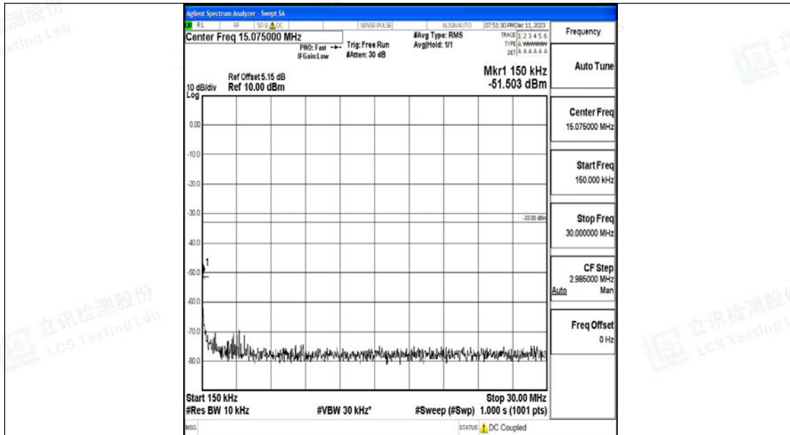
Band66_5MHz_16QAM_131997_1RB#0_0.15~30_0.15~30
