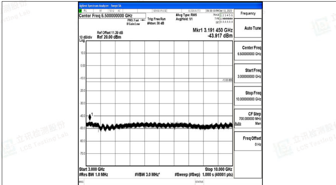
Band71_10MHz_QPSK_133422_1RB#0_3000~10000_3000~10000
