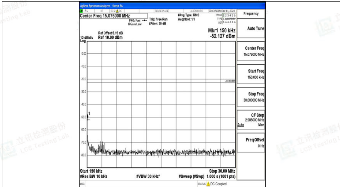
Band71_5MHz_16QAM_133447_1RB#0_0.15~30_0.15~30
