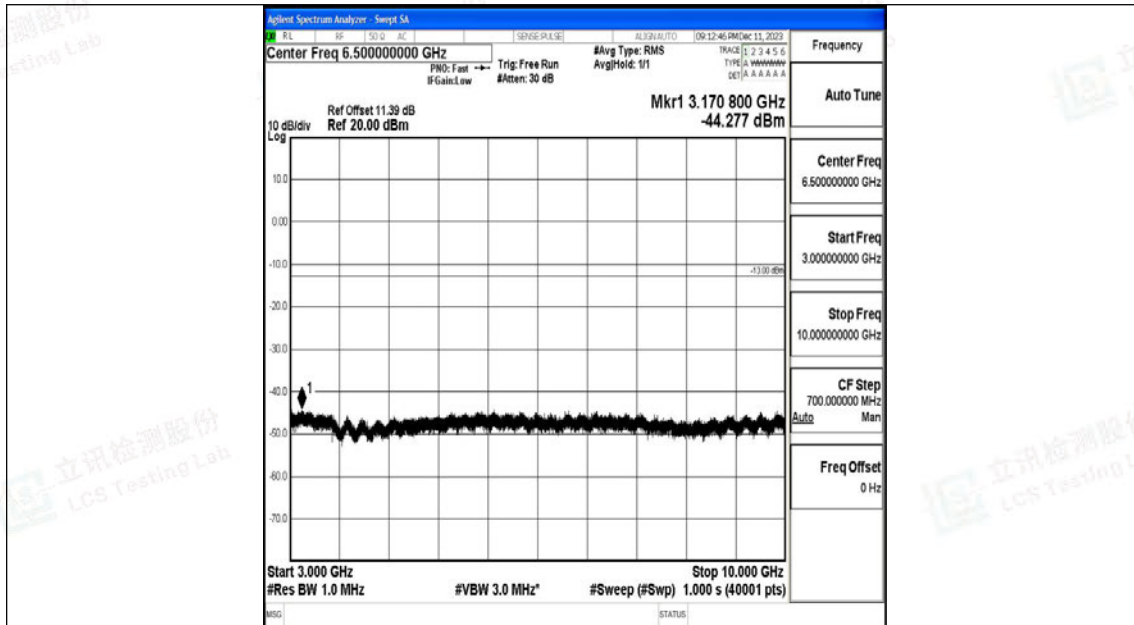
Band71_5MHz_QPSK_133447_1RB#0_3000~10000_3000~10000
