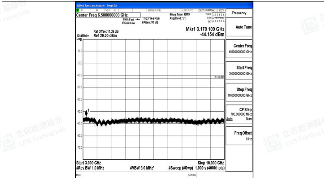
Band71_15MHz_QPSK_133197_1RB#0_3000~10000_3000~10000
