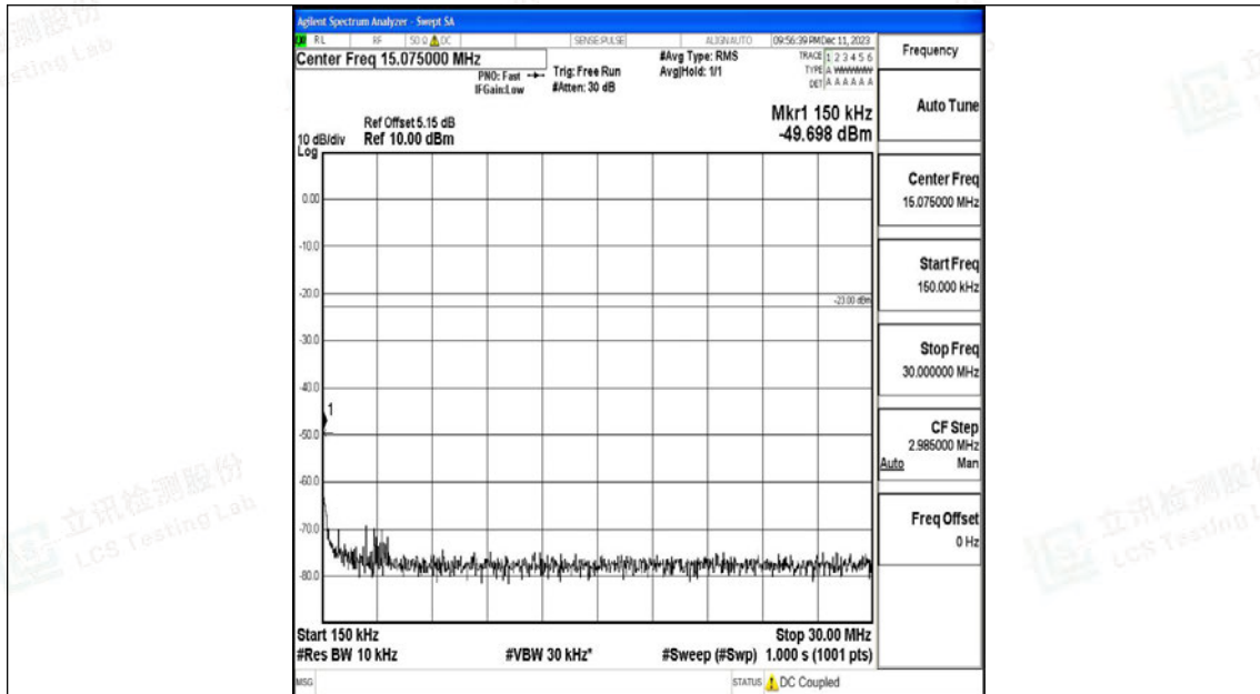
Band71_15MHz_16QAM_133197_1RB#0_0.15~30_0.15~30
