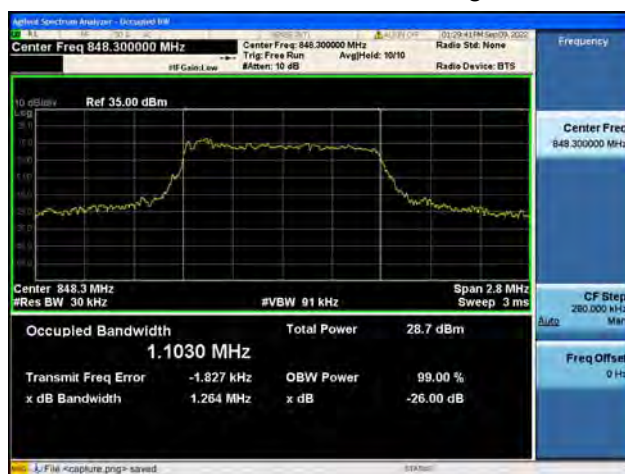
Band5 / 1.4MHz / 16QAM/ High CH
