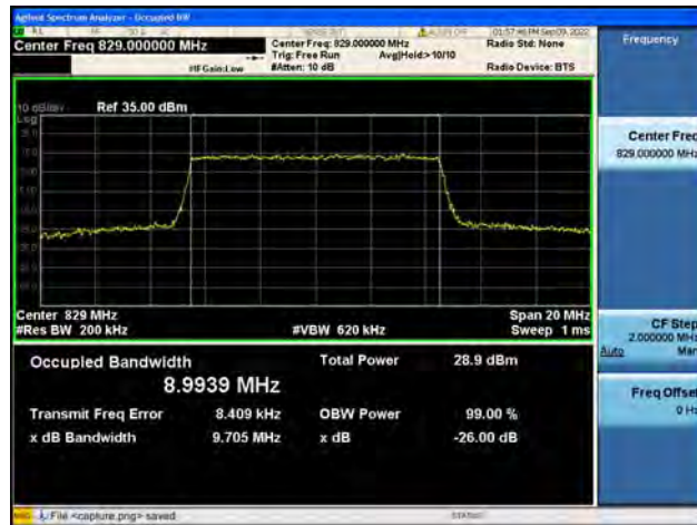
Band26Part22 / 10MHz / QPSK/ Mid CH
