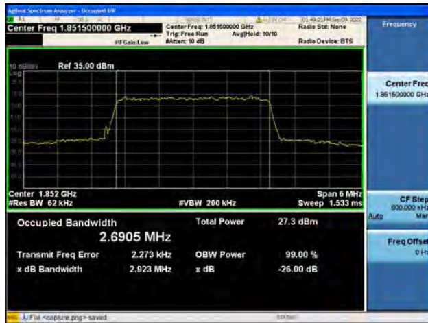
Band25 / 3MHz / QPSK/ Mid CH
