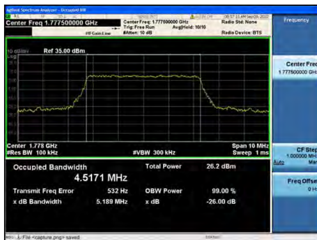
Band66 / 5MHz / 16QAM/ High CH
