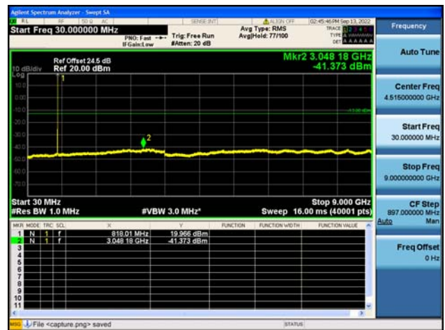
Band26Part90 / 3MHz / High CH / 16QAM
