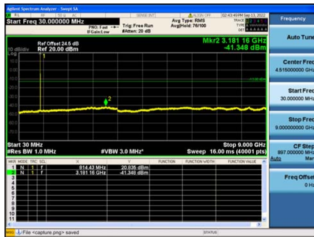
Band26Part90 / 1.4MHz / Mid CH / QPSK
