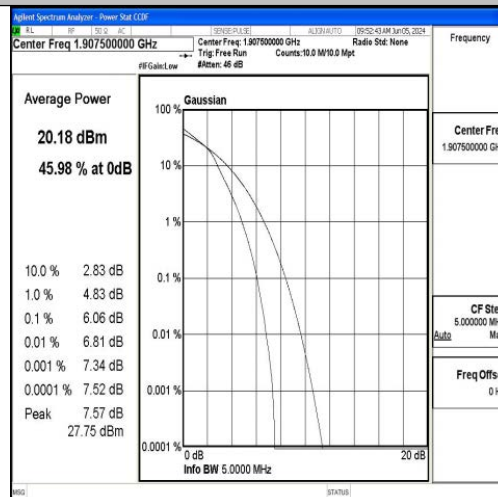
Band2-5MHz-16QAM-19175-25RB#0-PASS
