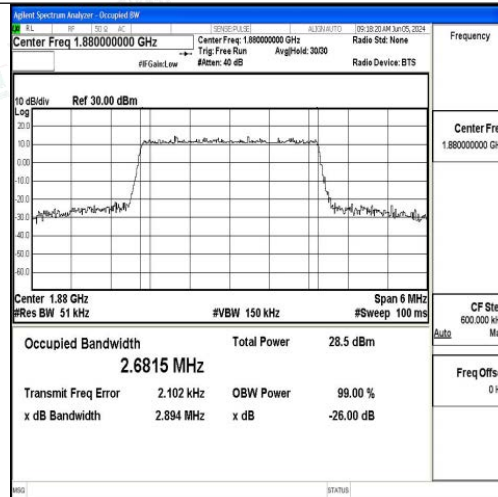
Band2-3MHz-16QAM-18900-15RB#0-PASS
