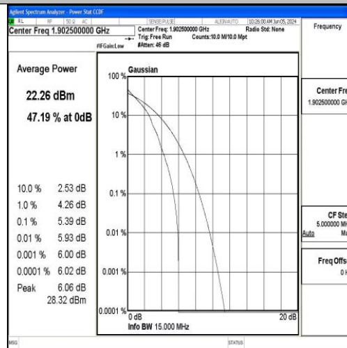
Band2-15MHz-QPSK-19125-1RB#0-PASS
