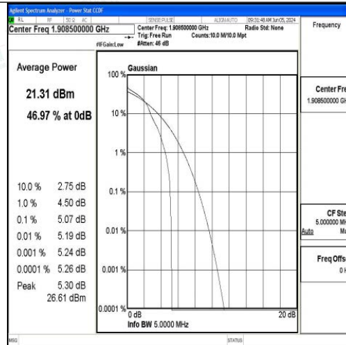
Band2-3MHz-16QAM-19185-1RB#0-PASS
