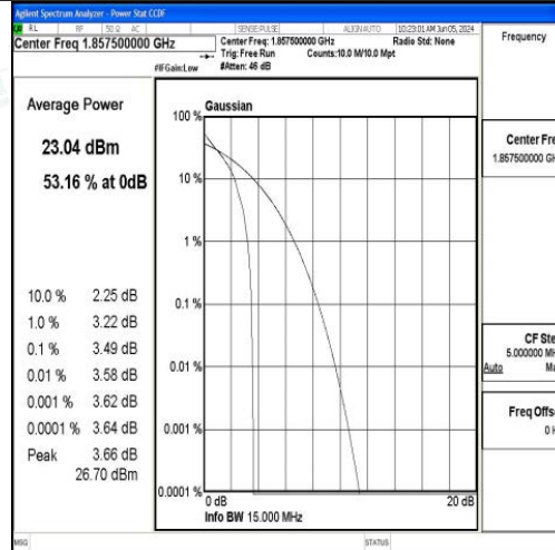
Band2-15MHz-QPSK-18675-1RB#0-PASS
