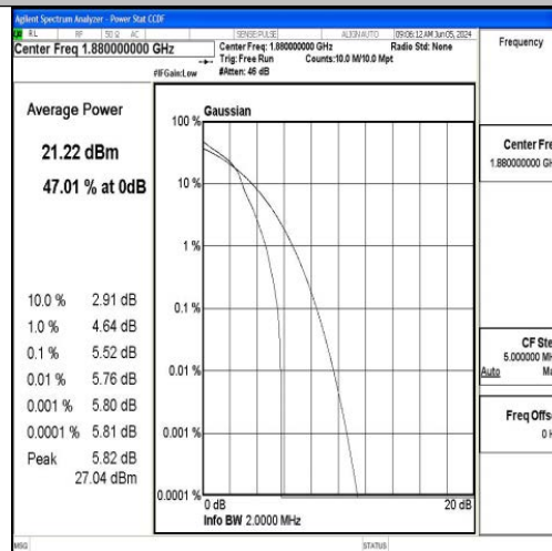
Band2-1.4MHz-16QAM-18900-1RB#0-PASS
