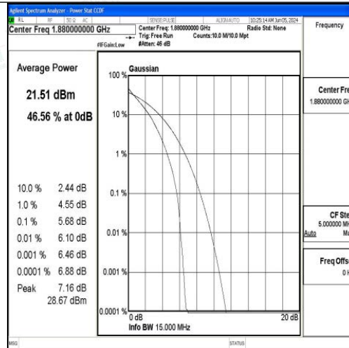
Band2-15MHz-QPSK-18900-75RB#0-PASS
