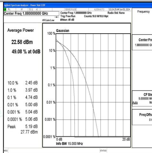
Band2-15MHz-QPSK-18900-1RB#0-PASS
