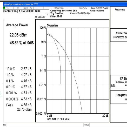
Band2-15MHz-16QAM-18675-1RB#0-PASS
