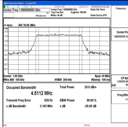
Band2-5MHz-16QAM-18900-25RB#0-PASS
