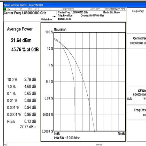
Band2-15MHz-16QAM-18900-1RB#0-PASS
