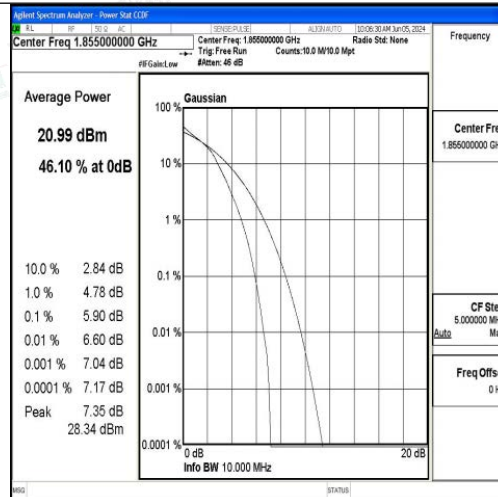
Band2-10MHz-16QAM-18650-50RB#0-PASS
