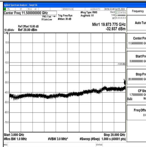
Band2_1.4MHz_QPSK_19193_1RB#0_3000~20000_3000~20000
