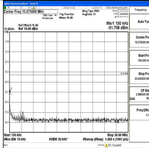
Band2_5MHz_16QAM_18900_1RB#0_0.15~30_0.15~30
