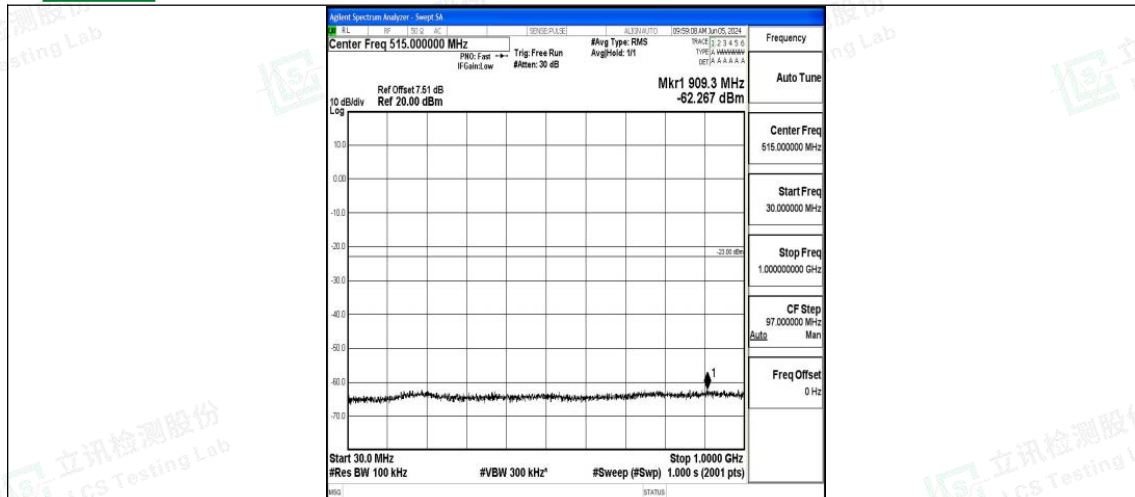
Band2_10MHz_16QAM_18650_1RB#0_30~1000_30~1000
