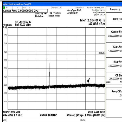
Band2_5MHz_QPSK_18625_1RB#0_1000~3000_1000~3000
