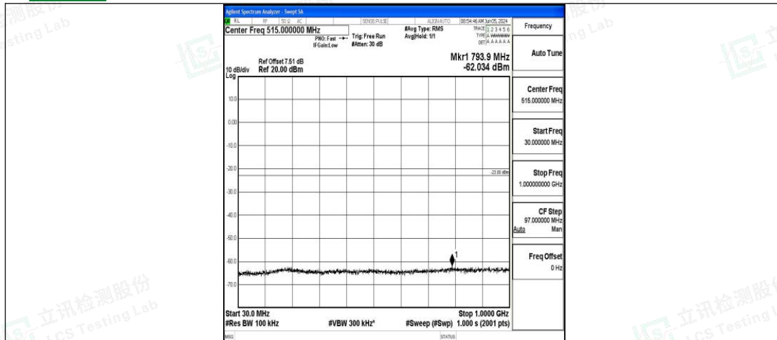
Band2_1.4MHz_16QAM_18607_1RB#0_30~1000_30~1000
