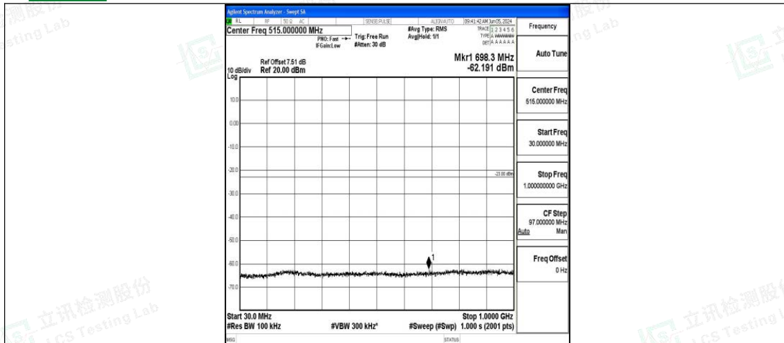
Band2_5MHz_QPSK_19175_1RB#0_30~1000_30~1000
