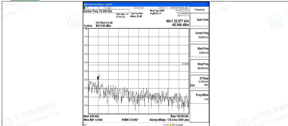
Band2_10MHz_QPSK_18900_1RB#0_0.009~0.15_0.009~0.15
