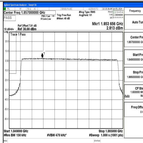
Band2_15MHz_16QAM_18675_75RB#0
