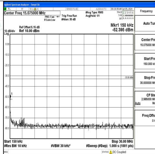
Band2_3MHz_QPSK_18615_1RB#0_0.15~30_0.15~30
