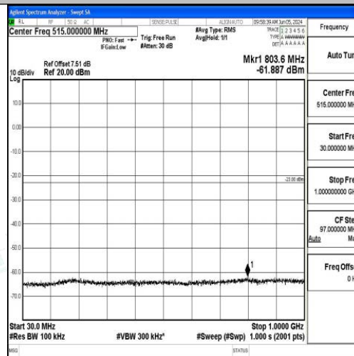
Band2_10MHz_QPSK_18650_1RB#0_30~1000_30~1000
