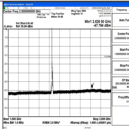
Band2_10MHz_QPSK_18650_1RB#0_1000~3000_1000~3000
