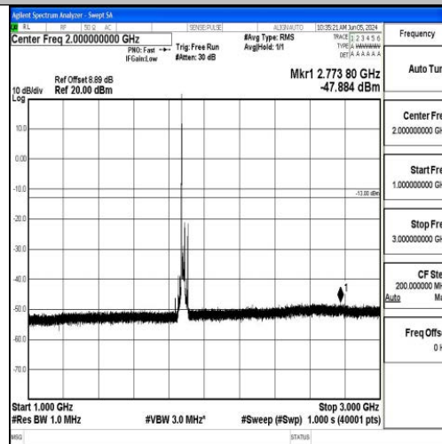
Band2_20MHz_16QAM_18900_1RB#0_1000~3000_1000~3000
