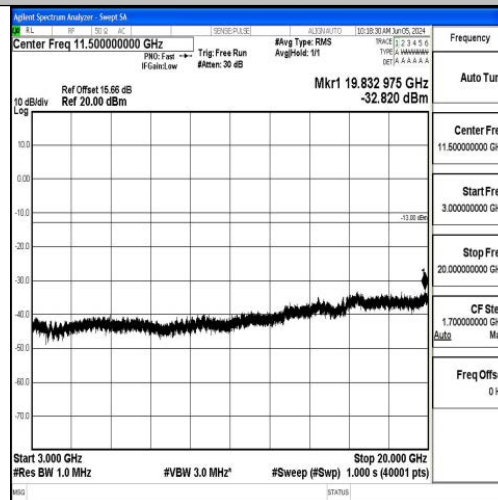
Band2_15MHz_QPSK_19125_1RB#0_3000~20000_3000~20000
