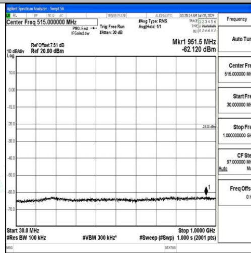
Band2_20MHz_16QAM_18900_1RB#0_30~1000_30~1000
