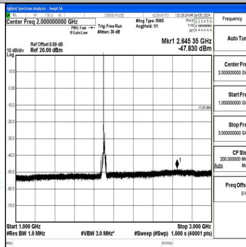
Band2_15MHz_QPSK_19125_1RB#0_1000~3000_1000~3000
