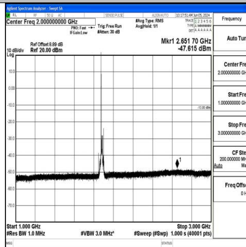
Band2_15MHz_16QAM_18900_1RB#0_1000~3000_1000~3000
