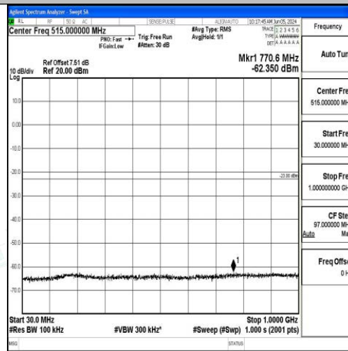
Band2_15MHz_16QAM_18900_1RB#0_30~1000_30~1000
