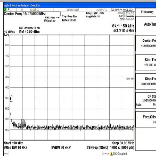
Band2_20MHz_QPSK_19100_1RB#0_0.15~30_0.15~30
