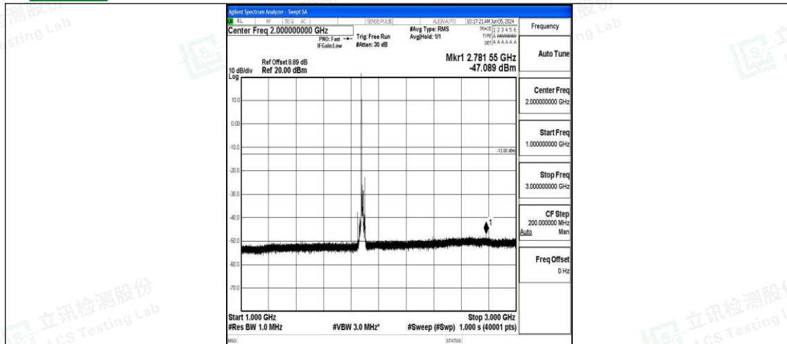
Band2_15MHz_QPSK_18900_1RB#0_1000~3000_1000~3000
