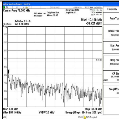
Band2_20MHz_QPSK_18700_1RB#0_0.009~0.15_0.009~0.15
