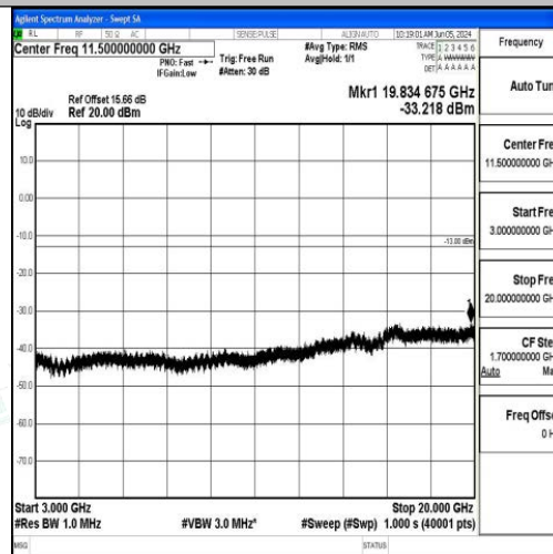
Band2_15MHz_16QAM_19125_1RB#0_3000~20000_3000~20000
