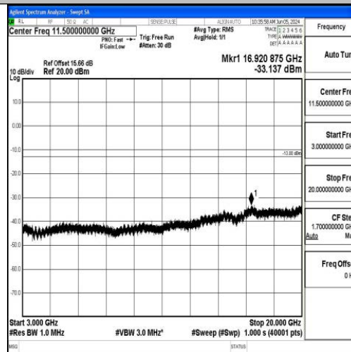
Band2_20MHz_QPSK_19100_1RB#0_3000~20000_3000~20000
