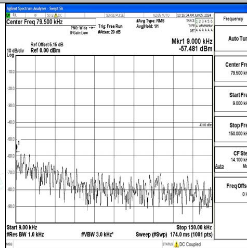
Band2_15MHz_16QAM_18675_1RB#0_0.009~0.15_0.009~0.15
