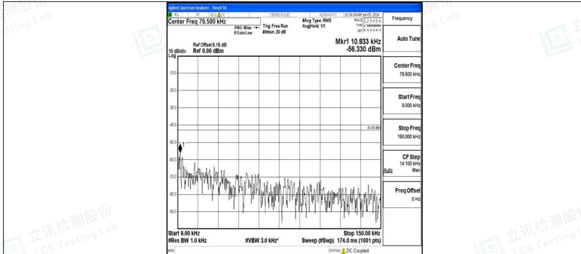
Band2_20MHz_QPSK_18900_1RB#0_0.009~0.15_0.009~0.15
