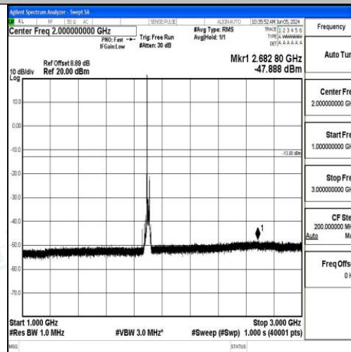
Band2_20MHz_QPSK_19100_1RB#0_1000~3000_1000~3000
