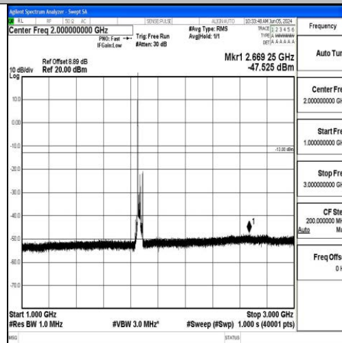
Band2_20MHz_QPSK_18700_1RB#0_1000~3000_1000~3000
