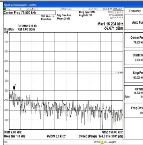
Band2_20MHz_QPSK_19100_1RB#0_0.009~0.15_0.009~0.15
