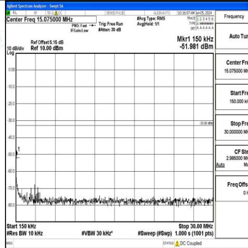
Band2_15MHz_QPSK_18675_1RB#0_0.15~30_0.15~30
