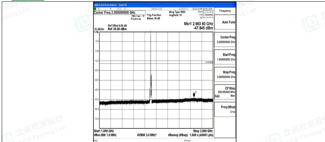
Band2_10MHz_16QAM_19150_1RB#0_1000~3000_1000~3000
