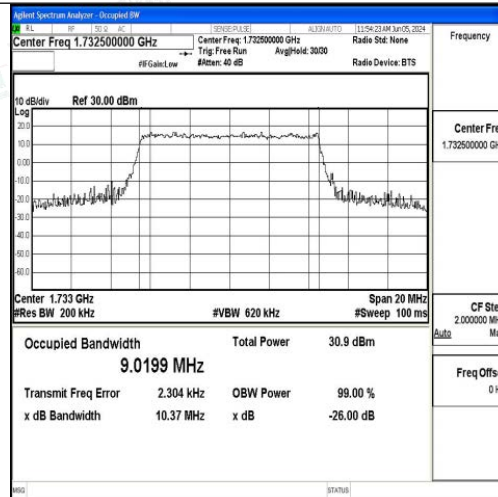
Band4-10MHz-16QAM-20175-50RB#0-PASS
