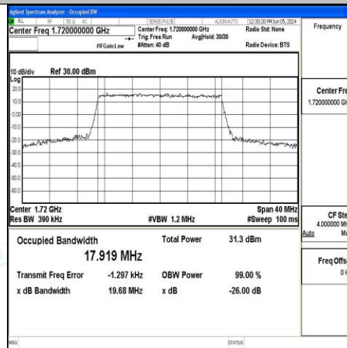
Band4-20MHz-16QAM-20050-100RB#0-PASS
