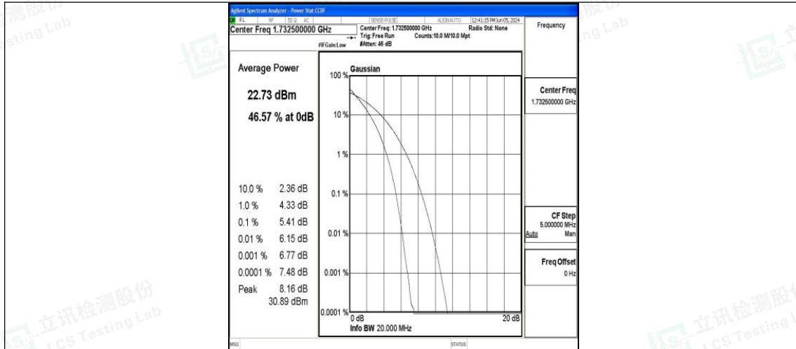
Band4-20MHz-QPSK-20175-100RB#0-PASS
