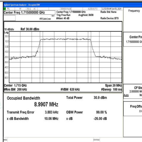
Band4-10MHz-16QAM-20000-50RB#0-PASS
