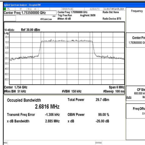
Band4-3MHz-16QAM-20385-15RB#0-PASS
