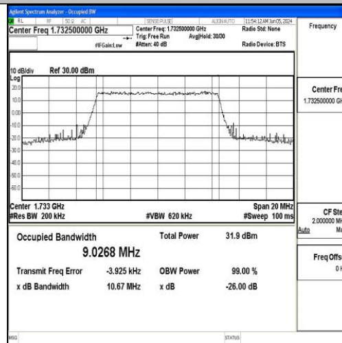
Band4-10MHz-QPSK-20175-50RB#0-PASS
