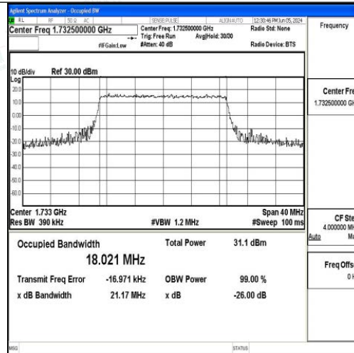
Band4-20MHz-16QAM-20175-100RB#0-PASS
