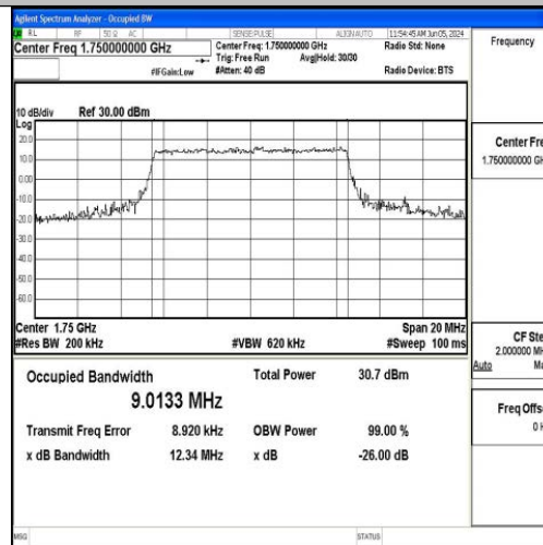
Band4-10MHz-16QAM-20350-50RB#0-PASS
