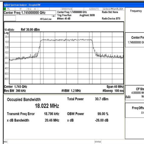
Band4-20MHz-16QAM-20300-100RB#0-PASS
