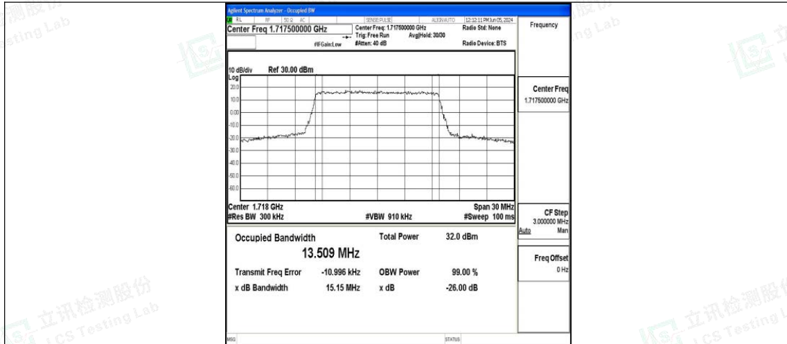
Band4-15MHz-QPSK-20025-75RB#0-PASS
