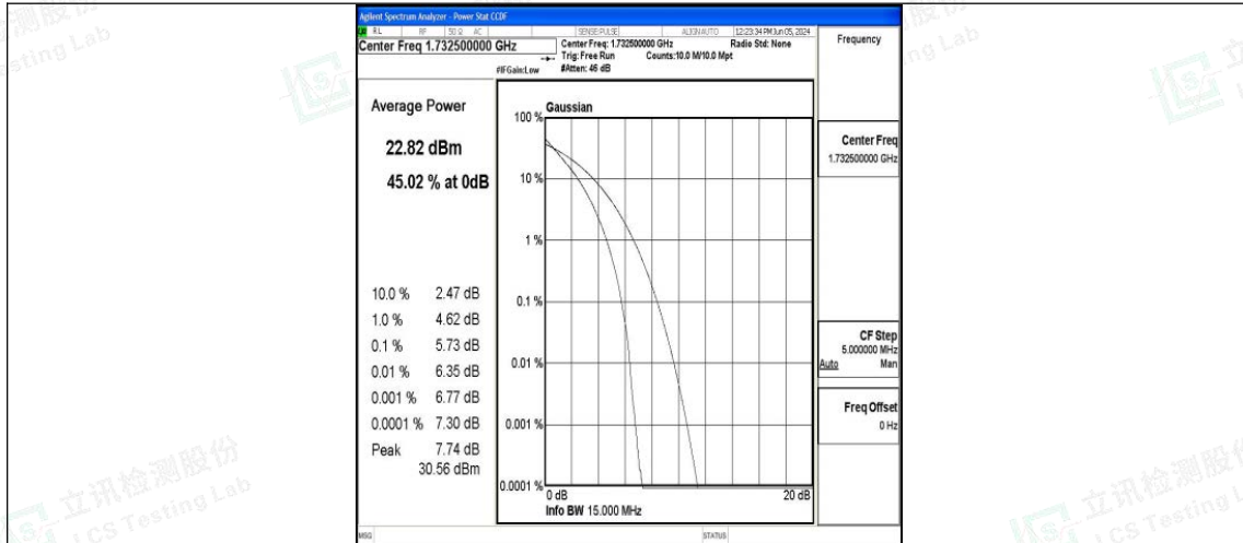
Band4-15MHz-QPSK-20175-75RB#0-PASS
