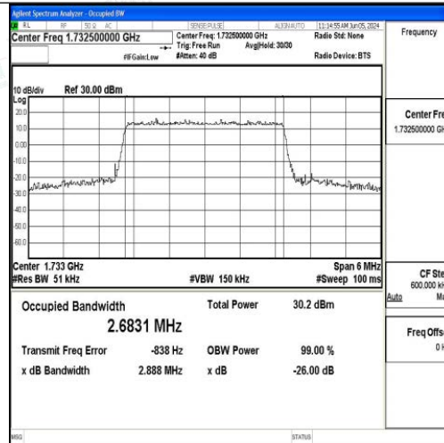
Band4-3MHz-16QAM-20175-15RB#0-PASS
