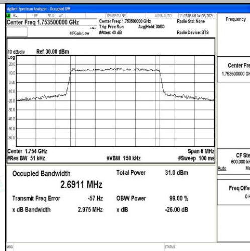
Band4-3MHz-QPSK-20385-15RB#0-PASS
