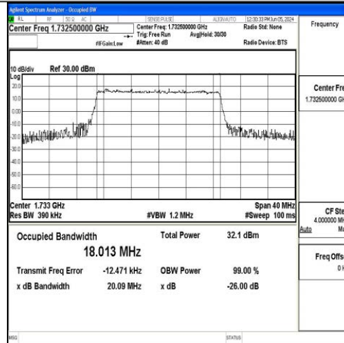
Band4-20MHz-QPSK-20175-100RB#0-PASS
