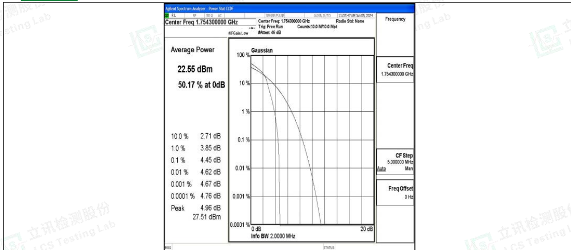
Band4-1.4MHz-16QAM-20393-1RB#0-PASS
