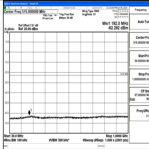
Band4_15MHz_QPSK_20325_1RB#0_30~1000_30~1000
