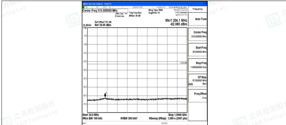
Band4_15MHz_16QAM_20025_1RB#0_30~1000_30~1000
