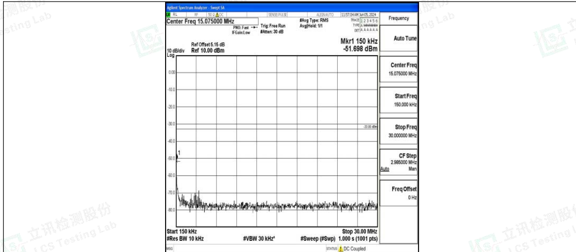
Band4_10MHz_16QAM_20175_1RB#0_0.15~30_0.15~30
