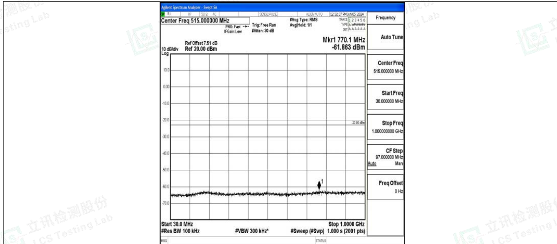
Band4_20MHz_16QAM_20050_1RB#0_30~1000_30~1000
