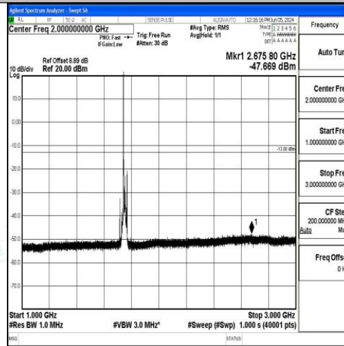
Band4_15MHz_QPSK_20325_1RB#0_1000~3000_1000~3000
