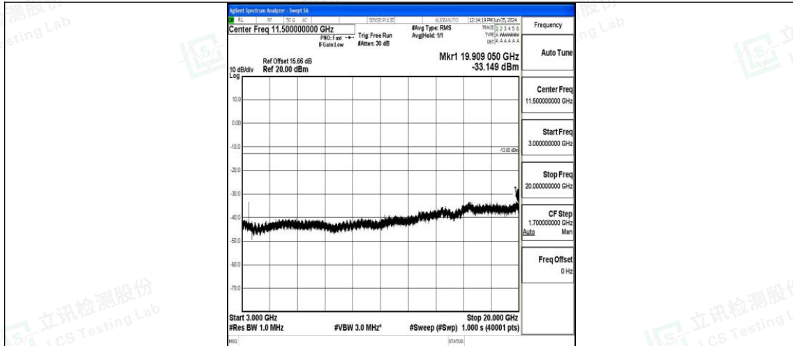
Band4_15MHz_QPSK_20025_1RB#0_3000~20000_3000~20000
