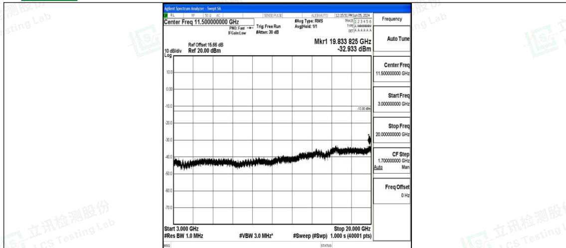
Band4_15MHz_16QAM_20175_1RB#0_3000~20000_3000~20000
