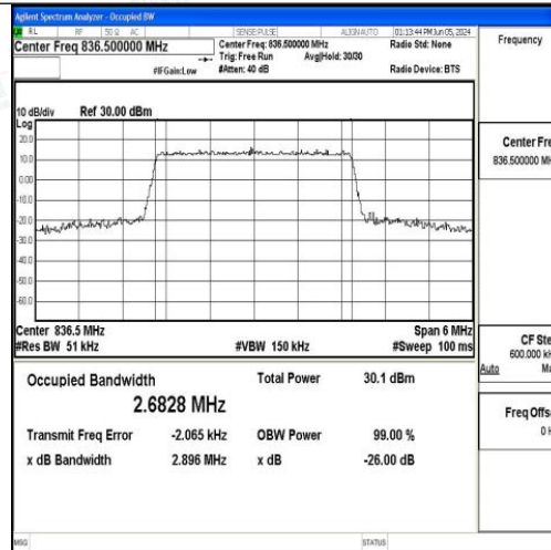
Band5-3MHz-16QAM-20525-15RB#0-PASS
