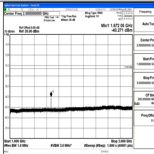
Band5_1.4MHz_QPSK_20525_1RB#0_1000~3000_1000~3000
