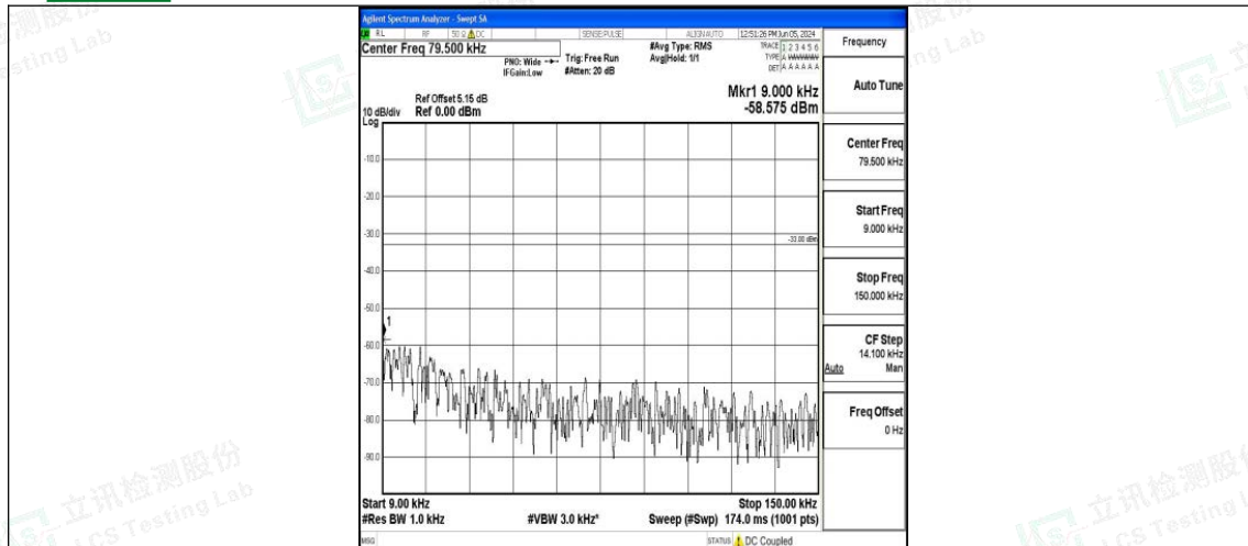
Band5_1.4MHz_QPSK_20643_1RB#0_0.009~0.15_0.009~0.15
