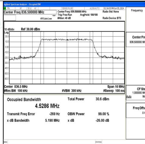
Band5-5MHz-16QAM-20525-25RB#0-PASS
