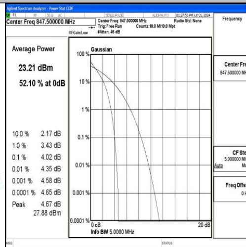
Band5-3MHz-QPSK-20635-15RB#0-PASS
