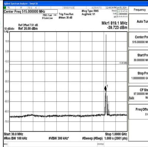
Band5_1.4MHz_QPSK_20407_1RB#0_30~1000_30~1000
