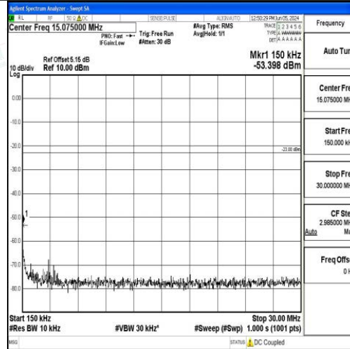
Band5_1.4MHz_QPSK_20525_1RB#0_0.15~30_0.15~30
