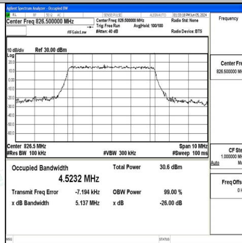
Band5-5MHz-16QAM-20425-25RB#0-PASS
