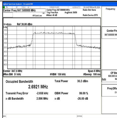
Band5-3MHz-16QAM-20635-15RB#0-PASS
