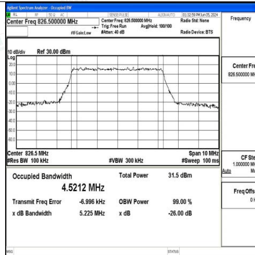
Band5-5MHz-QPSK-20425-25RB#0-PASS
