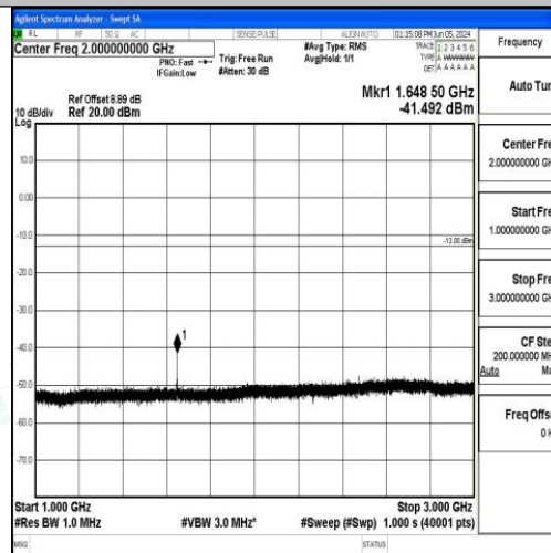
Band5_3MHz_QPSK_20415_1RB#0_1000~3000_1000~3000
