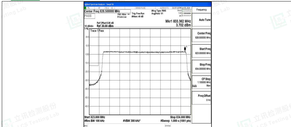
Band5_10MHz_16QAM_20450_50RB#0
