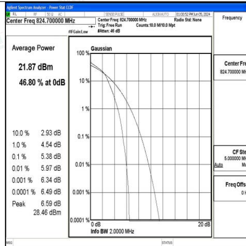
Band5-1.4MHz-16QAM-20407-6RB#0-PASS
