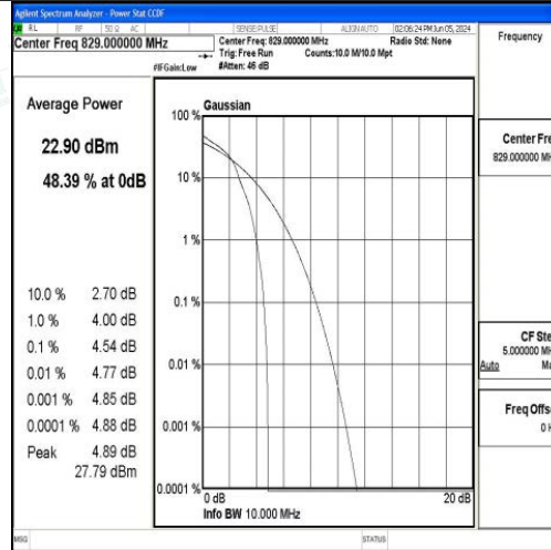
Band5-10MHz-16QAM-20450-1RB#0-PASS
