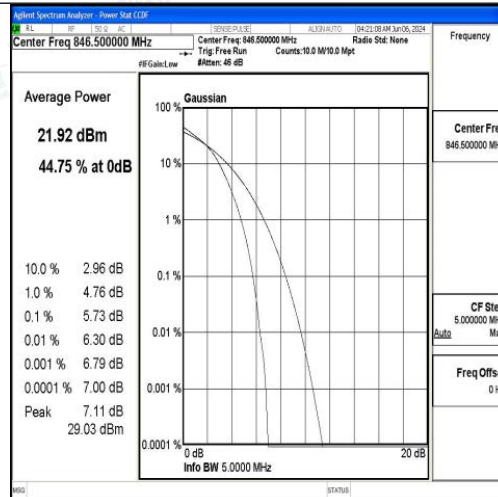
Band5-5MHz-16QAM-20625-25RB#0-PASS
