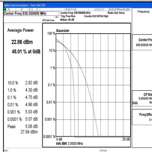
Band5-1.4MHz-16QAM-20525-1RB#0-PASS
