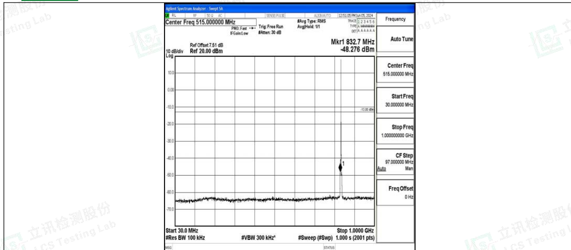
Band5_1.4MHz_16QAM_20525_1RB#0_30~1000_30~1000
