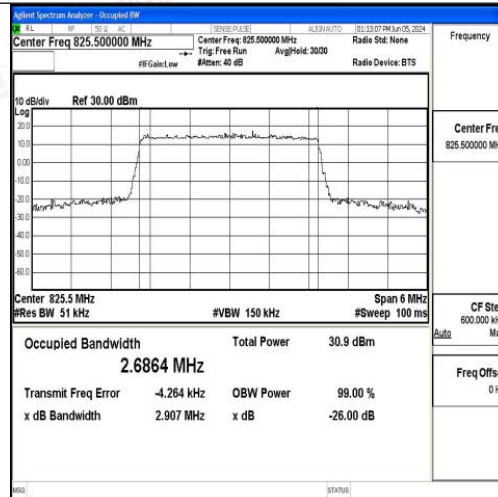
Band5-3MHz-QPSK-20415-15RB#0-PASS
