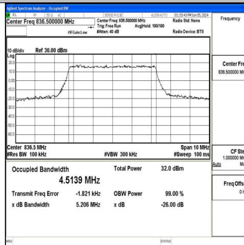
Band5-5MHz-QPSK-20525-25RB#0-PASS
