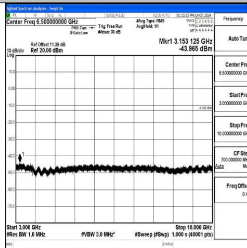
Band5_3MHz_QPSK_20415_1RB#0_3000~10000_3000~10000
