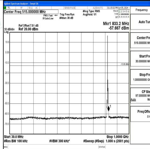
Band5_3MHz_QPSK_20415_1RB#0_30~1000_30~1000
