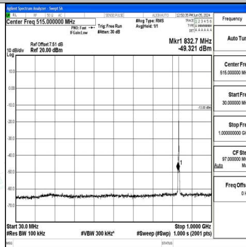
Band5_1.4MHz_QPSK_20525_1RB#0_30~1000_30~1000
