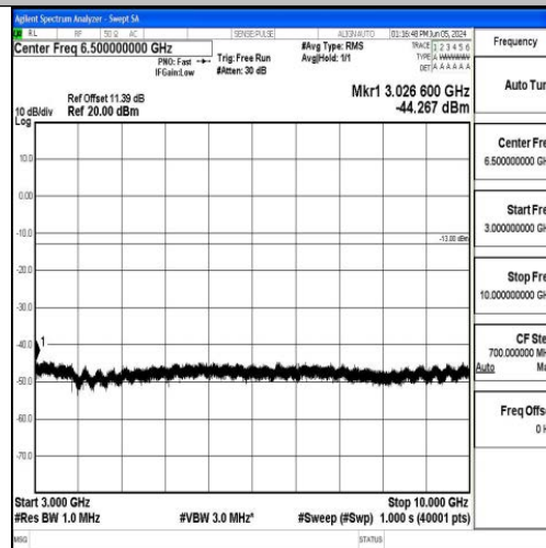
Band5_3MHz_16QAM_20525_1RB#0_3000~10000_3000~10000
