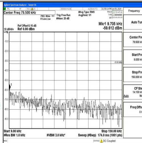
Band5_10MHz_16QAM_20525_1RB#0_0.009~0.15_0.009~0.15
