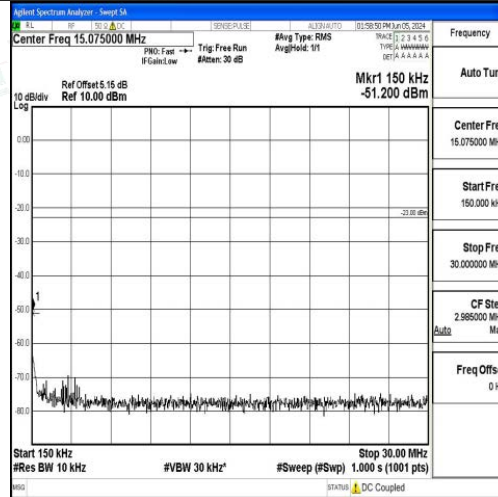
Band5_10MHz_QPSK_20525_1RB#0_0.15~30_0.15~30
