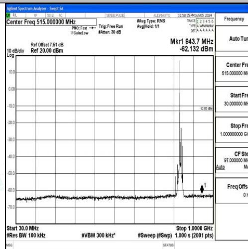
Band5_10MHz_QPSK_20525_1RB#0_30~1000_30~1000
