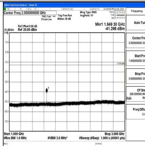
Band5_10MHz_QPSK_20450_1RB#0_1000~3000_1000~3000
