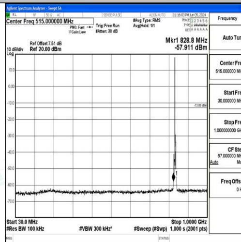
Band5_3MHz_QPSK_20525_1RB#0_30~1000_30~1000
