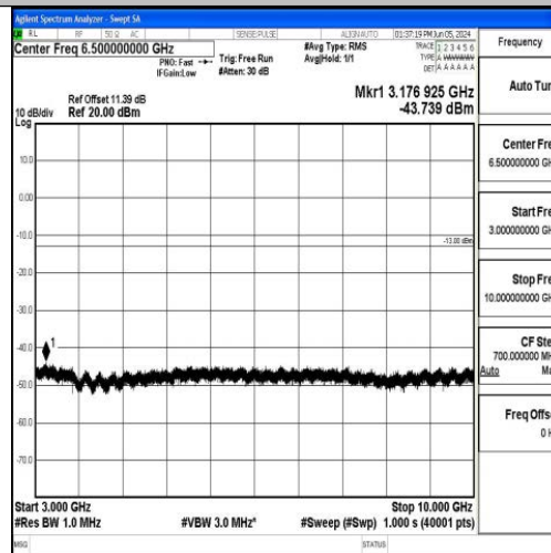
Band5_5MHz_16QAM_20525_1RB#0_3000~10000_3000~10000
