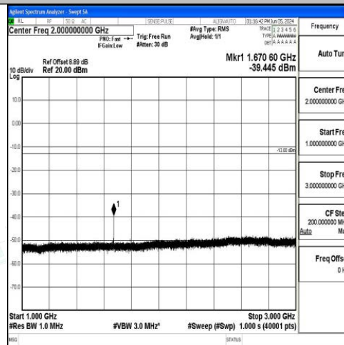
Band5_3MHz_16QAM_20525_1RB#0_1000~3000_1000~3000
