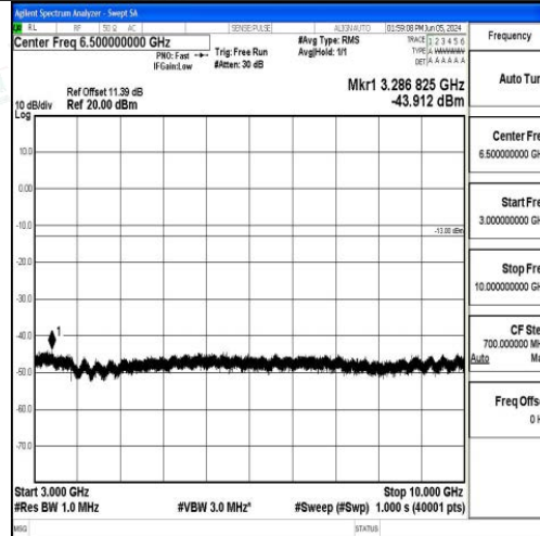
Band5_10MHz_QPSK_20525_1RB#0_3000~10000_3000~10000
