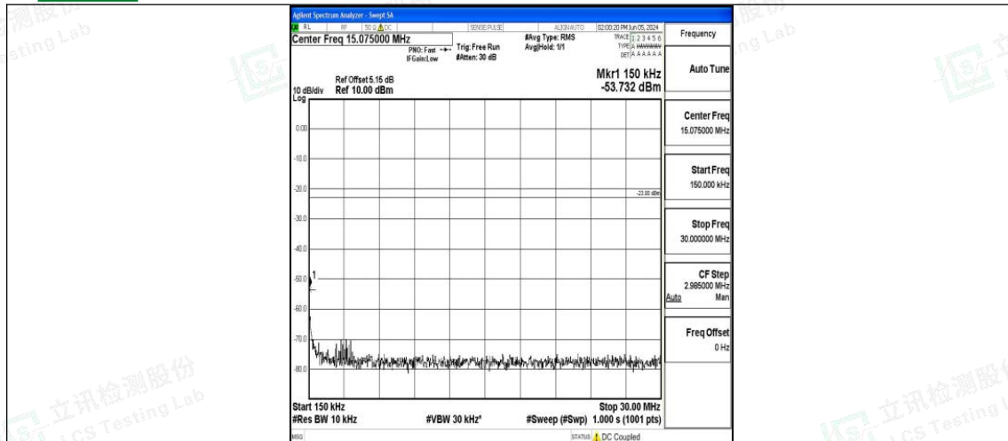
Band5_10MHz_16QAM_20600_1RB#0_0.15~30_0.15~30
