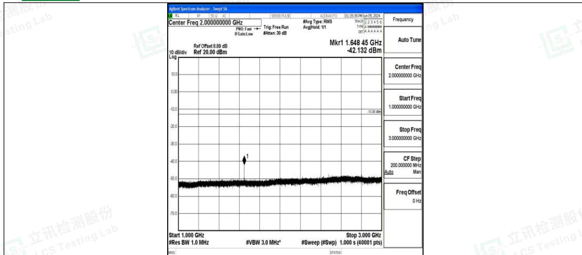
Band5_3MHz_16QAM_20415_1RB#0_1000~3000_1000~3000
