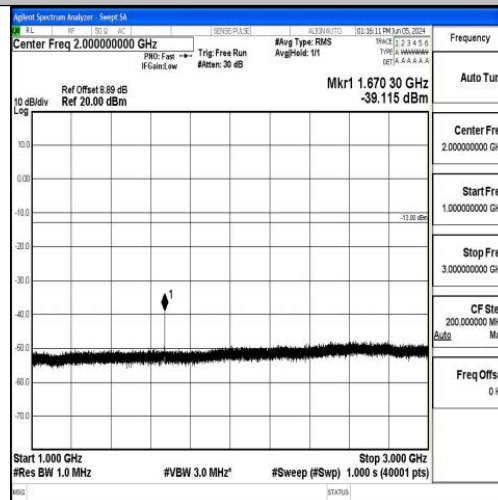
Band5_3MHz_QPSK_20525_1RB#0_1000~3000_1000~3000
