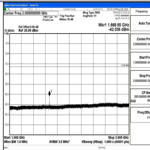
Band5_5MHz_16QAM_20525_1RB#0_1000~3000_1000~3000
