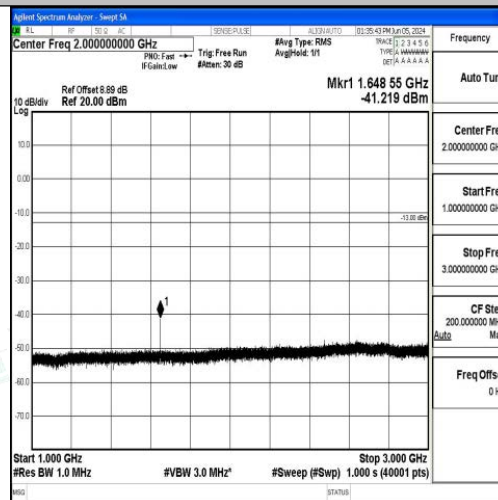
Band5_5MHz_QPSK_20425_1RB#0_1000~3000_1000~3000
