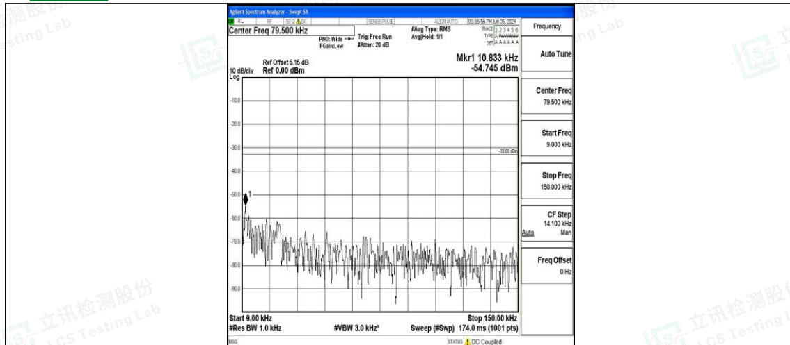
Band5_3MHz_QPSK_20635_1RB#0_0.009~0.15_0.009~0.15
