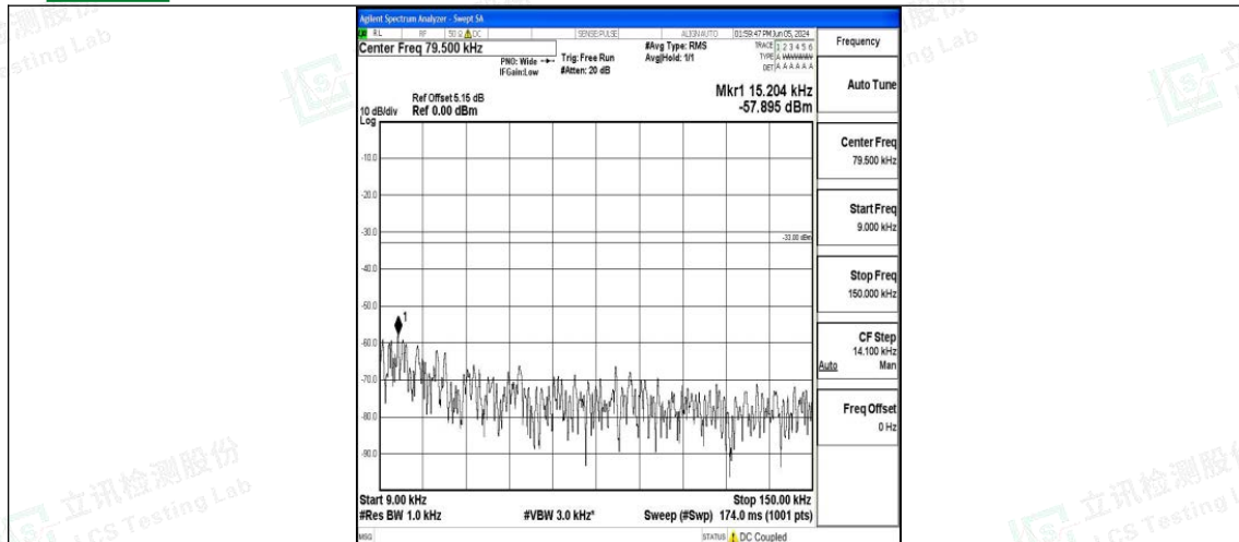
Band5_10MHz_QPSK_20600_1RB#0_0.009~0.15_0.009~0.15
