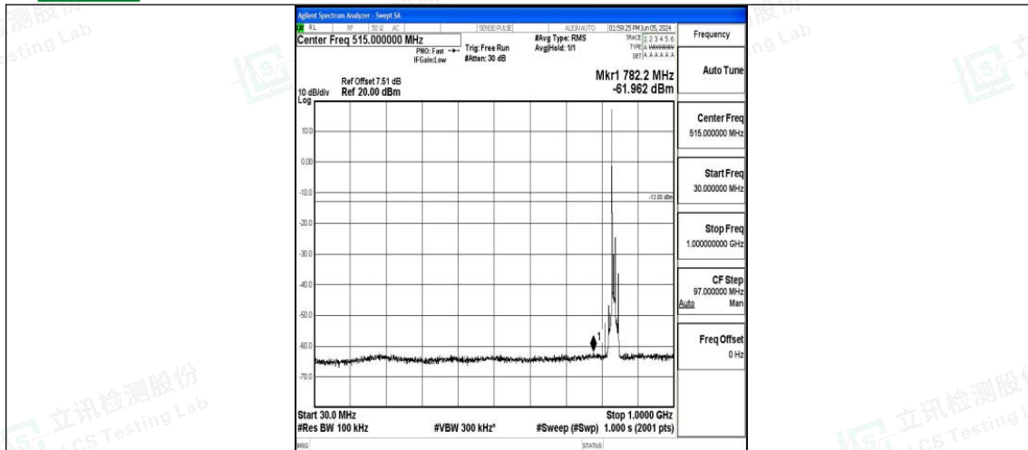
Band5_10MHz_16QAM_20525_1RB#0_30~1000_30~1000
