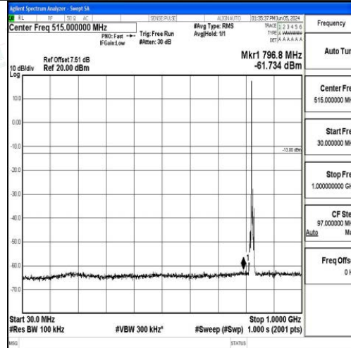
Band5_5MHz_QPSK_20425_1RB#0_30~1000_30~1000
