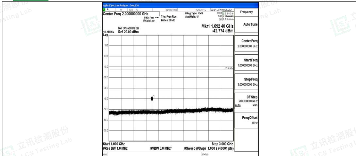
Band5_3MHz_QPSK_20635_1RB#0_1000~3000_1000~3000
