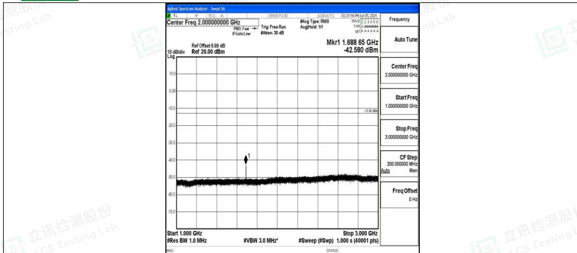
Band5_5MHz_QPSK_20625_1RB#0_1000~3000_1000~3000
