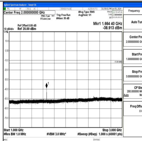
Band5_10MHz_QPSK_20525_1RB#0_1000~3000_1000~3000
