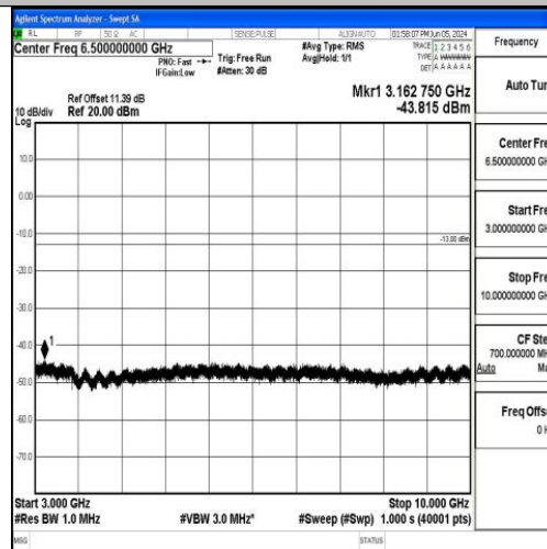
Band5_10MHz_QPSK_20450_1RB#0_3000~10000_3000~10000
