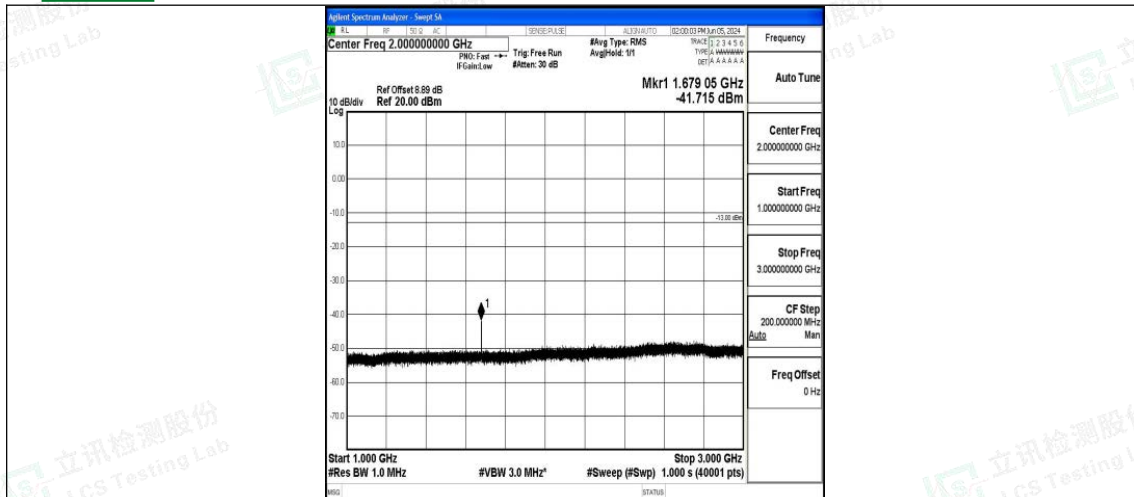
Band5_10MHz_QPSK_20600_1RB#0_1000~3000_1000~3000
