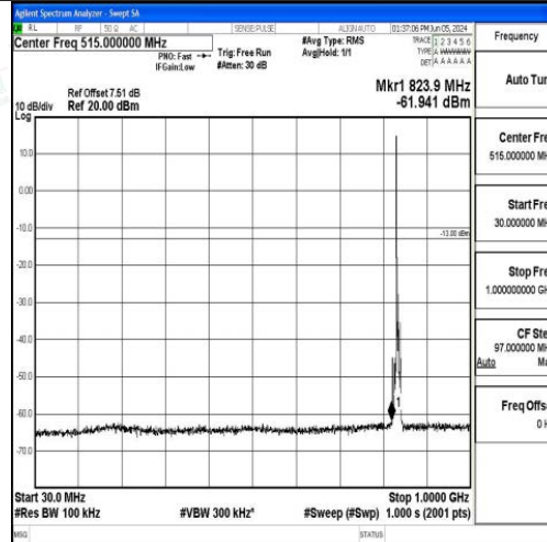
Band5_5MHz_16QAM_20525_1RB#0_30~1000_30~1000
