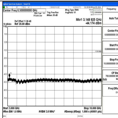
Band5_5MHz_QPSK_20425_1RB#0_3000~10000_3000~10000
