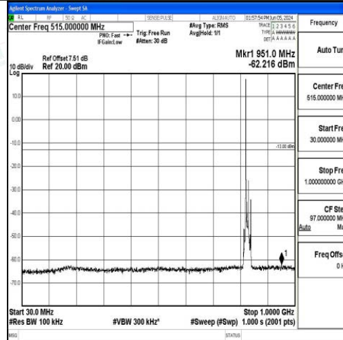
Band5_10MHz_QPSK_20450_1RB#0_30~1000_30~1000
