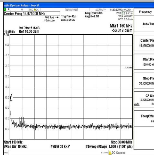
Band5_10MHz_16QAM_20525_1RB#0_0.15~30_0.15~30
