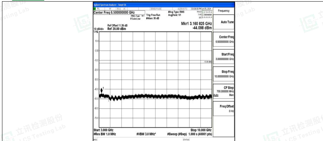
Band12_5MHz_QPSK_23095_1RB#0_3000~10000_3000~10000
