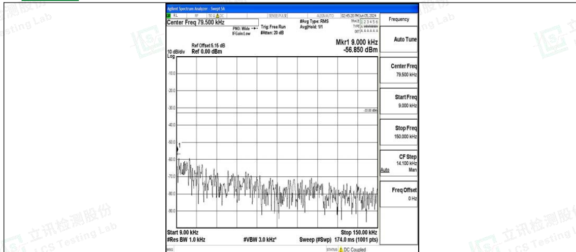
Band12_3MHz_16QAM_23025_1RB#0_0.009~0.15_0.009~0.15
