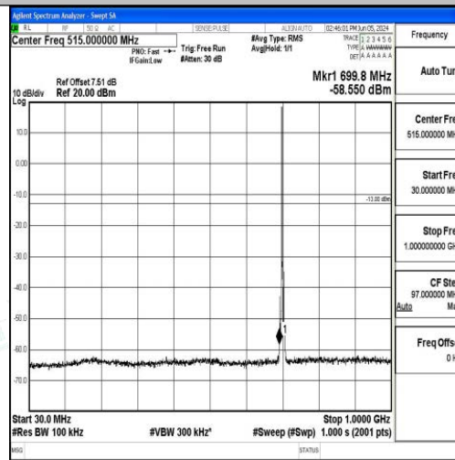
Band12_3MHz_QPSK_23095_1RB#0_30~1000_30~1000
