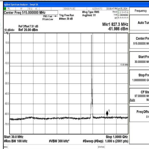
Band12_5MHz_QPSK_23035_1RB#0_30~1000_30~1000
