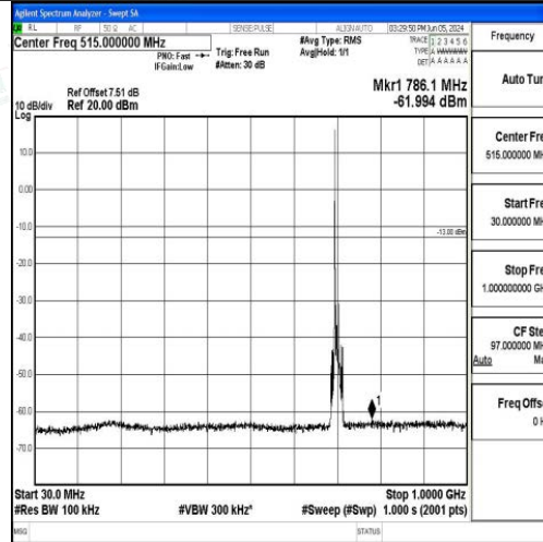
Band12_10MHz_16QAM_23095_1RB#0_30~1000_30~1000
