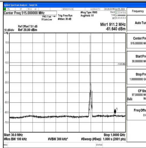
Band12_10MHz_QPSK_23095_1RB#0_30~1000_30~1000
