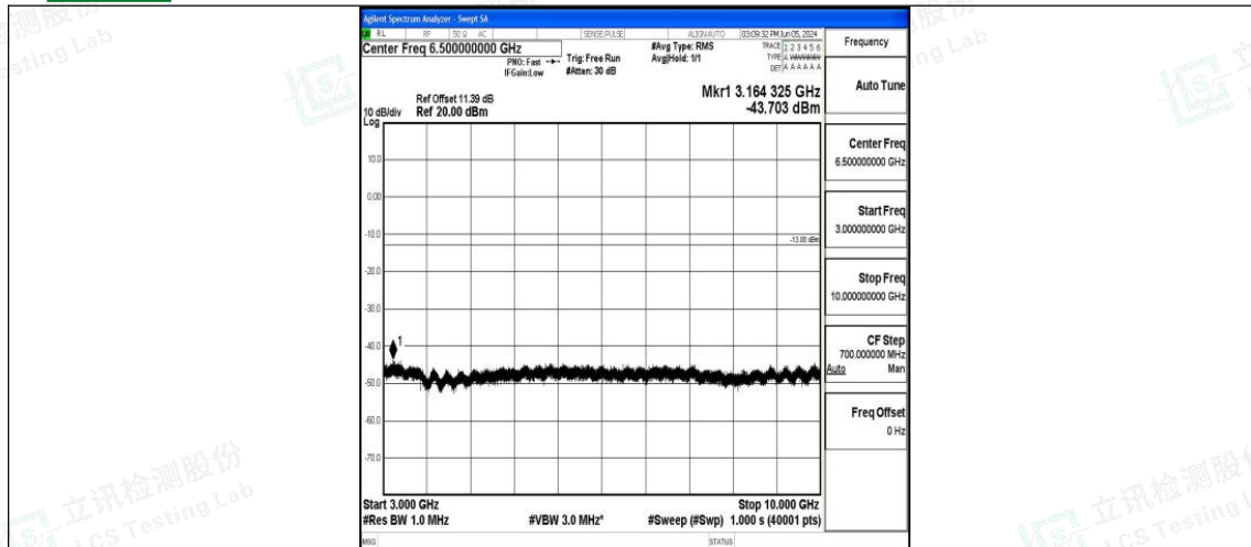
Band12_5MHz_16QAM_23155_1RB#0_3000~10000_3000~10000
