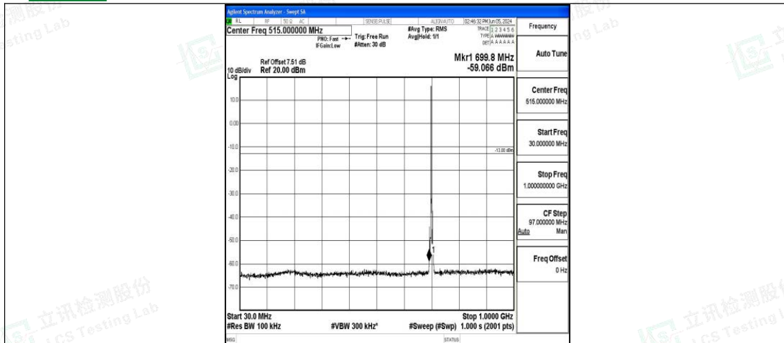
Band12_3MHz_16QAM_23095_1RB#0_30~1000_30~1000
