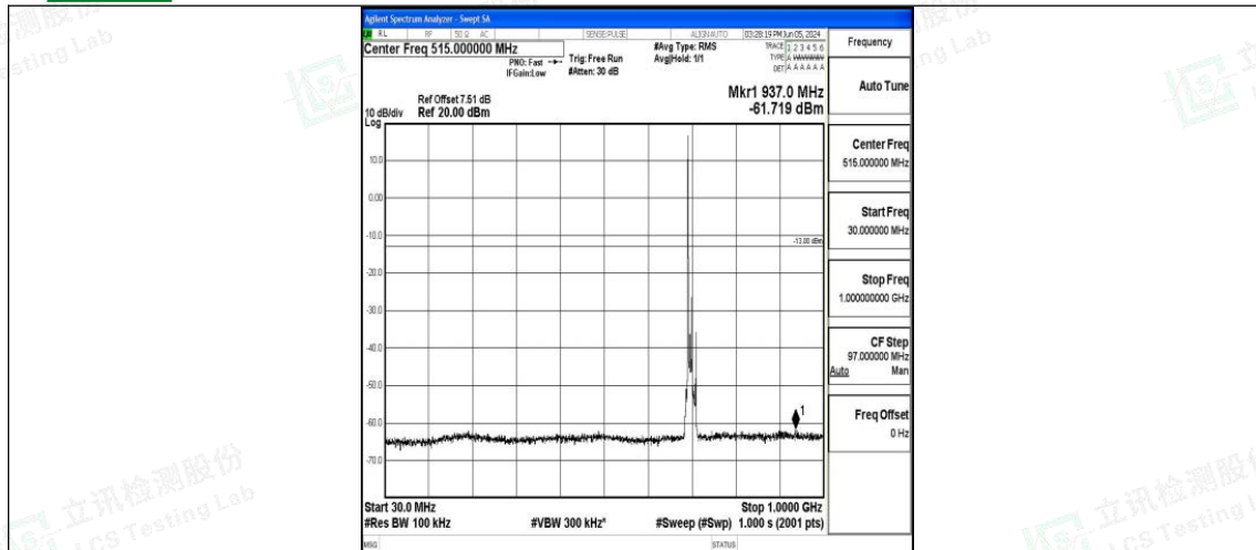
Band12_10MHz_QPSK_23060_1RB#0_30~1000_30~1000
