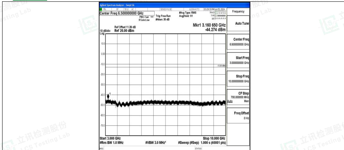
Band12_10MHz_QPSK_23095_1RB#0_3000~10000_3000~10000
