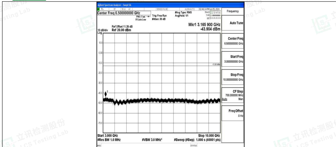
Band12_3MHz_QPSK_23095_1RB#0_3000~10000_3000~10000
