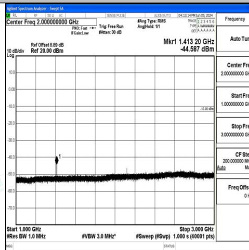
Band17_10MHz_QPSK_23800_1RB#0_1000~3000_1000~3000
