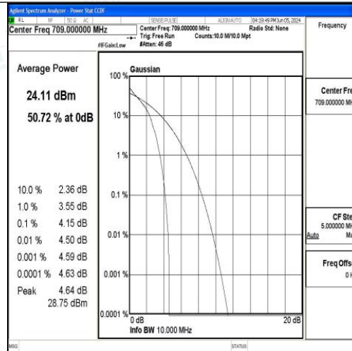
Band17-10MHz-QPSK-23780-1RB#0-PASS
