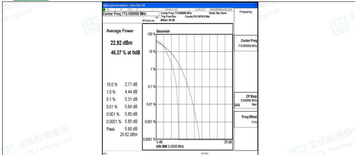
Band17-5MHz-16QAM-23825-1RB#0-PASS
