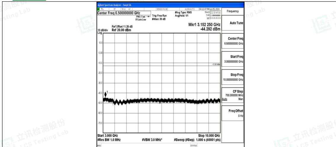
Band17_10MHz_16QAM_23790_1RB#0_3000~10000_3000~10000
