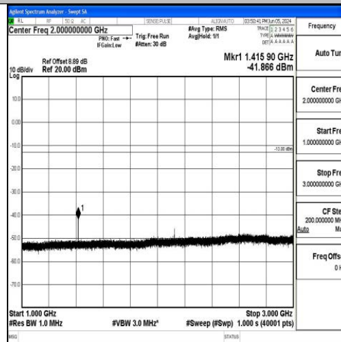
Band17_5MHz_16QAM_23790_1RB#0_1000~3000_1000~3000
