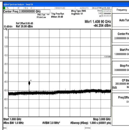
Band17_10MHz_16QAM_23780_1RB#0_1000~3000_1000~3000
