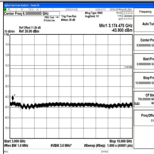
Band17_5MHz_QPSK_23825_1RB#0_3000~10000_3000~10000
