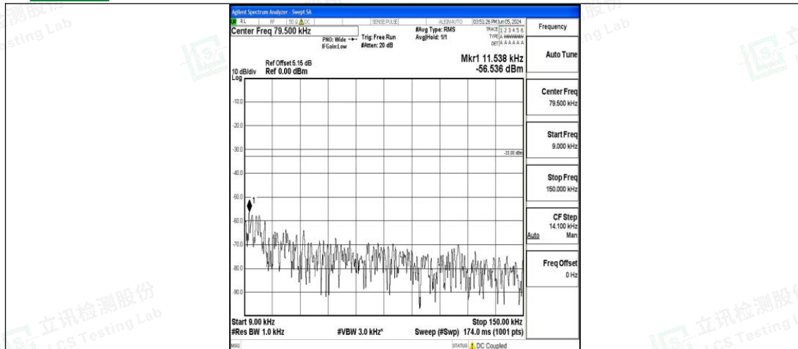
Band17_5MHz_16QAM_23825_1RB#0_0.009~0.15_0.009~0.15
