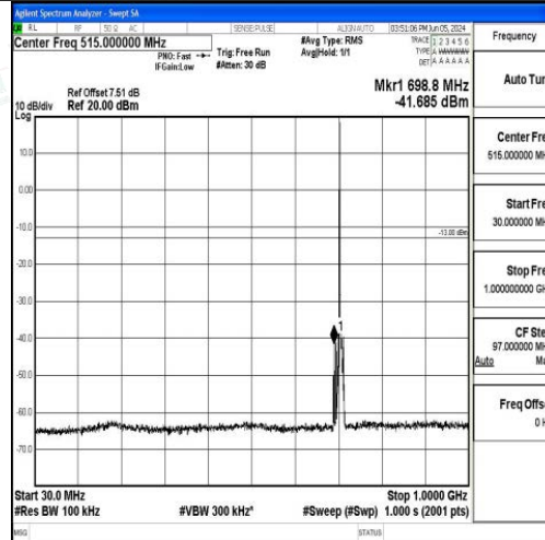
Band17_5MHz_QPSK_23825_1RB#0_30~1000_30~1000
