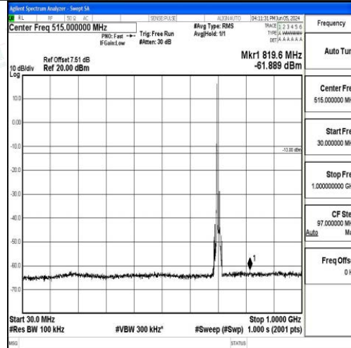
Band17_10MHz_16QAM_23780_1RB#0_30~1000_30~1000
