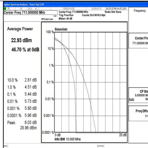
Band17-10MHz-16QAM-23800-1RB#0-PASS
