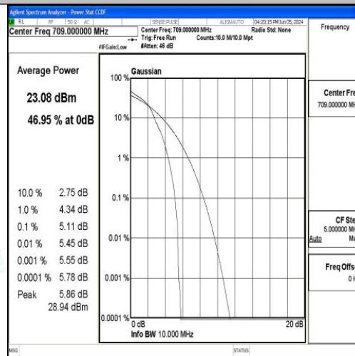
Band17-10MHz-16QAM-23780-1RB#0-PASS
