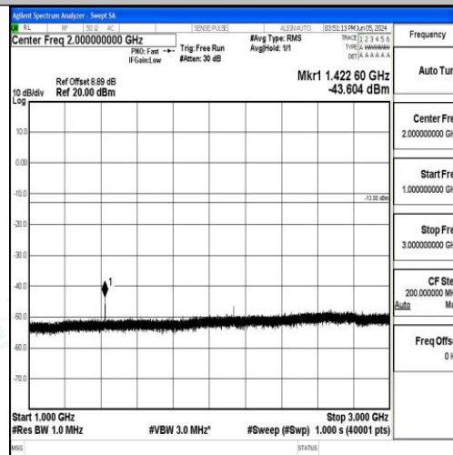
Band17_5MHz_QPSK_23825_1RB#0_1000~3000_1000~3000
