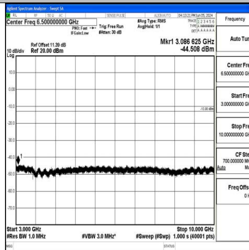
Band17_10MHz_QPSK_23800_1RB#0_3000~10000_3000~10000
