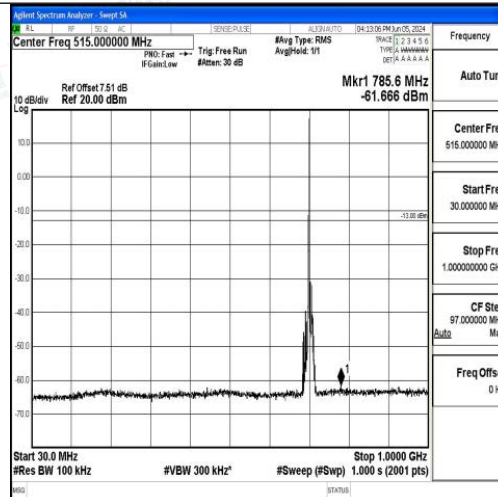
Band17_10MHz_QPSK_23800_1RB#0_30~1000_30~1000
