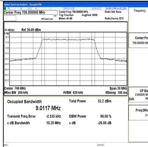
Band17-10MHz-QPSK-23780-50RB#0-PASS
