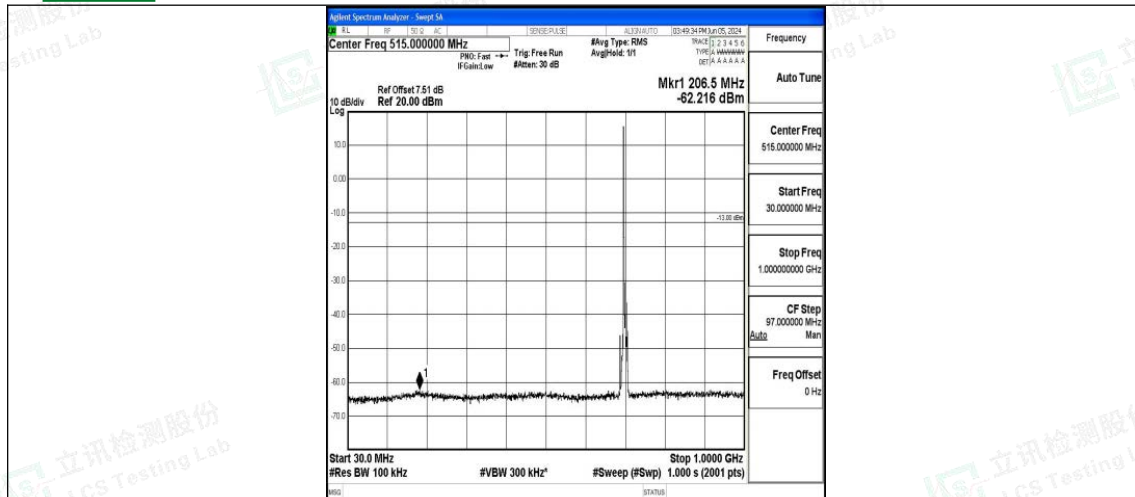
Band17_5MHz_16QAM_23755_1RB#0_30~1000_30~1000
