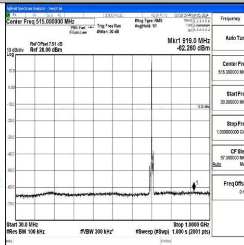
Band17_5MHz_16QAM_23790_1RB#0_30~1000_30~1000
