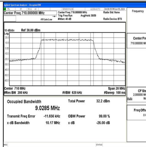
Band17-10MHz-QPSK-23790-50RB#0-PASS
