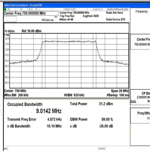
Band17-10MHz-16QAM-23780-50RB#0-PASS
