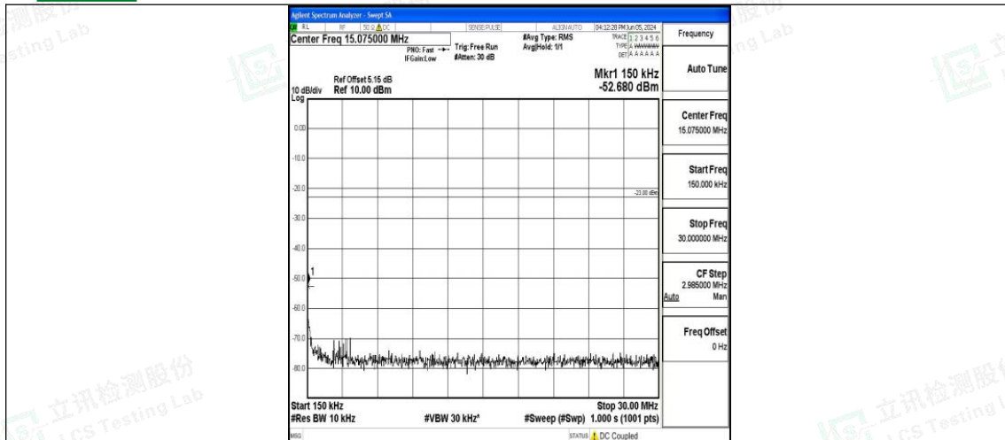
Band17_10MHz_16QAM_23790_1RB#0_0.15~30_0.15~30
