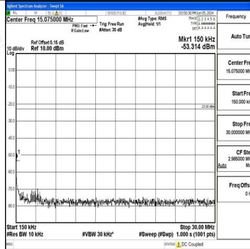
Band17_5MHz_16QAM_23790_1RB#0_0.15~30_0.15~30
