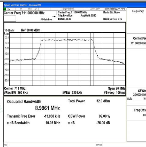
Band17-10MHz-QPSK-23800-50RB#0-PASS
