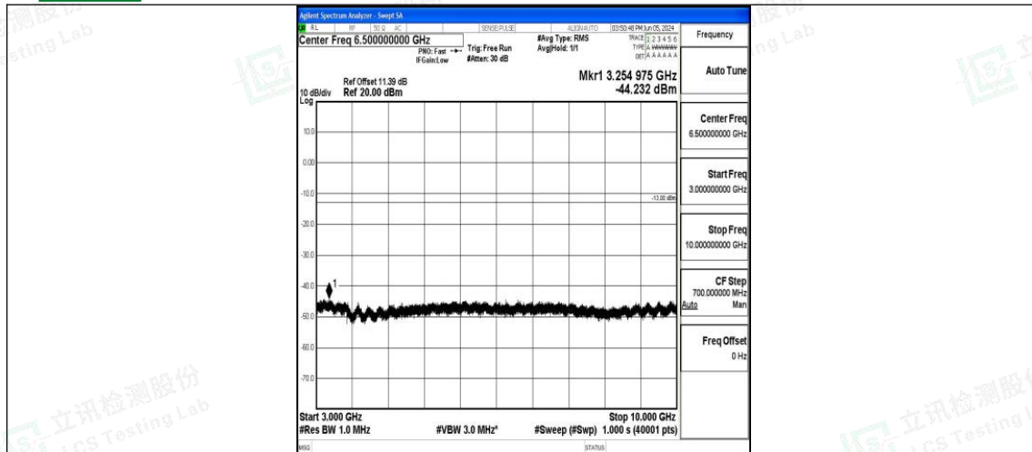
Band17_5MHz_16QAM_23790_1RB#0_3000~10000_3000~10000
