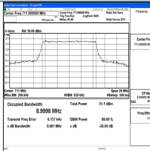
Band17-10MHz-16QAM-23800-50RB#0-PASS
