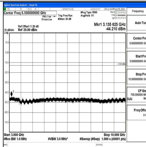
Band17_10MHz_16QAM_23780_1RB#0_3000~10000_3000~10000
