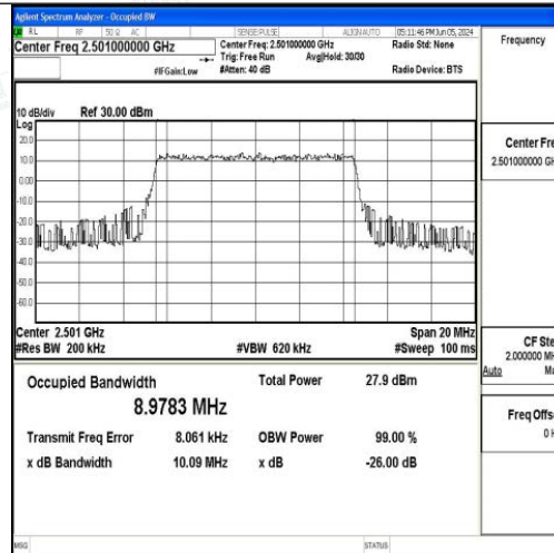
Band41-10MHz-QPSK-39700-50RB#0-PASS
