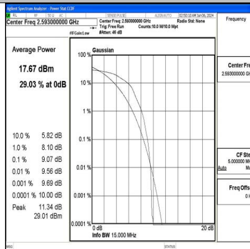
Band41-15MHz-16QAM-40620-1RB#0-PASS
