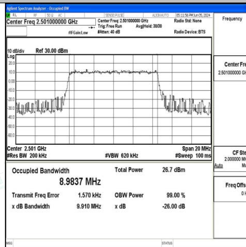
Band41-10MHz-16QAM-39700-50RB#0-PASS
