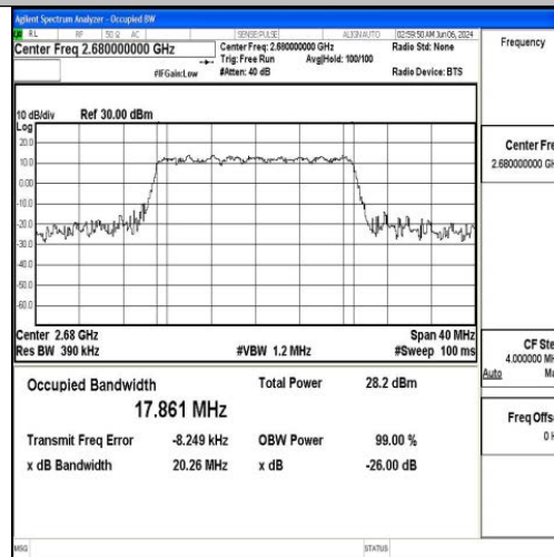
Band41-20MHz-16QAM-41490-100RB#0-PASS
