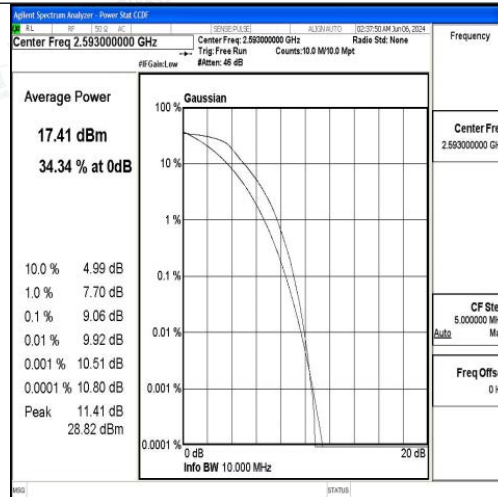
Band41-10MHz-QPSK-40620-50RB#0-PASS
