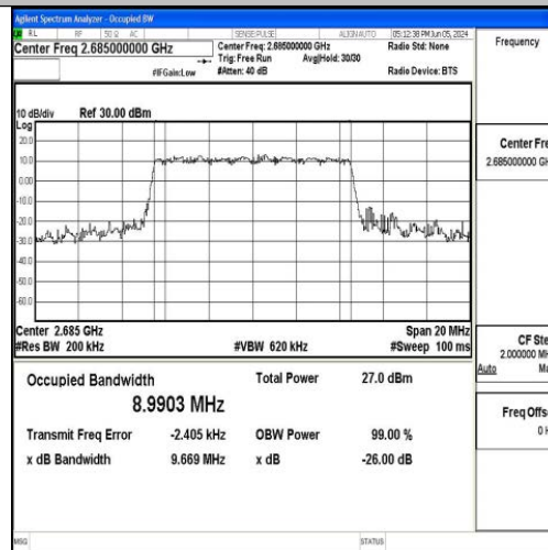
Band41-10MHz-16QAM-41540-50RB#0-PASS
