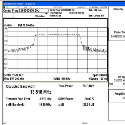
Band41-15MHz-QPSK-39725-75RB#0-PASS
