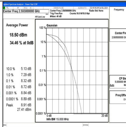
Band41-15MHz-QPSK-40620-1RB#0-PASS
