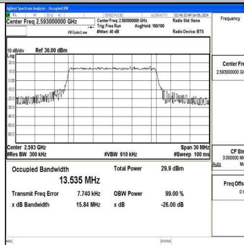
Band41-15MHz-QPSK-40620-75RB#0-PASS
