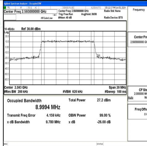
Band41-10MHz-16QAM-40620-50RB#0-PASS
