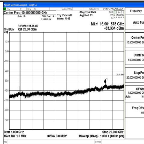
Band41_5MHz_16QAM_41565_1RB#0_1000~20000_1000~20000
