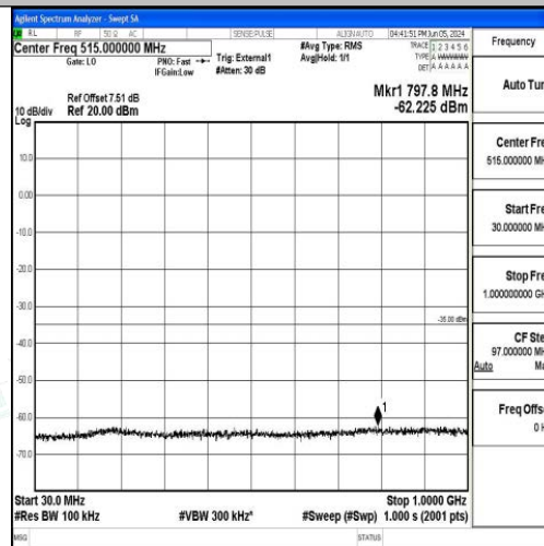
Band41_5MHz_QPSK_40620_1RB#0_30~1000_30~1000
