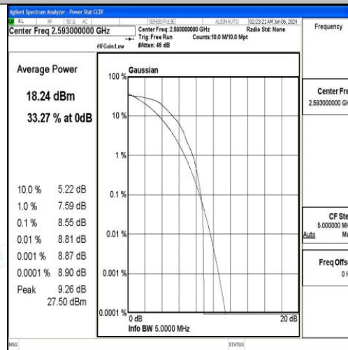
Band41-5MHz-QPSK-40620-1RB#0-PASS
