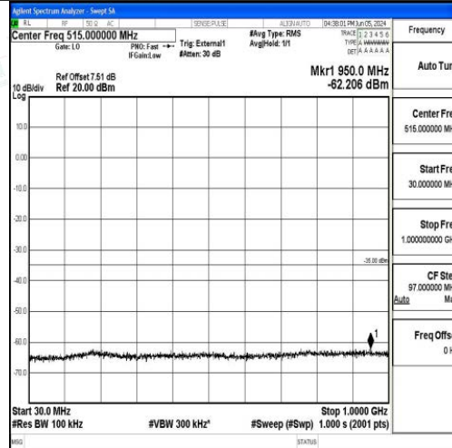
Band41_5MHz_QPSK_39675_1RB#0_30~1000_30~1000
