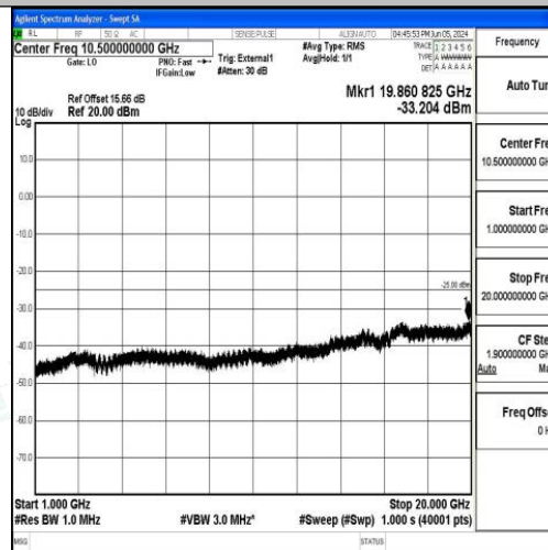
Band41_5MHz_16QAM_40620_1RB#0_1000~20000_1000~20000
