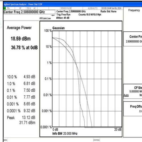
Band41-20MHz-QPSK-39750-1RB#0-PASS
