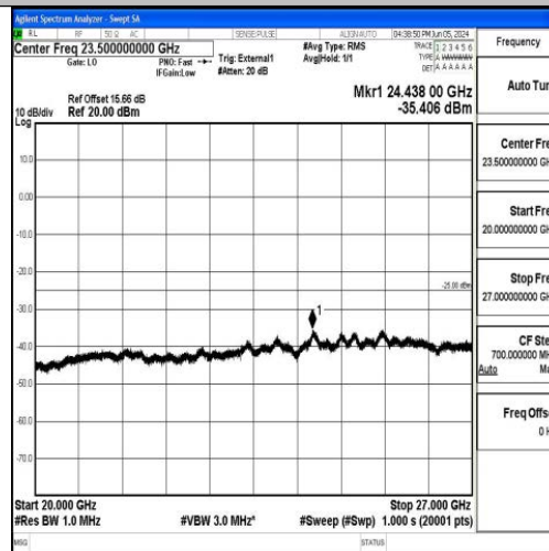
Band41_5MHz_QPSK_39675_1RB#0_20000~27000_20000~27000
