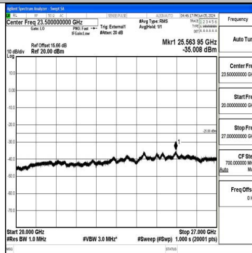
Band41_5MHz_16QAM_40620_1RB#0_20000~27000_20000~27000
