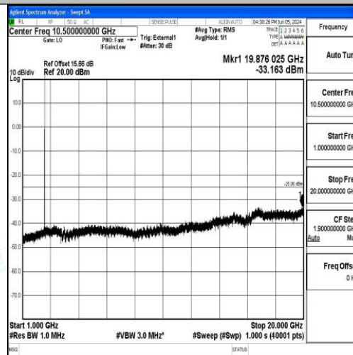
Band41_5MHz_QPSK_39675_1RB#0_1000~20000_1000~20000
