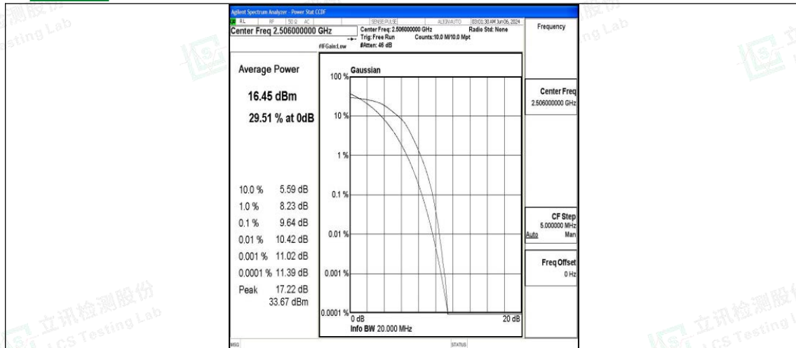
Band41-20MHz-16QAM-39750-100RB#0-PASS
