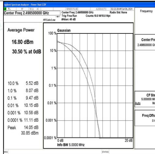
Band41-5MHz-16QAM-39675-25RB#0-PASS
