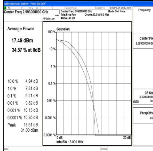
Band41-15MHz-QPSK-40620-75RB#0-PASS
