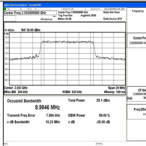
Band41-10MHz-QPSK-40620-50RB#0-PASS
