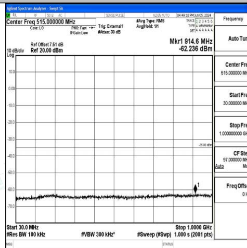
Band41_5MHz_16QAM_41565_1RB#0_30~1000_30~1000
