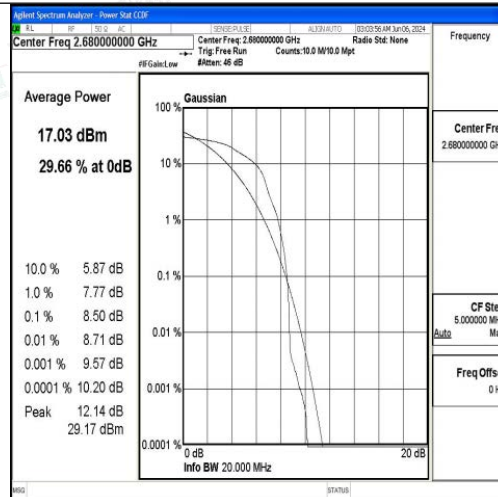
Band41-20MHz-16QAM-41490-1RB#0-PASS
