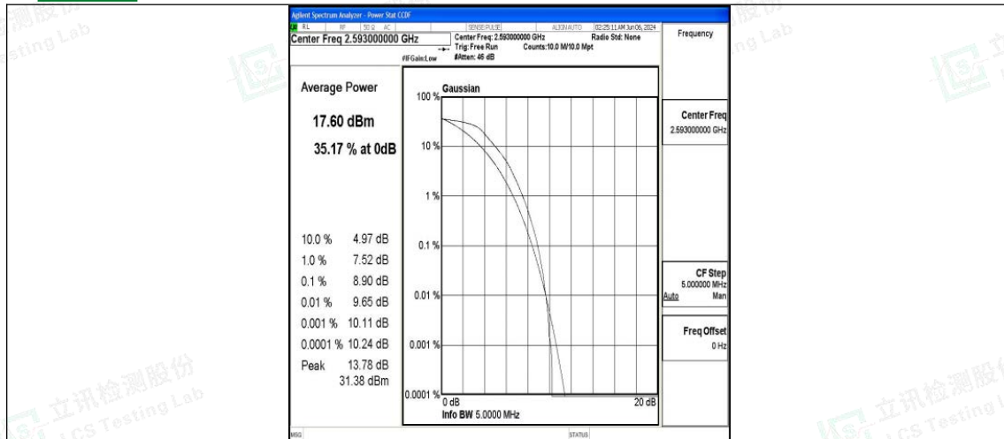
Band41-5MHz-QPSK-40620-25RB#0-PASS
