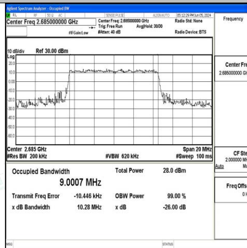
Band41-10MHz-QPSK-41540-50RB#0-PASS
