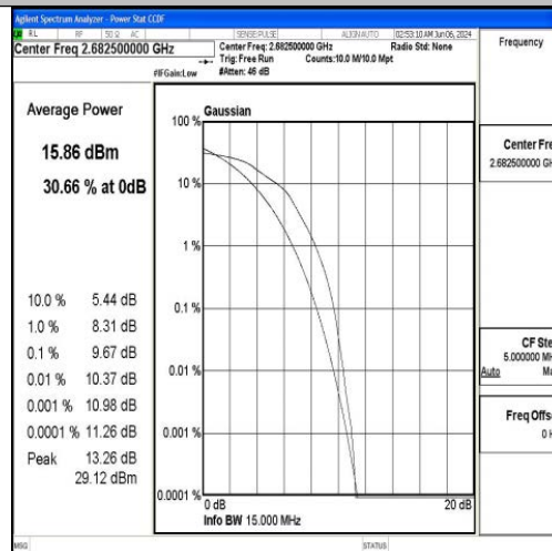
Band41-15MHz-16QAM-41515-75RB#0-PASS
