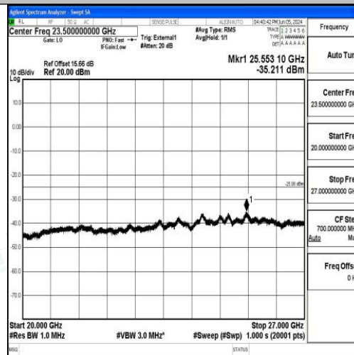
Band41_5MHz_16QAM_39675_1RB#0_20000~27000_20000~27000
