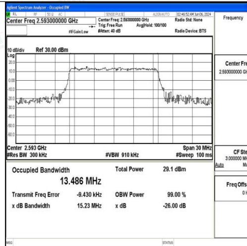
Band41-15MHz-16QAM-40620-75RB#0-PASS
