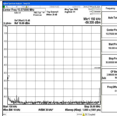
Band41_5MHz_QPSK_40620_1RB#0_0.15~30_0.15~30
