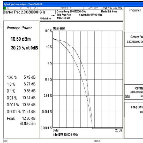
Band41-15MHz-16QAM-39725-75RB#0-PASS
