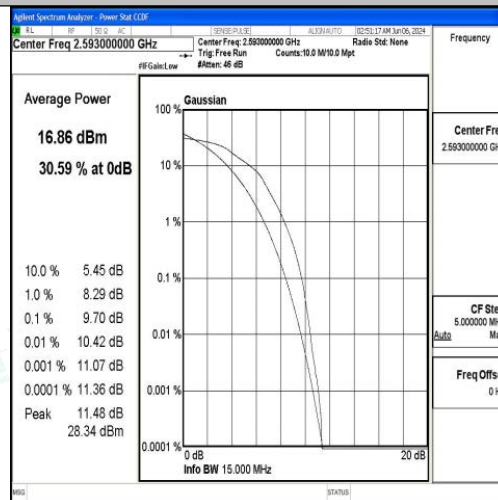
Band41-15MHz-16QAM-40620-75RB#0-PASS
