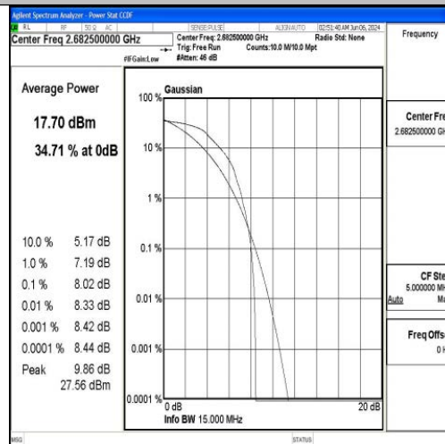
Band41-15MHz-QPSK-41515-1RB#0-PASS
