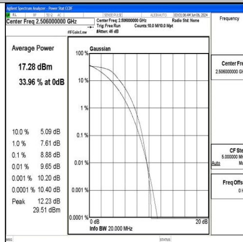
Band41-20MHz-QPSK-39750-100RB#0-PASS
