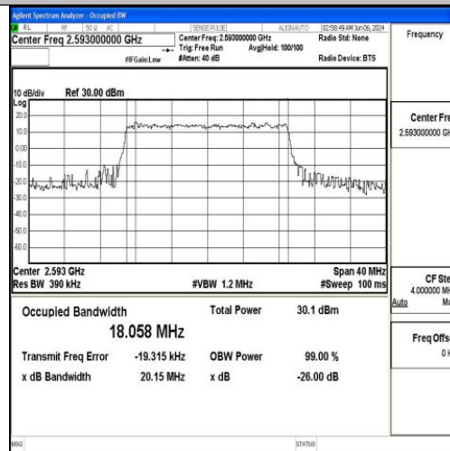
Band41-20MHz-QPSK-40620-100RB#0-PASS
