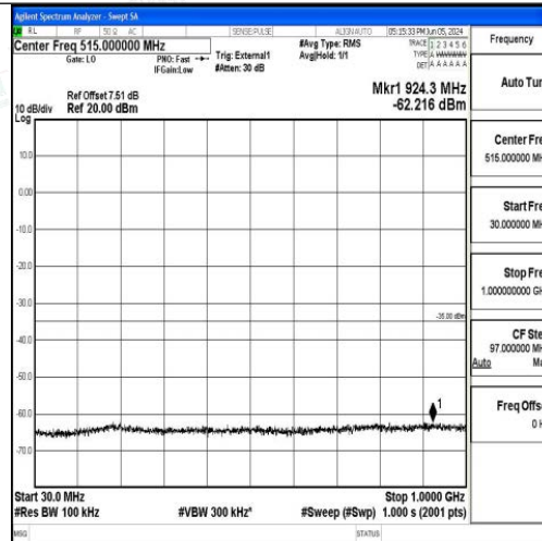
Band41_10MHz_QPSK_39700_1RB#0_30~1000_30~1000
