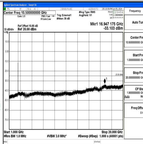
Band41_10MHz_QPSK_39700_1RB#0_1000~20000_1000~20000
