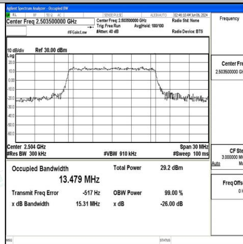
Band41-15MHz-16QAM-39725-75RB#0-PASS
