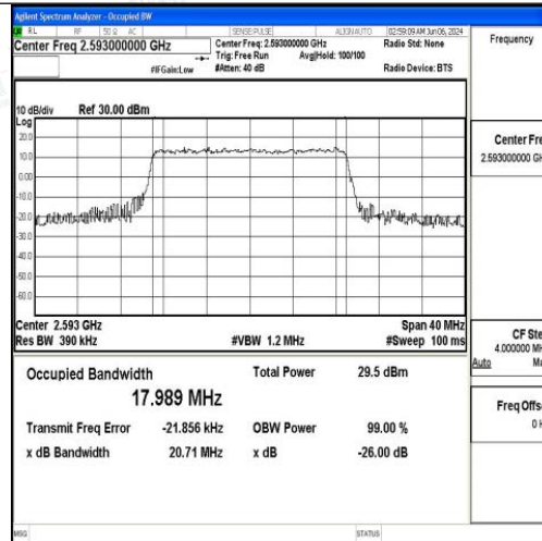
Band41-20MHz-16QAM-40620-100RB#0-PASS
