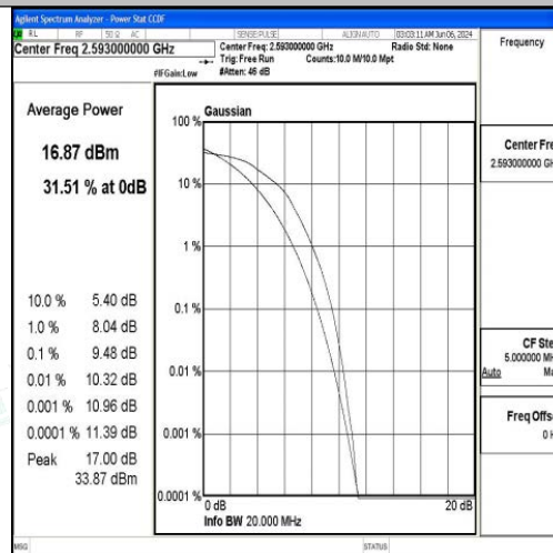
Band41-20MHz-16QAM-40620-100RB#0-PASS
