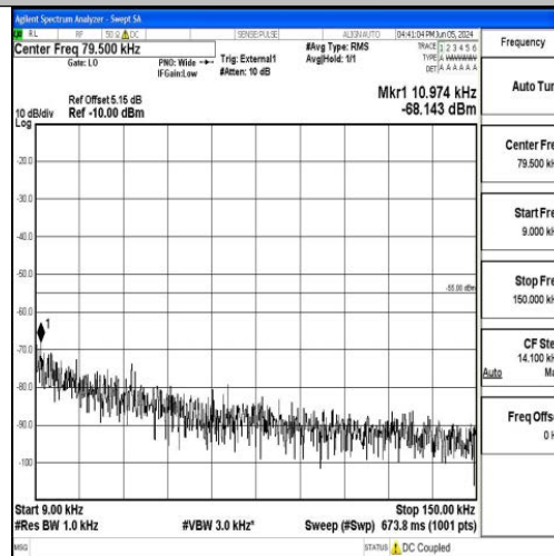
Band41_5MHz_QPSK_40620_1RB#0_0.009~0.15_0.009~0.15
