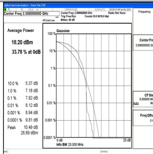
Band41-20MHz-16QAM-39750-1RB#0-PASS
