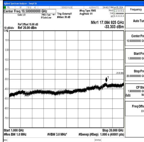
Band41_5MHz_16QAM_39675_1RB#0_1000~20000_1000~20000
