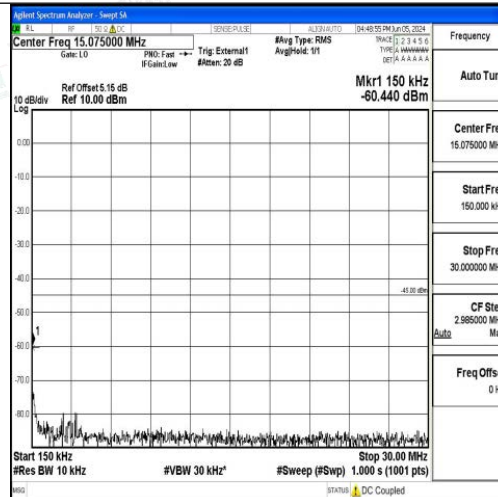
Band41_5MHz_16QAM_41565_1RB#0_0.15~30_0.15~30
