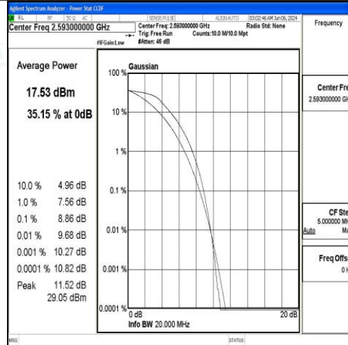
Band41-20MHz-QPSK-40620-100RB#0-PASS
