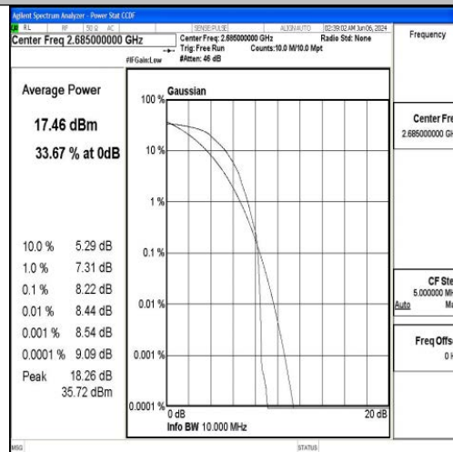
Band41-10MHz-QPSK-41540-1RB#0-PASS
