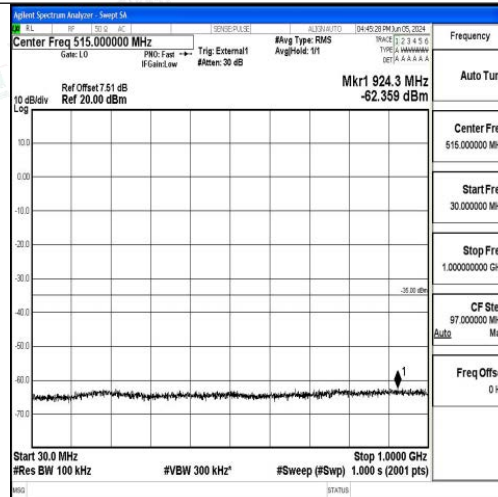
Band41_5MHz_16QAM_40620_1RB#0_30~1000_30~1000
