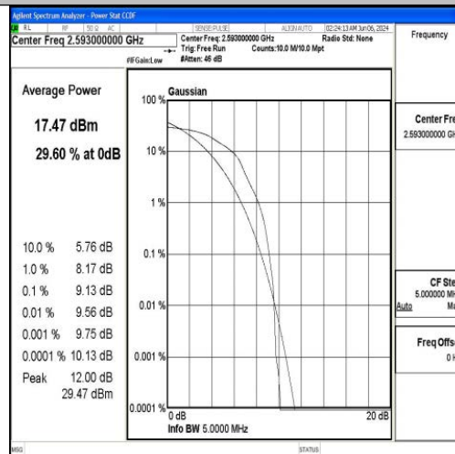
Band41-5MHz-16QAM-40620-1RB#0-PASS
