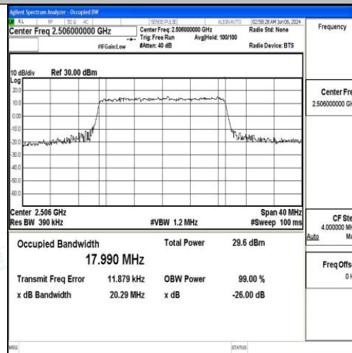
Band41-20MHz-16QAM-39750-100RB#0-PASS
