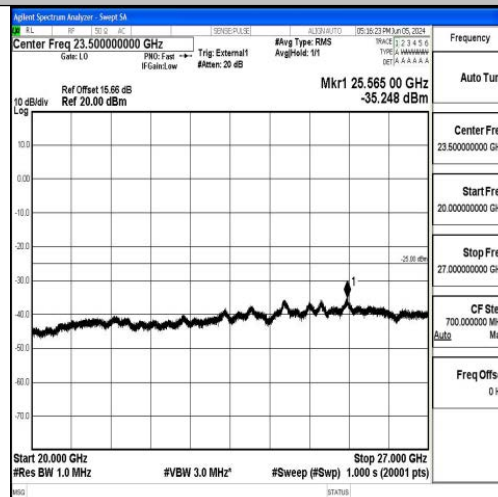
Band41_10MHz_QPSK_39700_1RB#0_20000~27000_20000~27000
