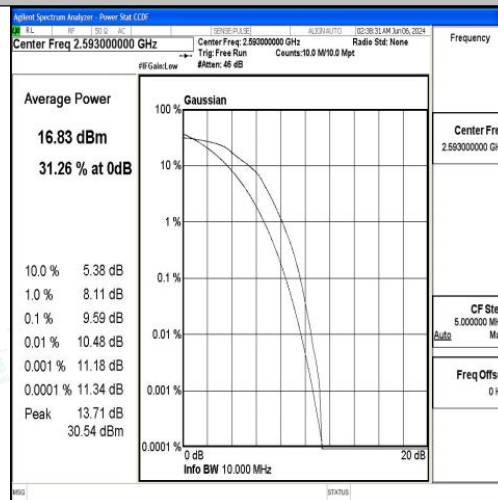
Band41-10MHz-16QAM-40620-50RB#0-PASS
