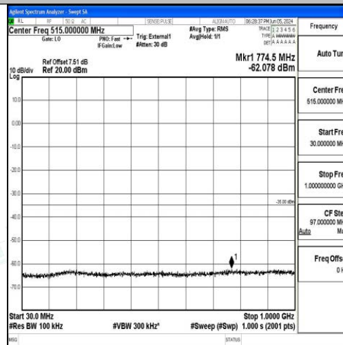
Band41_20MHz_16QAM_41490_1RB#0_30~1000_30~1000
