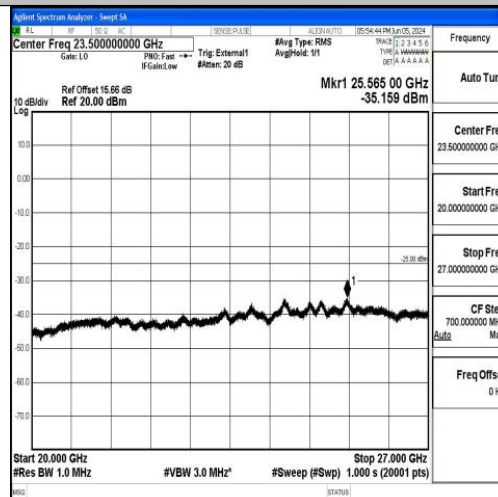
Band41_15MHz_16QAM_40620_1RB#0_20000~27000_20000~27000
