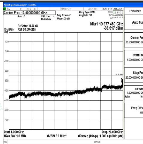
Band41_15MHz_QPSK_39725_1RB#0_1000~20000_1000~20000
