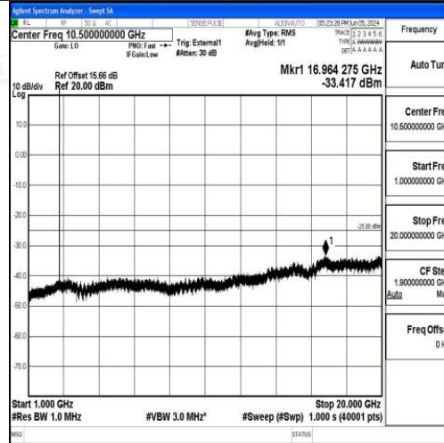
Band41_10MHz_QPSK_41540_1RB#0_1000~20000_1000~20000
