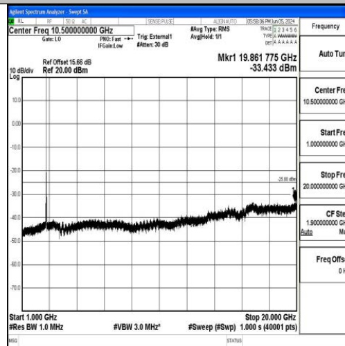
Band41_15MHz_16QAM_41515_1RB#0_1000~20000_1000~20000
