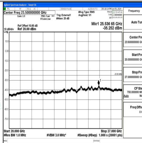
Band41_10MHz_16QAM_39700_1RB#0_20000~27000_20000~27000
