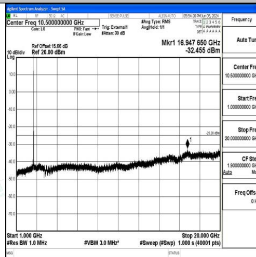
Band41_15MHz_16QAM_40620_1RB#0_1000~20000_1000~20000
