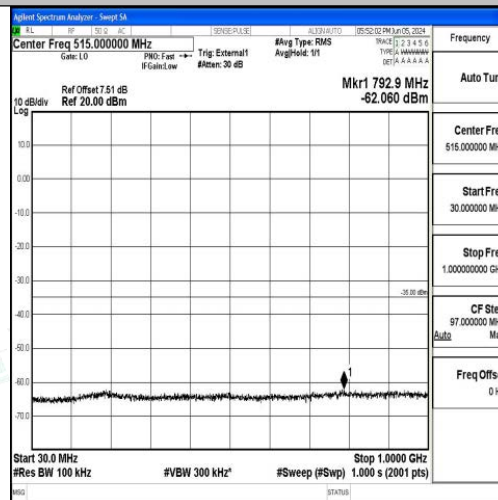
Band41_15MHz_QPSK_40620_1RB#0_30~1000_30~1000
