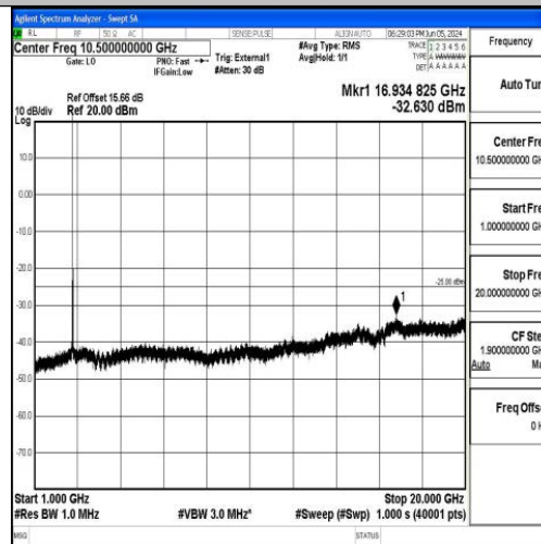
Band41_20MHz_16QAM_41490_1RB#0_1000~20000_1000~20000
