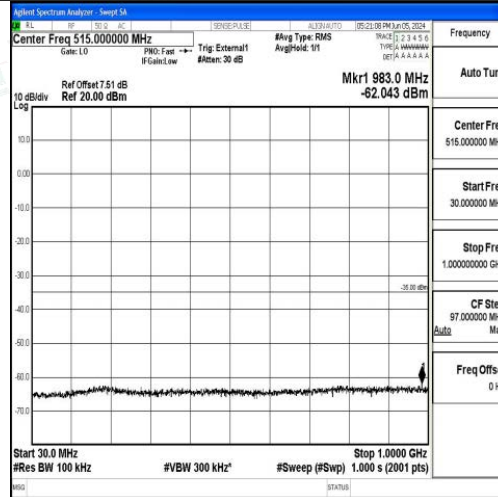
Band41_10MHz_16QAM_40620_1RB#0_30~1000_30~1000
