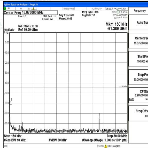
Band41_20MHz_QPSK_40620_1RB#0_0.15~30_0.15~30
