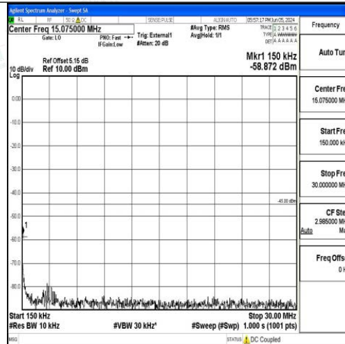
Band41_15MHz_16QAM_41515_1RB#0_0.15~30_0.15~30
