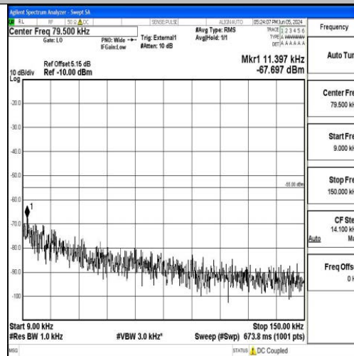
Band41_10MHz_16QAM_41540_1RB#0_0.009~0.15_0.009~0.15
