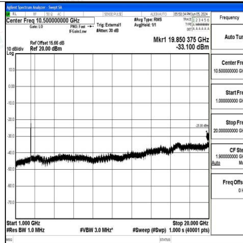
Band41_15MHz_16QAM_39725_1RB#0_1000~20000_1000~20000
