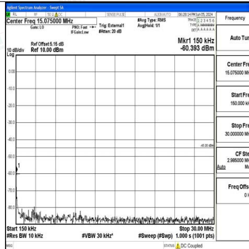
Band41_20MHz_16QAM_41490_1RB#0_0.15~30_0.15~30
