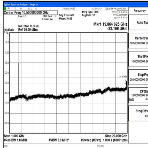
Band41_10MHz_16QAM_39700_1RB#0_1000~20000_1000~20000
