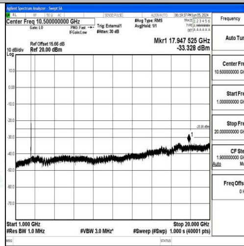
Band41_20MHz_QPSK_39750_1RB#0_1000~20000_1000~20000
