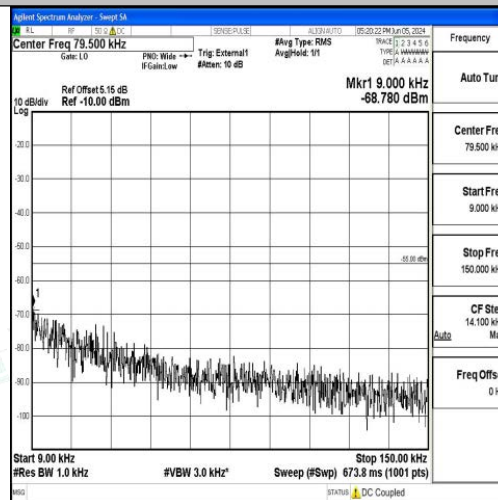
Band41_10MHz_16QAM_40620_1RB#0_0.009~0.15_0.009~0.15
