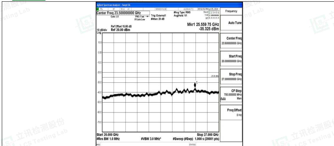
Band41_15MHz_QPSK_40620_1RB#0_20000~27000_20000~27000
