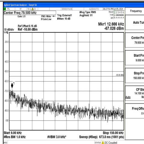
Band41_20MHz_16QAM_41490_1RB#0_0.009~0.15_0.009~0.15
