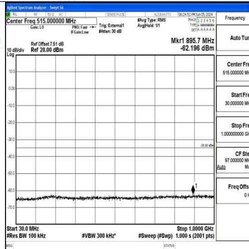
Band41_20MHz_16QAM_40620_1RB#0_30~1000_30~1000
