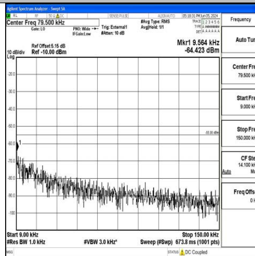
Band41_10MHz_QPSK_40620_1RB#0_0.009~0.15_0.009~0.15
