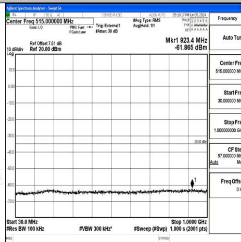
Band41_10MHz_QPSK_40620_1RB#0_30~1000_30~1000
