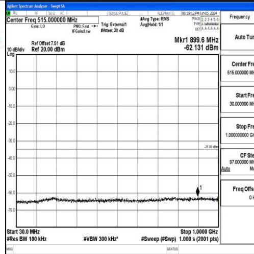
Band41_20MHz_QPSK_39750_1RB#0_30~1000_30~1000
