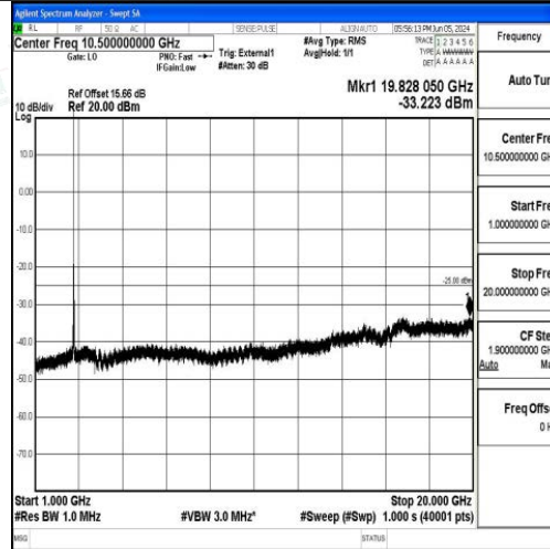
Band41_15MHz_QPSK_41515_1RB#0_1000~20000_1000~20000
