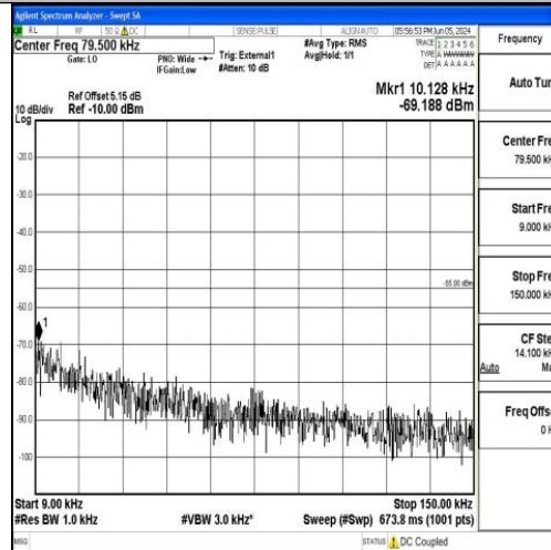
Band41_15MHz_16QAM_41515_1RB#0_0.009~0.15_0.009~0.15
