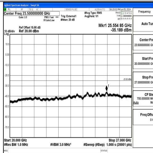
Band41_20MHz_QPSK_39750_1RB#0_20000~27000_20000~27000
