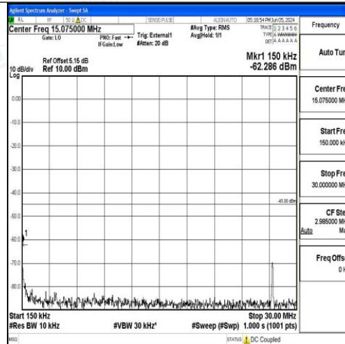
Band41_10MHz_QPSK_40620_1RB#0_0.15~30_0.15~30
