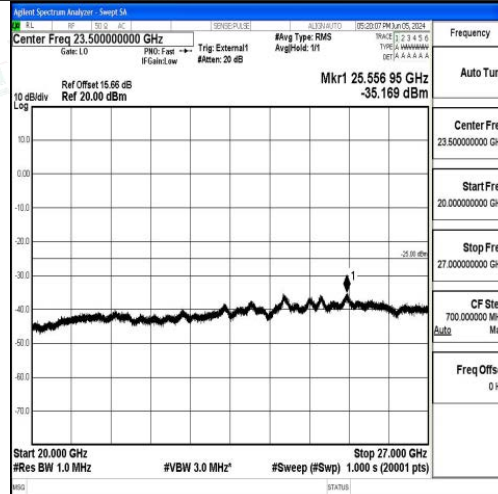
Band41_10MHz_QPSK_40620_1RB#0_20000~27000_20000~27000
