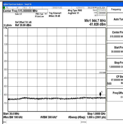
Band41_20MHz_QPSK_40620_1RB#0_30~1000_30~1000
