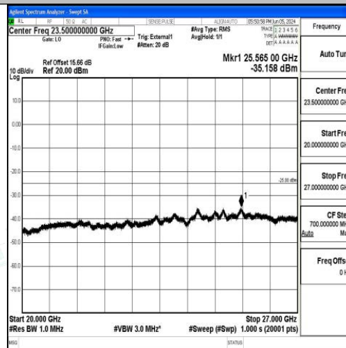
Band41_15MHz_16QAM_39725_1RB#0_20000~27000_20000~27000
