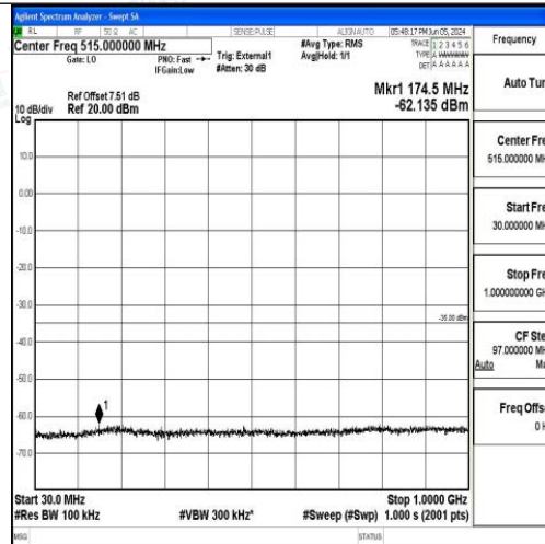
Band41_15MHz_QPSK_39725_1RB#0_30~1000_30~1000
