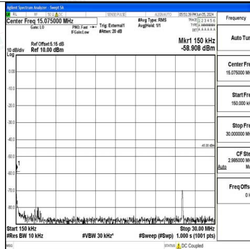
Band41_15MHz_QPSK_40620_1RB#0_0.15~30_0.15~30
