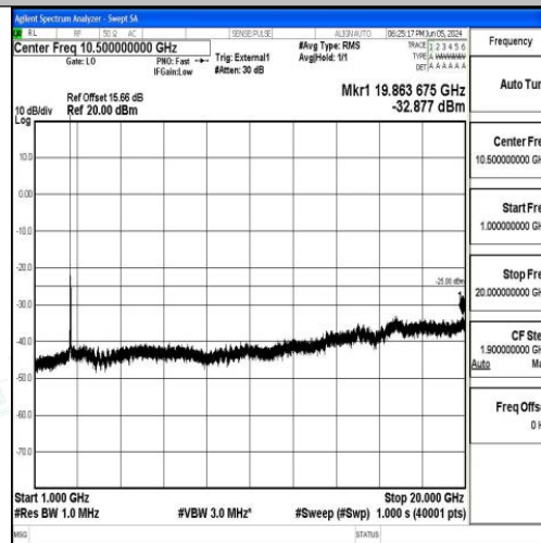
Band41_20MHz_16QAM_40620_1RB#0_1000~20000_1000~20000
