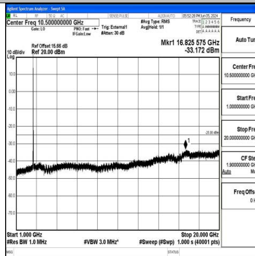
Band41_15MHz_QPSK_40620_1RB#0_1000~20000_1000~20000
