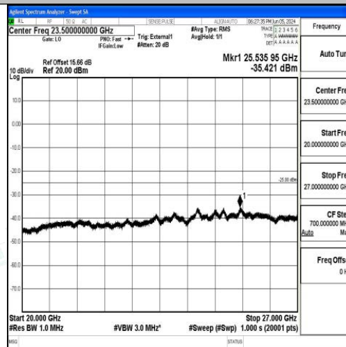
Band41_20MHz_QPSK_41490_1RB#0_20000~27000_20000~27000
