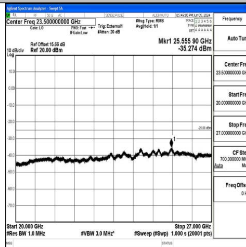
Band41_15MHz_QPSK_39725_1RB#0_20000~27000_20000~27000
