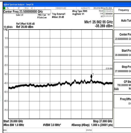
Band41_10MHz_QPSK_41540_1RB#0_20000~27000_20000~27000
