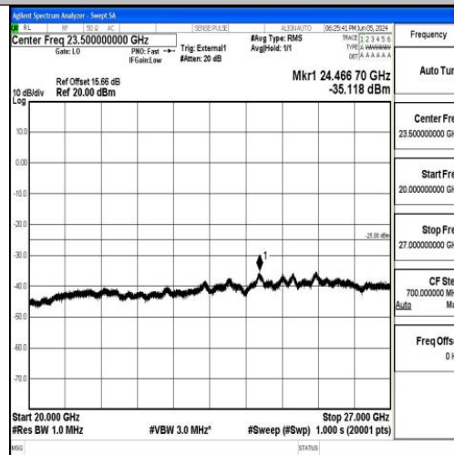
Band41_20MHz_16QAM_40620_1RB#0_20000~27000_20000~27000
