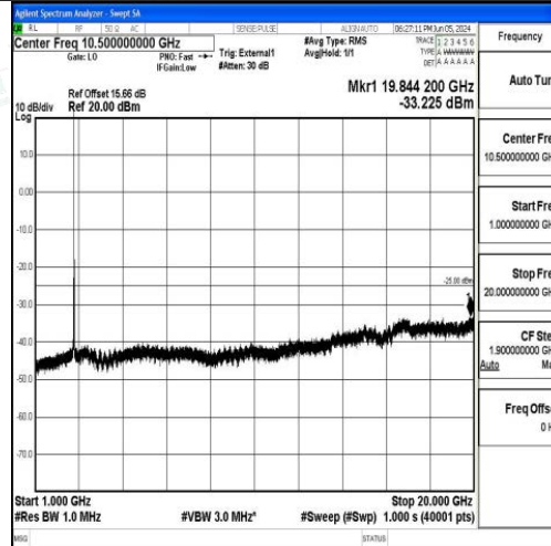
Band41_20MHz_QPSK_41490_1RB#0_1000~20000_1000~20000
