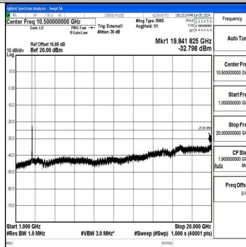
Band41_20MHz_QPSK_40620_1RB#0_1000~20000_1000~20000
