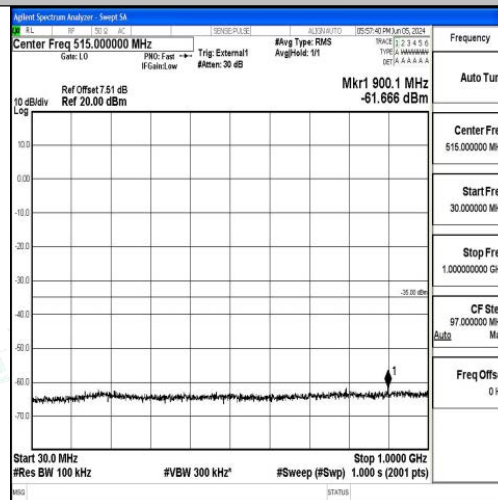
Band41_15MHz_16QAM_41515_1RB#0_30~1000_30~1000
