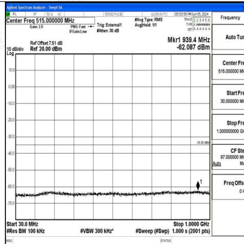
Band41_15MHz_16QAM_40620_1RB#0_30~1000_30~1000
