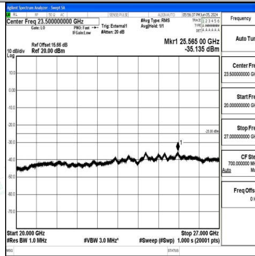
Band41_15MHz_QPSK_41515_1RB#0_20000~27000_20000~27000
