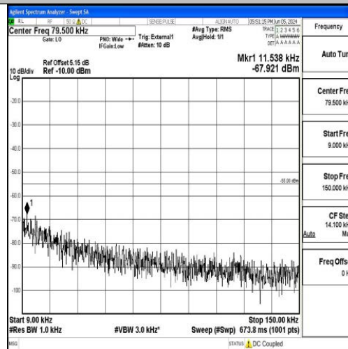
Band41_15MHz_QPSK_40620_1RB#0_0.009~0.15_0.009~0.15
