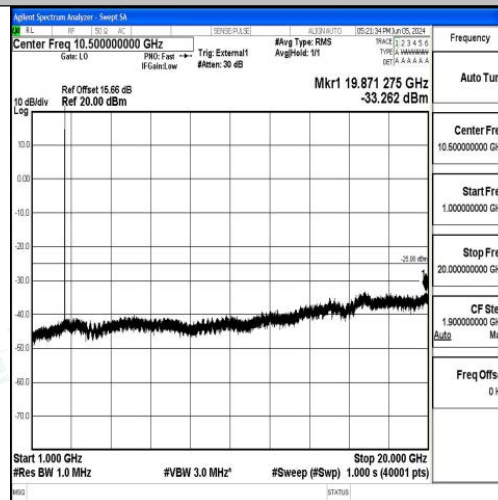
Band41_10MHz_16QAM_40620_1RB#0_1000~20000_1000~20000
