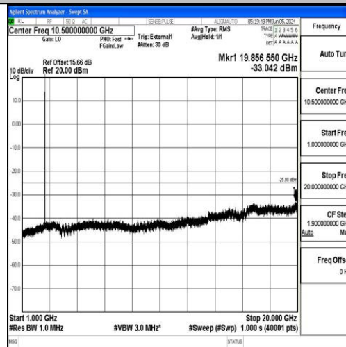
Band41_10MHz_QPSK_40620_1RB#0_1000~20000_1000~20000
