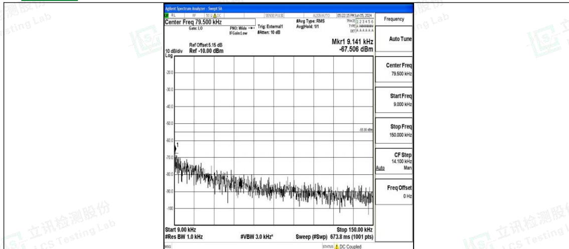
Band41_10MHz_QPSK_41540_1RB#0_0.009~0.15_0.009~0.15
