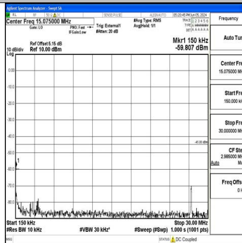
Band41_10MHz_16QAM_40620_1RB#0_0.15~30_0.15~30
