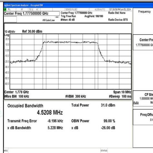
Band66-5MHz-QPSK-132647-25RB#0-PASS
