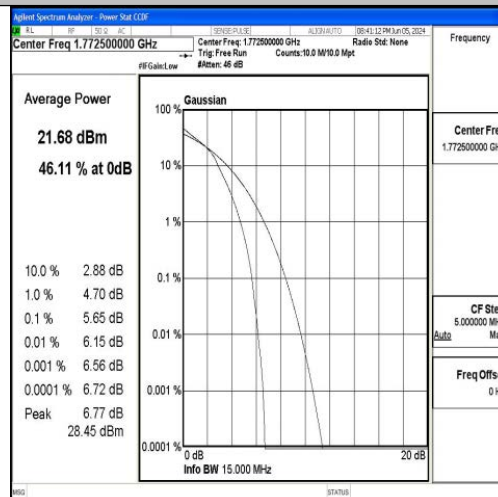
Band66-15MHz-16QAM-132597-75RB#0-PASS
