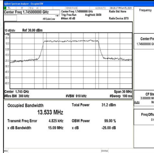
Band66-15MHz-16QAM-132322-75RB#0-PASS
