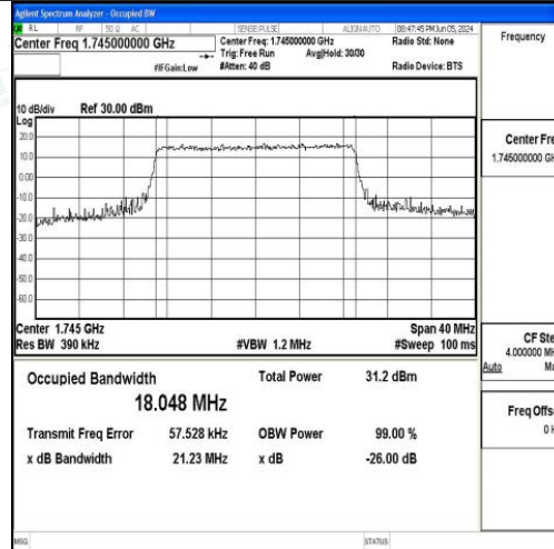
Band66-20MHz-16QAM-132322-100RB#0-PASS
