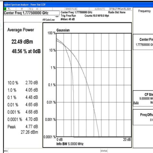
Band66-5MHz-16QAM-132647-1RB#0-PASS
