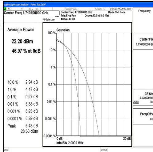
Band66-1.4MHz-16QAM-131979-6RB#0-PASS
