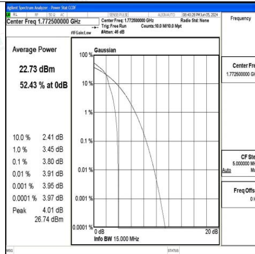
Band66-15MHz-16QAM-132597-1RB#0-PASS
