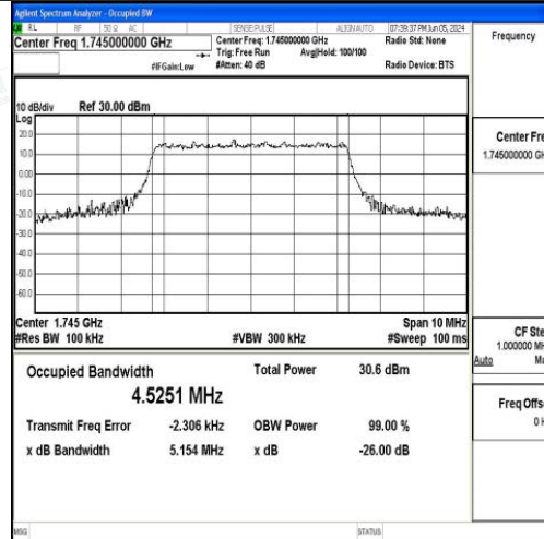
Band66-5MHz-16QAM-132322-25RB#0-PASS
