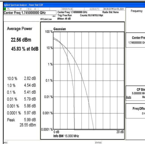
Band66-15MHz-16QAM-132322-1RB#0-PASS
