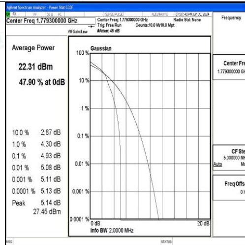
Band66-1.4MHz-16QAM-132665-1RB#0-PASS
