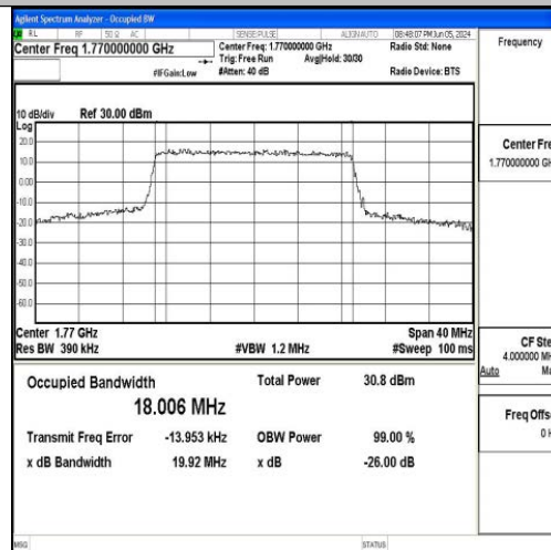
Band66-20MHz-16QAM-132572-100RB#0-PASS
