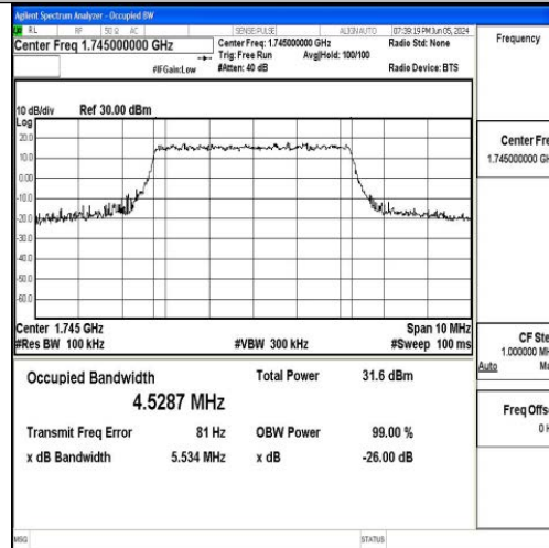
Band66-5MHz-QPSK-132322-25RB#0-PASS
