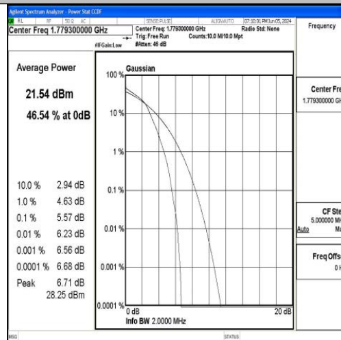
Band66-1.4MHz-16QAM-132665-6RB#0-PASS
