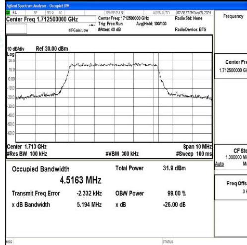
Band66-5MHz-QPSK-131997-25RB#0-PASS
