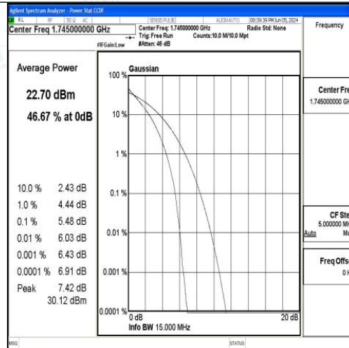
Band66-15MHz-QPSK-132322-75RB#0-PASS
