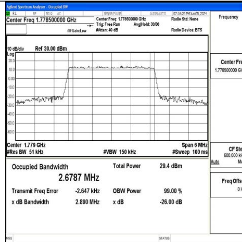
Band66-3MHz-16QAM-132657-15RB#0-PASS
