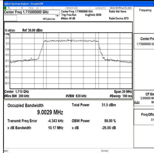
Band66-10MHz-QPSK-132022-50RB#0-PASS
