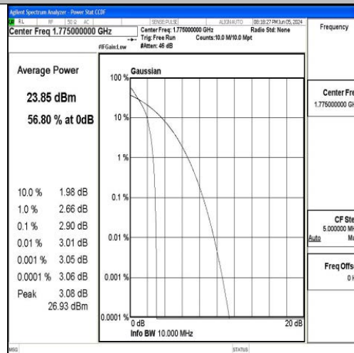
Band66-10MHz-QPSK-132622-1RB#0-PASS
