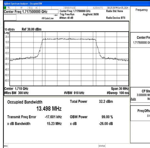
Band66-15MHz-QPSK-132047-75RB#0-PASS
