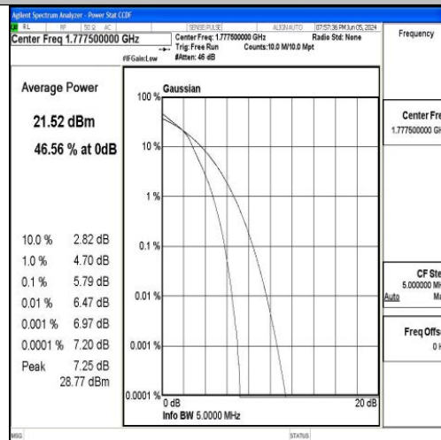
Band66-5MHz-16QAM-132647-25RB#0-PASS
