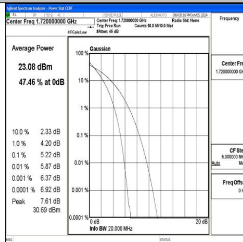
Band66-20MHz-QPSK-132072-100RB#0-PASS
