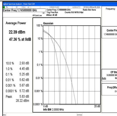
Band66-1.4MHz-16QAM-132322-1RB#0-PASS
