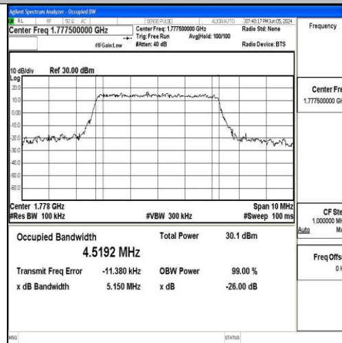
Band66-5MHz-16QAM-132647-25RB#0-PASS
