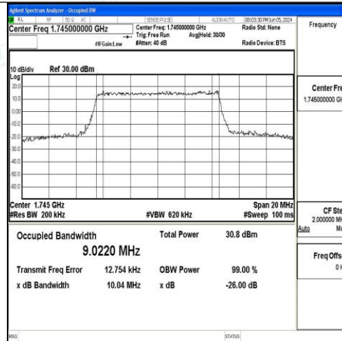
Band66-10MHz-16QAM-132322-50RB#0-PASS
