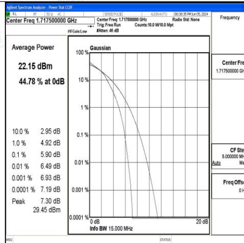
Band66-15MHz-16QAM-132047-75RB#0-PASS
