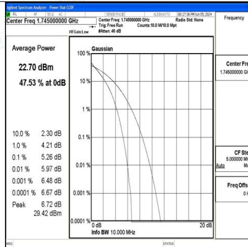
Band66-10MHz-QPSK-132322-50RB#0-PASS
