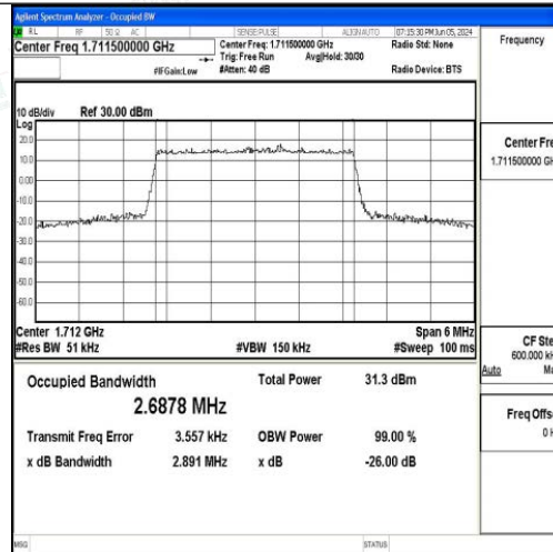
Band66-3MHz-QPSK-131987-15RB#0-PASS
