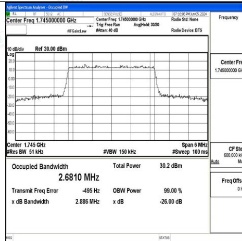
Band66-3MHz-16QAM-132322-15RB#0-PASS
