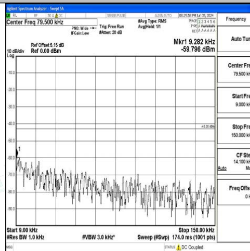
Band66_15MHz_QPSK_132597_1RB#0_0.009~0.15_0.009~0.15
