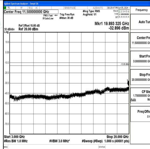
Band66_15MHz_16QAM_132322_1RB#0_3000~20000_3000~20000
