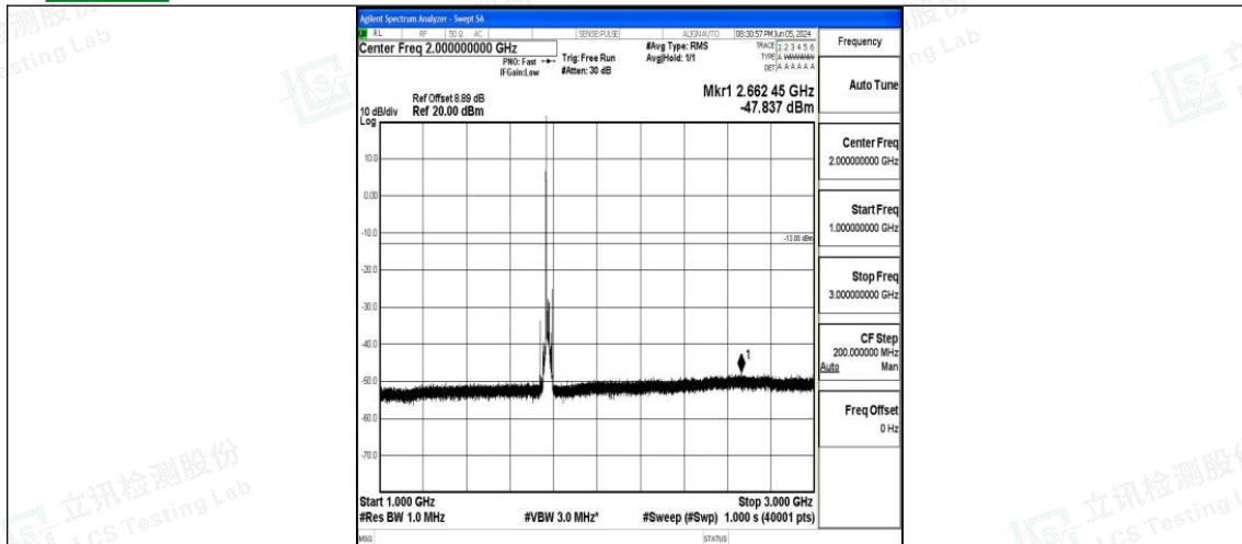
Band66_15MHz_16QAM_132597_1RB#0_1000~3000_1000~3000
