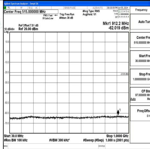
Band66_15MHz_QPSK_132597_1RB#0_30~1000_30~1000
