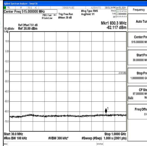
Band66_20MHz_QPSK_132572_1RB#0_30~1000_30~1000
