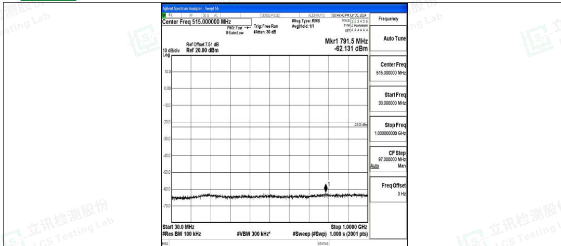
Band66_20MHz_16QAM_132072_1RB#0_30~1000_30~1000
