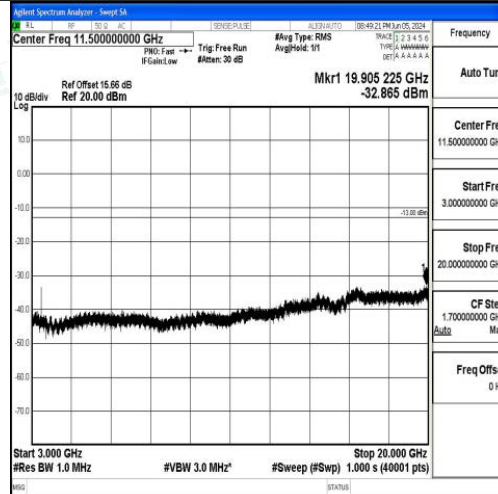
Band66_20MHz_QPSK_132072_1RB#0_3000~20000_3000~20000
