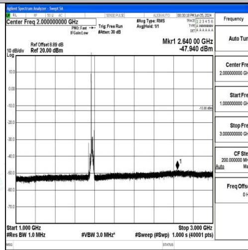
Band66_15MHz_QPSK_132597_1RB#0_1000~3000_1000~3000
