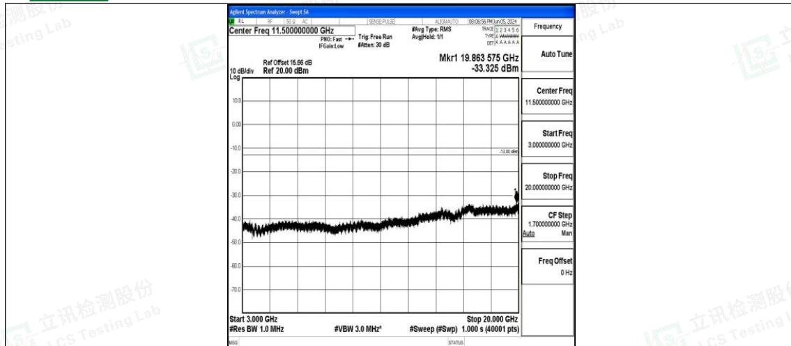
Band66_10MHz_16QAM_132322_1RB#0_3000~20000_3000~20000
