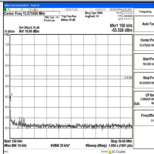
Band66_15MHz_QPSK_132597_1RB#0_0.15~30_0.15~30
