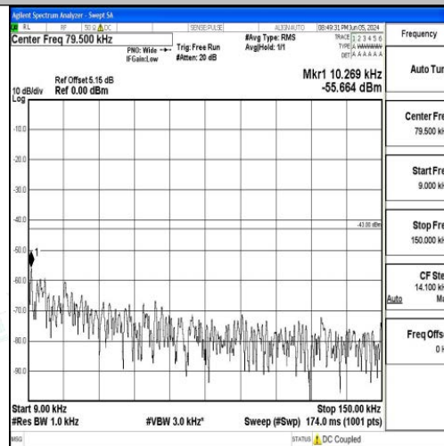
Band66_20MHz_16QAM_132072_1RB#0_0.009~0.15_0.009~0.15
