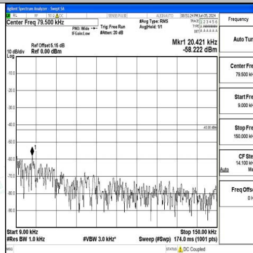
Band66_20MHz_QPSK_132572_1RB#0_0.009~0.15_0.009~0.15
