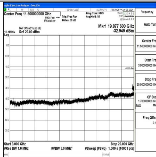
Band66_15MHz_QPSK_132597_1RB#0_3000~20000_3000~20000
