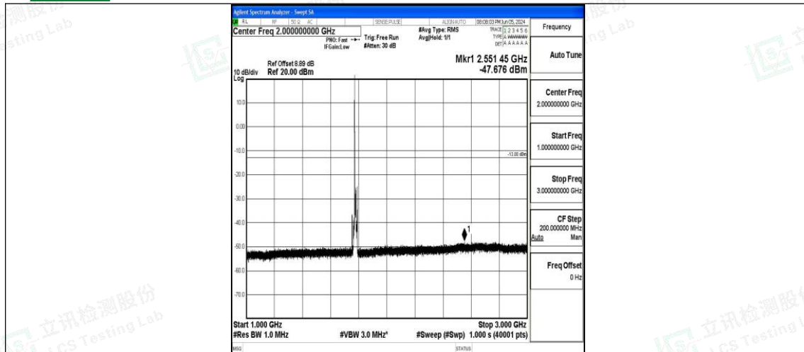
Band66_10MHz_16QAM_132622_1RB#0_1000~3000_1000~3000
