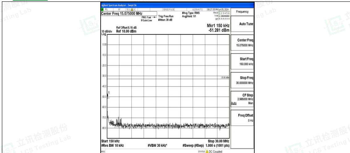
Band66_15MHz_QPSK_132047_1RB#0_0.15~30_0.15~30
