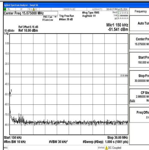
Band66_20MHz_16QAM_132072_1RB#0_0.15~30_0.15~30
