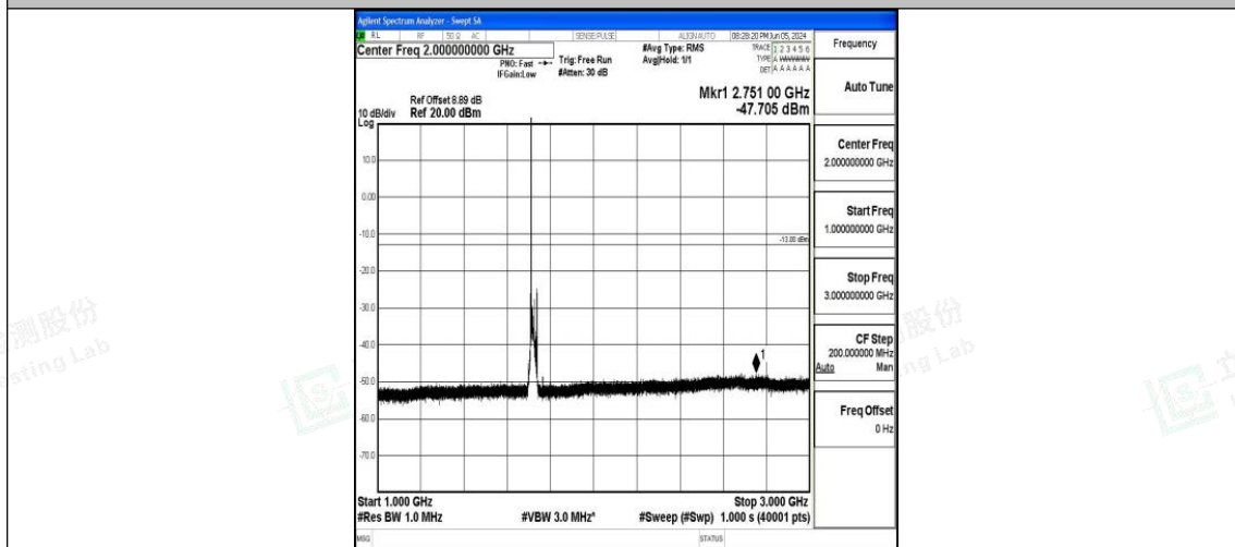
Band66_15MHz_16QAM_132047_1RB#0_1000~3000_1000~3000
