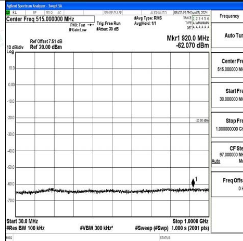
Band66_10MHz_QPSK_132622_1RB#0_30~1000_30~1000
