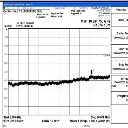
Band66_20MHz_QPSK_132572_1RB#0_3000~20000_3000~20000
