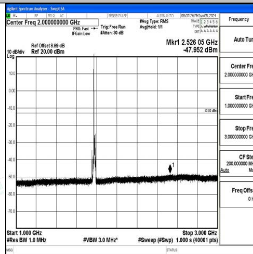
Band66_10MHz_QPSK_132622_1RB#0_1000~3000_1000~3000
