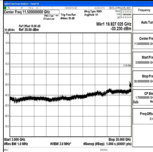
Band66_20MHz_16QAM_132322_1RB#0_3000~20000_3000~20000
