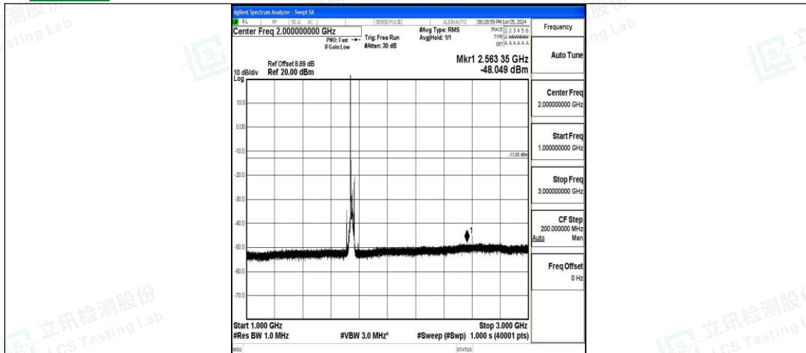
Band66_15MHz_QPSK_132322_1RB#0_1000~3000_1000~3000
