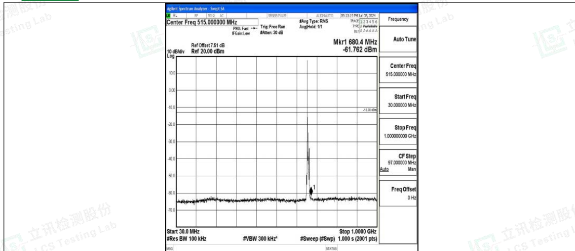
Band71_5MHz_QPSK_133147_1RB#0_30~1000_30~1000
