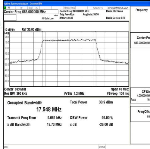
Band71-20MHz-16QAM-133322-100RB#0-PASS
