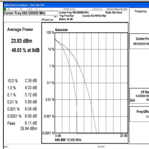
Band71-15MHz-QPSK-133297-1RB#0-PASS
