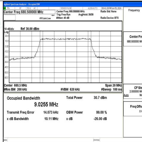
Band71-10MHz-16QAM-133297-50RB#0-PASS
