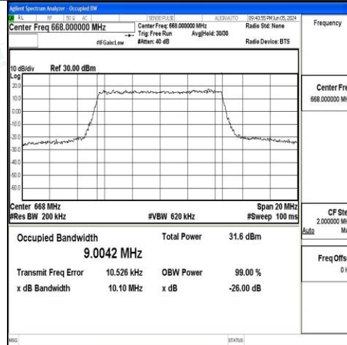
Band71-10MHz-QPSK-133172-50RB#0-PASS
