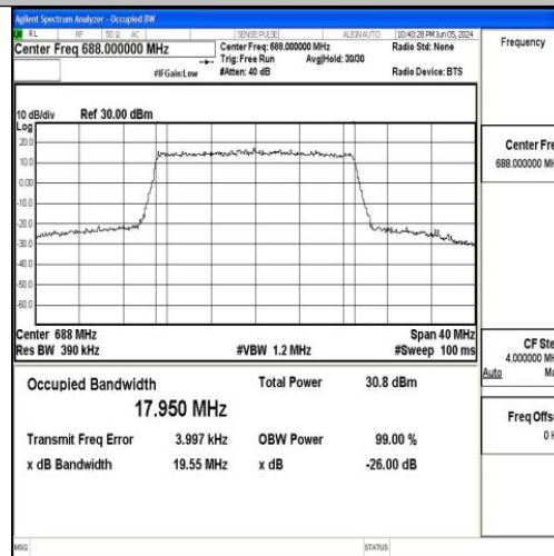
Band71-20MHz-16QAM-133372-100RB#0-PASS
