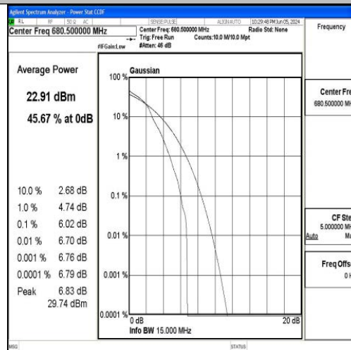
Band71-15MHz-16QAM-133297-1RB#0-PASS
