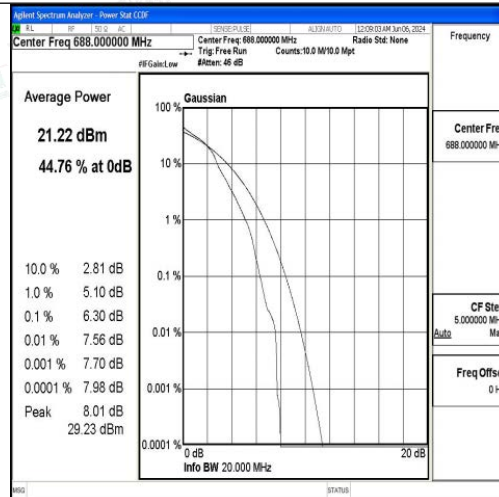
Band71-20MHz-16QAM-133372-1RB#0-PASS
