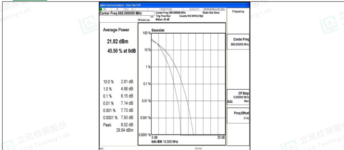
Band71-10MHz-16QAM-133172-50RB#0-PASS
