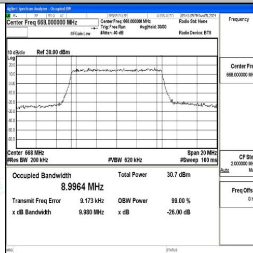
Band71-10MHz-16QAM-133172-50RB#0-PASS
