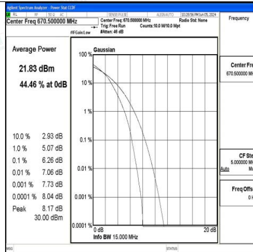
Band71-15MHz-16QAM-133197-75RB#0-PASS
