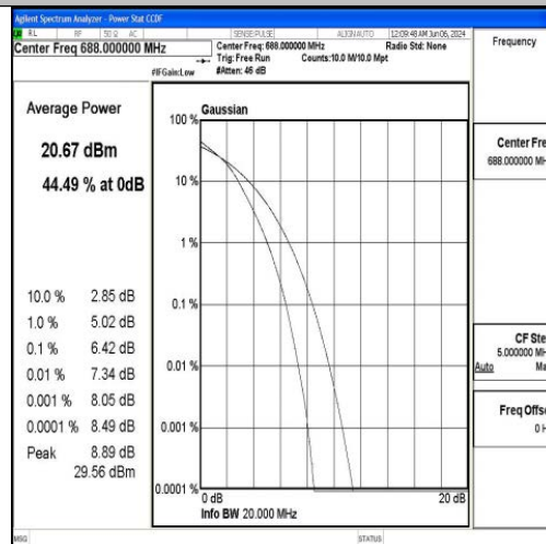
Band71-20MHz-16QAM-133372-100RB#0-PASS
