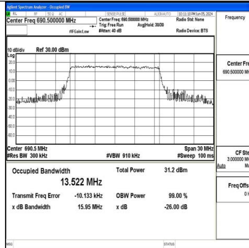
Band71-15MHz-16QAM-133397-75RB#0-PASS
