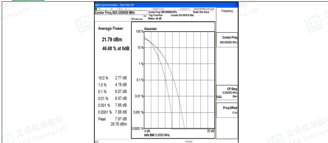
Band71-5MHz-16QAM-133147-25RB#0-PASS
