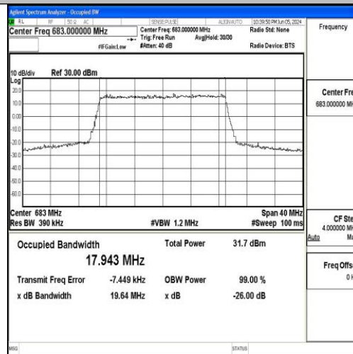
Band71-20MHz-QPSK-133322-100RB#0-PASS
