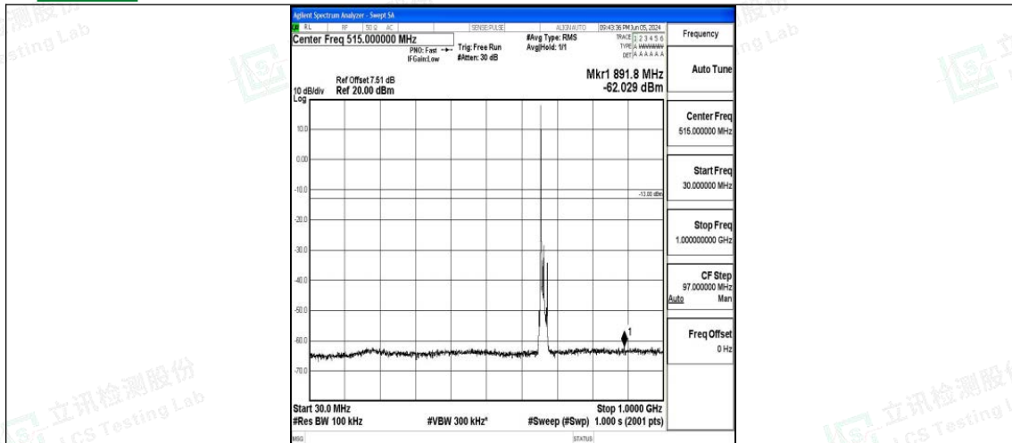
Band71_10MHz_QPSK_133172_1RB#0_30~1000_30~1000
