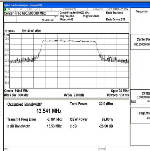
Band71-15MHz-QPSK-133397-75RB#0-PASS
