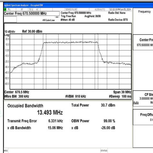
Band71-15MHz-16QAM-133197-75RB#0-PASS
