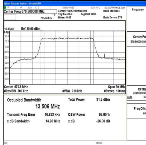
Band71-15MHz-QPSK-133197-75RB#0-PASS
