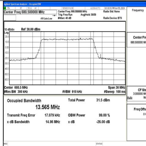
Band71-15MHz-QPSK-133297-75RB#0-PASS
