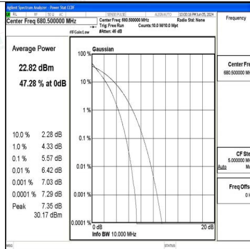
Band71-10MHz-QPSK-133297-50RB#0-PASS
