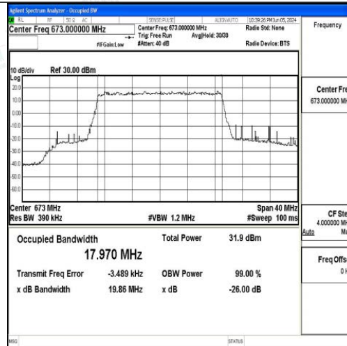
Band71-20MHz-QPSK-133222-100RB#0-PASS
