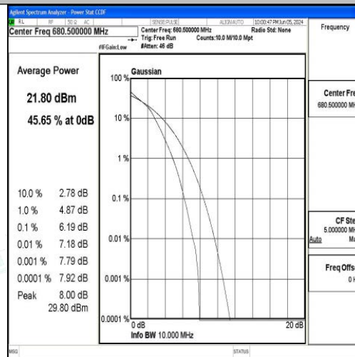
Band71-10MHz-16QAM-133297-50RB#0-PASS
