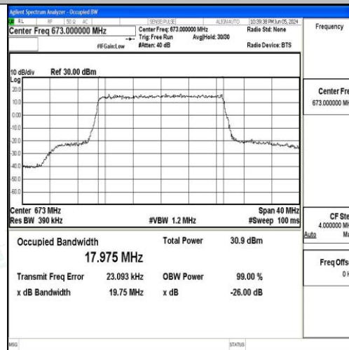
Band71-20MHz-16QAM-133222-100RB#0-PASS
