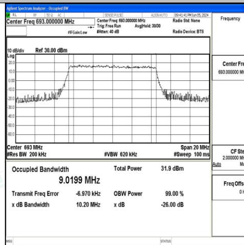
Band71-10MHz-QPSK-133422-50RB#0-PASS
