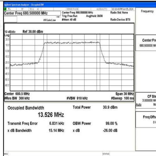
Band71-15MHz-16QAM-133297-75RB#0-PASS
