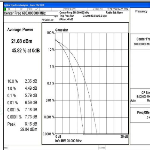
Band71-20MHz-QPSK-133372-100RB#0-PASS
