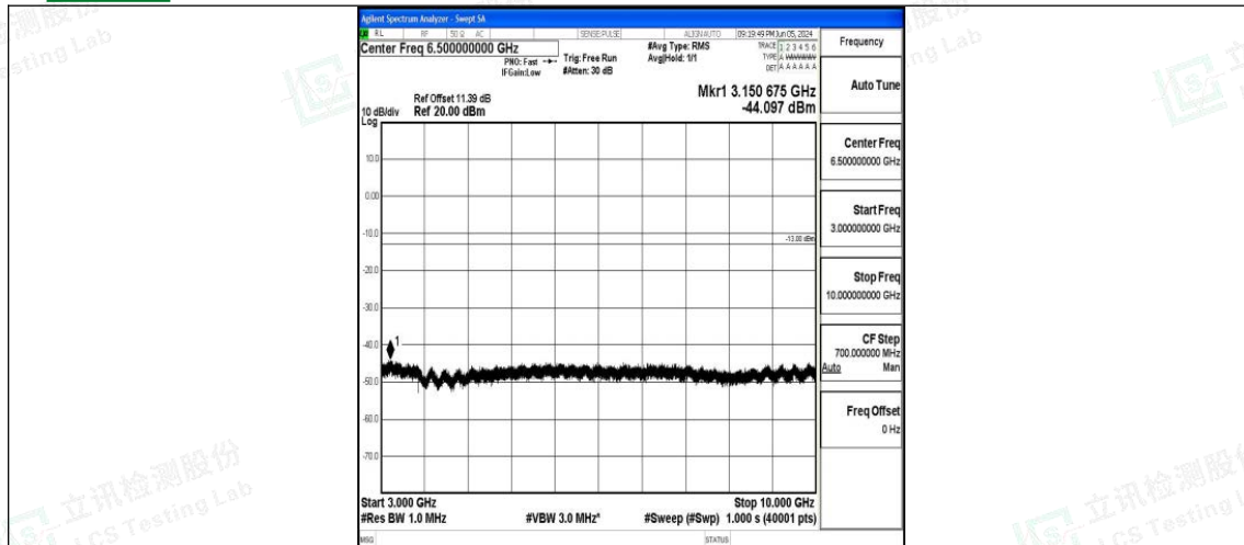
Band71_5MHz_16QAM_133447_1RB#0_3000~10000_3000~10000
