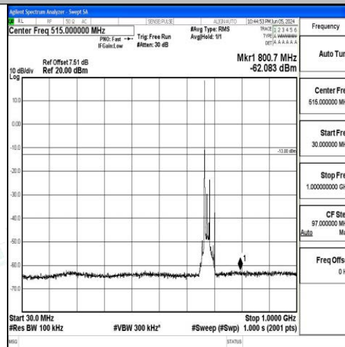
Band71_20MHz_QPSK_133322_1RB#0_30~1000_30~1000
