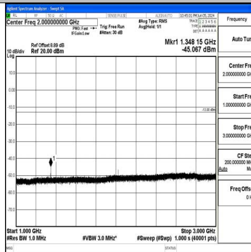
Band71_20MHz_QPSK_133322_1RB#0_1000~3000_1000~3000
