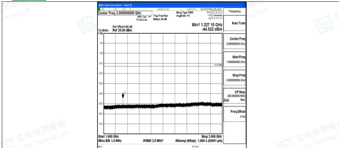
Band71_10MHz_16QAM_133172_1RB#0_1000~3000_1000~3000
