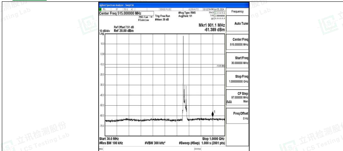
Band71_15MHz_QPSK_133197_1RB#0_30~1000_30~1000
