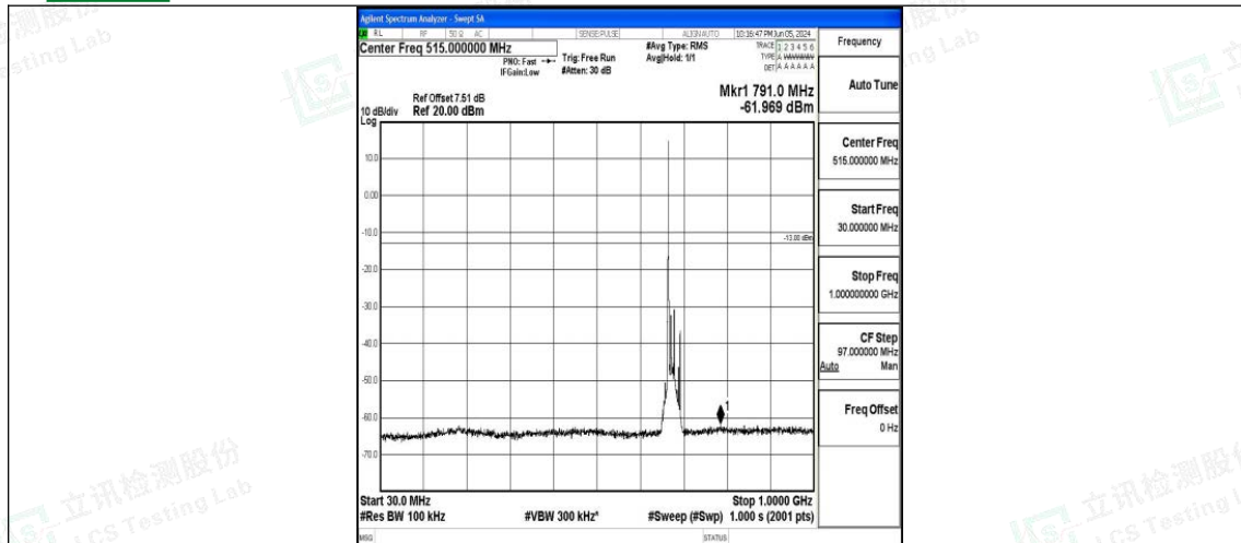
Band71_15MHz_16QAM_133297_1RB#0_30~1000_30~1000
