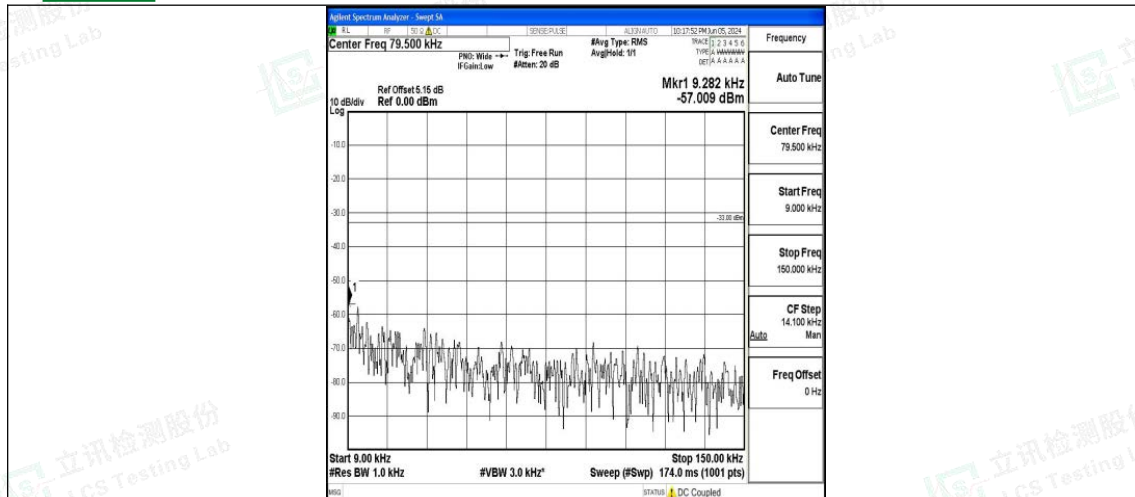
Band71_15MHz_QPSK_133397_1RB#0_0.009~0.15_0.009~0.15
