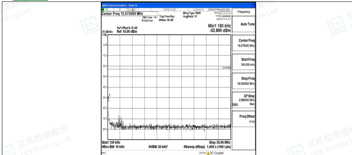
Band71_10MHz_16QAM_133422_1RB#0_0.15~30_0.15~30
