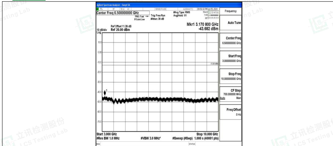
Band71_10MHz_16QAM_133422_1RB#0_3000~10000_3000~10000
