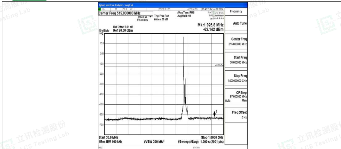
Band71_20MHz_16QAM_133322_1RB#0_30~1000_30~1000
