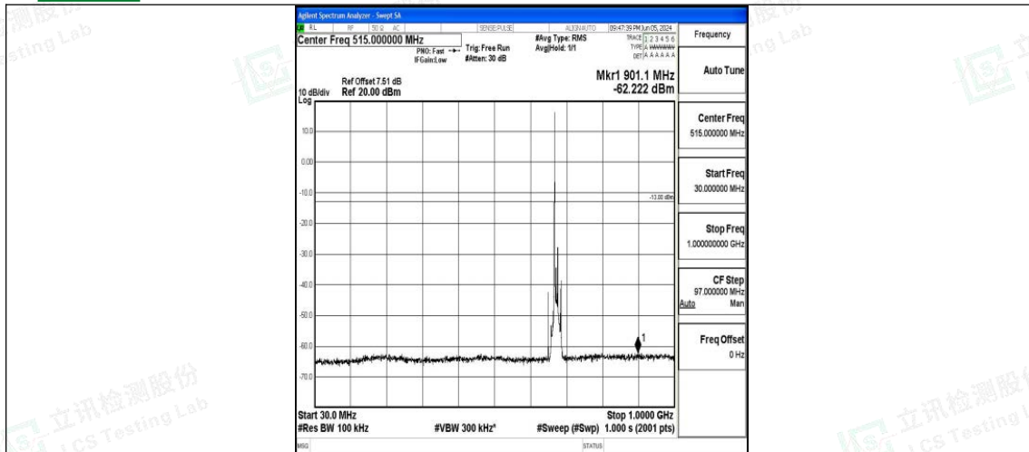
Band71_10MHz_16QAM_133297_1RB#0_30~1000_30~1000
