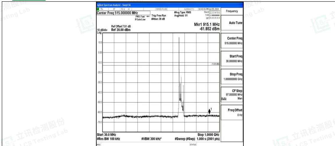
Band71_20MHz_16QAM_133222_1RB#0_30~1000_30~1000
