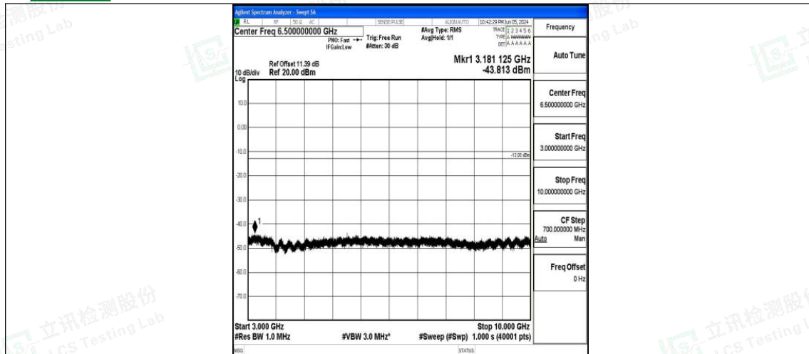
Band71_20MHz_QPSK_133222_1RB#0_3000~10000_3000~10000
