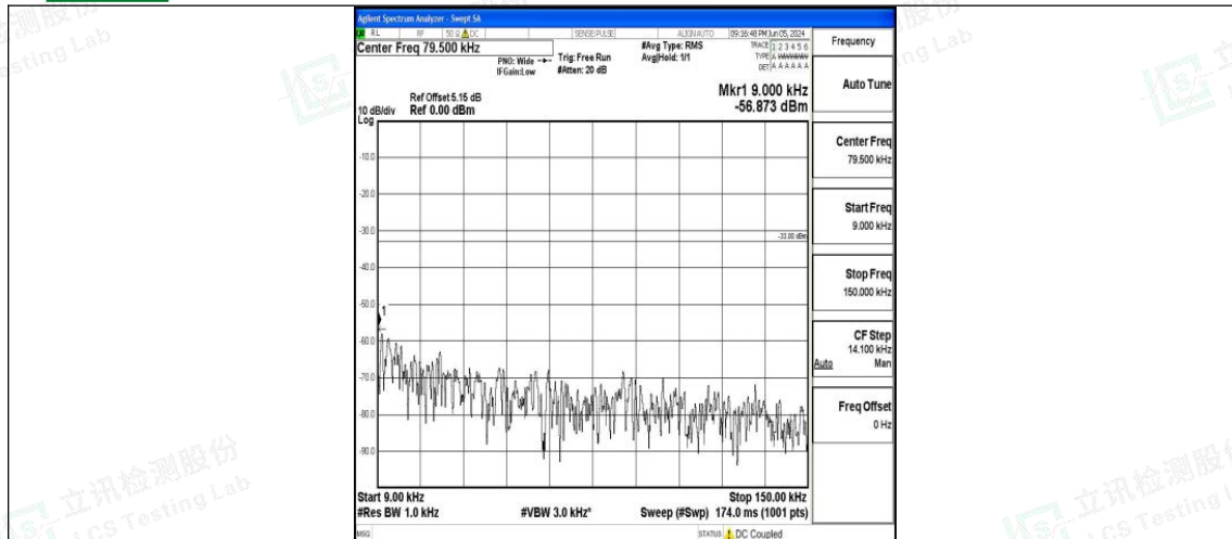
Band71_5MHz_16QAM_133297_1RB#0_0.009~0.15_0.009~0.15
