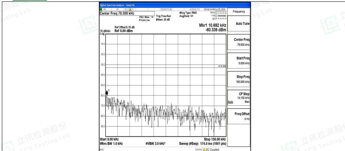
Band71_10MHz_QPSK_133422_1RB#0_0.009~0.15_0.009~0.15
