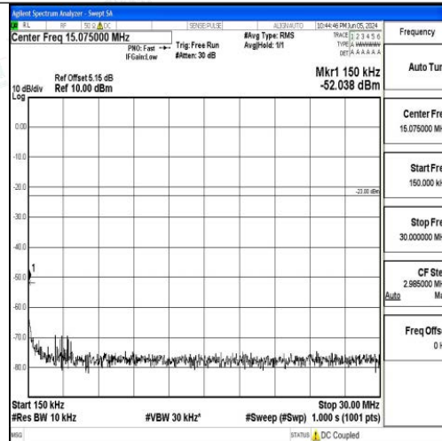
Band71_20MHz_QPSK_133322_1RB#0_0.15~30_0.15~30
