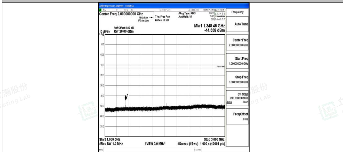
Band71_20MHz_16QAM_133322_1RB#0_1000~3000_1000~3000
