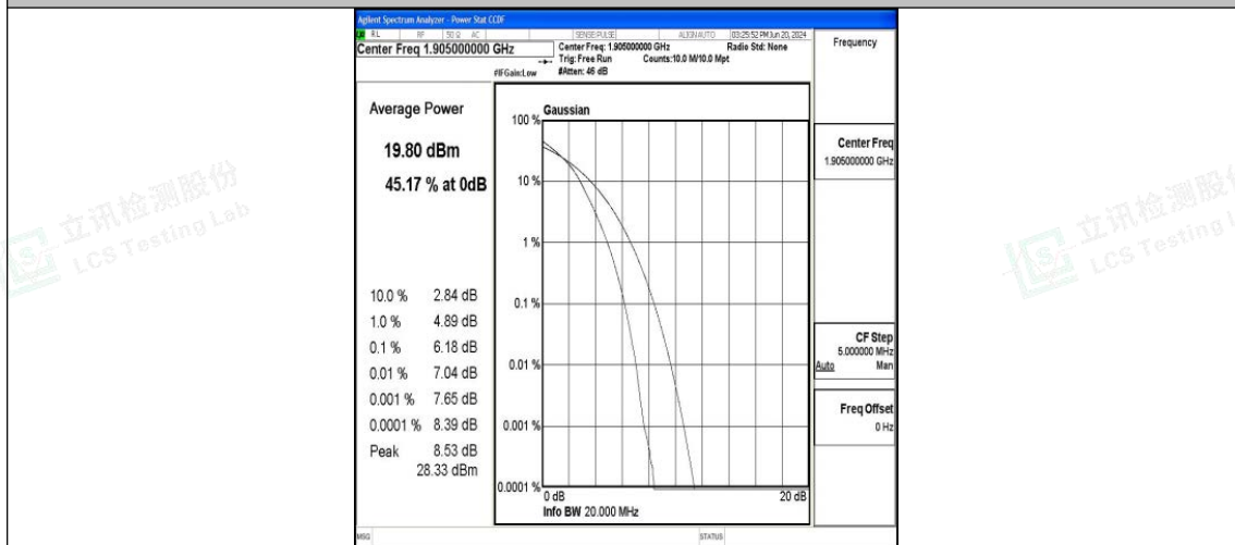
Band25-20MHz-16QAM-26590-100RB#0-PASS
