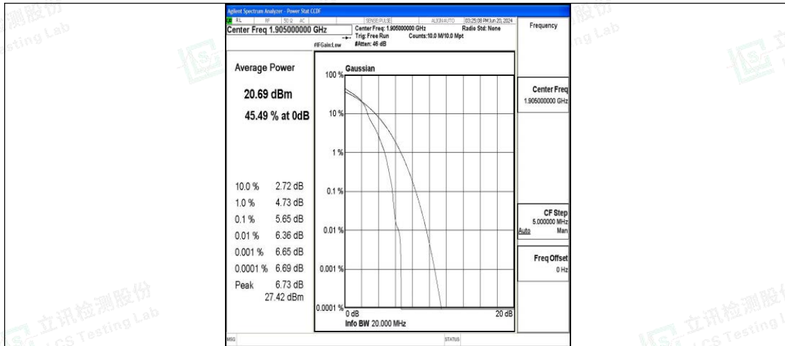
Band25-20MHz-16QAM-26590-1RB#0-PASS
