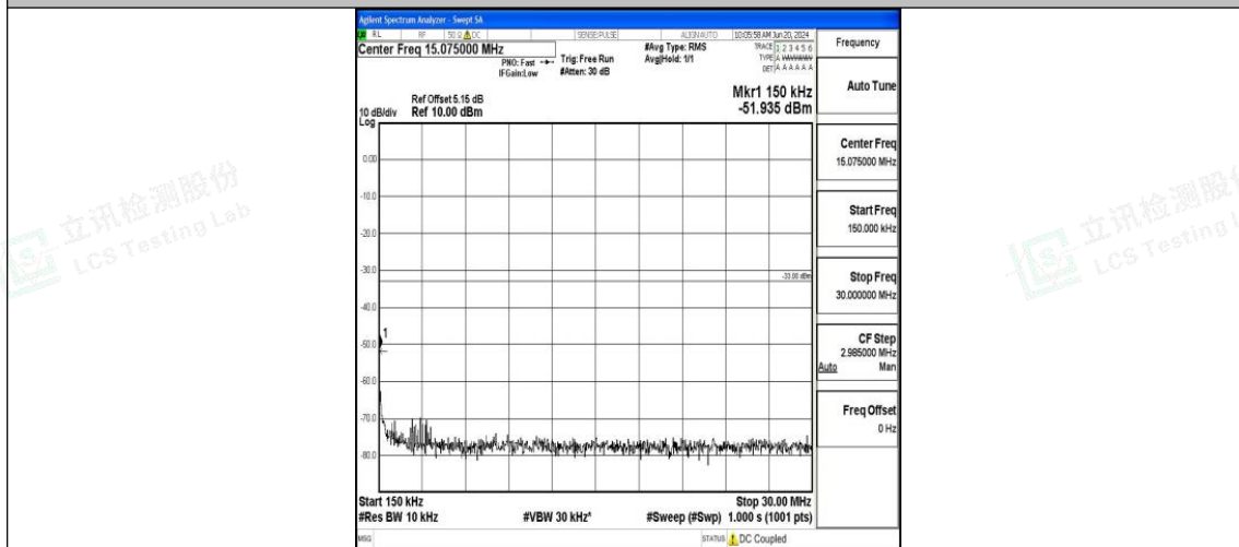
Band25_1.4MHz_16QAM_26047_1RB#0_0.15~30_0.15~30
