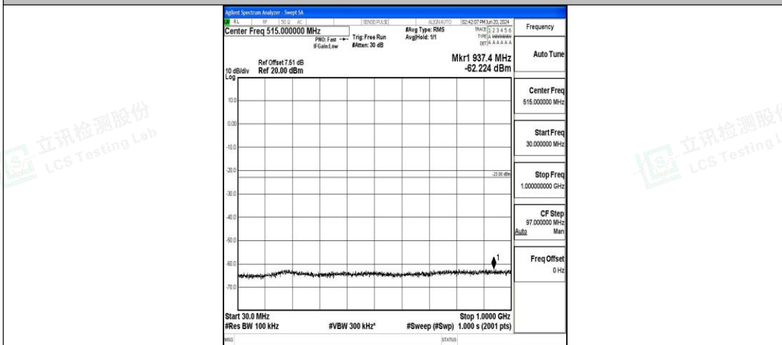
Band25_10MHz_16QAM_26640_1RB#0_30~1000_30~1000
