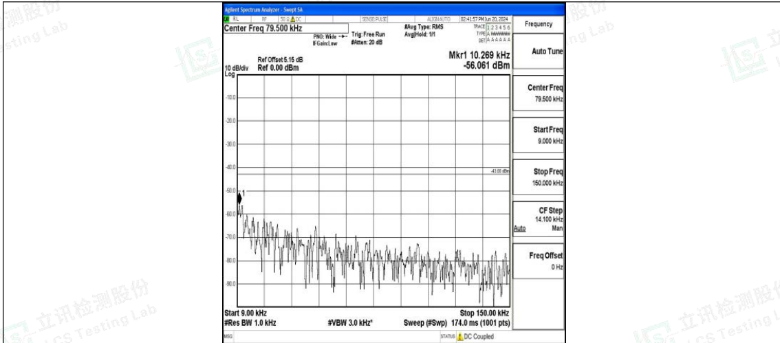
Band25_10MHz_16QAM_26640_1RB#0_0.009~0.15_0.009~0.15
