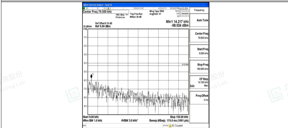
Band25_20MHz_16QAM_26140_1RB#0_0.009~0.15_0.009~0.15
