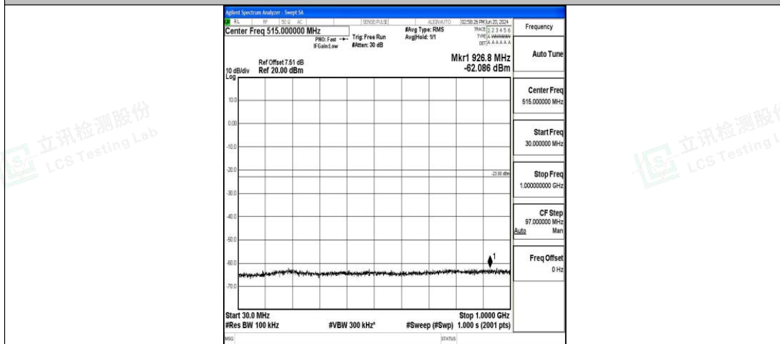
Band25_15MHz_QPSK_26365_1RB#0_30~1000_30~1000
