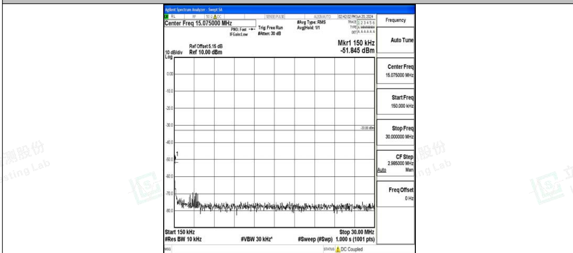
Band25_10MHz_16QAM_26640_1RB#0_0.15~30_0.15~30
