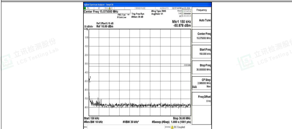
Band25_15MHz_16QAM_26115_1RB#0_0.15~30_0.15~30
