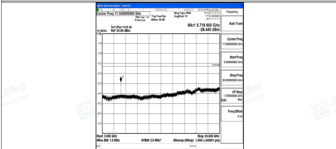
Band25_10MHz_16QAM_26640_1RB#0_3000~20000_3000~20000
