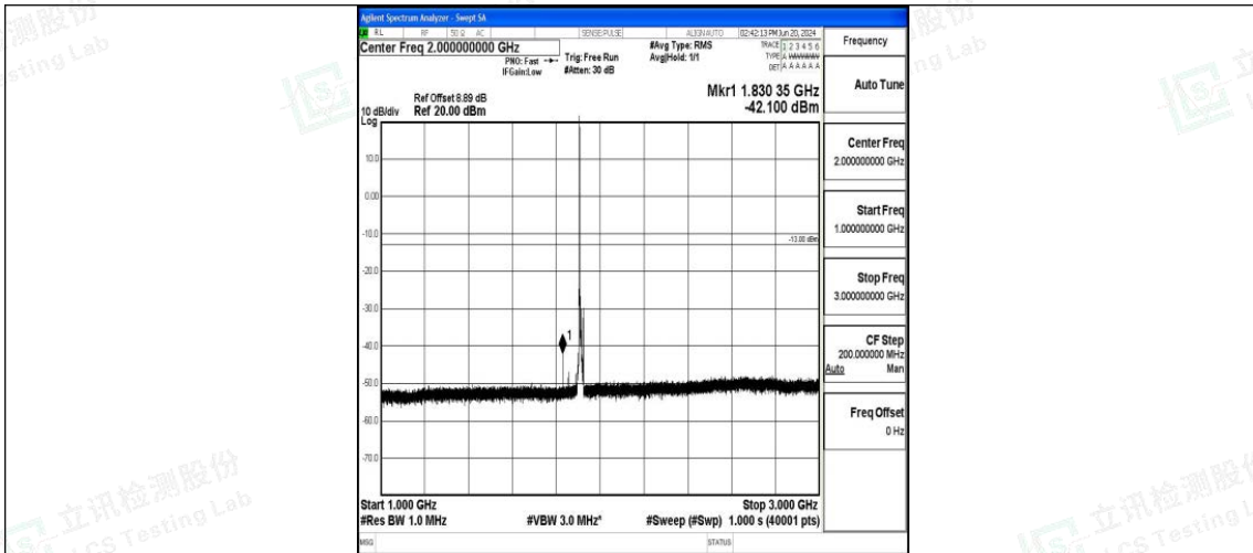
Band25_10MHz_16QAM_26640_1RB#0_1000~3000_1000~3000
