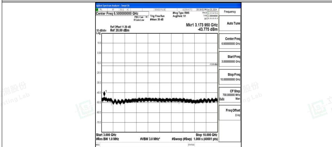
Band26_5MHz_QPSK_26815_1RB#0_3000~10000_3000~10000
