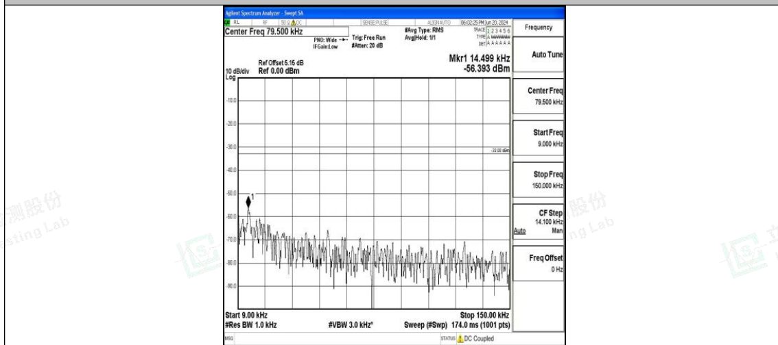
Band26_10MHz_16QAM_26990_1RB#0_0.009~0.15_0.009~0.15
