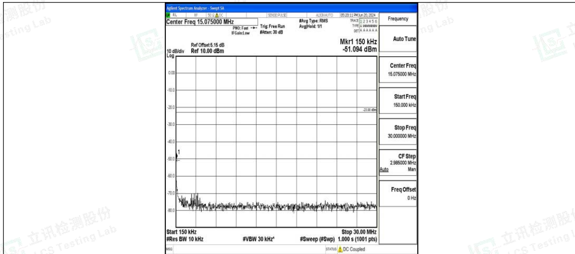
Band26_3MHz_QPSK_27025_1RB#0_0.15~30_0.15~30
