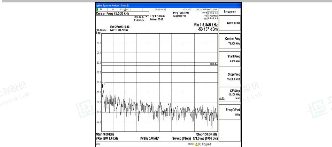
Band26_15MHz_16QAM_26965_1RB#0_0.009~0.15_0.009~0.15
