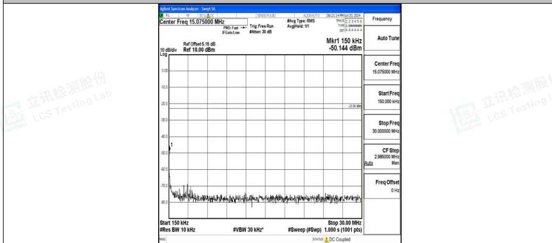
Band26_15MHz_16QAM_26965_1RB#0_0.15~30_0.15~30
