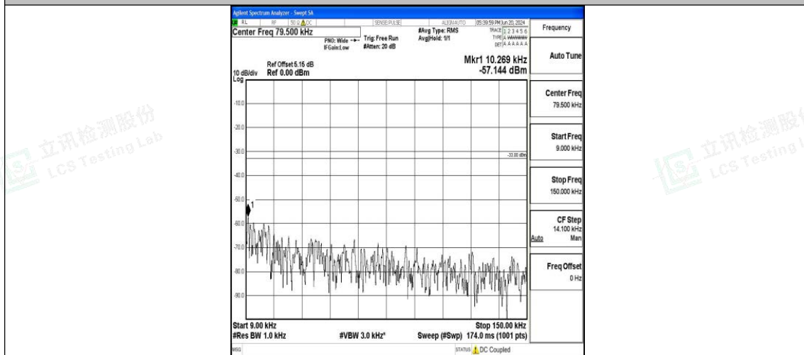
Band26_5MHz_16QAM_26815_1RB#0_0.009~0.15_0.009~0.15
