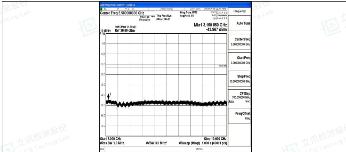
Band26_3MHz_QPSK_27025_1RB#0_3000~10000_3000~10000
