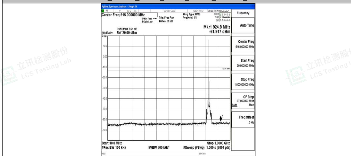
Band26_15MHz_QPSK_26865_1RB#0_30~1000_30~1000
