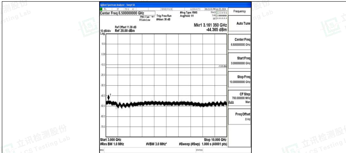
Band26_15MHz_QPSK_26965_1RB#0_3000~10000_3000~10000
