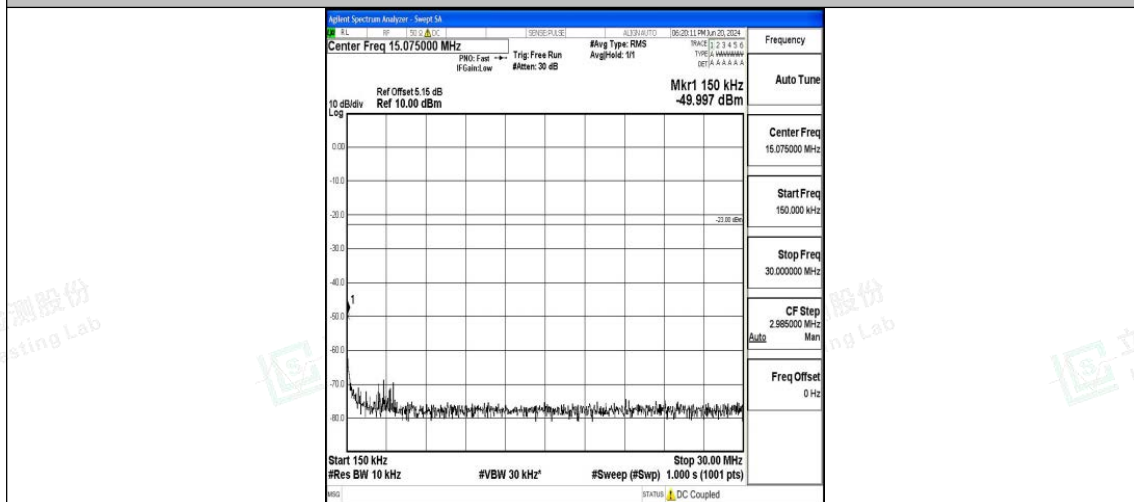
Band26_15MHz_16QAM_26915_1RB#0_0.15~30_0.15~30
