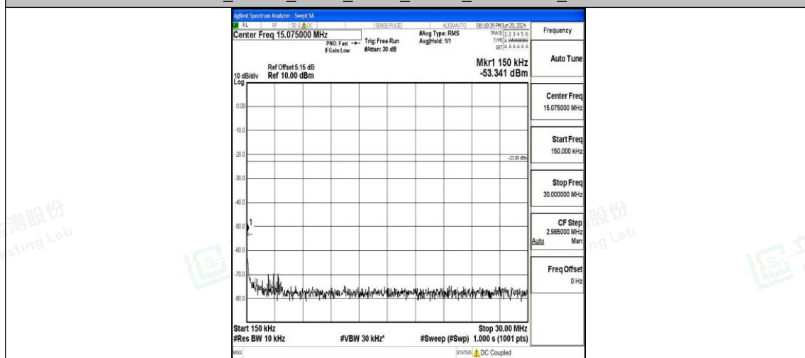
Band26_15MHz_QPSK_26865_1RB#0_0.15~30_0.15~30
