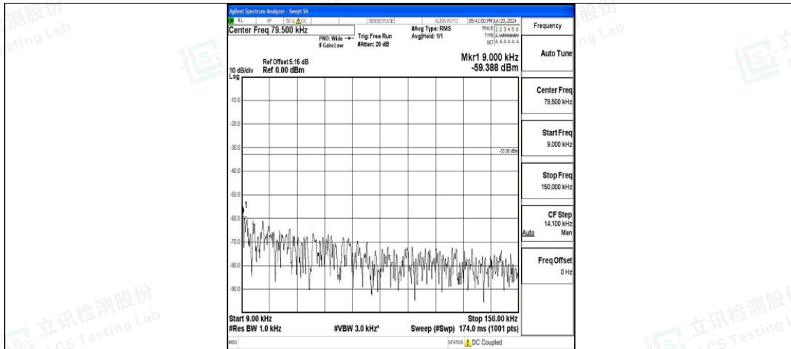
Band26_5MHz_16QAM_26915_1RB#0_0.009~0.15_0.009~0.15
