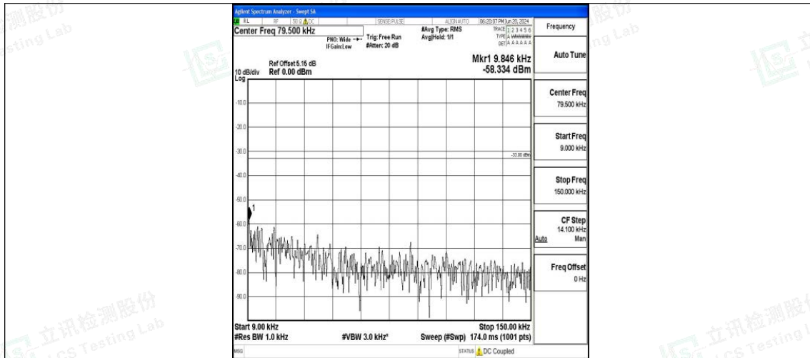
Band26_15MHz_16QAM_26915_1RB#0_0.009~0.15_0.009~0.15
