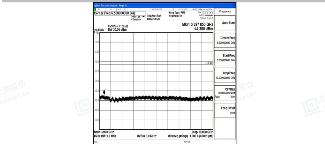
Band26_15MHz_16QAM_26915_1RB#0_3000~10000_3000~10000
