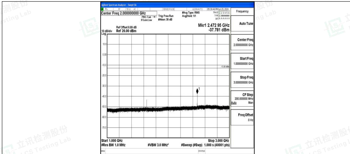
Band26_5MHz_QPSK_26815_1RB#0_1000~3000_1000~3000
