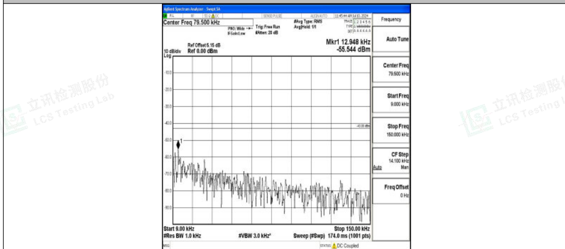
Band2_5MHz_16QAM_18900_1RB#0_0.009~0.15_0.009~0.15
