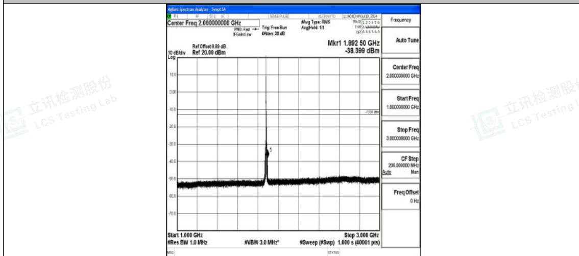
Band2_5MHz_16QAM_18900_1RB#0_1000~3000_1000~3000
