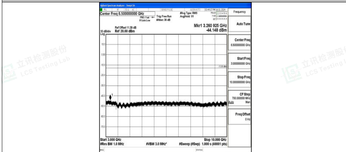
Band5_5MHz_16QAM_20525_1RB#0_3000~10000_3000~10000
