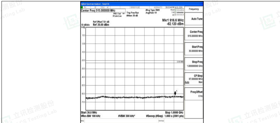
Band25_3MHz_16QAM_26055_1RB#0_30~1000_30~1000
