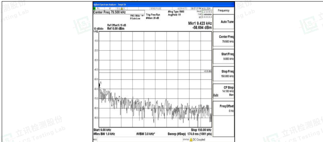
Band25_5MHz_QPSK_26365_1RB#0_0.009~0.15_0.009~0.15
