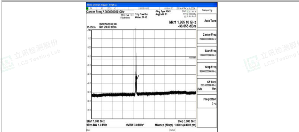
Band25_5MHz_QPSK_26065_1RB#0_1000~3000_1000~3000
