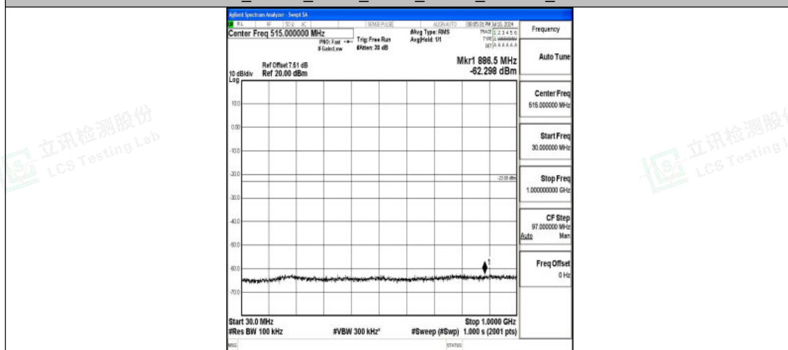
Band25_20MHz_QPSK_26365_1RB#0_30~1000_30~1000
