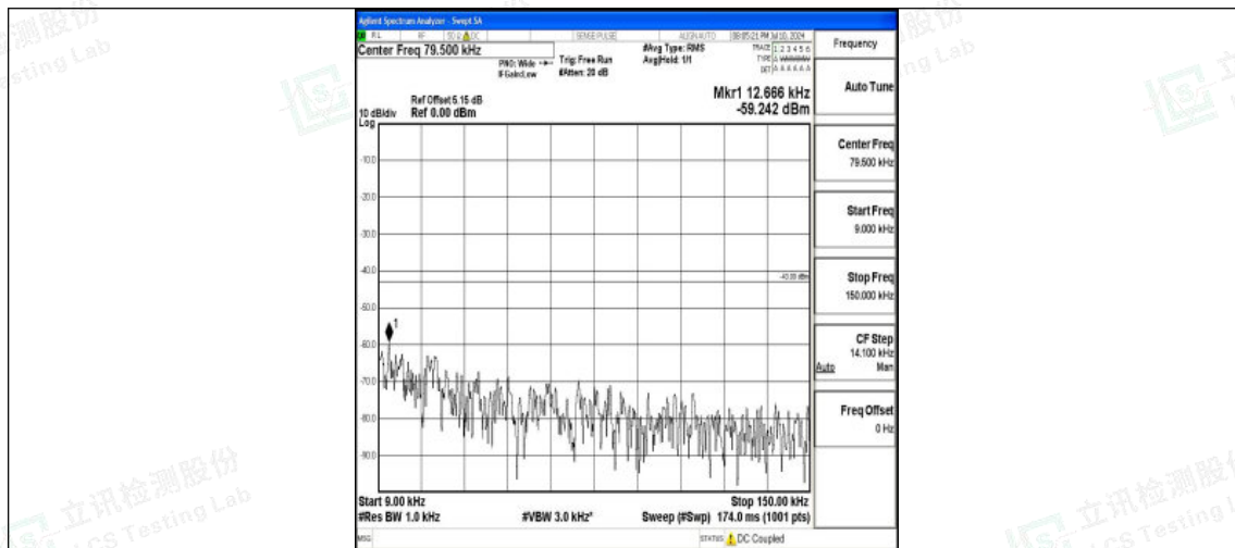
Band25_20MHz_QPSK_26365_1RB#0_0.009~0.15_0.009~0.15
