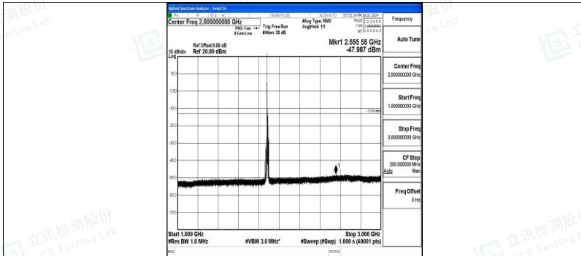
Band25_10MHz_QPSK_26365_1RB#0_1000~3000_1000~3000
