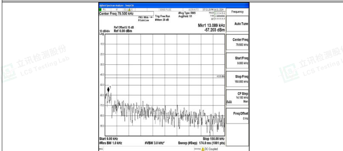
Band25_10MHz_16QAM_26365_1RB#0_0.009~0.15_0.009~0.15
