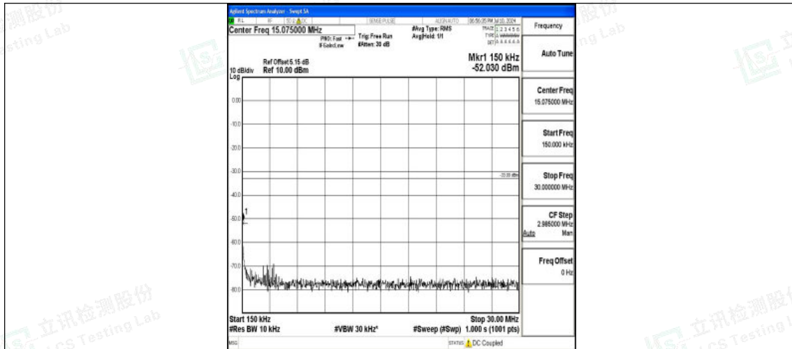
Band25_5MHz_QPSK_26065_1RB#0_0.15~30_0.15~30
