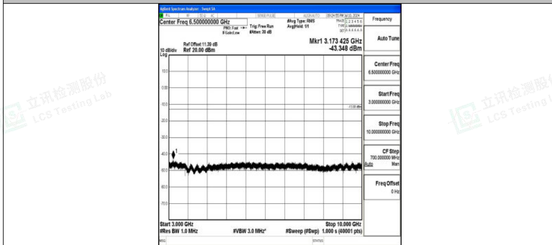
Band26_5MHz_QPSK_26765_1RB#0_3000~10000_3000~10000
