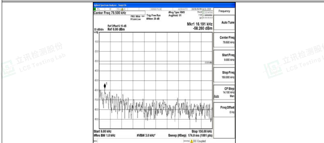
Band26_3MHz_QPSK_26705_1RB#0_0.009~0.15_0.009~0.15
