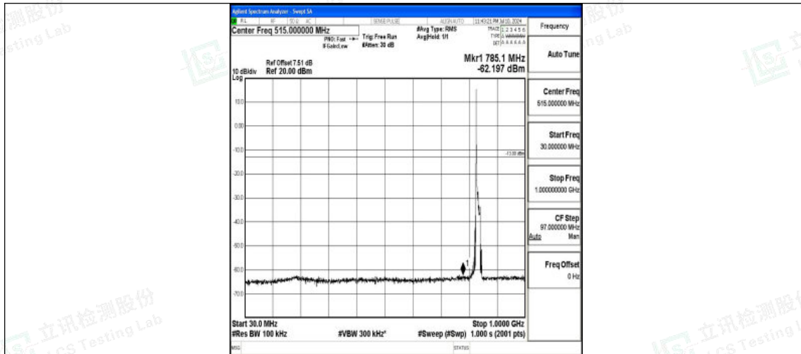
Band26_15MHz_QPSK_26915_1RB#0_30~1000_30~1000
