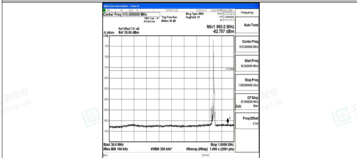
Band26_10MHz_QPSK_26990_1RB#0_30~1000_30~1000
