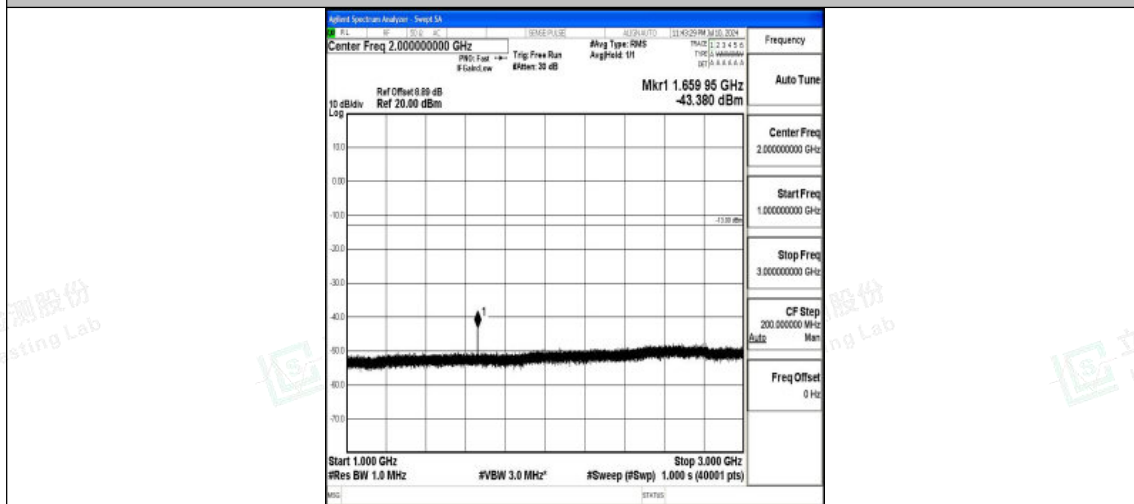
Band26_15MHz_QPSK_26915_1RB#0_1000~3000_1000~3000
