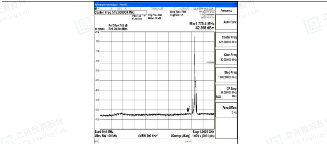
Band26_10MHz_QPSK_26915_1RB#0_30~1000_30~1000
