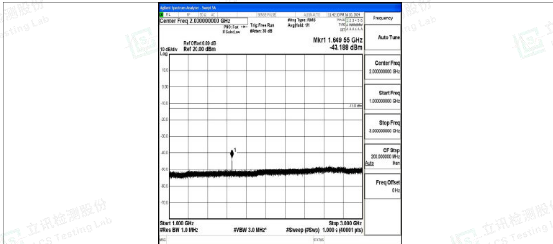
Band26_15MHz_QPSK_26865_1RB#0_1000~3000_1000~3000
