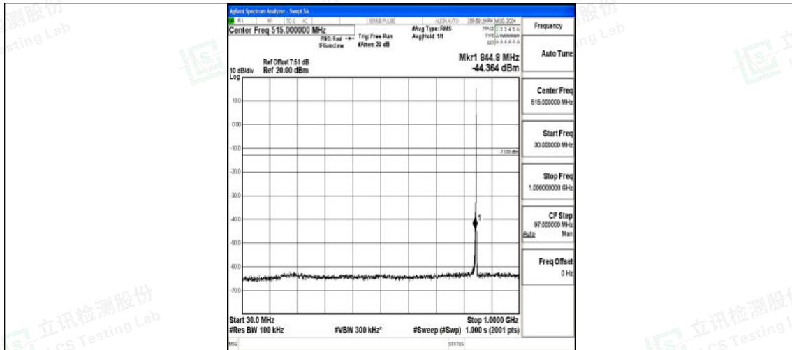
Band26_1.4MHz_16QAM_27033_1RB#0_30~1000_30~1000
