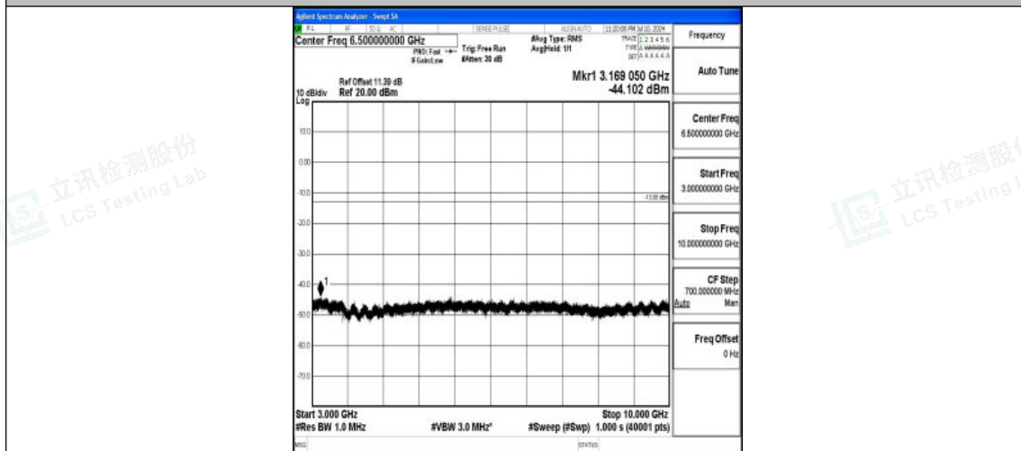
Band26_10MHz_QPSK_26915_1RB#0_3000~10000_3000~10000
