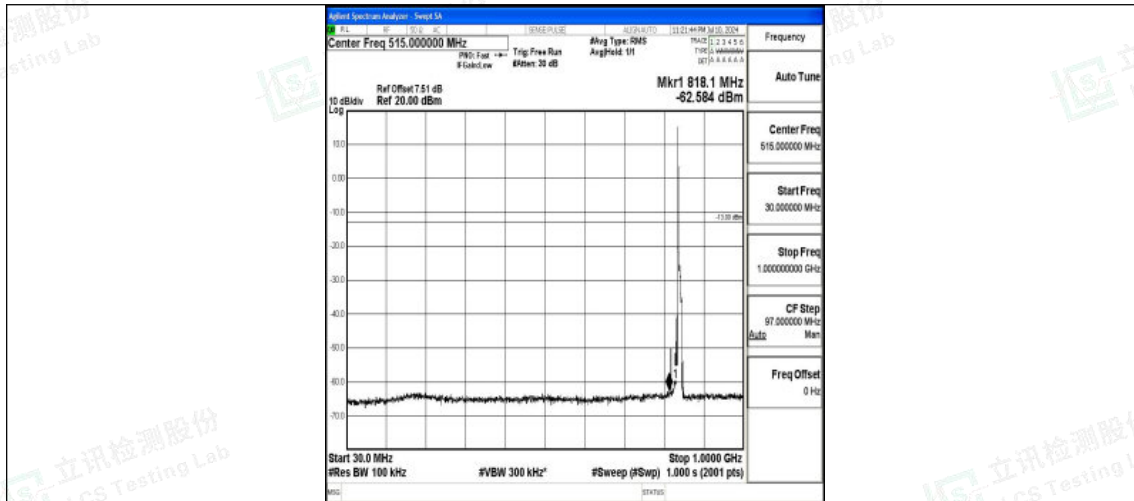
Band26_10MHz_16QAM_26990_1RB#0_30~1000_30~1000
