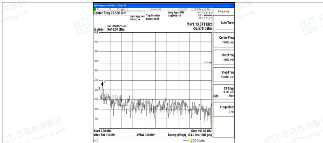
Band26_10MHz_QPSK_26840_1RB#0_0.009~0.15_0.009~0.15
