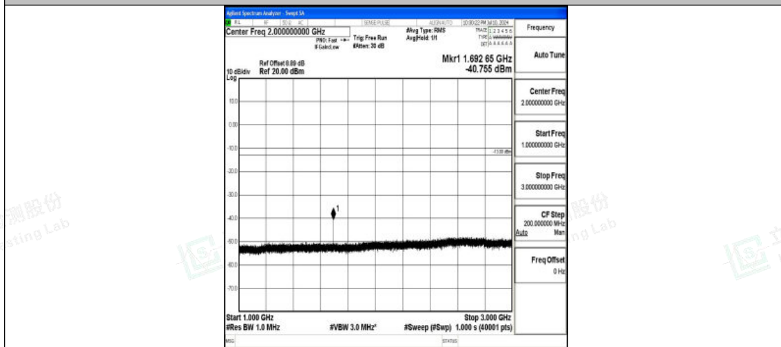
Band26_3MHz_16QAM_27025_1RB#0_1000~3000_1000~3000
