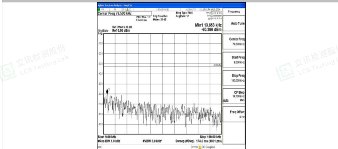
Band26_10MHz_16QAM_26840_1RB#0_0.009~0.15_0.009~0.15
