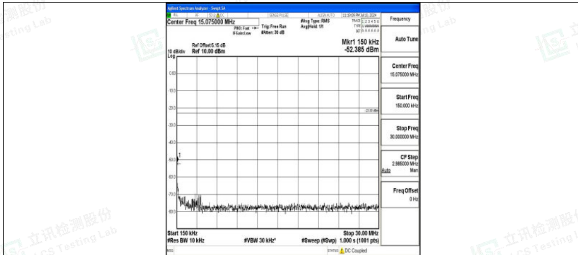
Band26_10MHz_16QAM_26840_1RB#0_0.15~30_0.15~30
