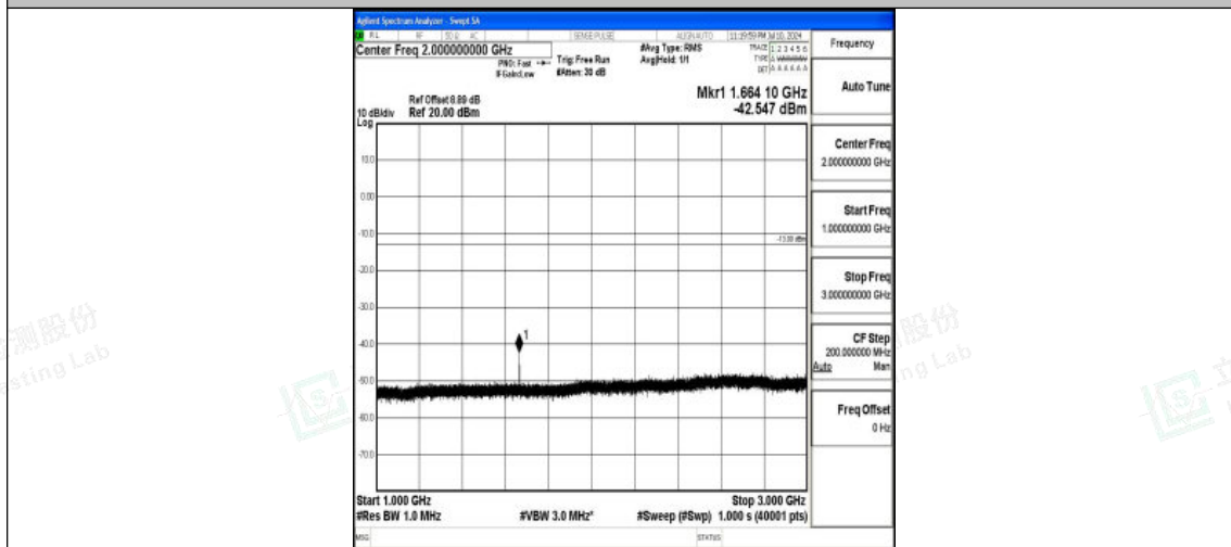
Band26_10MHz_QPSK_26915_1RB#0_1000~3000_1000~3000
