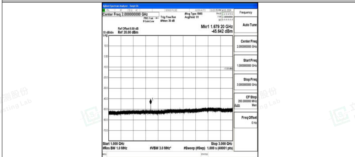
Band26_10MHz_16QAM_26990_1RB#0_1000~3000_1000~3000
