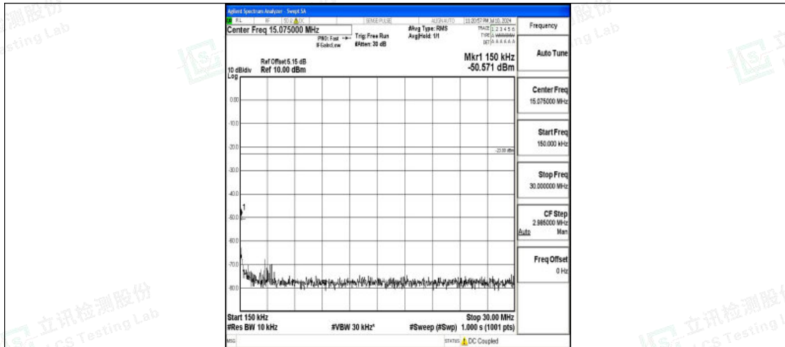
Band26_10MHz_QPSK_26990_1RB#0_0.15~30_0.15~30
