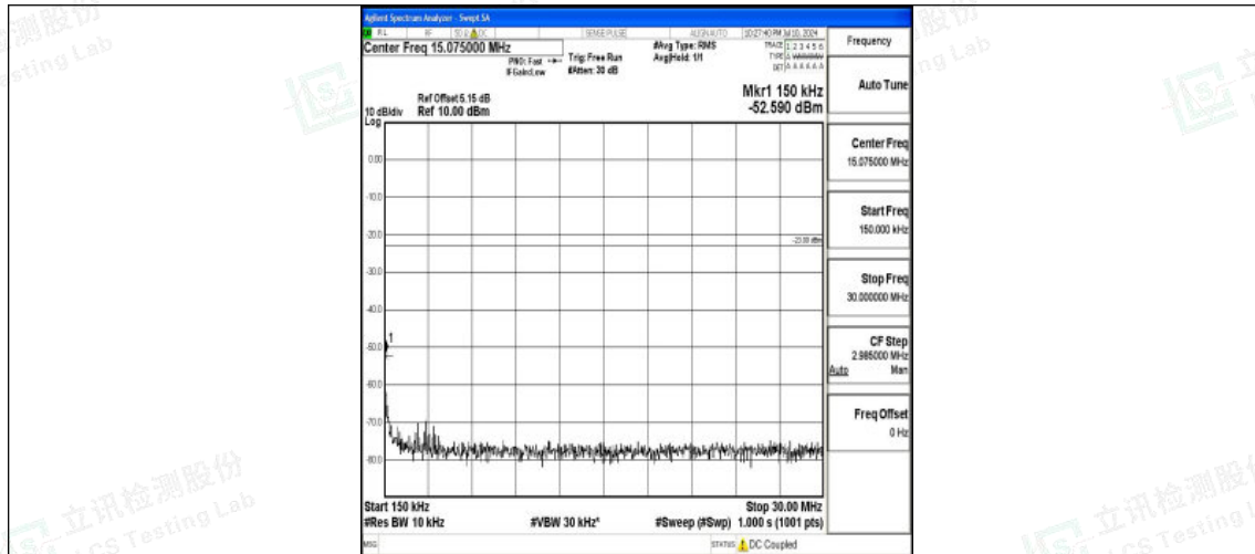
Band26_3MHz_16QAM_26805_1RB#0_0.15~30_0.15~30
