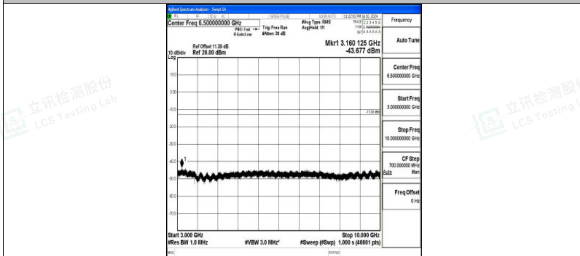
Band26_10MHz_16QAM_26990_1RB#0_3000~10000_3000~10000
