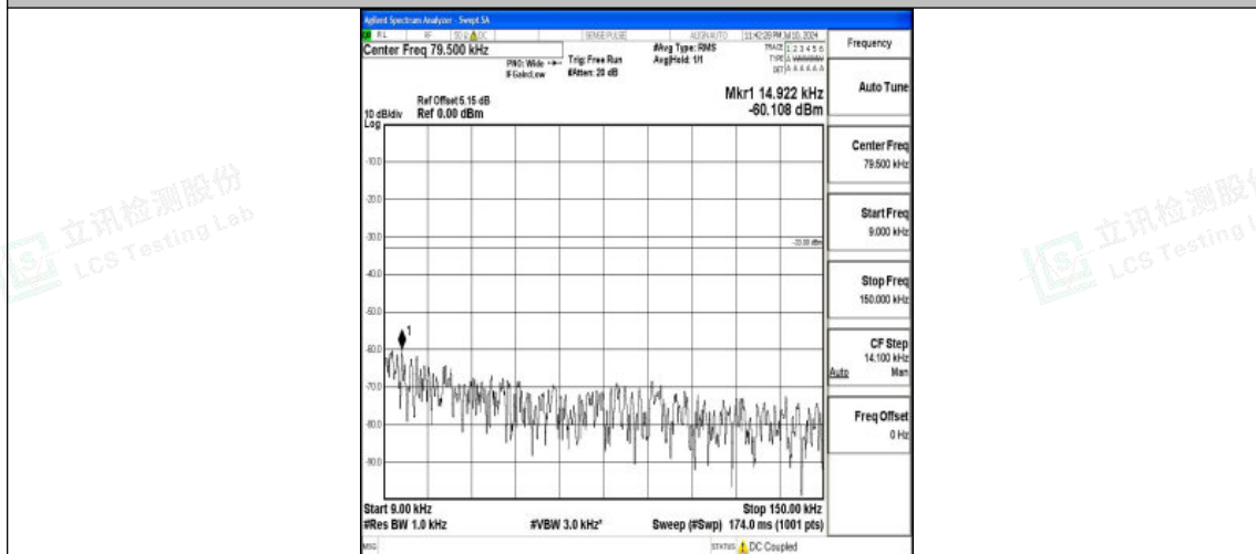
Band26_15MHz_16QAM_26865_1RB#0_0.009~0.15_0.009~0.15
