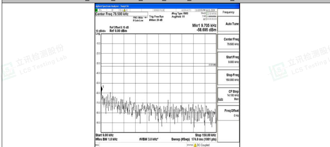
Band26_10MHz_QPSK_26990_1RB#0_0.009~0.15_0.009~0.15
