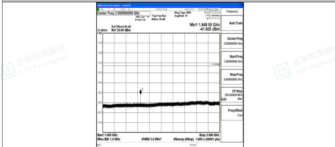
Band26_3MHz_16QAM_26805_1RB#0_1000~3000_1000~3000
