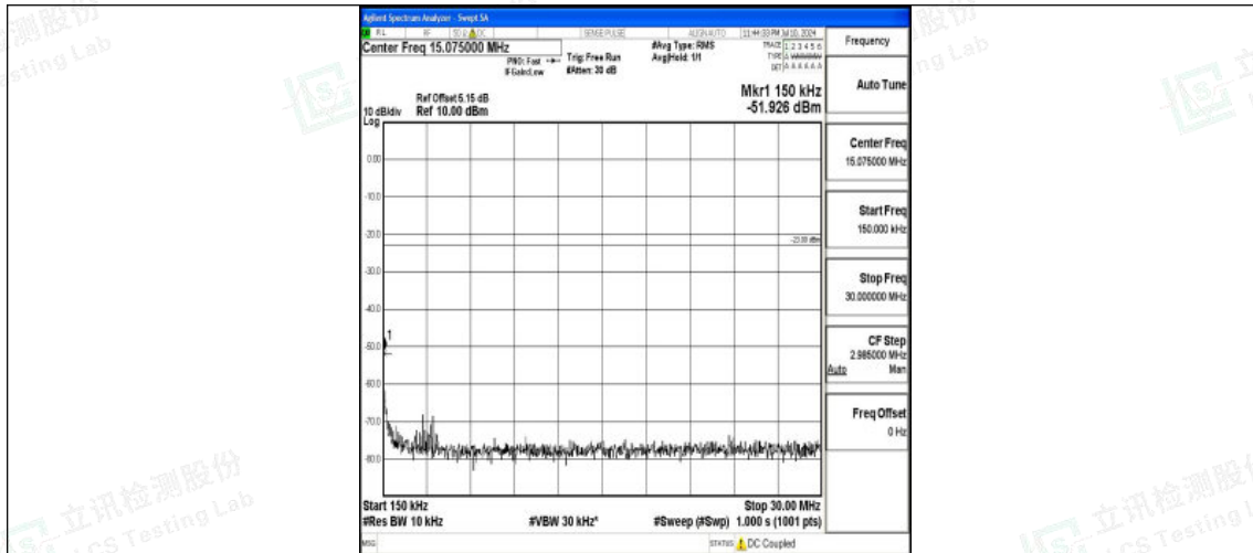
Band26_15MHz_QPSK_26965_1RB#0_0.15~30_0.15~30
