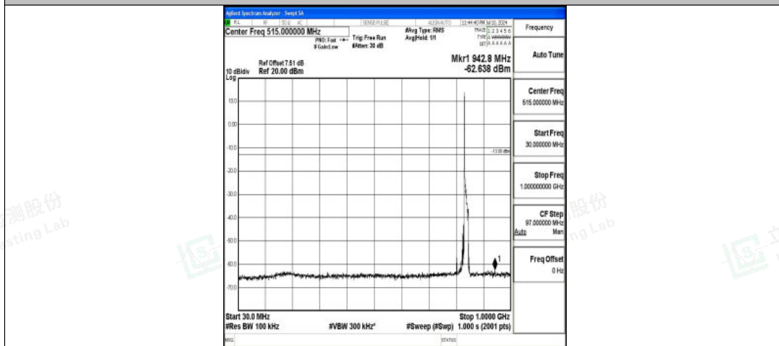
Band26_15MHz_QPSK_26965_1RB#0_30~1000_30~1000
