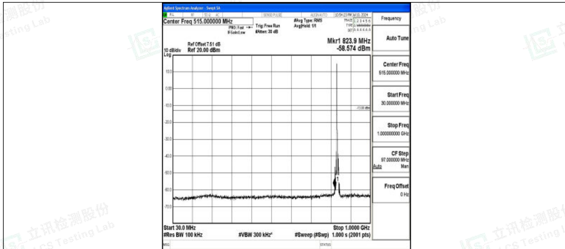
Band26_5MHz_QPSK_26915_1RB#0_30~1000_30~1000
