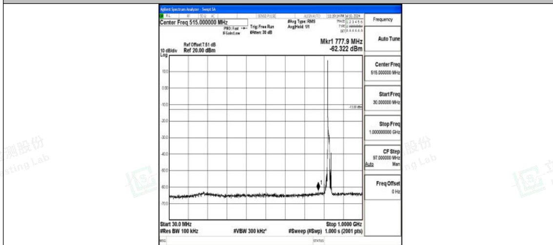
Band26_10MHz_16QAM_26840_1RB#0_30~1000_30~1000
