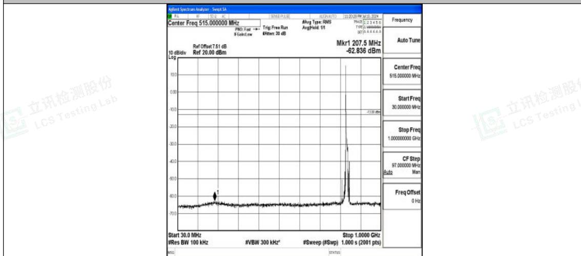
Band26_10MHz_16QAM_26915_1RB#0_30~1000_30~1000
