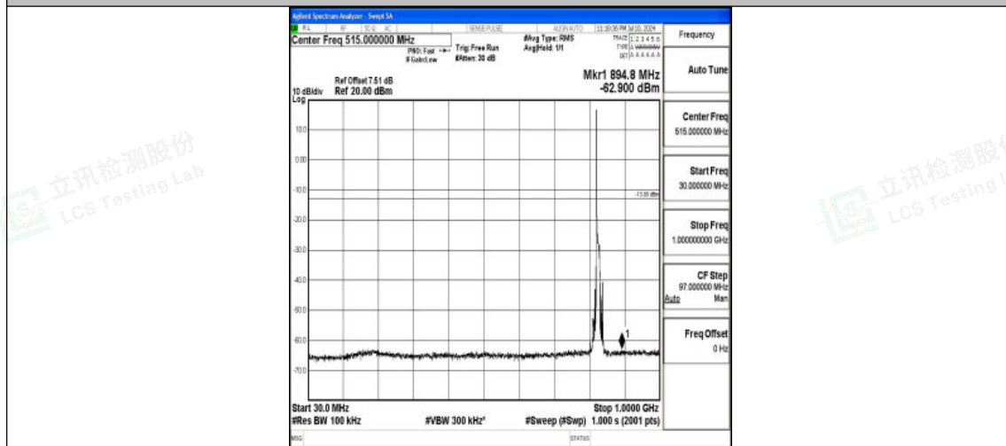
Band26_10MHz_QPSK_26840_1RB#0_30~1000_30~1000
