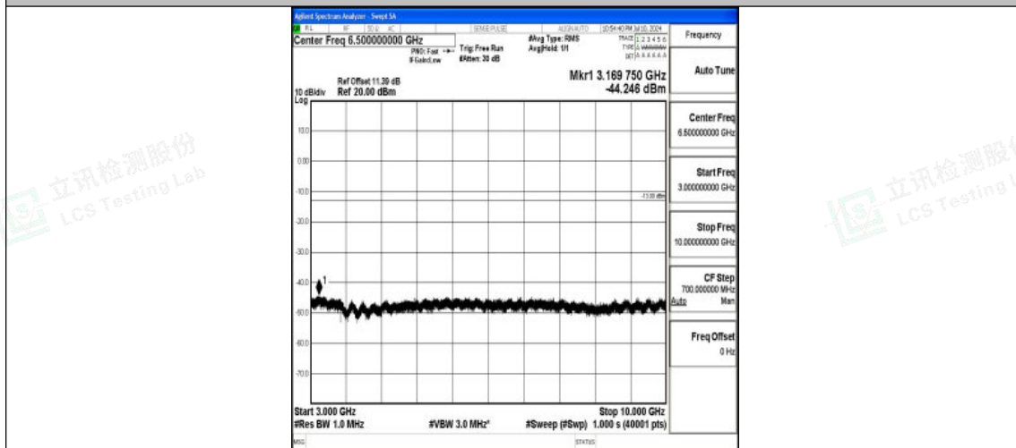
Band26_5MHz_QPSK_26915_1RB#0_3000~10000_3000~10000
