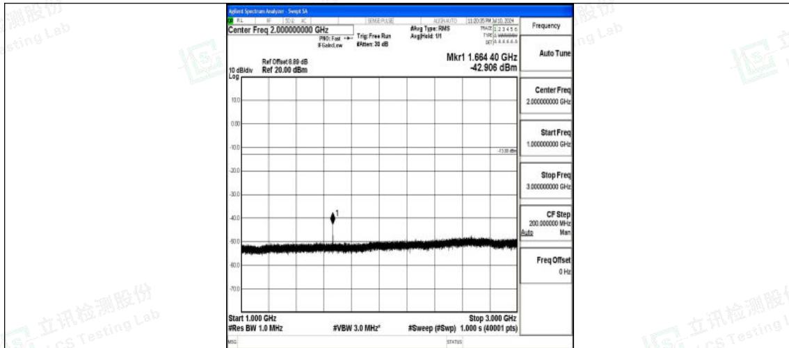
Band26_10MHz_16QAM_26915_1RB#0_1000~3000_1000~3000
