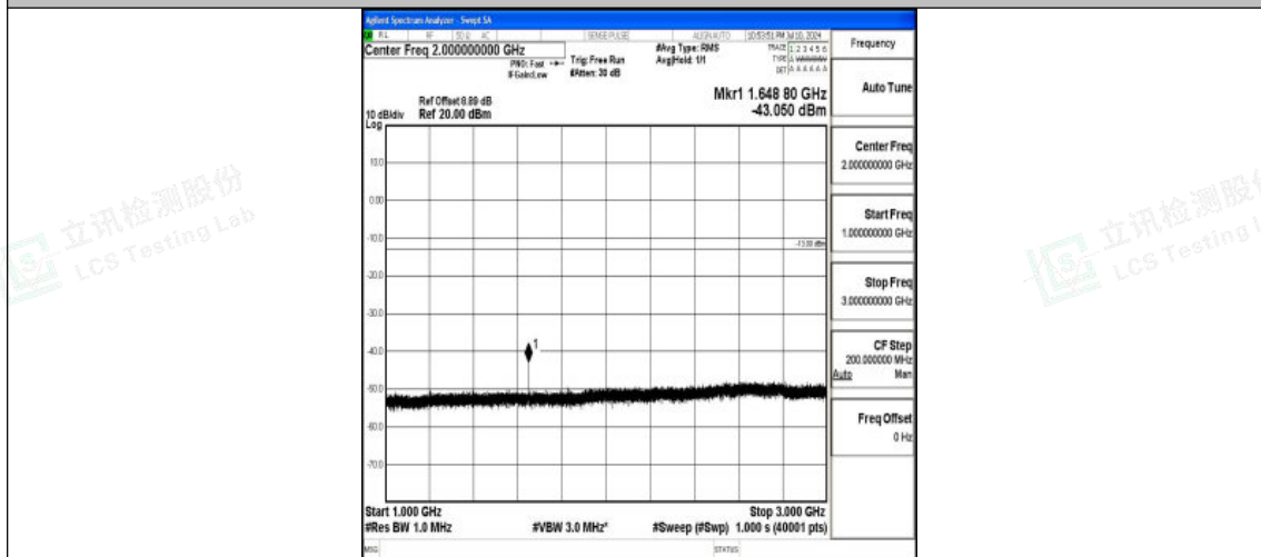
Band26_5MHz_16QAM_26815_1RB#0_1000~3000_1000~3000
