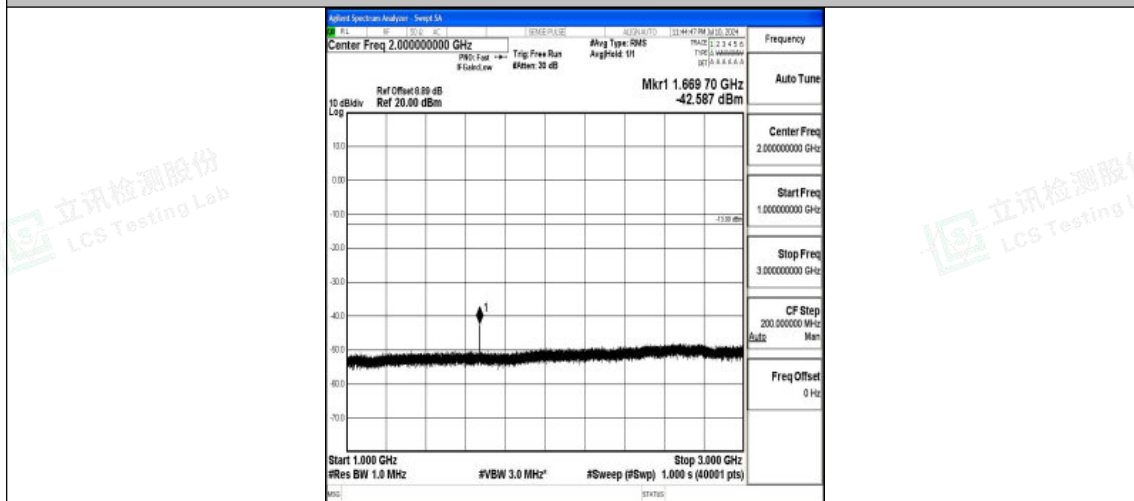
Band26_15MHz_QPSK_26965_1RB#0_1000~3000_1000~3000
