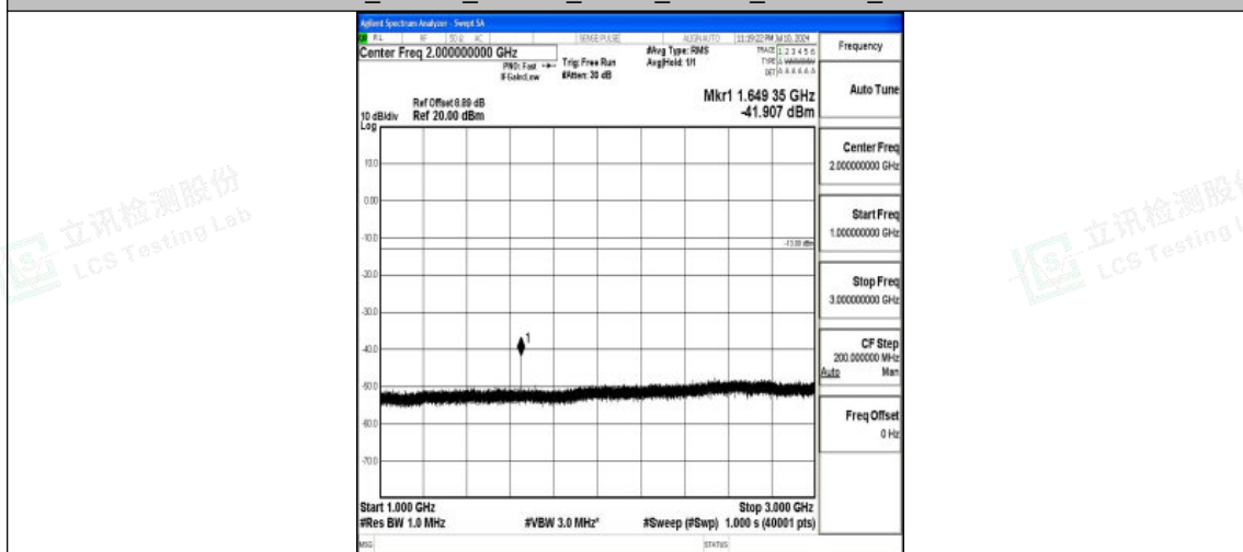
Band26_10MHz_16QAM_26840_1RB#0_1000~3000_1000~3000
