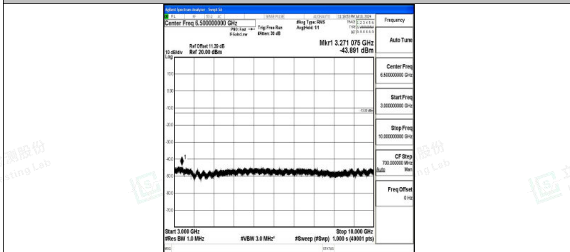
Band26_10MHz_QPSK_26840_1RB#0_3000~10000_3000~10000
