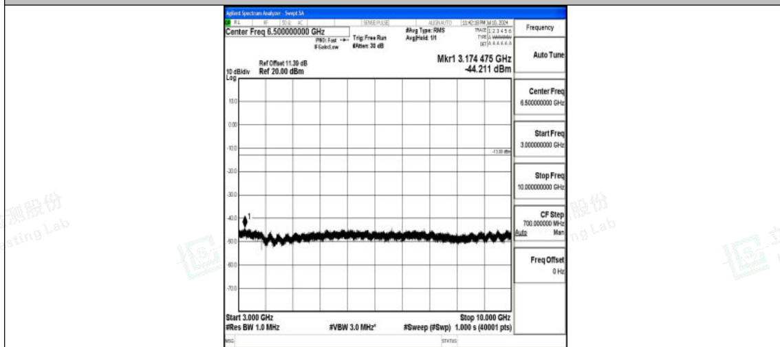
Band26_15MHz_QPSK_26865_1RB#0_3000~10000_3000~10000
