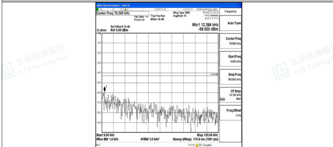
Band66_10MHz_16QAM_132322_1RB#0_0.009~0.15_0.009~0.15
