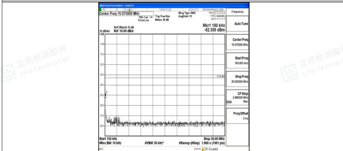
Band66_20MHz_QPSK_132572_1RB#0_0.15~30_0.15~30
