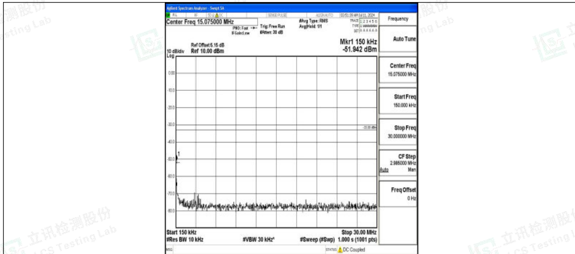
Band66_10MHz_QPSK_132022_1RB#0_0.15~30_0.15~30
