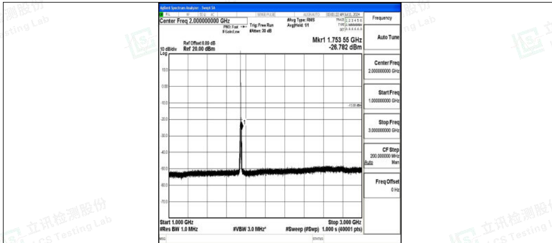
Band66_3MHz_QPSK_132322_1RB#0_1000~3000_1000~3000
