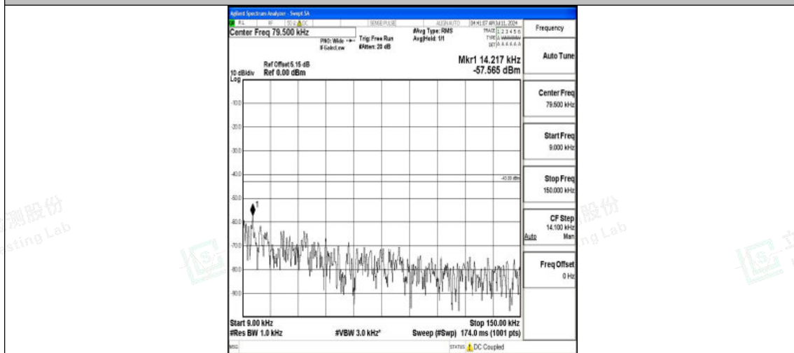
Band66_20MHz_16QAM_132072_1RB#0_0.009~0.15_0.009~0.15
