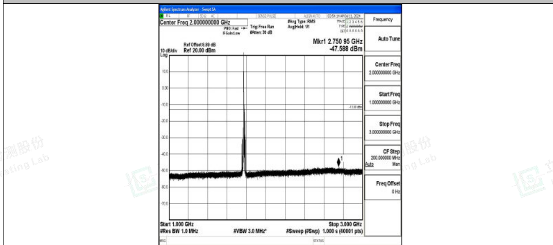
Band66_10MHz_QPSK_132622_1RB#0_1000~3000_1000~3000
