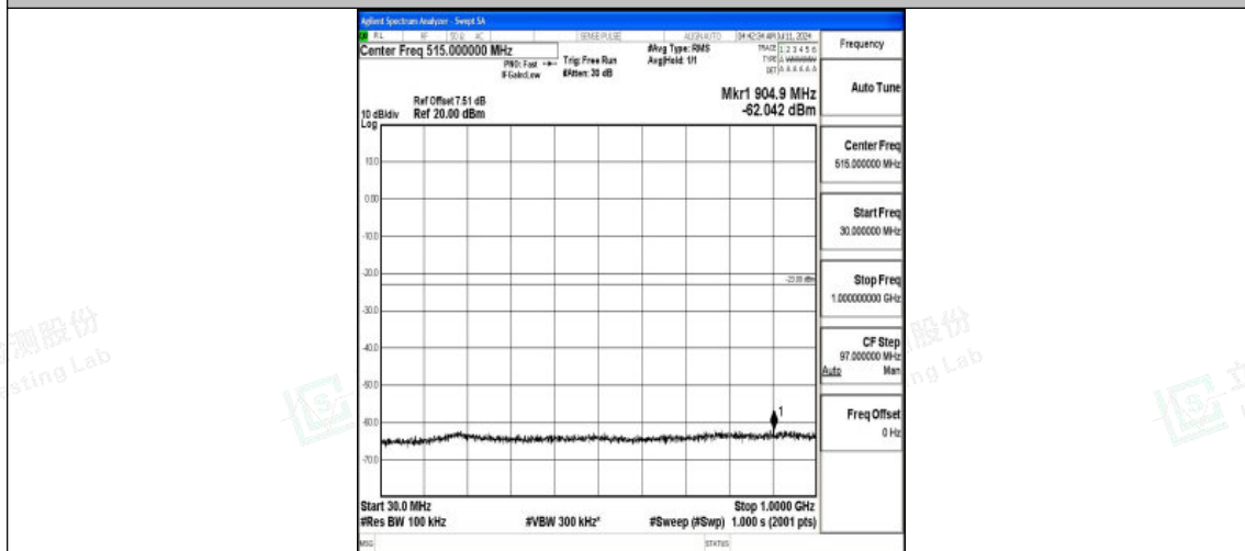
Band66_20MHz_16QAM_132322_1RB#0_30~1000_30~1000
