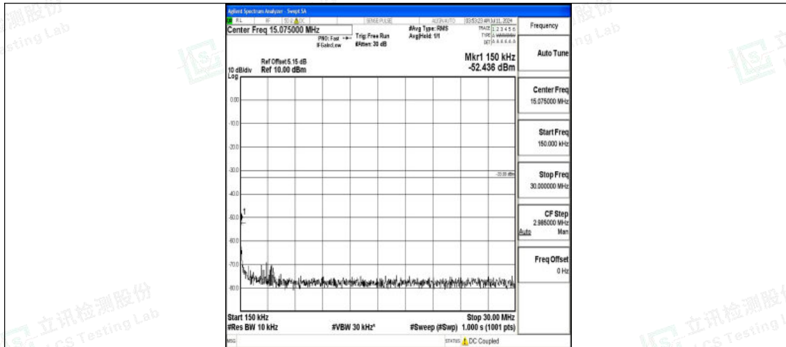
Band66_10MHz_16QAM_132322_1RB#0_0.15~30_0.15~30
