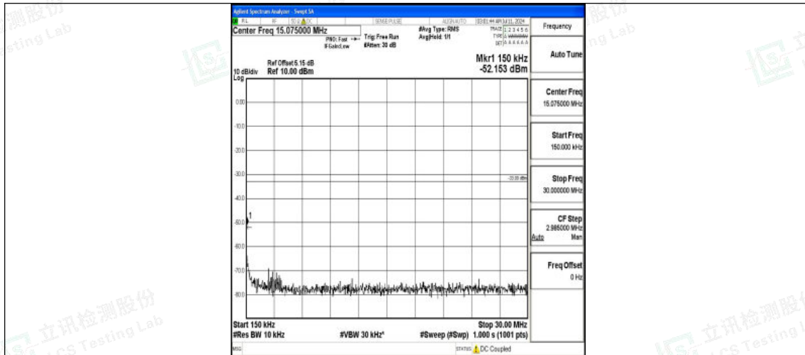
Band66_3MHz_16QAM_132322_1RB#0_0.15~30_0.15~30
