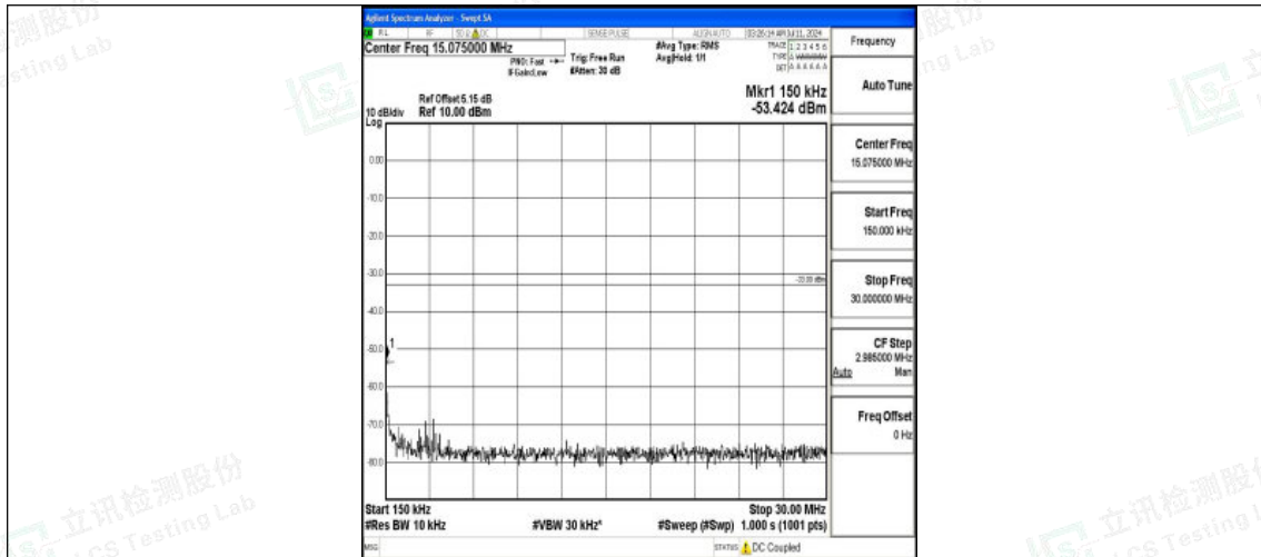
Band66_5MHz_QPSK_131997_1RB#0_0.15~30_0.15~30
