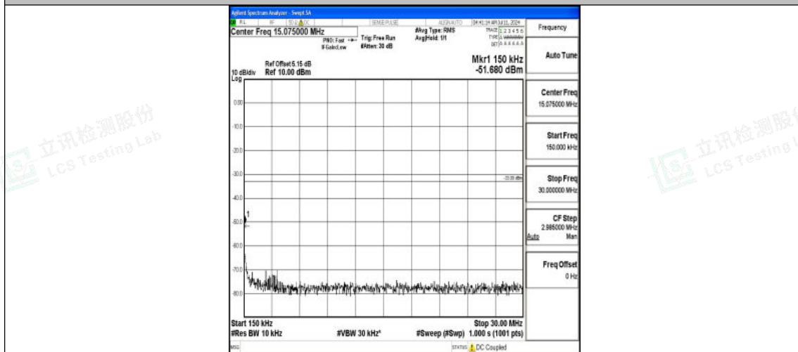
Band66_20MHz_16QAM_132072_1RB#0_0.15~30_0.15~30
