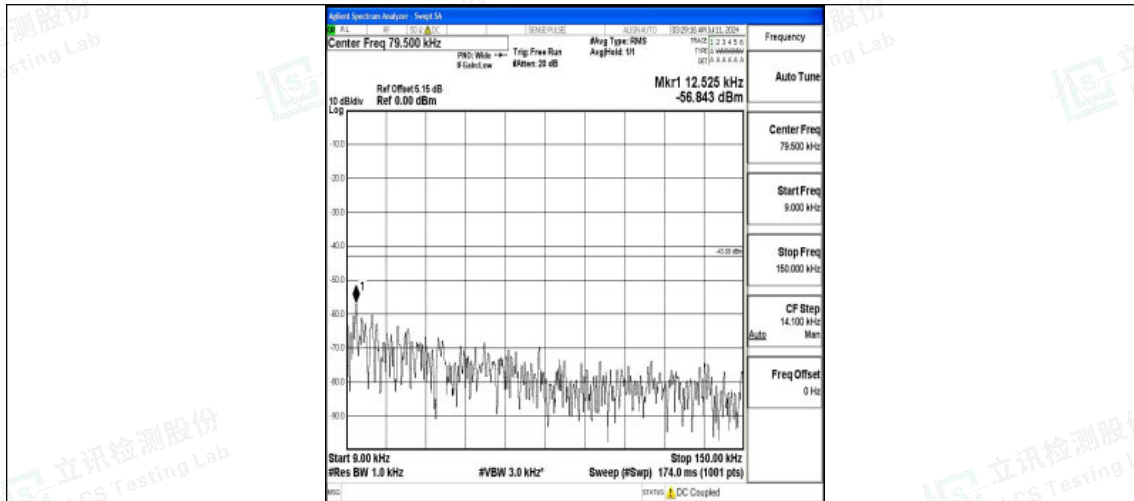
Band66_5MHz_16QAM_132647_1RB#0_0.009~0.15_0.009~0.15
