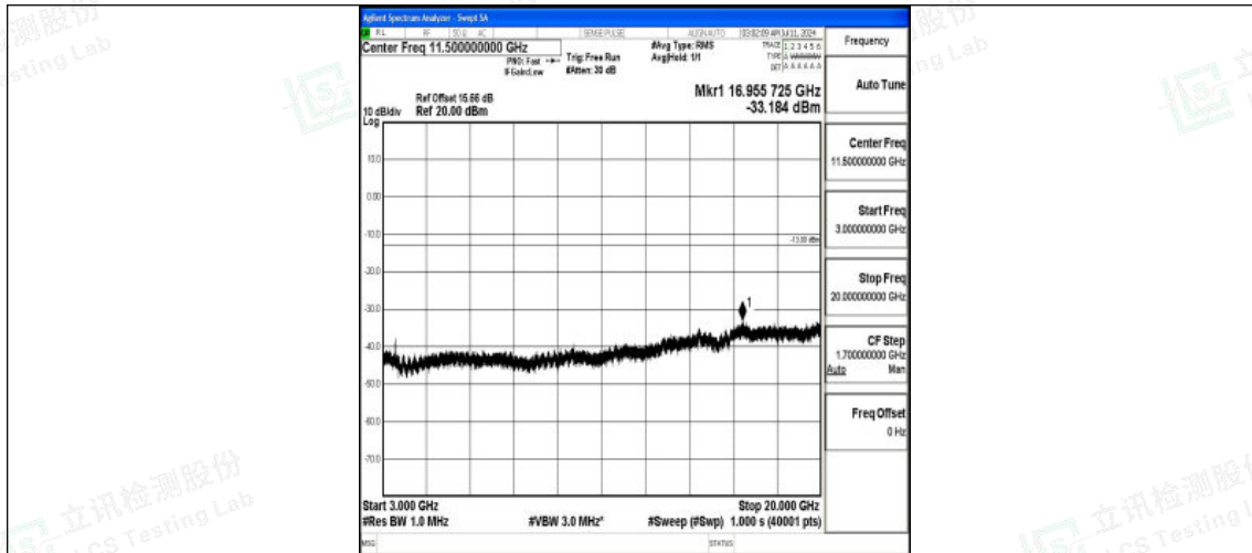
Band66_3MHz_16QAM_132322_1RB#0_3000~20000_3000~20000
