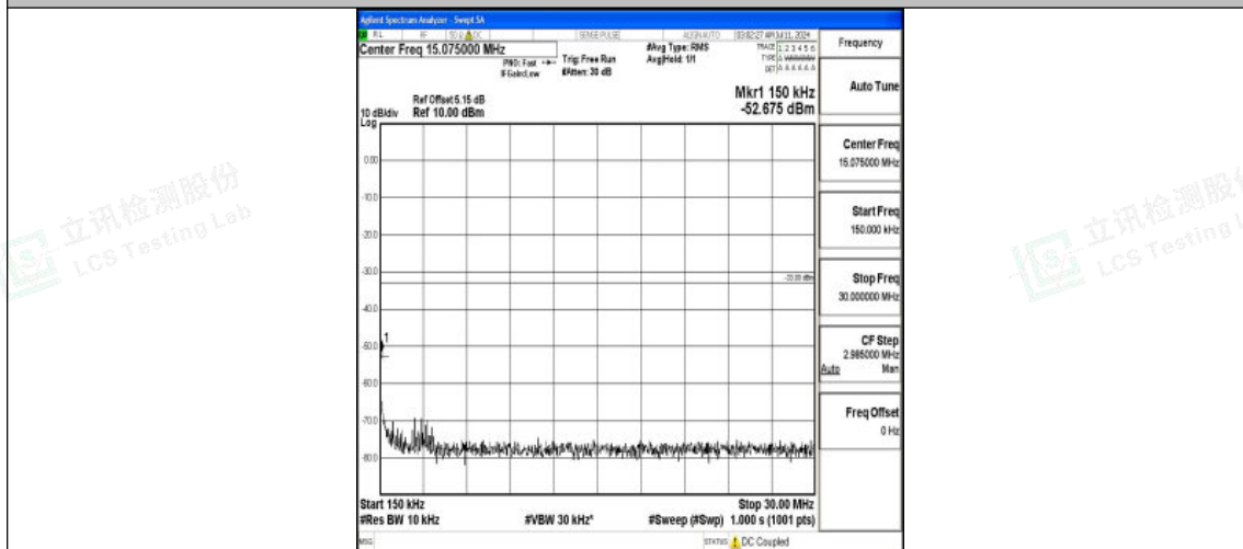
Band66_3MHz_QPSK_132657_1RB#0_0.15~30_0.15~30
