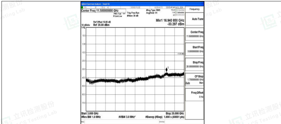
Band66_10MHz_16QAM_132322_1RB#0_3000~20000_3000~20000
