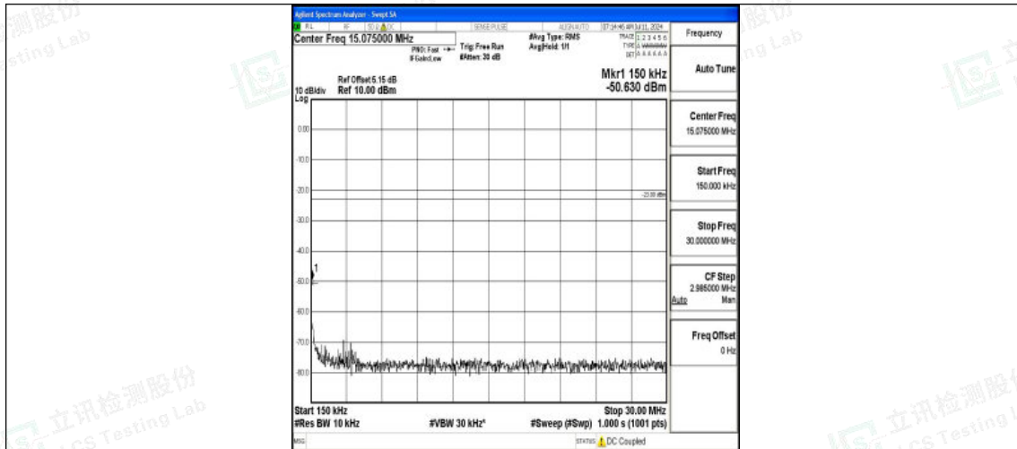
Band71_20MHz_16QAM_133372_1RB#0_0.15~30_0.15~30
