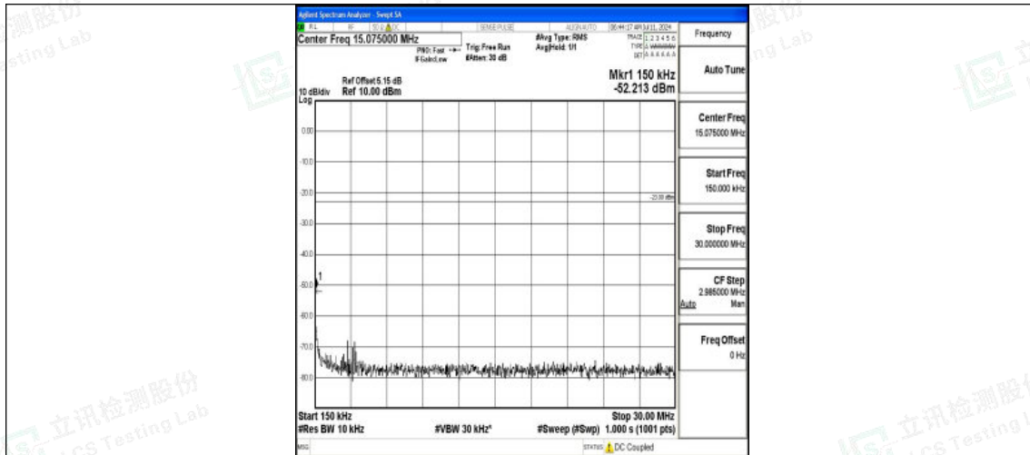
Band71_15MHz_16QAM_133397_1RB#0_0.15~30_0.15~30
