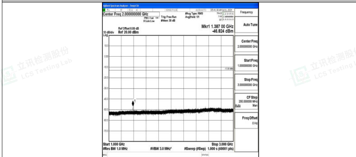
Band71_5MHz_16QAM_133447_1RB#0_1000~3000_1000~3000
