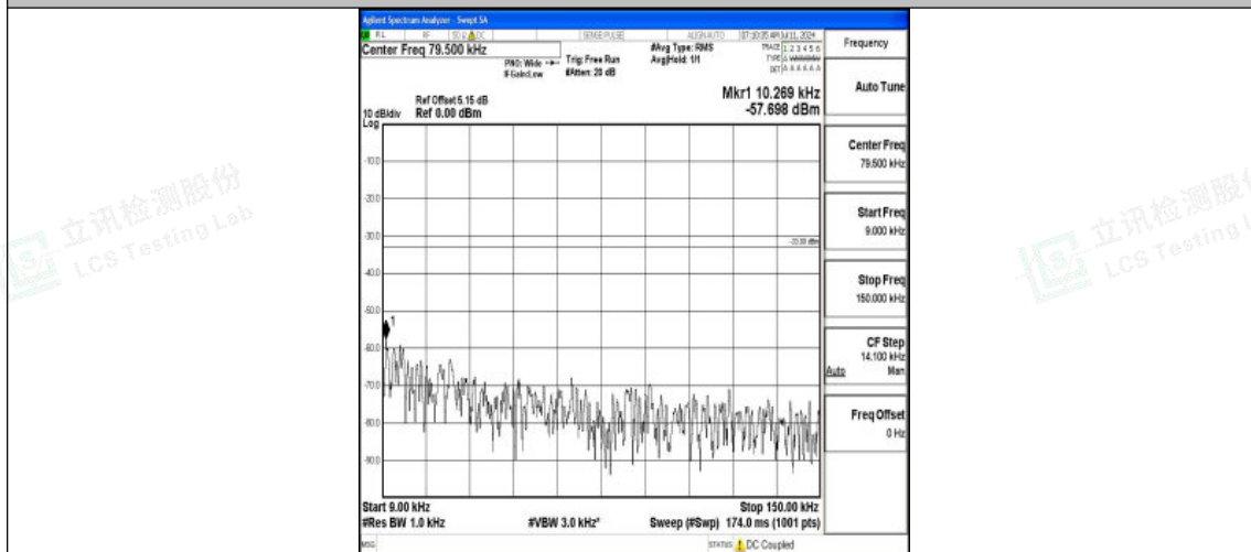
Band71_20MHz_QPSK_133322_1RB#0_0.009~0.15_0.009~0.15
