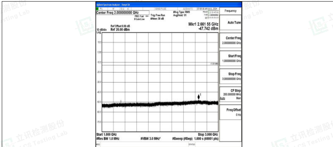
Band71_20MHz_16QAM_133222_1RB#0_1000~3000_1000~3000
