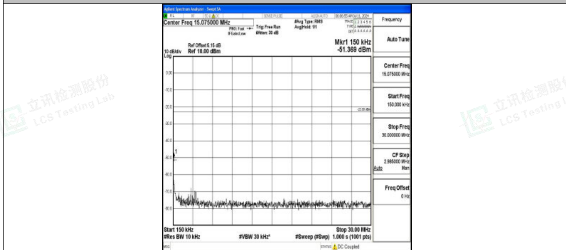
Band71_10MHz_QPSK_133172_1RB#0_0.15~30_0.15~30
