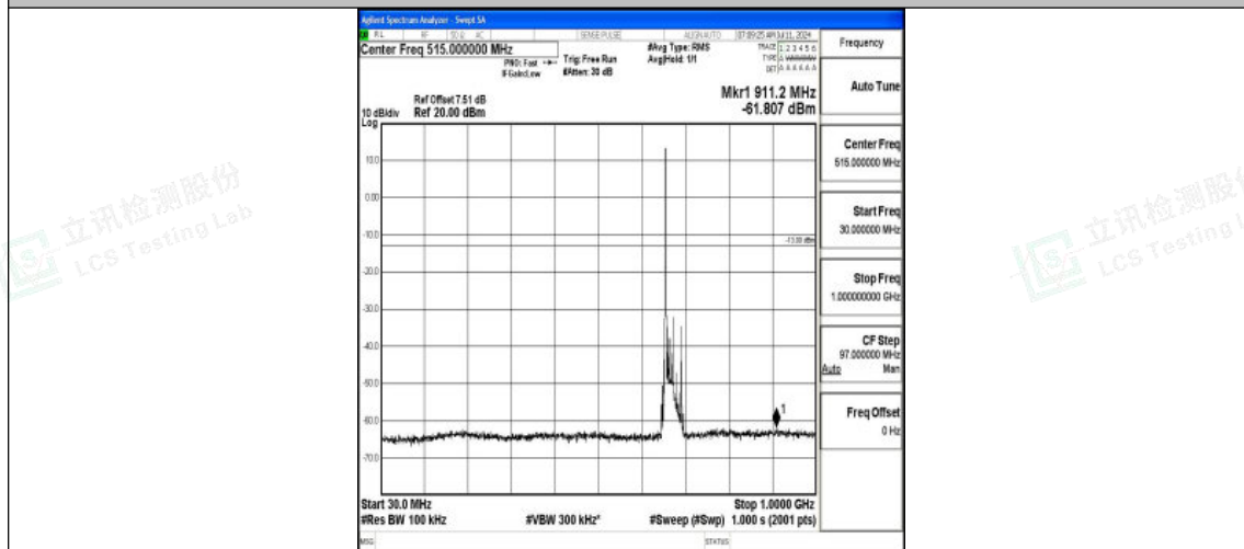
Band71_20MHz_16QAM_133222_1RB#0_30~1000_30~1000
