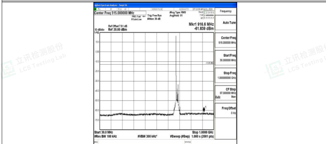
Band71_20MHz_QPSK_133372_1RB#0_30~1000_30~1000
