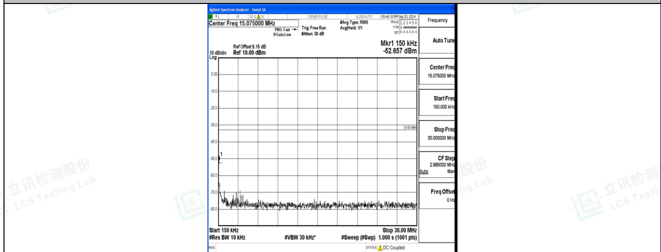
Band2_5MHz_QPSK_18900_1RB#0_0.15~30_0.15~30
