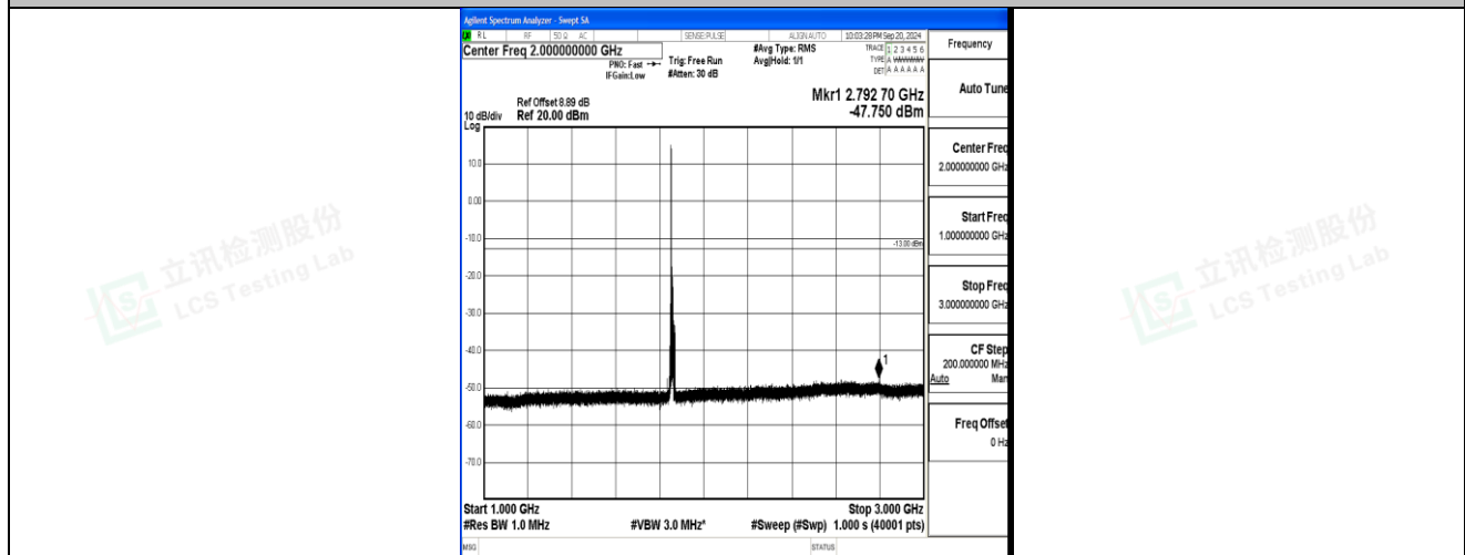
Band2_10MHz_QPSK_18650_1RB#0_1000~3000_1000~3000
