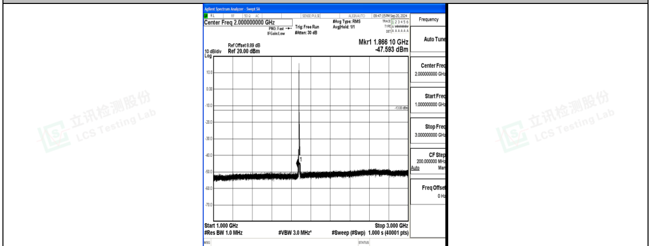
Band2_5MHz_16QAM_18900_1RB#0_1000~3000_1000~3000
