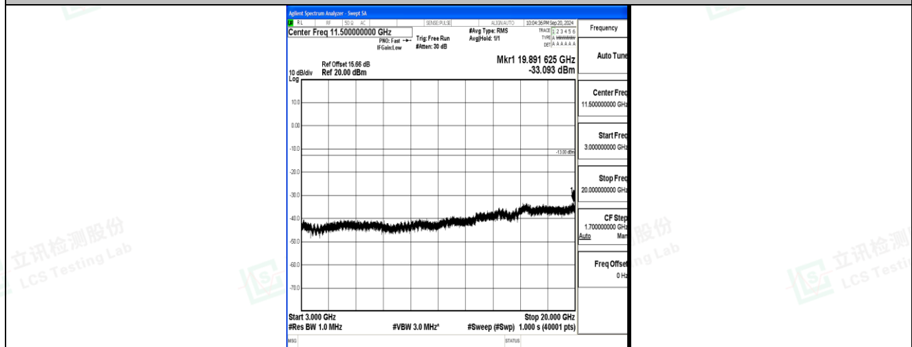
Band2_10MHz_QPSK_18900_1RB#0_3000~20000_3000~20000
