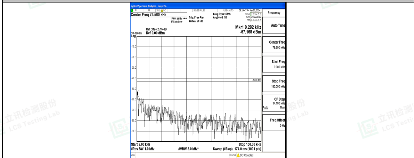
Band2_3MHz_QPSK_19185_1RB#0_0.009~0.15_0.009~0.15
