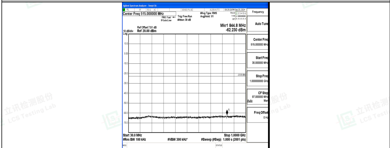
Band2_3MHz_16QAM_18900_1RB#0_30~1000_30~1000
