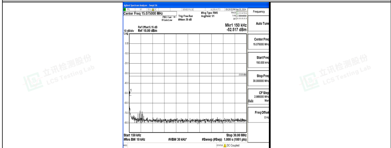
Band2_3MHz_QPSK_19185_1RB#0_0.15~30_0.15~30
