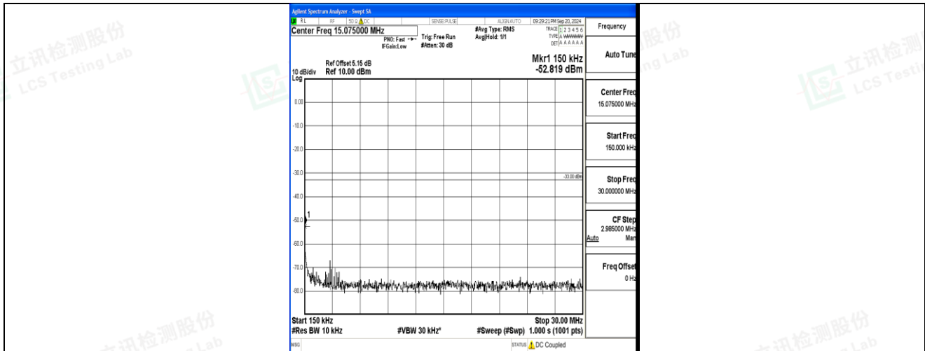
Band2_3MHz_16QAM_18900_1RB#0_0.15~30_0.15~30
