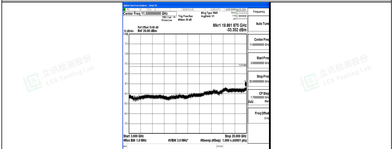
Band2_10MHz_QPSK_19150_1RB#0_3000~20000_3000~20000
