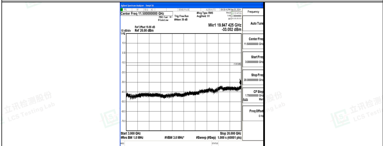
Band2_3MHz_16QAM_19185_1RB#0_3000~20000_3000~20000
