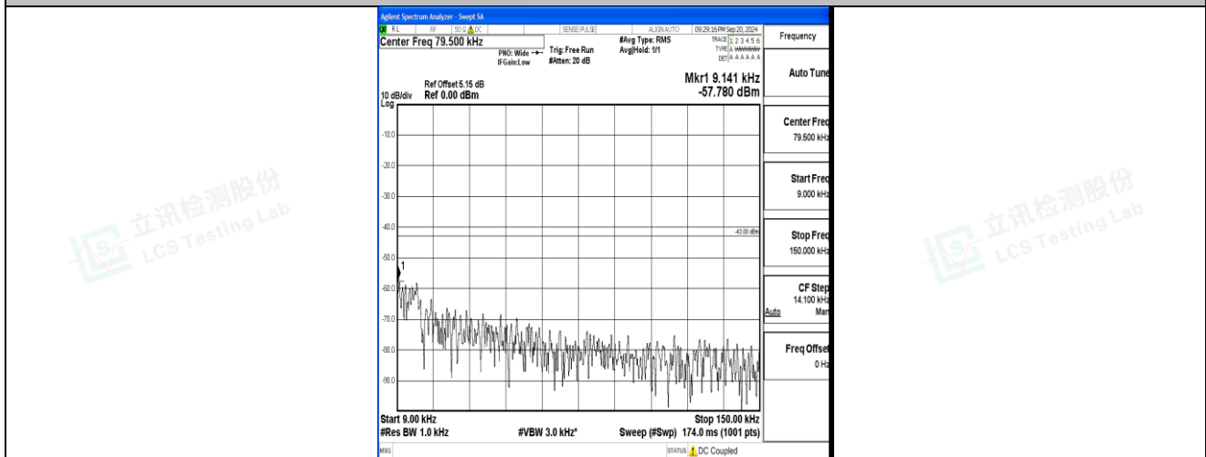
Band2_3MHz_16QAM_18900_1RB#0_0.009~0.15_0.009~0.15
