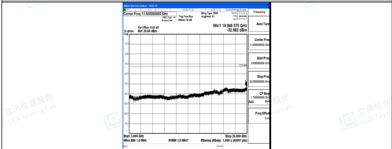
Band2_3MHz_QPSK_18900_1RB#0_3000~20000_3000~20000
