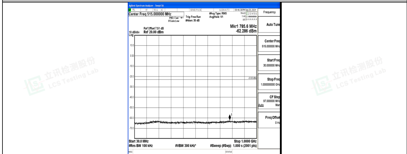
Band2_5MHz_QPSK_18900_1RB#0_30~1000_30~1000
