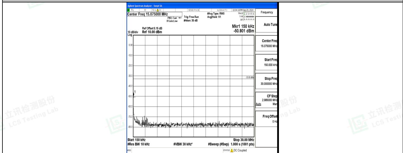
Band2_10MHz_QPSK_18900_1RB#0_0.15~30_0.15~30
