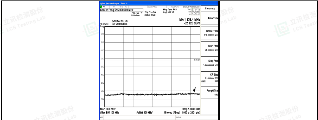
Band2_10MHz_QPSK_19150_1RB#0_30~1000_30~1000
