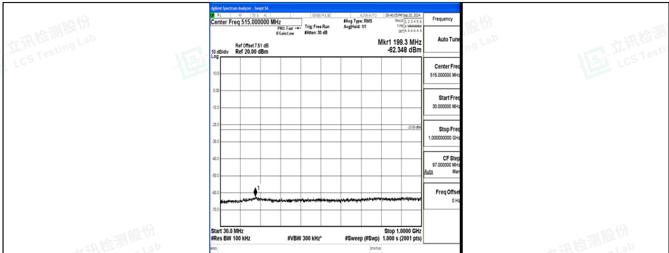
Band2_5MHz_16QAM_18625_1RB#0_30~1000_30~1000
