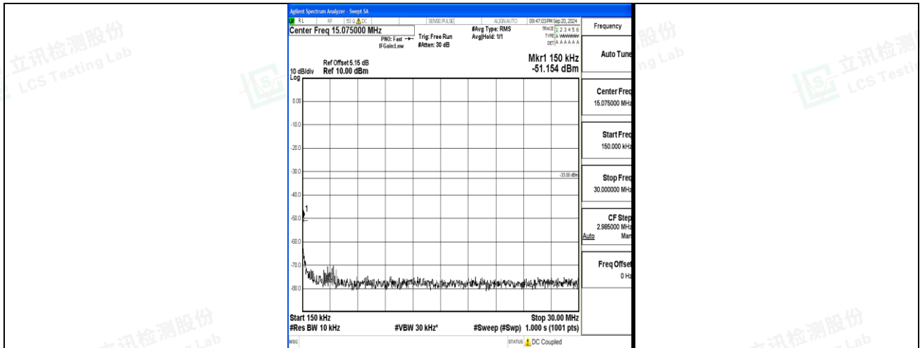
Band2_5MHz_16QAM_18900_1RB#0_0.15~30_0.15~30
