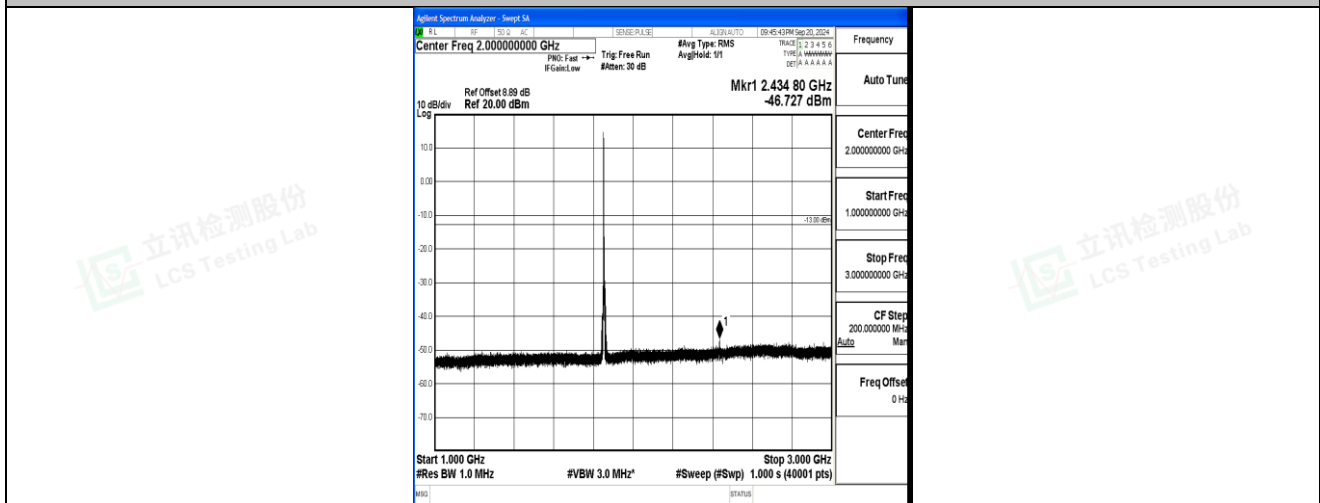
Band2_5MHz_QPSK_18625_1RB#0_1000~3000_1000~3000
