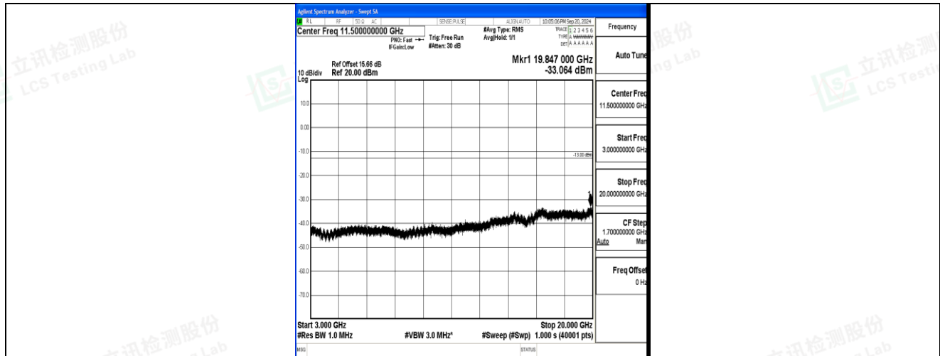
Band2_10MHz_16QAM_18900_1RB#0_3000~20000_3000~20000
