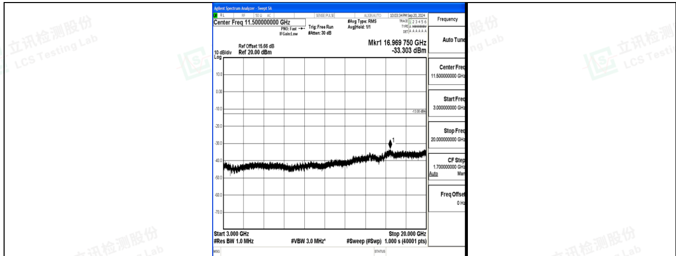
Band2_10MHz_QPSK_18650_1RB#0_3000~20000_3000~20000
