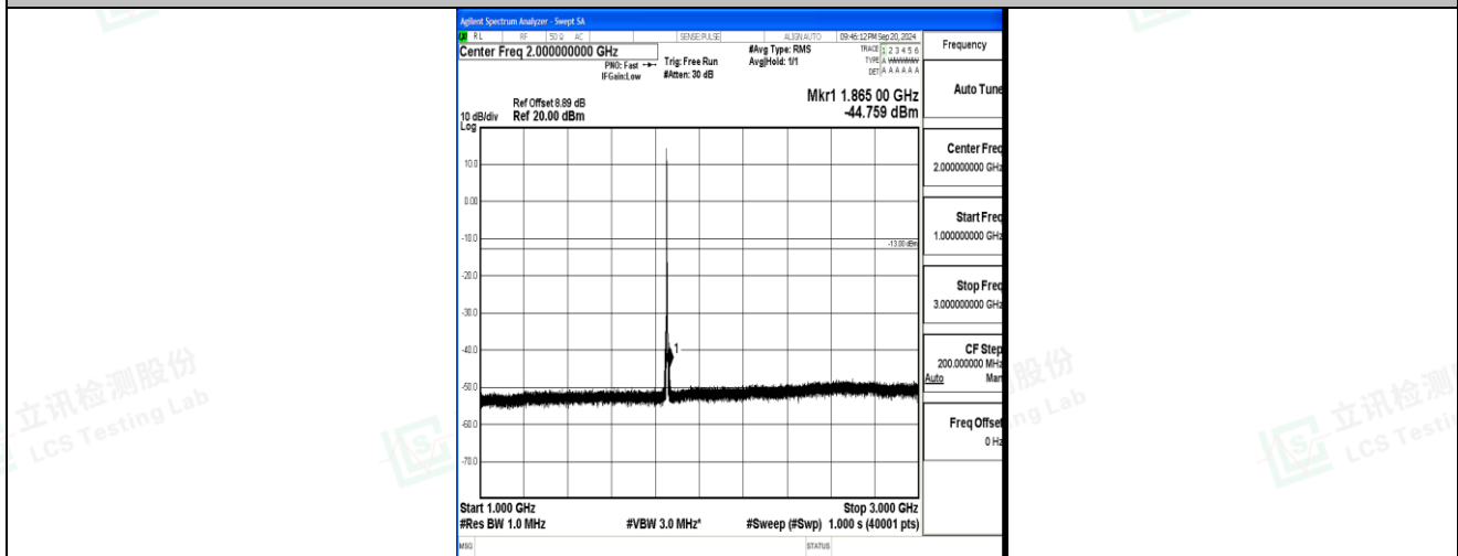
Band2_5MHz_16QAM_18625_1RB#0_1000~3000_1000~3000
