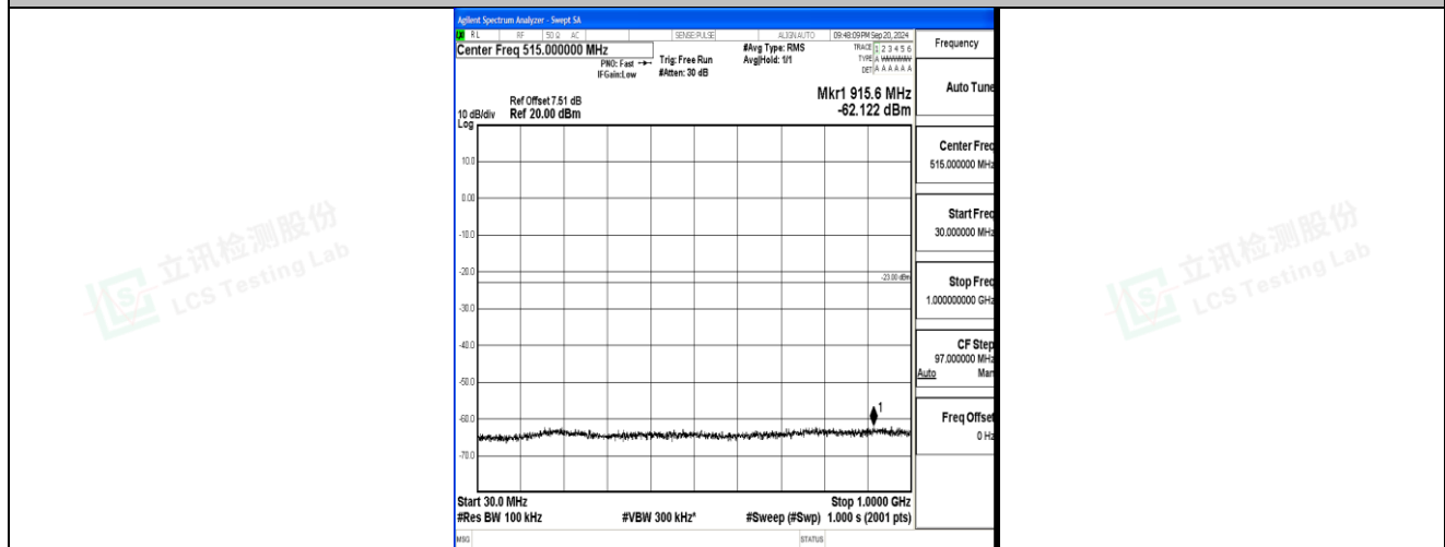
Band2_5MHz_16QAM_19175_1RB#0_30~1000_30~1000
