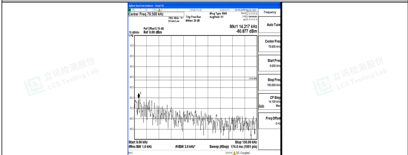
Band2_5MHz_QPSK_18625_1RB#0_0.009~0.15_0.009~0.15
