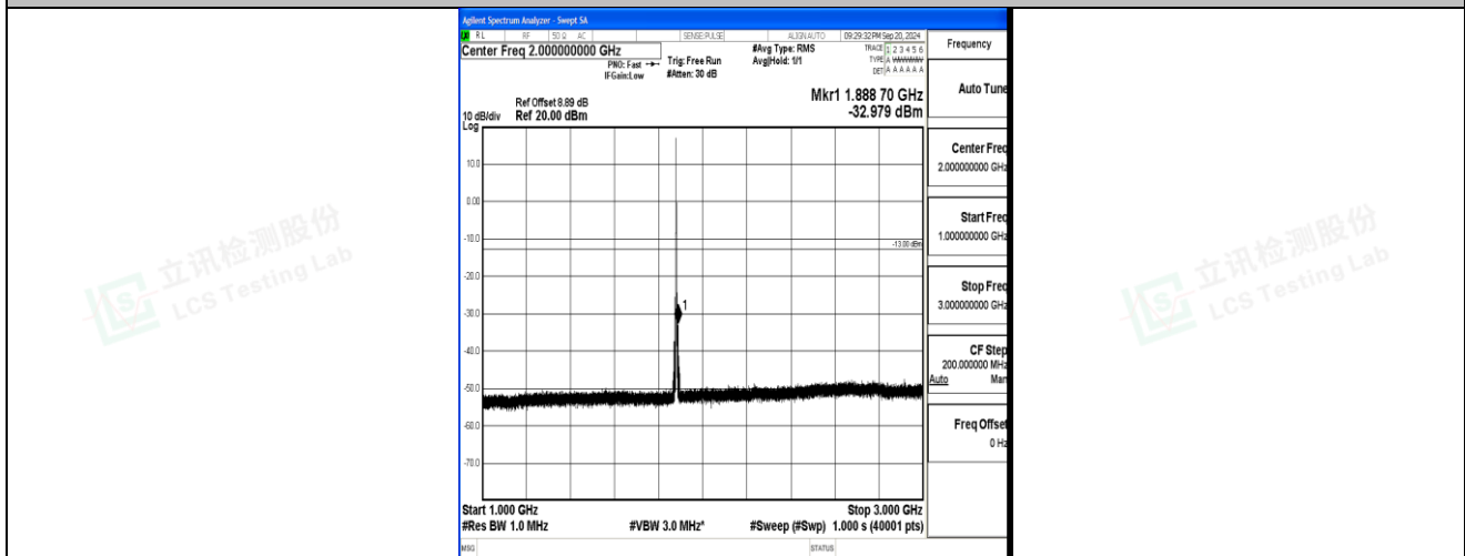
Band2_3MHz_16QAM_18900_1RB#0_1000~3000_1000~3000
