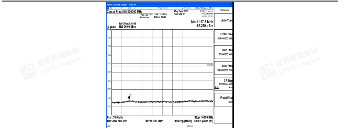
Band2_10MHz_QPSK_18900_1RB#0_30~1000_30~1000
