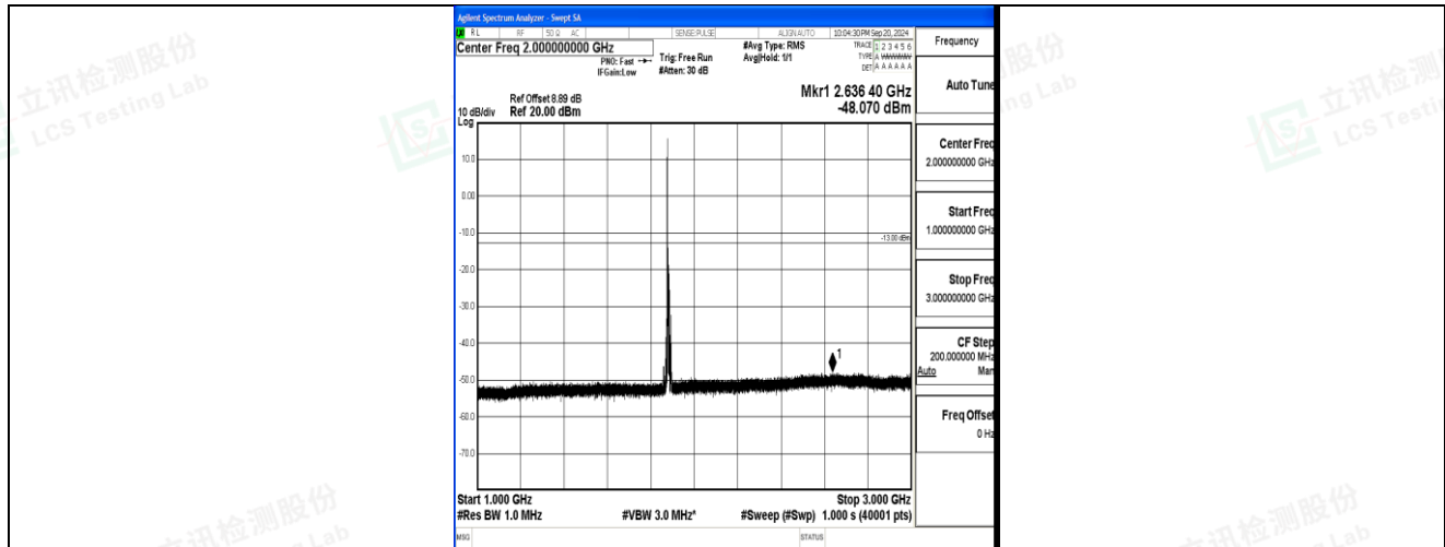
Band2_10MHz_QPSK_18900_1RB#0_1000~3000_1000~3000
