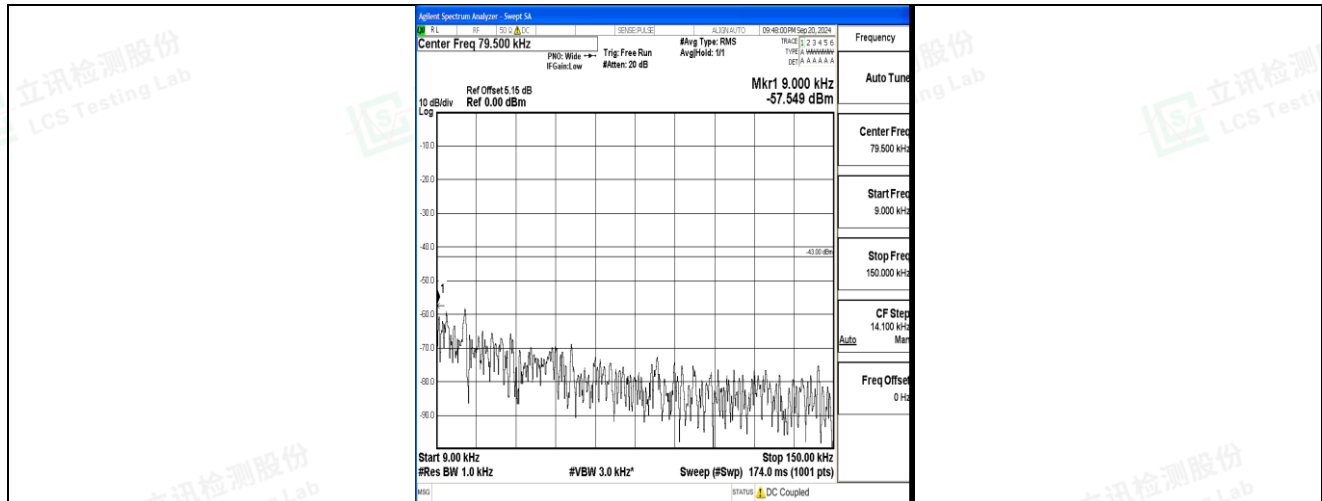
Band2_5MHz_16QAM_19175_1RB#0_0.009~0.15_0.009~0.15
