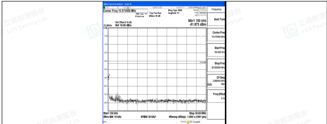
Band2_10MHz_QPSK_18650_1RB#0_0.15~30_0.15~30
