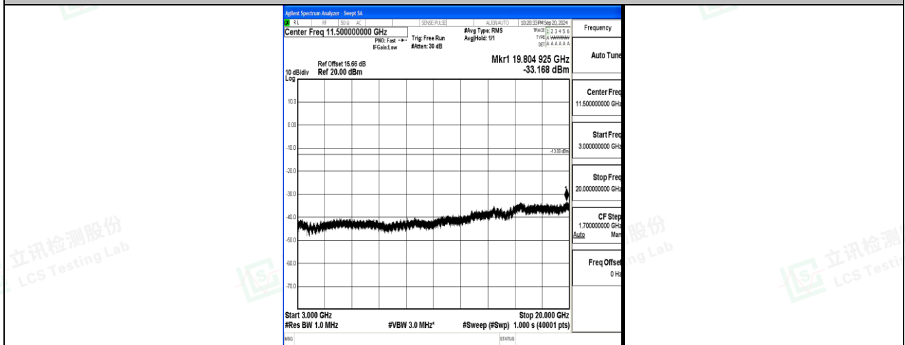
Band2_15MHz_QPSK_18900_1RB#0_3000~20000_3000~20000
