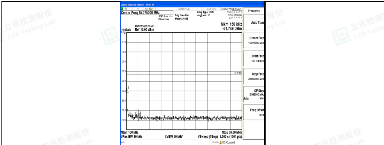
Band2_20MHz_16QAM_18900_1RB#0_0.15~30_0.15~30
