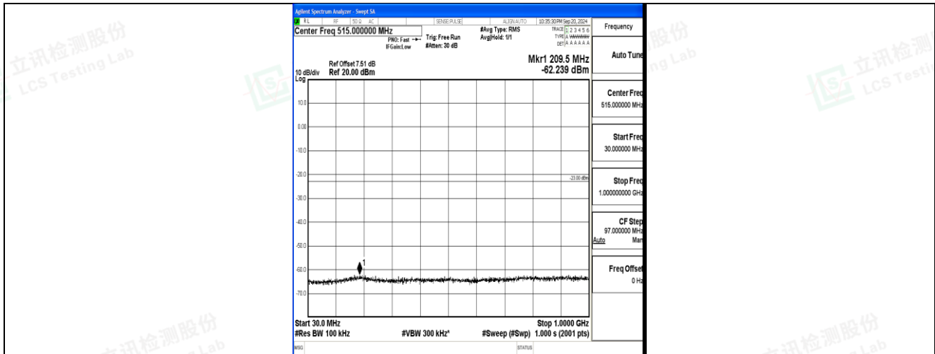
Band2_20MHz_16QAM_18700_1RB#0_30~1000_30~1000
