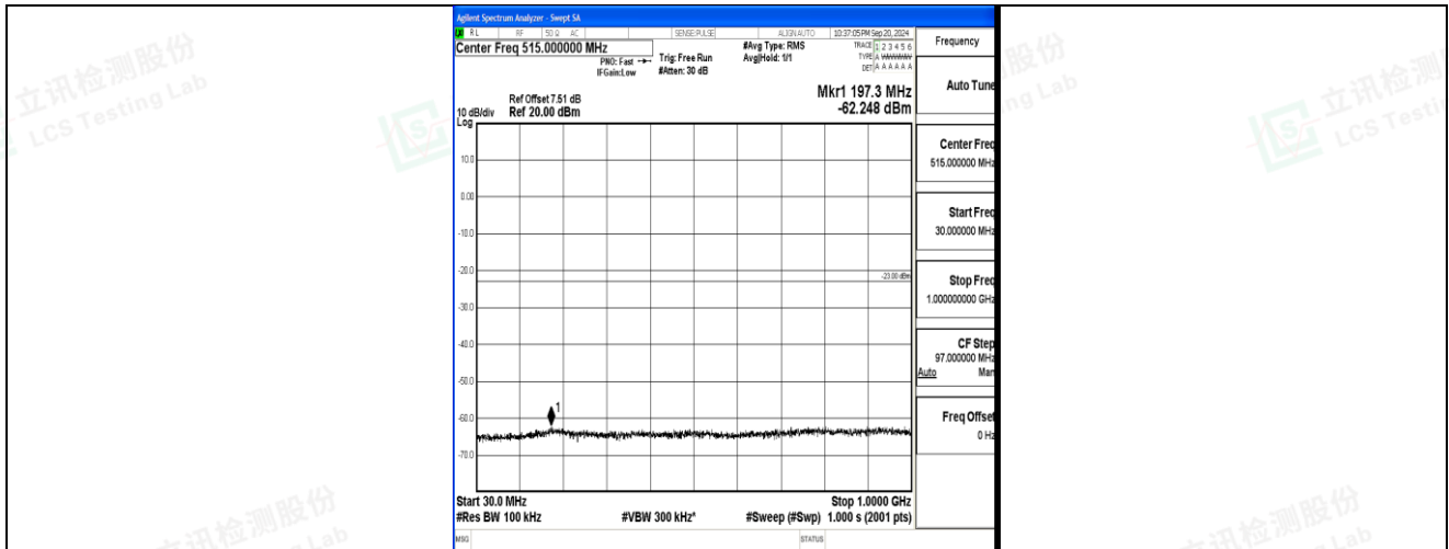
Band2_20MHz_QPSK_19100_1RB#0_30~1000_30~1000
