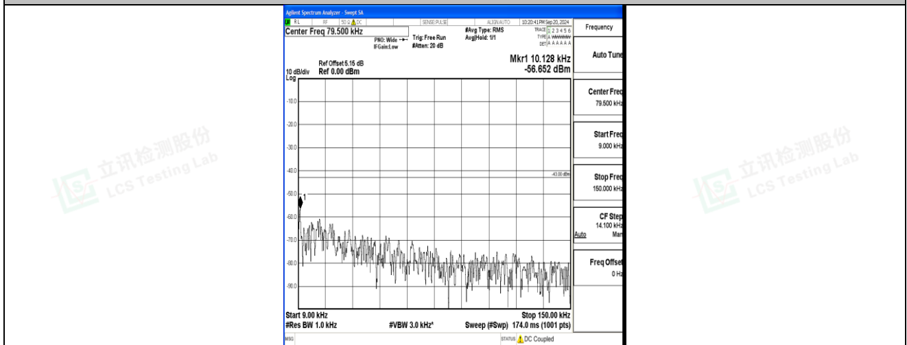
Band2_15MHz_16QAM_18900_1RB#0_0.009~0.15_0.009~0.15
