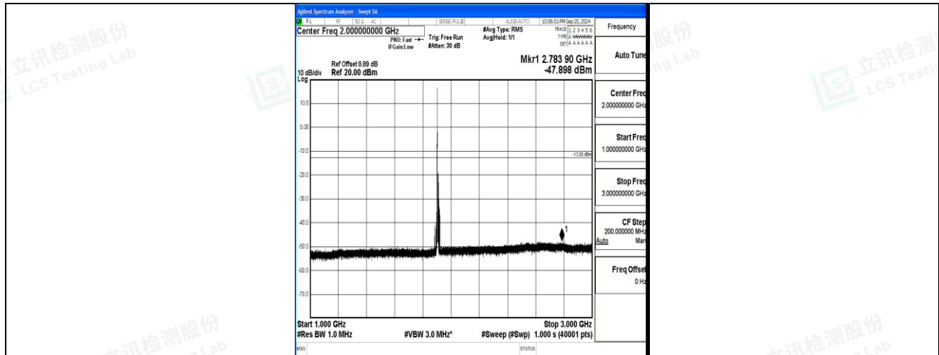
Band2_10MHz_16QAM_19150_1RB#0_1000~3000_1000~3000
