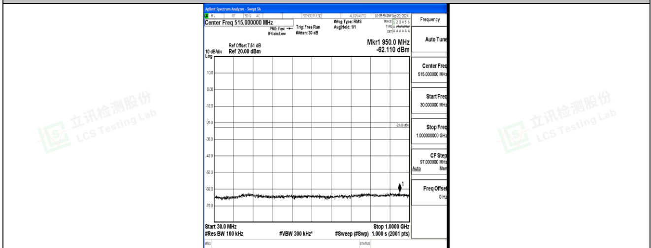
Band2_10MHz_16QAM_19150_1RB#0_30~1000_30~1000
