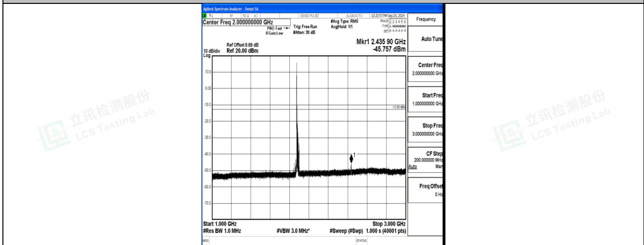
Band2_15MHz_16QAM_18900_1RB#0_1000~3000_1000~3000
