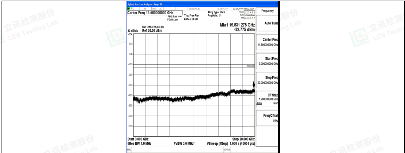
Band2_15MHz_QPSK_18675_1RB#0_3000~20000_3000~20000
