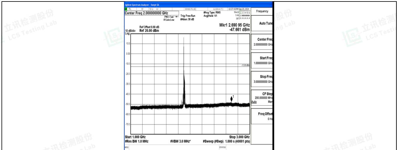
Band2_20MHz_16QAM_19100_1RB#0_1000~3000_1000~3000
