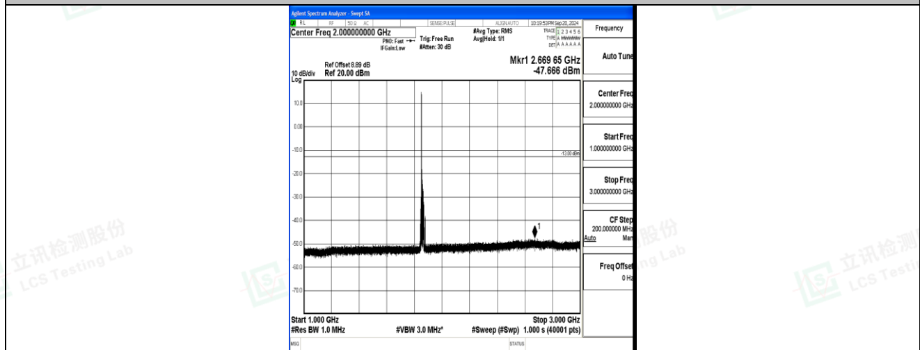
Band2_15MHz_16QAM_18675_1RB#0_1000~3000_1000~3000
