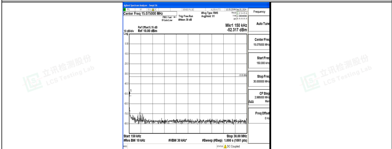
Band2_20MHz_16QAM_18700_1RB#0_0.15~30_0.15~30
