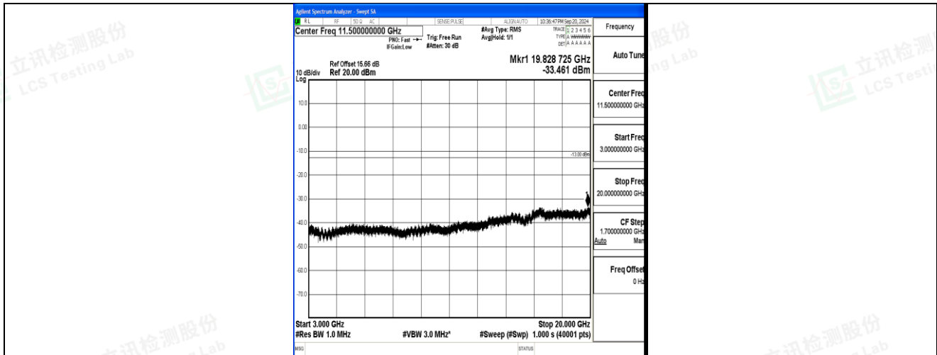
Band2_20MHz_16QAM_18900_1RB#0_3000~20000_3000~20000
