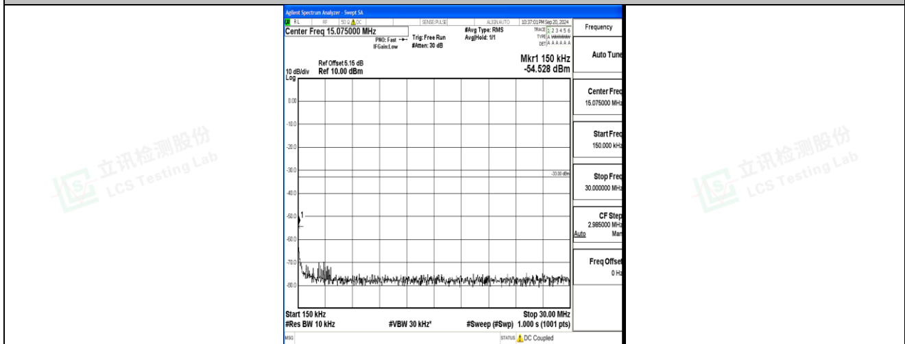
Band2_20MHz_QPSK_19100_1RB#0_0.15~30_0.15~30
