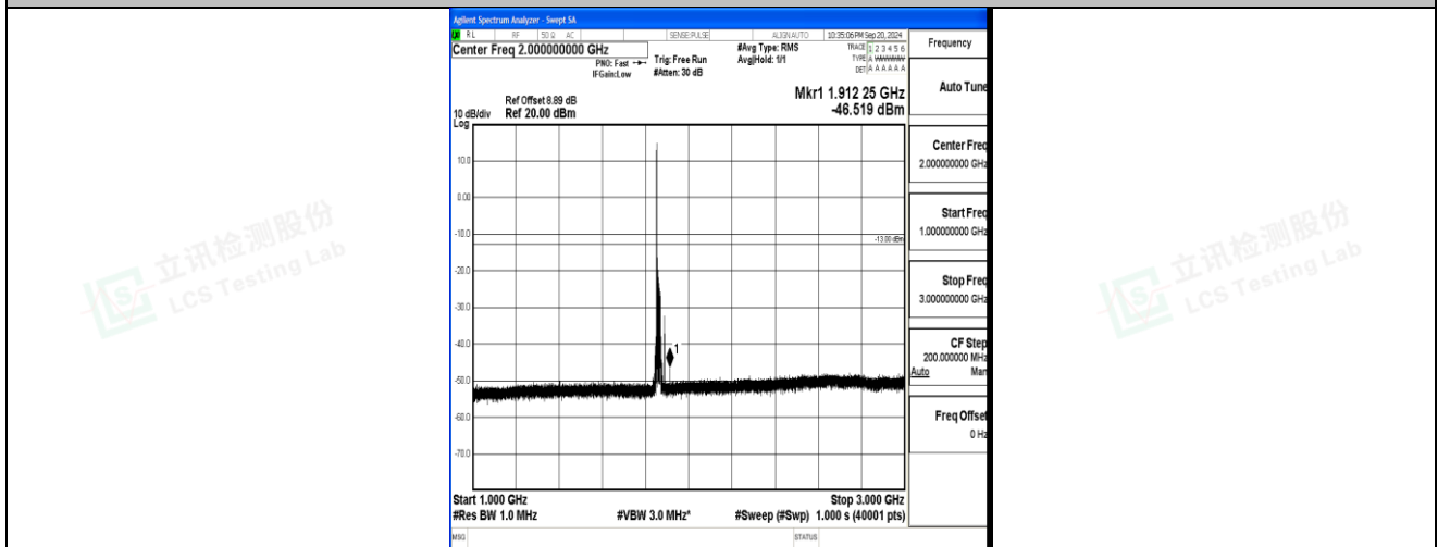
Band2_20MHz_QPSK_18700_1RB#0_1000~3000_1000~3000
