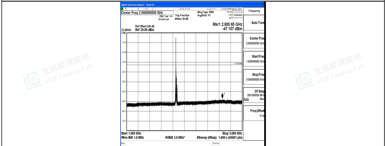
Band2_15MHz_QPSK_18675_1RB#0_1000~3000_1000~3000
