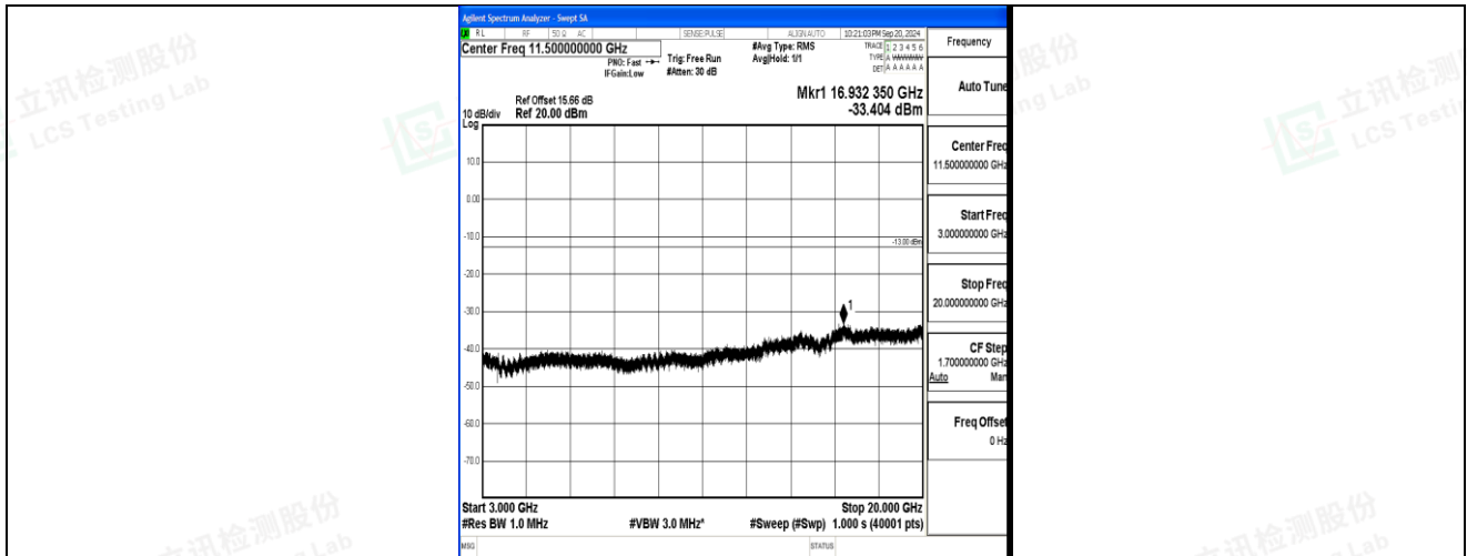
Band2_15MHz_16QAM_18900_1RB#0_3000~20000_3000~20000
