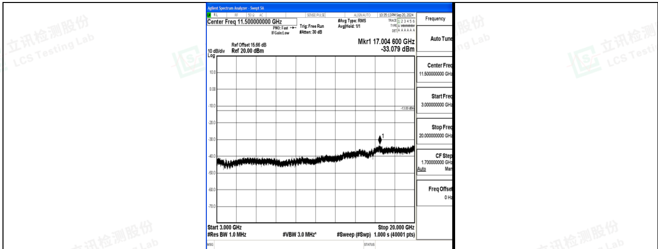
Band2_20MHz_QPSK_18700_1RB#0_3000~20000_3000~20000
