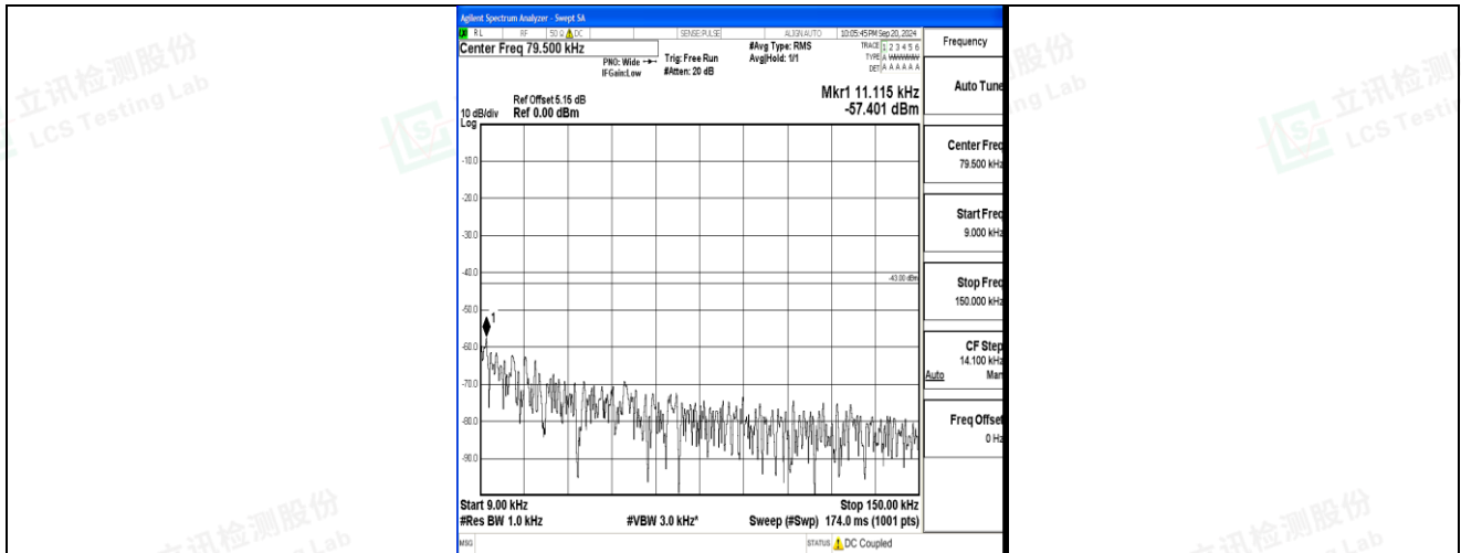
Band2_10MHz_16QAM_19150_1RB#0_0.009~0.15_0.009~0.15
