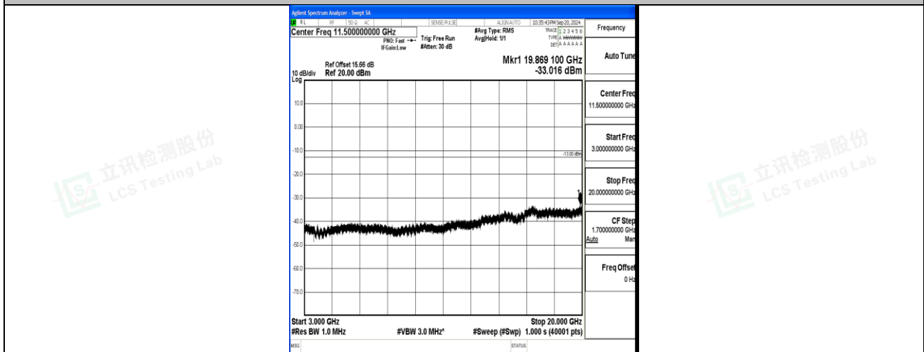
Band2_20MHz_16QAM_18700_1RB#0_3000~20000_3000~20000
