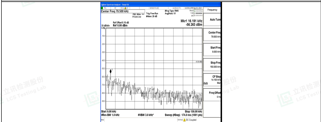
Band2_20MHz_16QAM_18700_1RB#0_0.009~0.15_0.009~0.15
