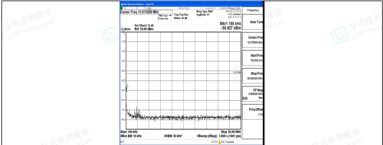
Band2_15MHz_QPSK_18675_1RB#0_0.15~30_0.15~30
