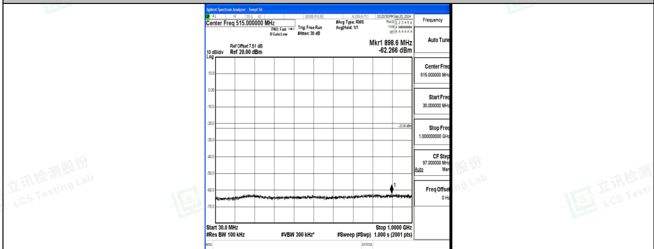
Band2_15MHz_16QAM_18900_1RB#0_30~1000_30~1000
