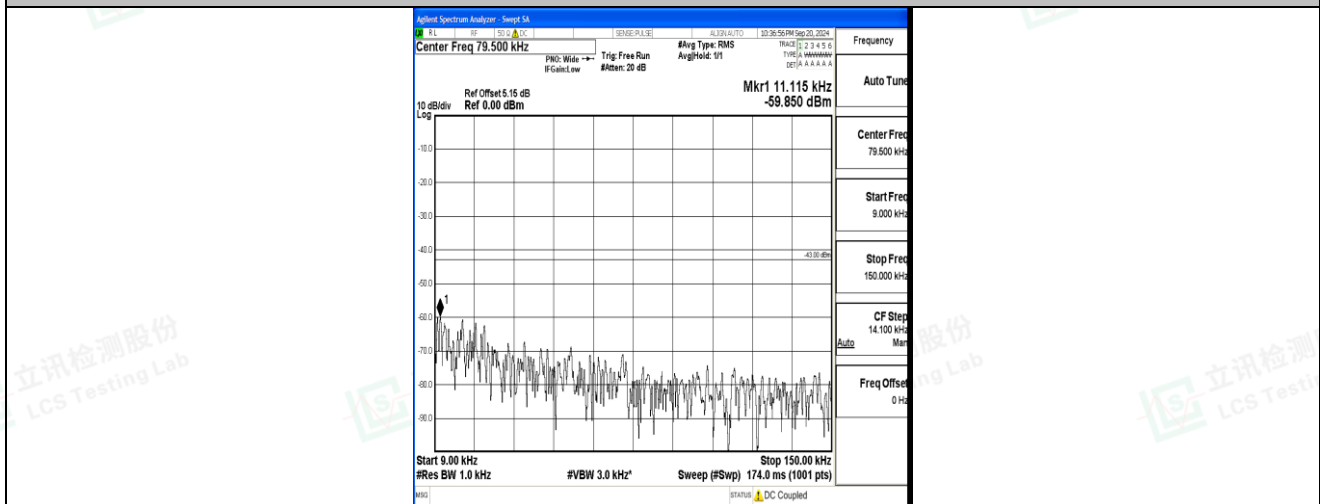
Band2_20MHz_QPSK_19100_1RB#0_0.009~0.15_0.009~0.15
