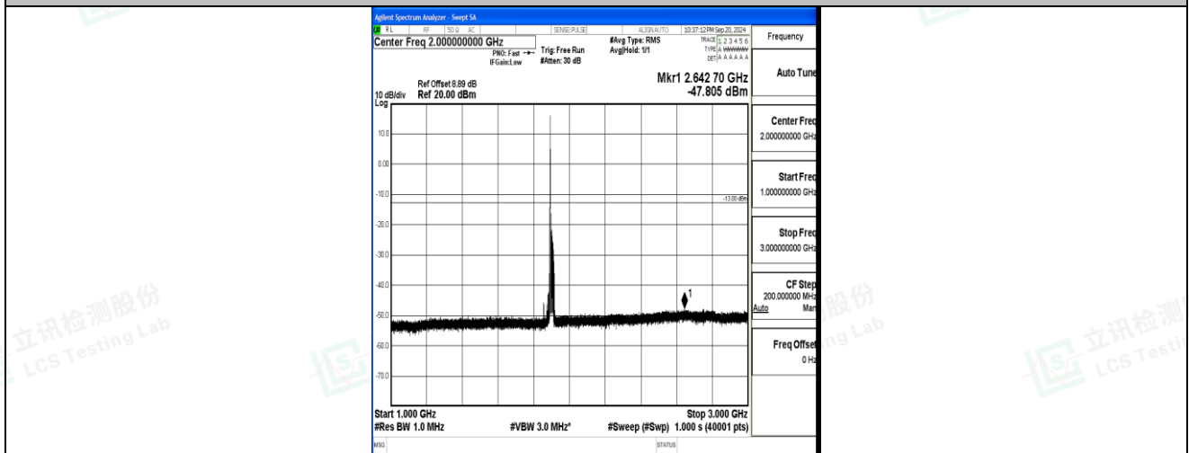
Band2_20MHz_QPSK_19100_1RB#0_1000~3000_1000~3000
