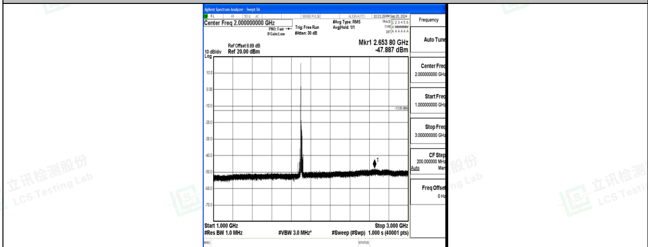
Band2_15MHz_QPSK_19125_1RB#0_1000~3000_1000~3000
