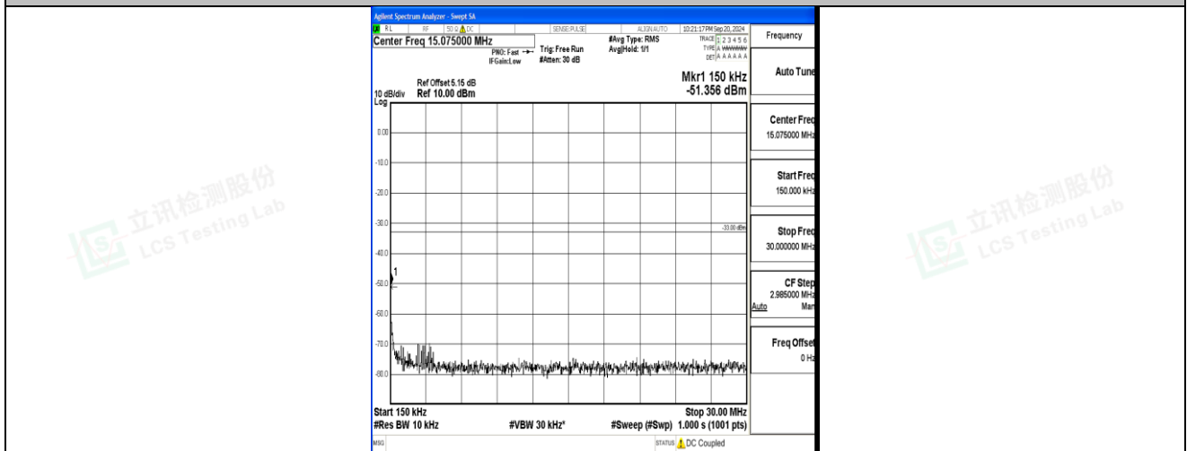
Band2_15MHz_QPSK_19125_1RB#0_0.15~30_0.15~30
