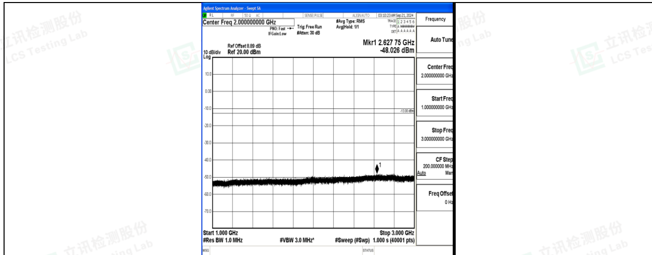
Band12_10MHz_16QAM_23095_1RB#0_1000~3000_1000~3000
