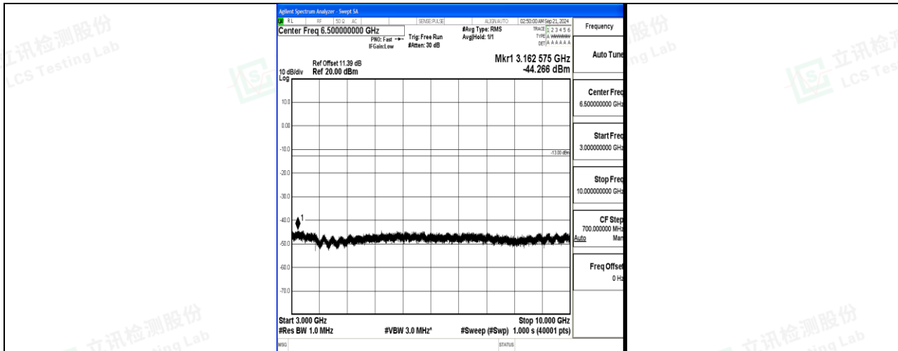
Band12_5MHz_QPSK_23155_1RB#0_3000~10000_3000~10000
