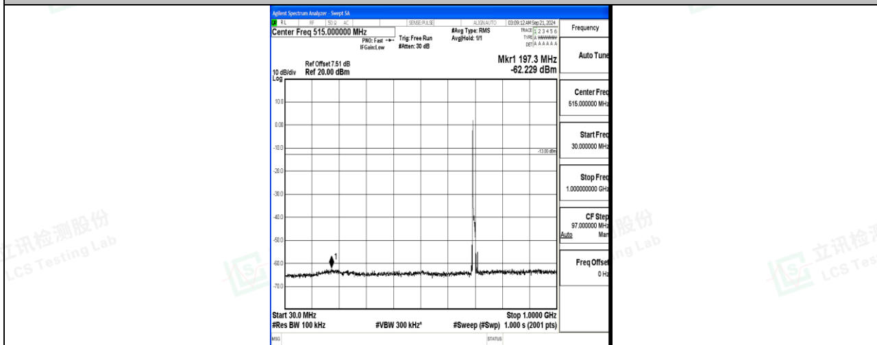
Band12_10MHz_16QAM_23060_1RB#0_30~1000_30~1000
