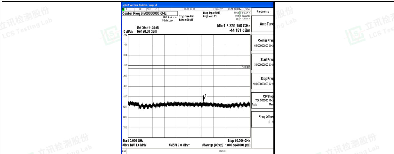
Band12_10MHz_16QAM_23060_1RB#0_3000~10000_3000~10000
