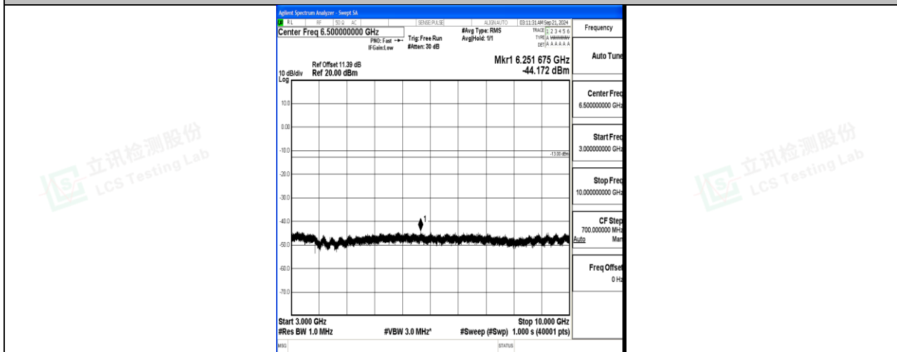
Band12_10MHz_16QAM_23130_1RB#0_3000~10000_3000~10000
