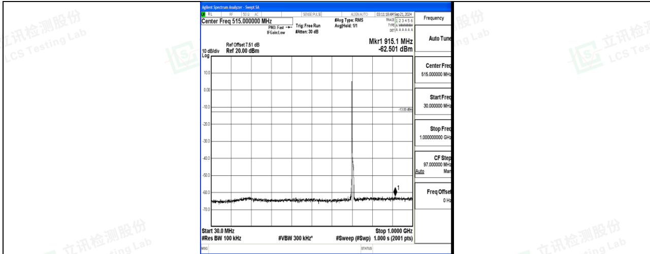
Band12_10MHz_16QAM_23130_1RB#0_30~1000_30~1000
