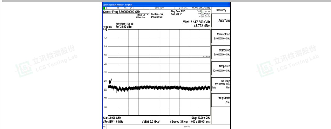
Band12_5MHz_QPSK_23095_1RB#0_3000~10000_3000~10000
