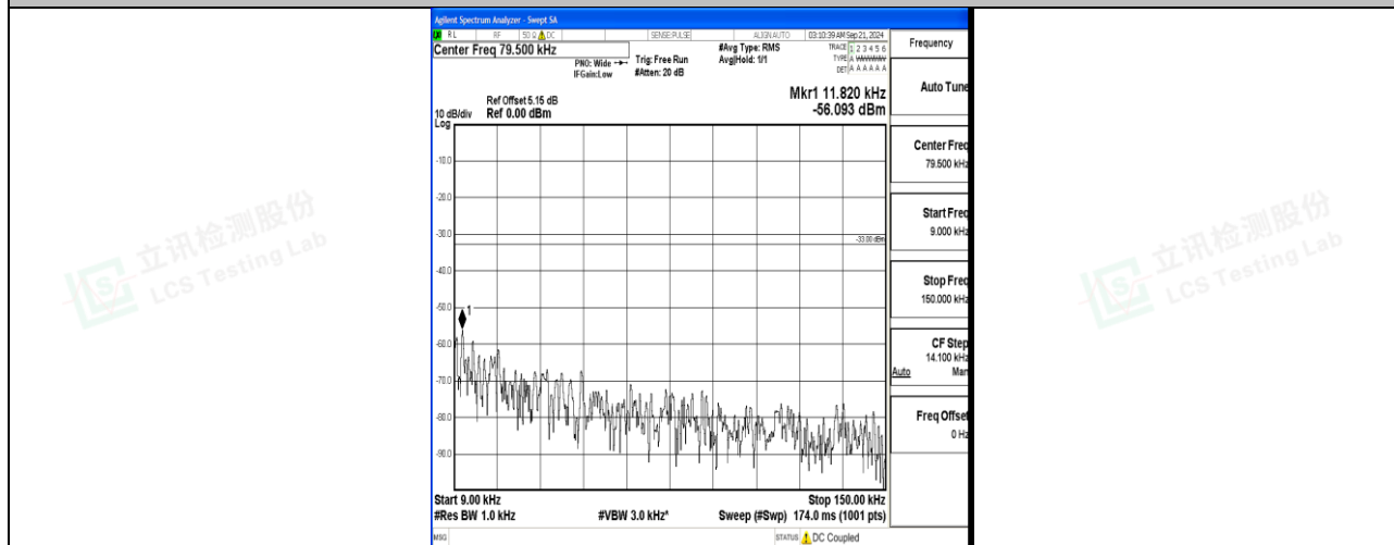
Band12_10MHz_QPSK_23130_1RB#0_0.009~0.15_0.009~0.15
