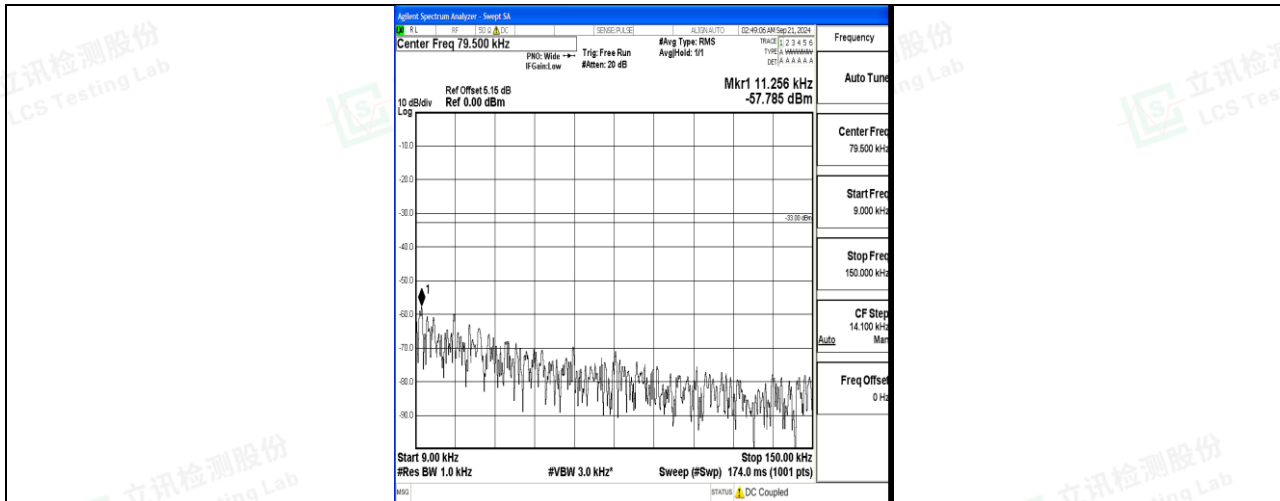
Band12_5MHz_16QAM_23095_1RB#0_0.009~0.15_0.009~0.15
