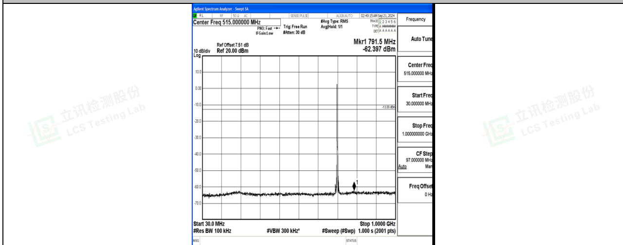
Band12_5MHz_16QAM_23095_1RB#0_30~1000_30~1000
