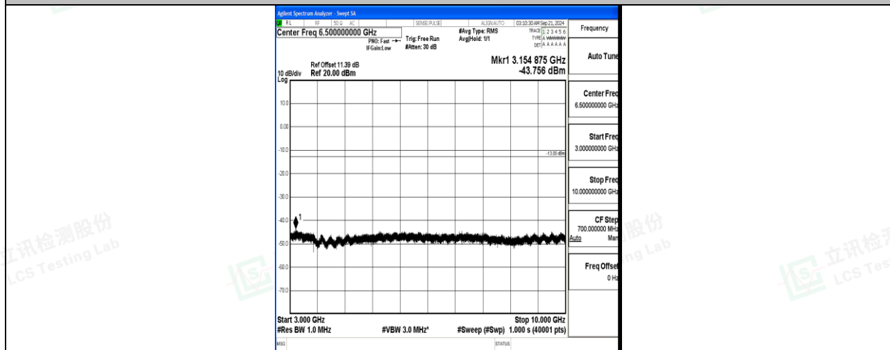
Band12_10MHz_16QAM_23095_1RB#0_3000~10000_3000~10000
