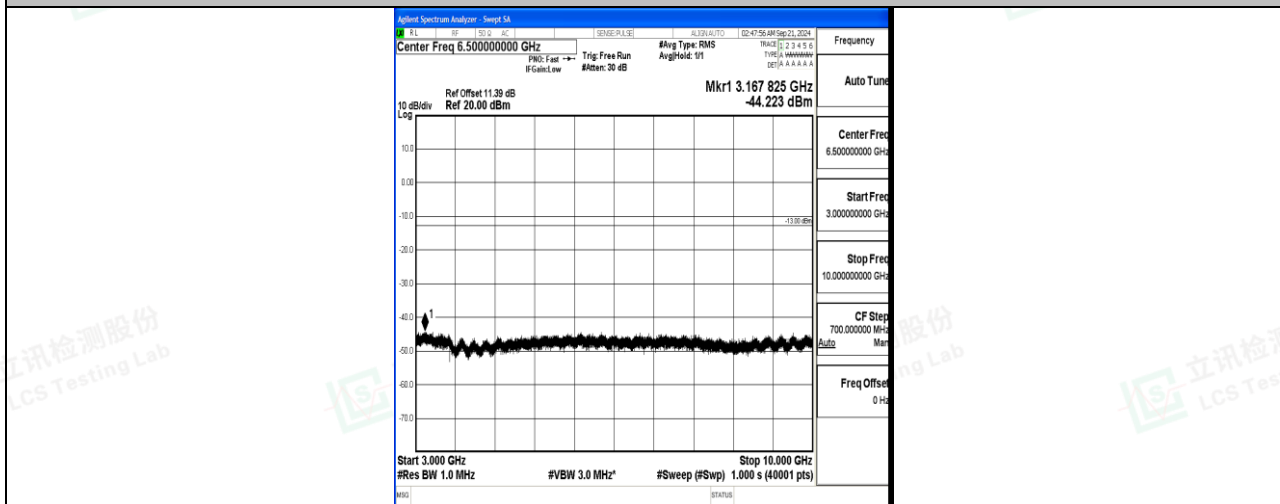
Band12_5MHz_QPSK_23035_1RB#0_3000~10000_3000~10000
