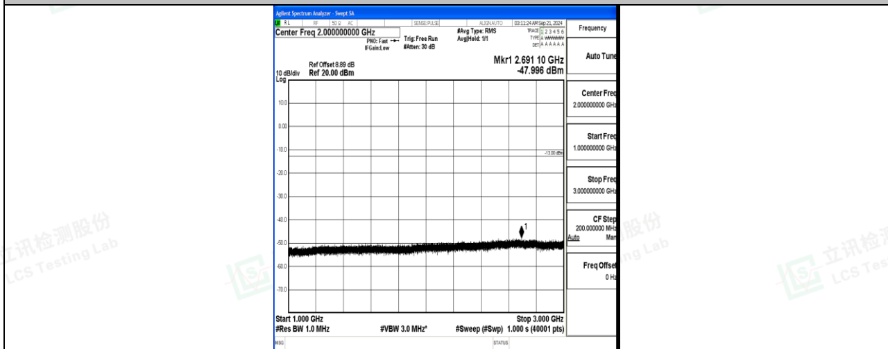
Band12_10MHz_16QAM_23130_1RB#0_1000~3000_1000~3000
