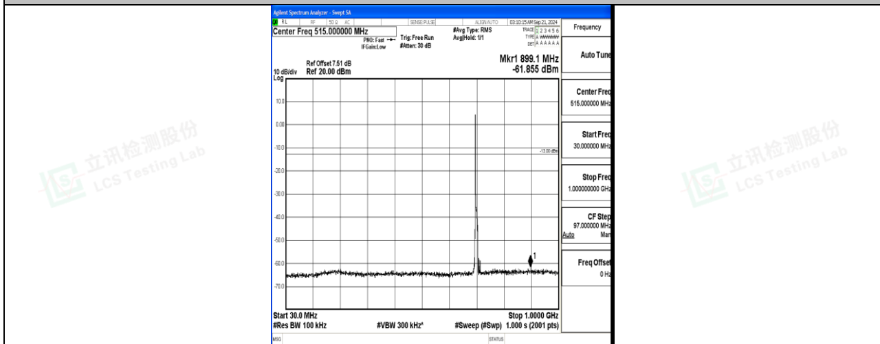
Band12_10MHz_16QAM_23095_1RB#0_30~1000_30~1000
