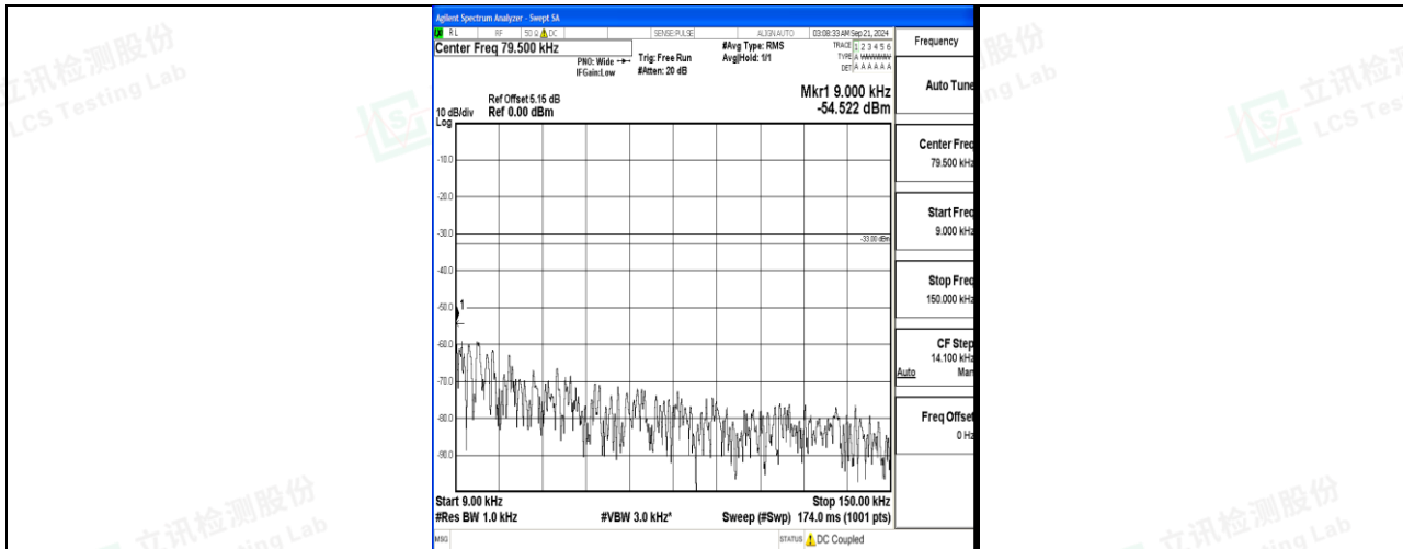
Band12_10MHz_QPSK_23060_1RB#0_0.009~0.15_0.009~0.15
