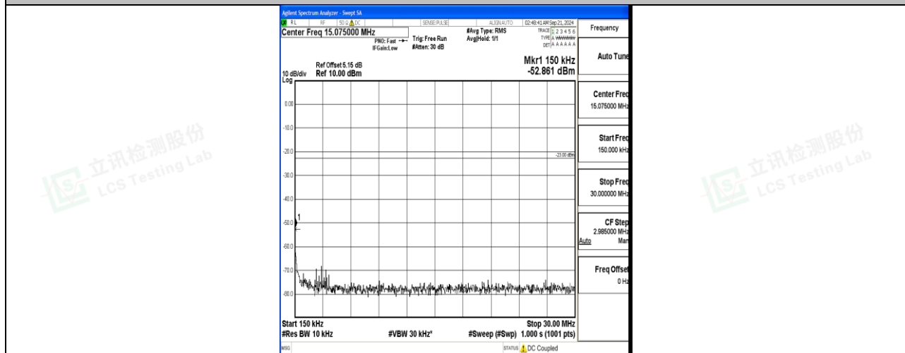
Band12_5MHz_QPSK_23095_1RB#0_0.15~30_0.15~30
