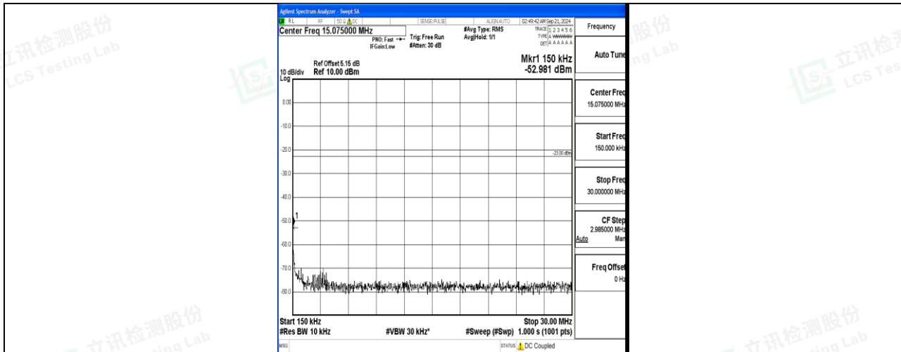
Band12_5MHz_QPSK_23155_1RB#0_0.15~30_0.15~30
