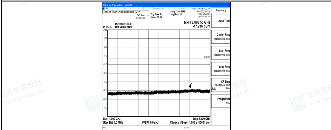
Band12_5MHz_16QAM_23155_1RB#0_1000~3000_1000~3000
