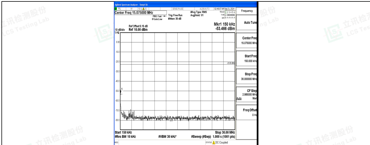
Band12_5MHz_16QAM_23035_1RB#0_0.15~30_0.15~30
