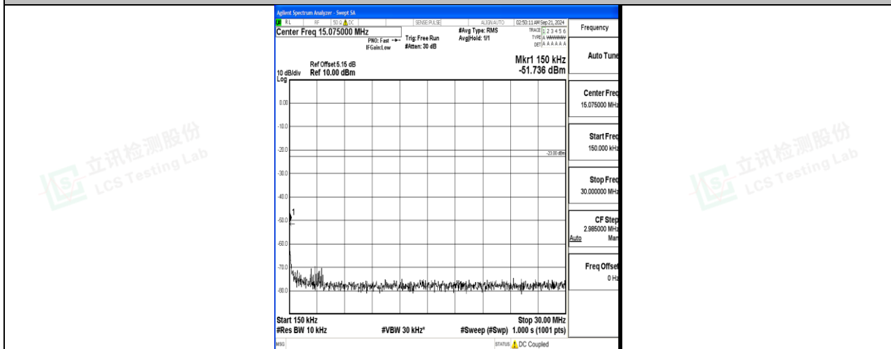
Band12_5MHz_16QAM_23155_1RB#0_0.15~30_0.15~30
