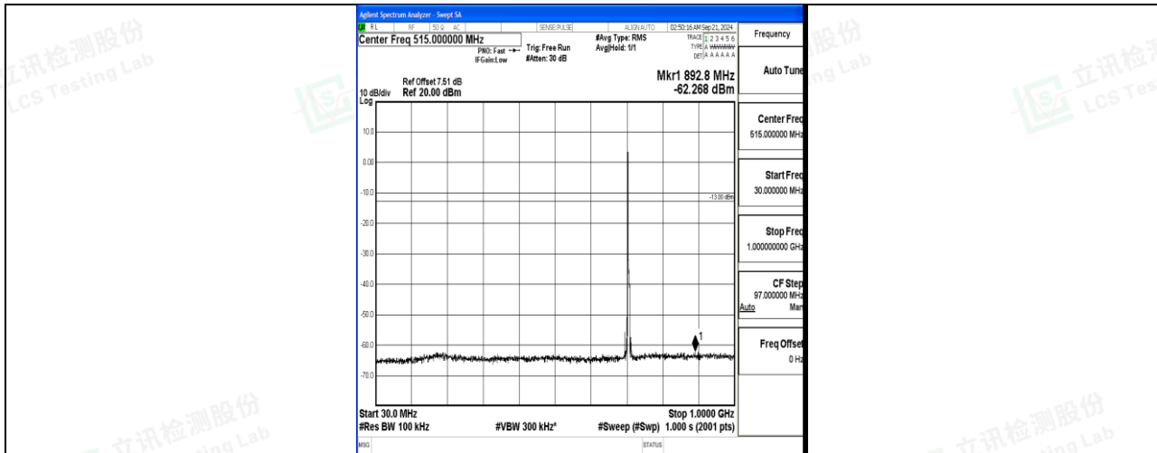
Band12_5MHz_16QAM_23155_1RB#0_30~1000_30~1000
