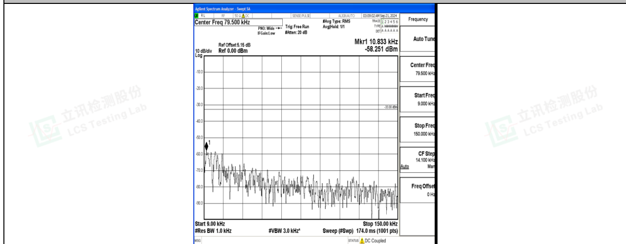
Band12_10MHz_16QAM_23060_1RB#0_0.009~0.15_0.009~0.15
