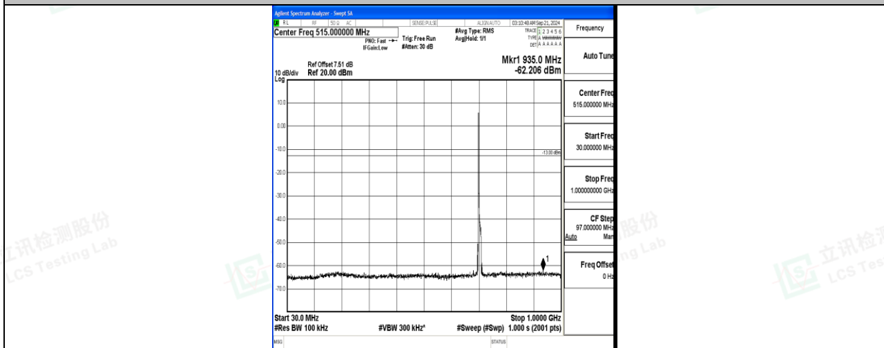
Band12_10MHz_QPSK_23130_1RB#0_30~1000_30~1000
