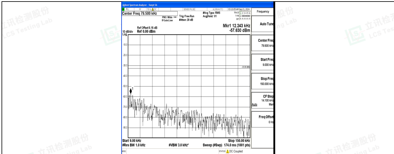
Band12_10MHz_16QAM_23095_1RB#0_0.009~0.15_0.009~0.15
