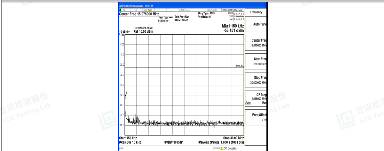
Band12_10MHz_16QAM_23095_1RB#0_0.15~30_0.15~30
