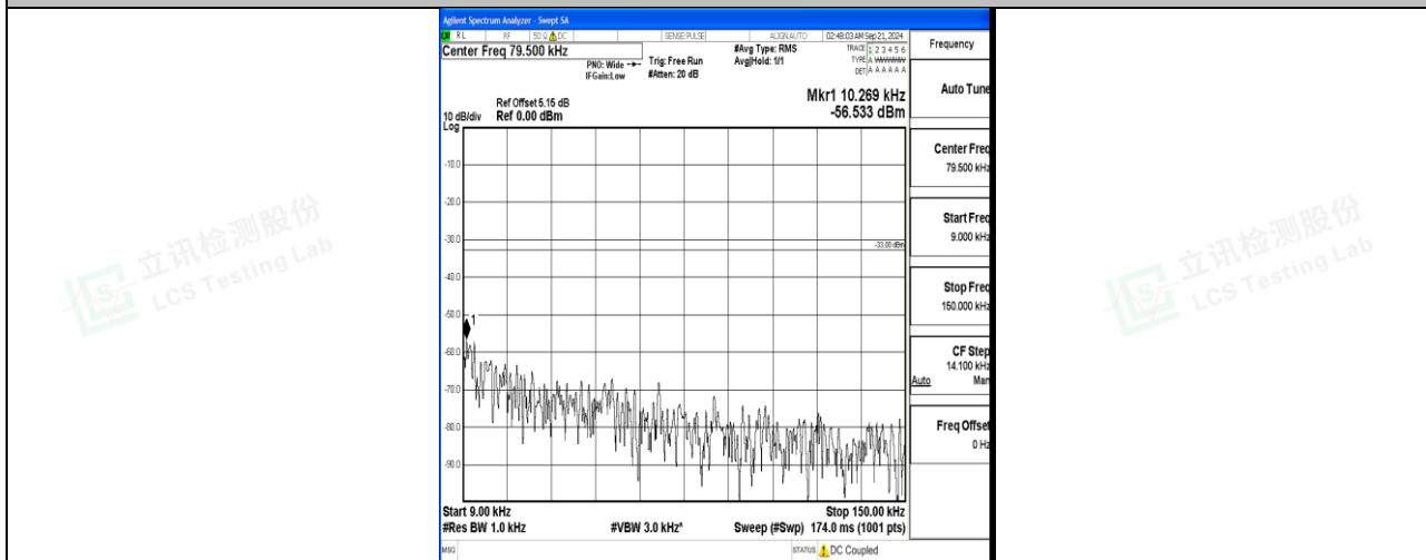
Band12_5MHz_16QAM_23035_1RB#0_0.009~0.15_0.009~0.15
