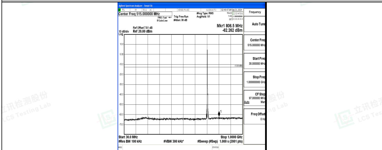
Band12_5MHz_QPSK_23155_1RB#0_30~1000_30~1000
