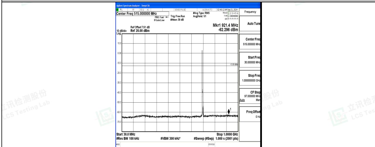
Band12_5MHz_16QAM_23035_1RB#0_30~1000_30~1000
