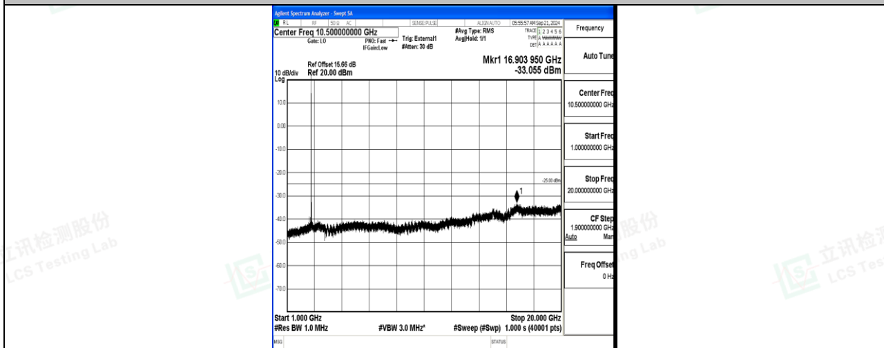
Band41_20MHz_16QAM_41490_1RB#0_1000~20000_1000~20000
