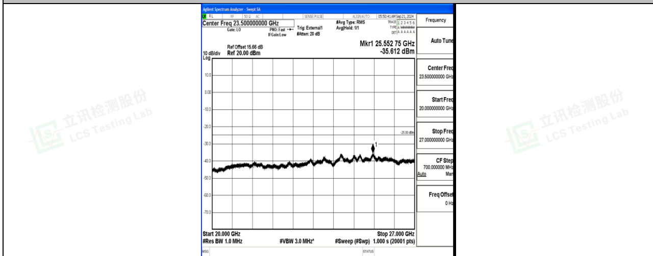
Band41_20MHz_QPSK_40620_1RB#0_20000~27000_20000~27000
