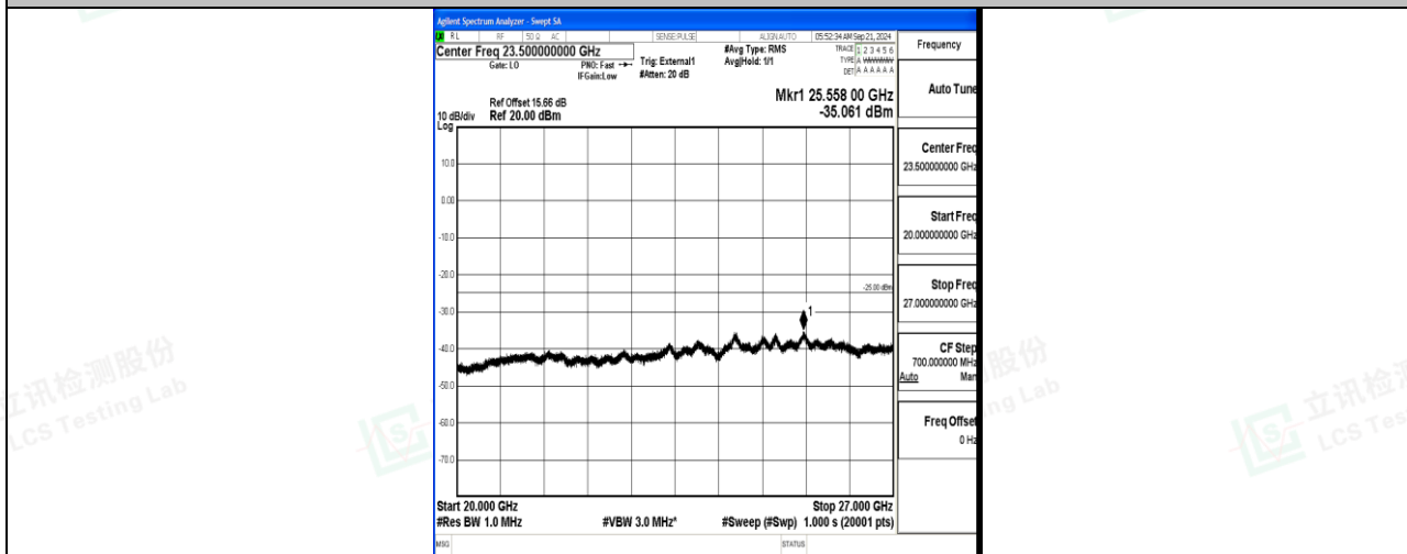
Band41_20MHz_16QAM_40620_1RB#0_20000~27000_20000~27000
