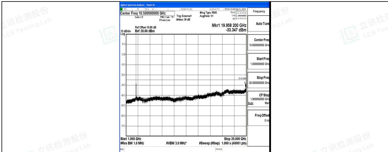
Band41_20MHz_16QAM_40620_1RB#0_1000~20000_1000~20000
