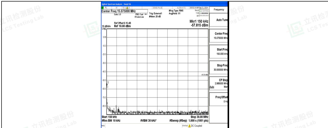
Band41_20MHz_QPSK_41490_1RB#0_0.15~30_0.15~30
