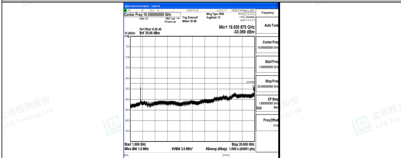
Band41_20MHz_QPSK_40620_1RB#0_1000~20000_1000~20000
