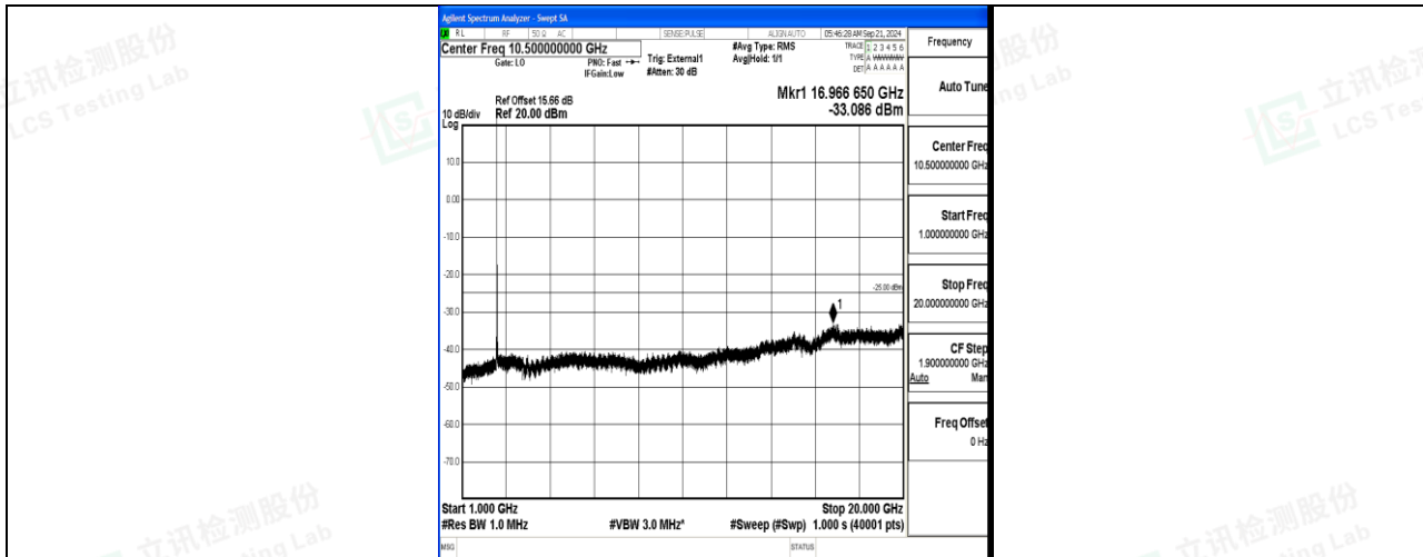
Band41_20MHz_QPSK_39750_1RB#0_1000~20000_1000~20000
