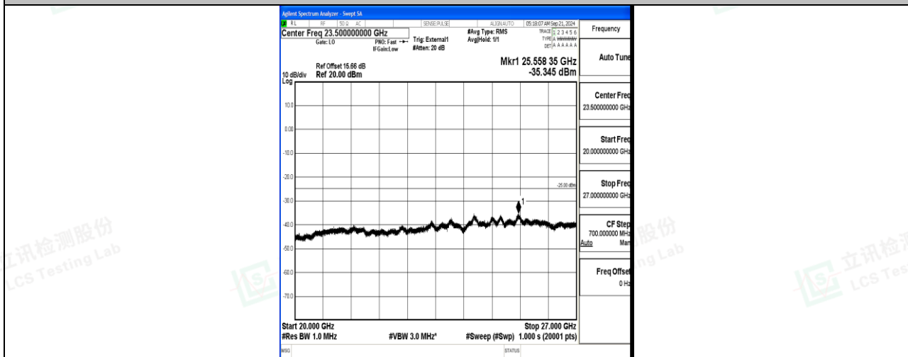
Band41_15MHz_QPSK_39725_1RB#0_20000~27000_20000~27000
