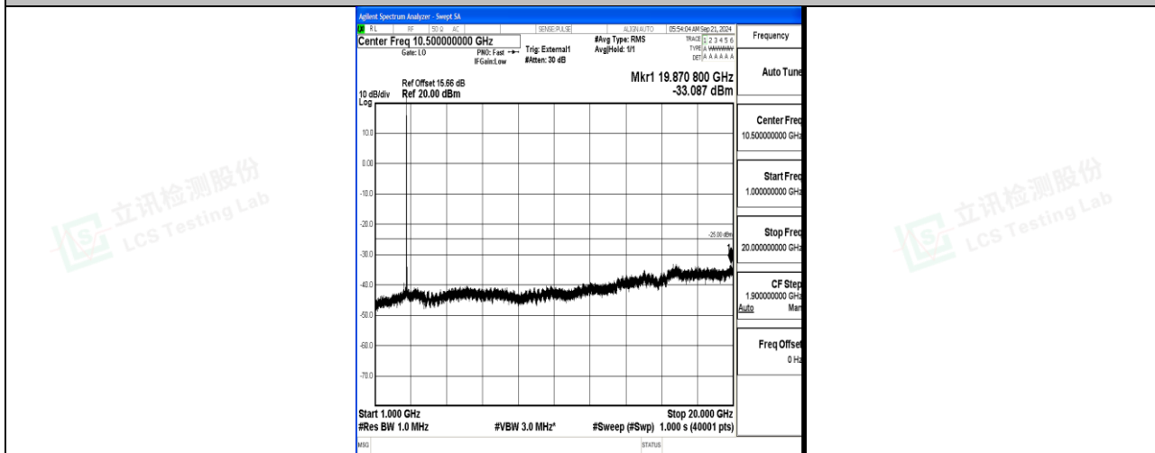
Band41_20MHz_QPSK_41490_1RB#0_1000~20000_1000~20000
