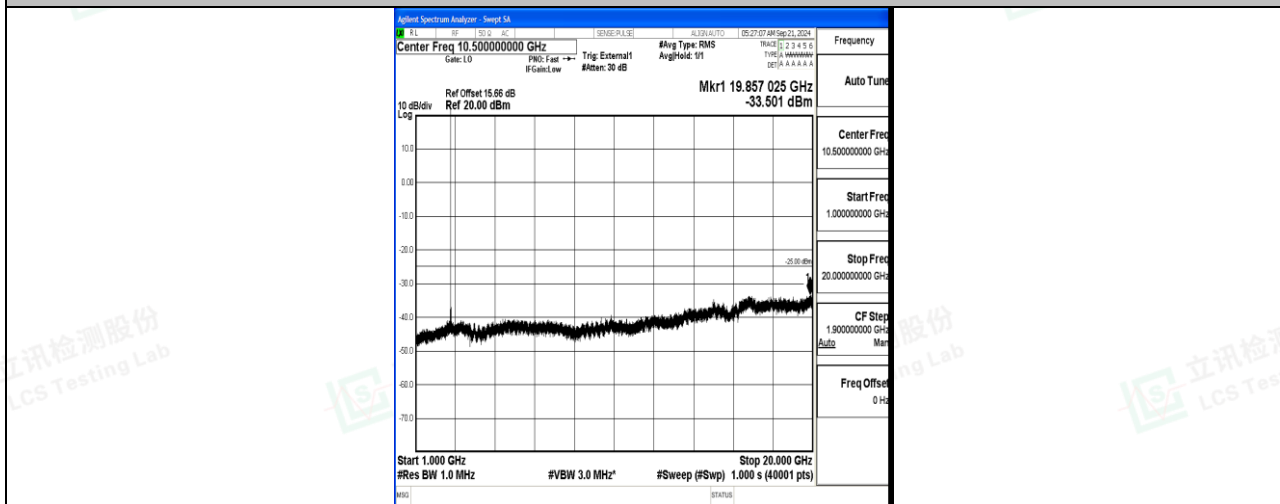
Band41_15MHz_16QAM_41515_1RB#0_1000~20000_1000~20000
