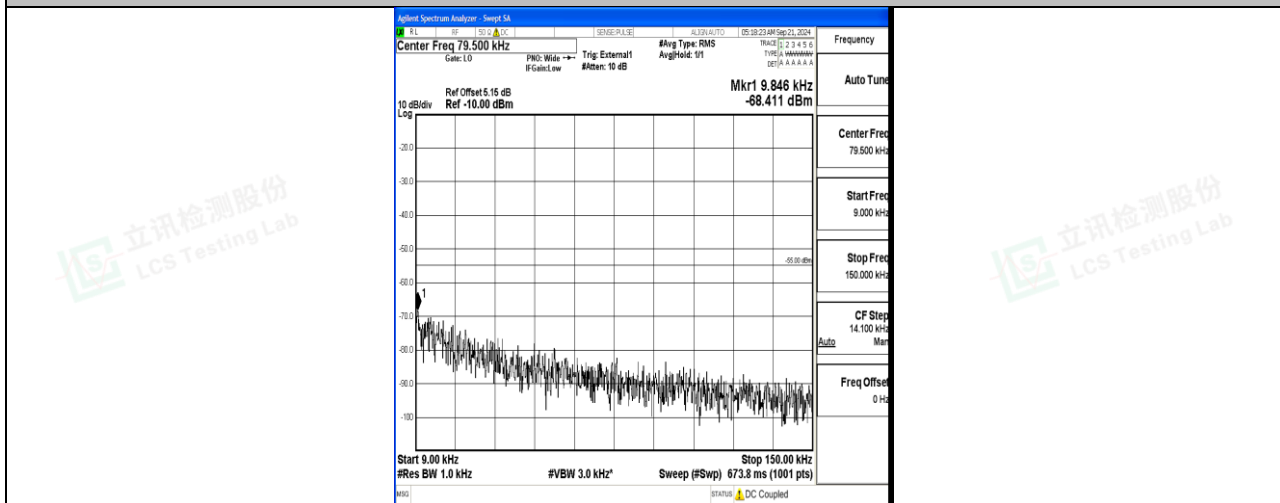
Band41_15MHz_16QAM_39725_1RB#0_0.009~0.15_0.009~0.15
