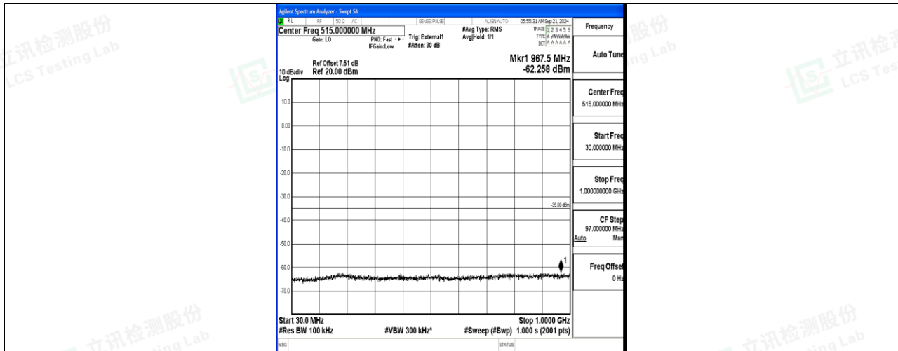
Band41_20MHz_16QAM_41490_1RB#0_30~1000_30~1000
