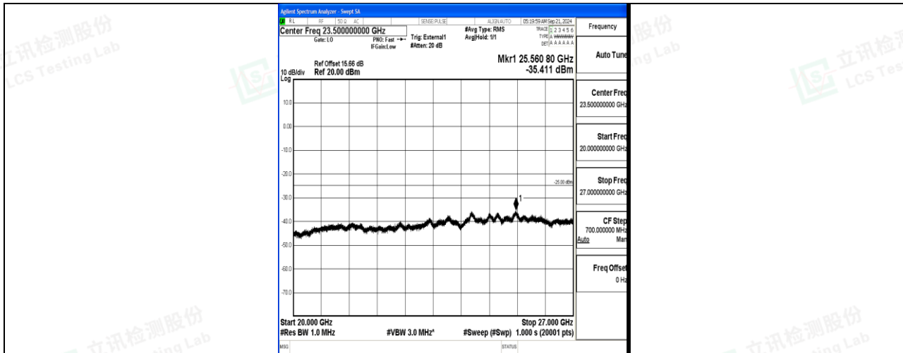
Band41_15MHz_16QAM_39725_1RB#0_20000~27000_20000~27000
