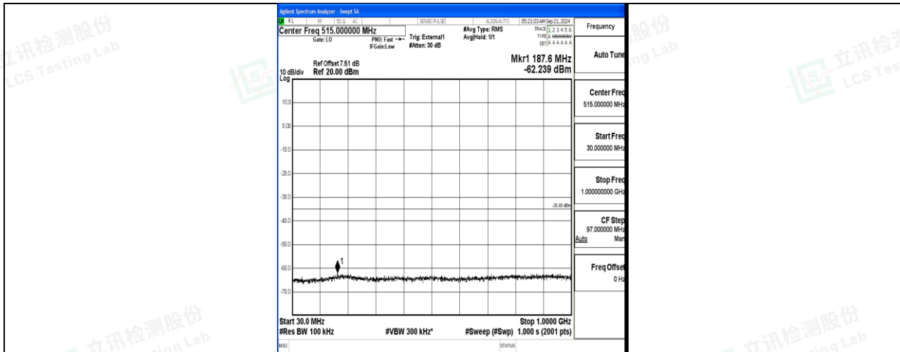
Band41_15MHz_QPSK_40620_1RB#0_30~1000_30~1000
