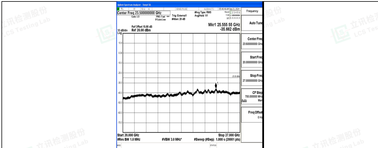
Band41_20MHz_16QAM_39750_1RB#0_20000~27000_20000~27000
