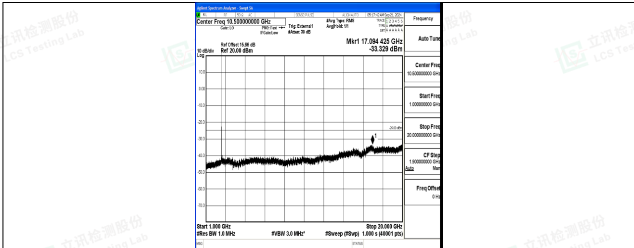
Band41_15MHz_QPSK_39725_1RB#0_1000~20000_1000~20000
