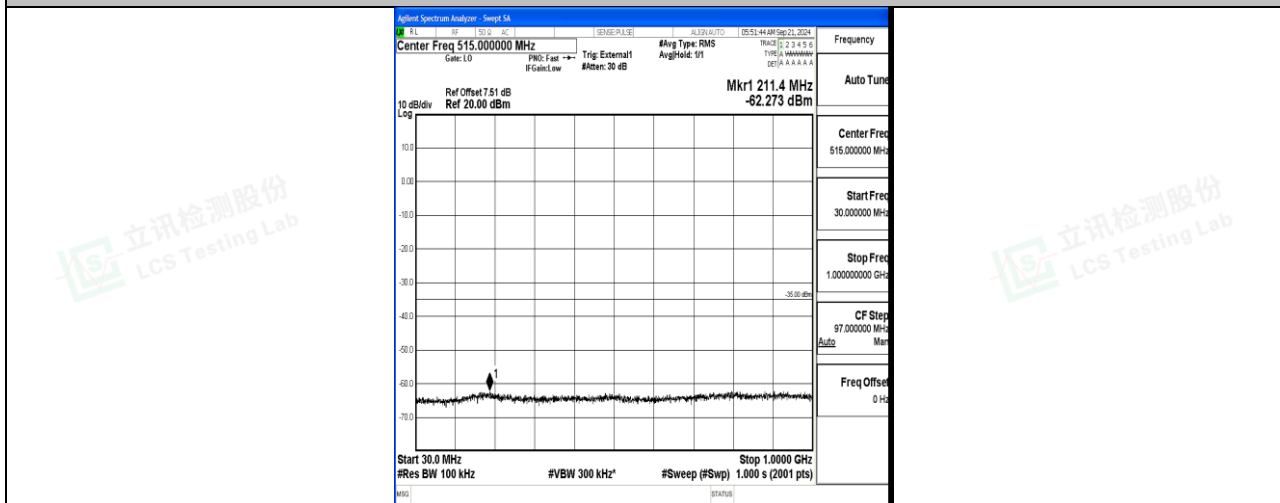
Band41_20MHz_16QAM_40620_1RB#0_30~1000_30~1000
