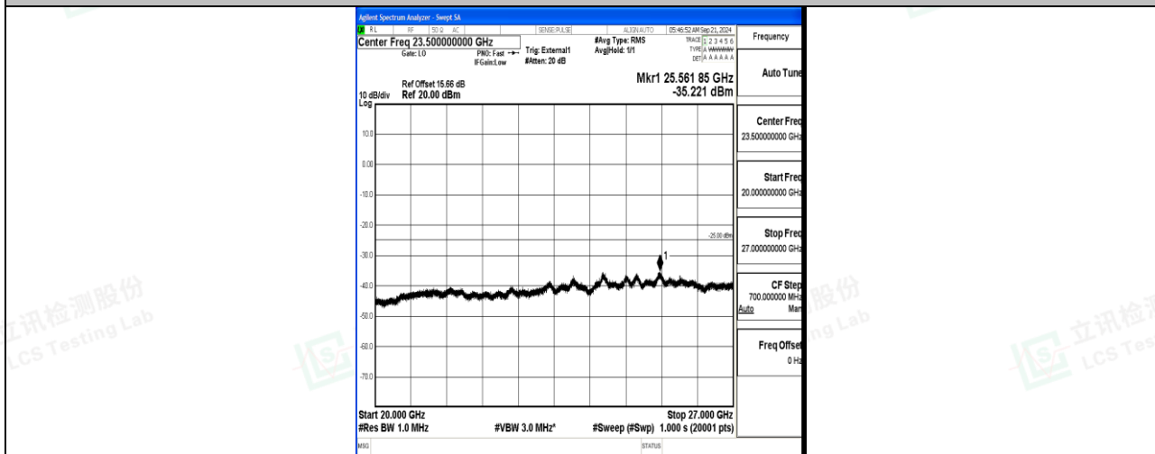
Band41_20MHz_QPSK_39750_1RB#0_20000~27000_20000~27000
