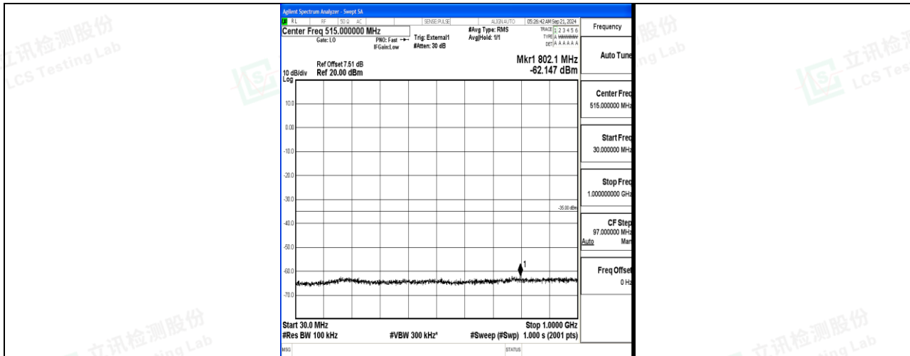
Band41_15MHz_16QAM_41515_1RB#0_30~1000_30~1000
