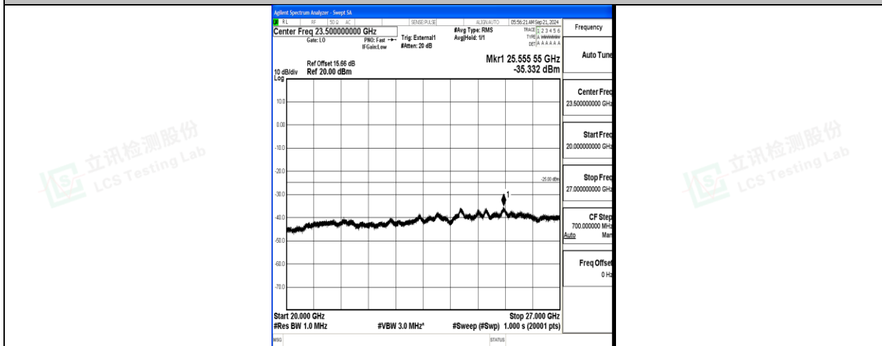
Band41_20MHz_16QAM_41490_1RB#0_20000~27000_20000~27000
