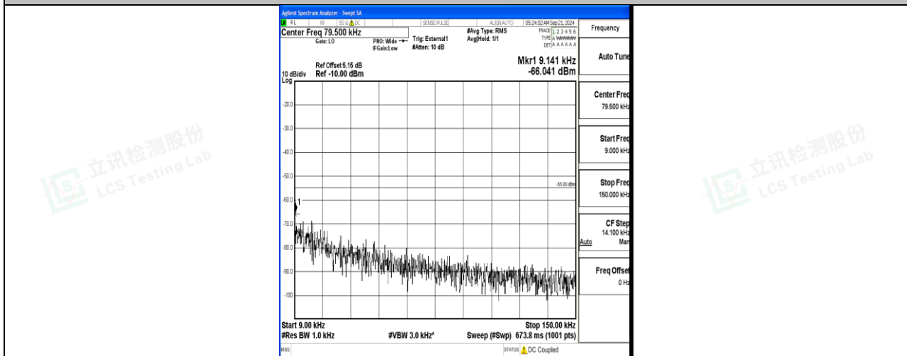
Band41_15MHz_QPSK_41515_1RB#0_0.009~0.15_0.009~0.15
