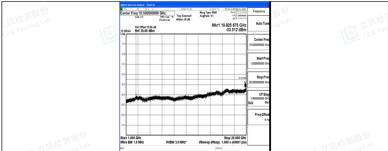
Band41_15MHz_16QAM_40620_1RB#0_1000~20000_1000~20000
