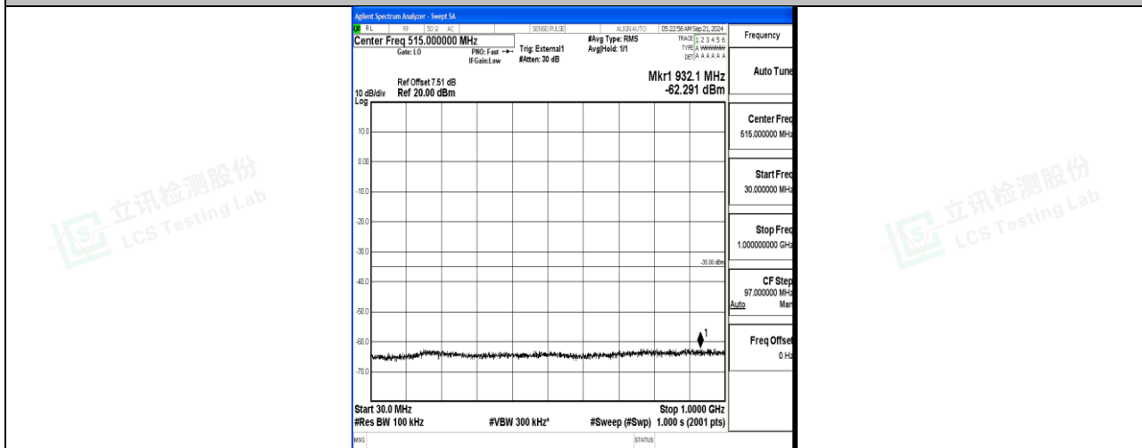
Band41_15MHz_16QAM_40620_1RB#0_30~1000_30~1000
