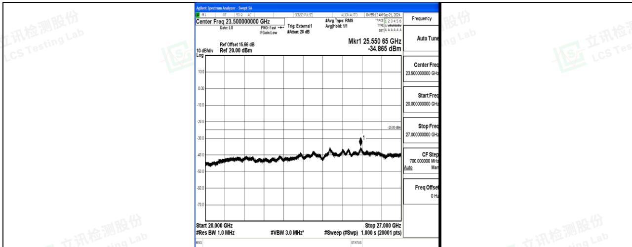
Band41_10MHz_QPSK_41540_1RB#0_20000~27000_20000~27000
