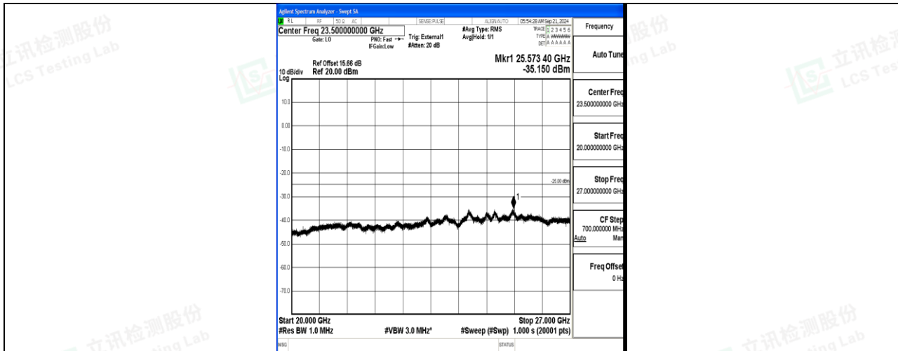
Band41_20MHz_QPSK_41490_1RB#0_20000~27000_20000~27000
