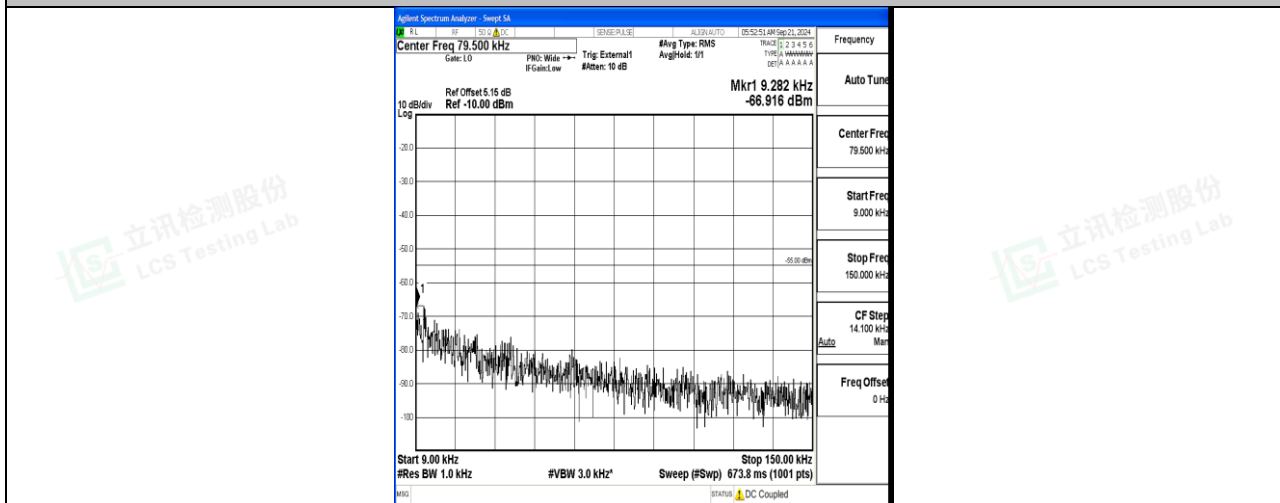
Band41_20MHz_QPSK_41490_1RB#0_0.009~0.15_0.009~0.15
