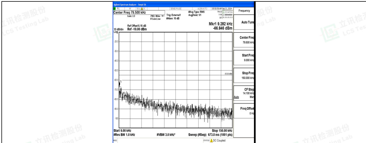
Band41_20MHz_16QAM_40620_1RB#0_0.009~0.15_0.009~0.15
