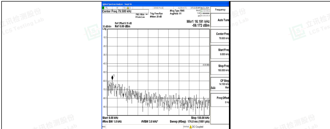
Band66_10MHz_QPSK_132322_1RB#0_0.009~0.15_0.009~0.15
