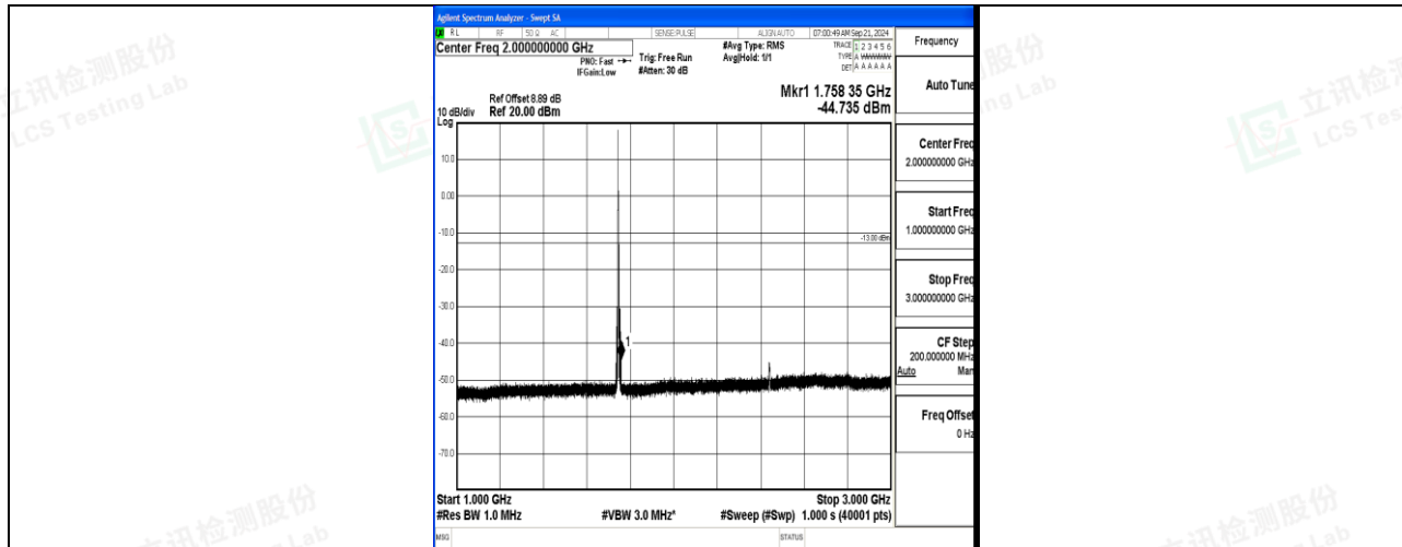
Band66_5MHz_QPSK_132322_1RB#0_1000~3000_1000~3000
