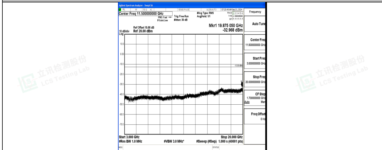
Band66_10MHz_16QAM_132022_1RB#0_3000~20000_3000~20000
