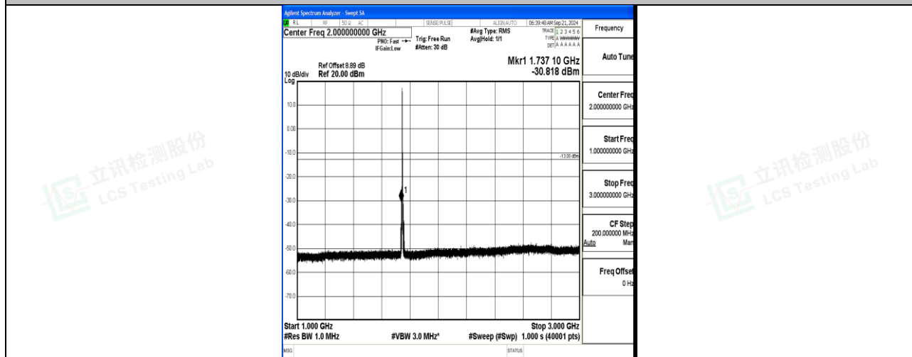
Band66_3MHz_16QAM_132322_1RB#0_1000~3000_1000~3000
