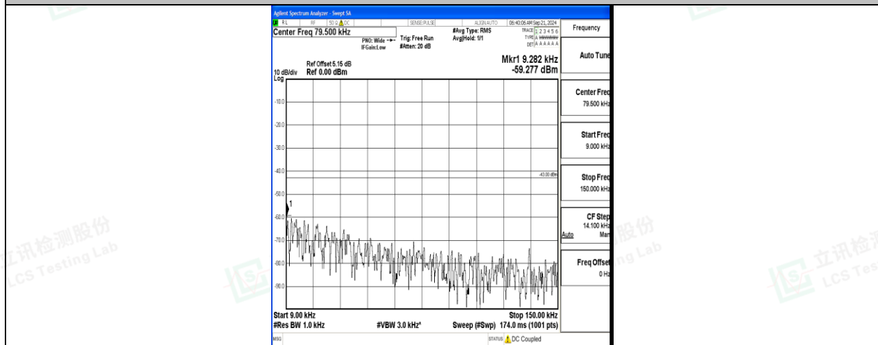
Band66_3MHz_QPSK_132657_1RB#0_0.009~0.15_0.009~0.15
