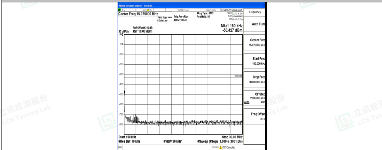
Band66_10MHz_QPSK_132322_1RB#0_0.15~30_0.15~30
