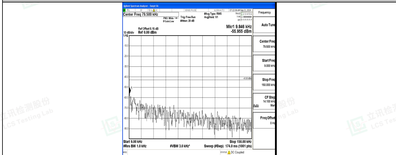
Band66_10MHz_QPSK_132622_1RB#0_0.009~0.15_0.009~0.15
