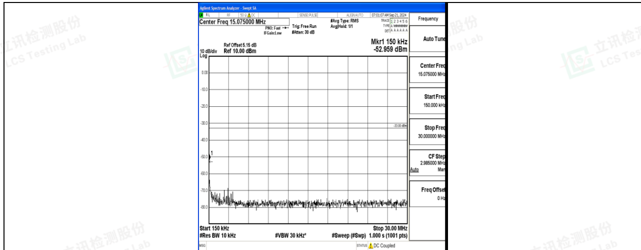
Band66_5MHz_16QAM_132322_1RB#0_0.15~30_0.15~30
