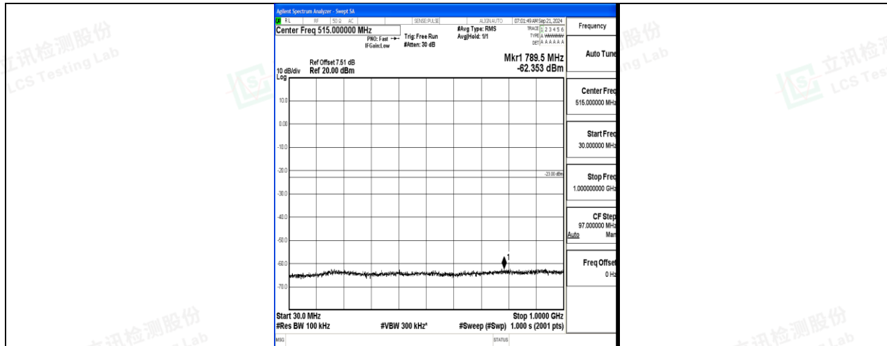
Band66_5MHz_QPSK_132647_1RB#0_30~1000_30~1000
