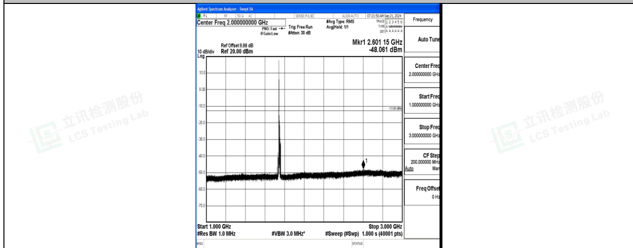
Band66_10MHz_16QAM_132322_1RB#0_1000~3000_1000~3000
