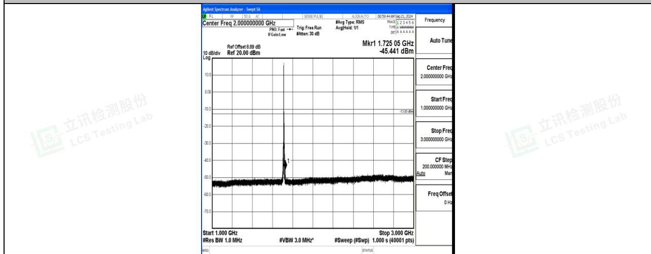
Band66_5MHz_QPSK_131997_1RB#0_1000~3000_1000~3000
