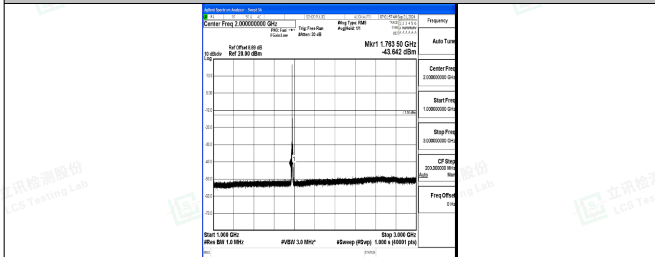
Band66_5MHz_QPSK_132647_1RB#0_1000~3000_1000~3000
