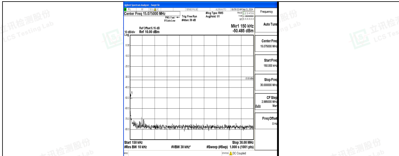
Band66_5MHz_QPSK_131997_1RB#0_0.15~30_0.15~30
