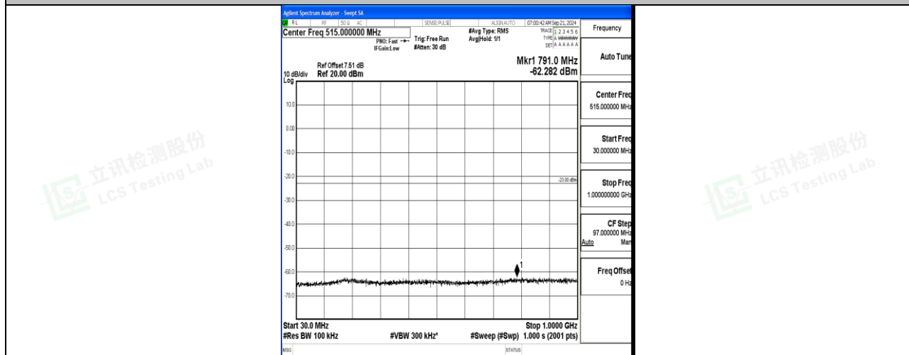
Band66_5MHz_QPSK_132322_1RB#0_30~1000_30~1000
