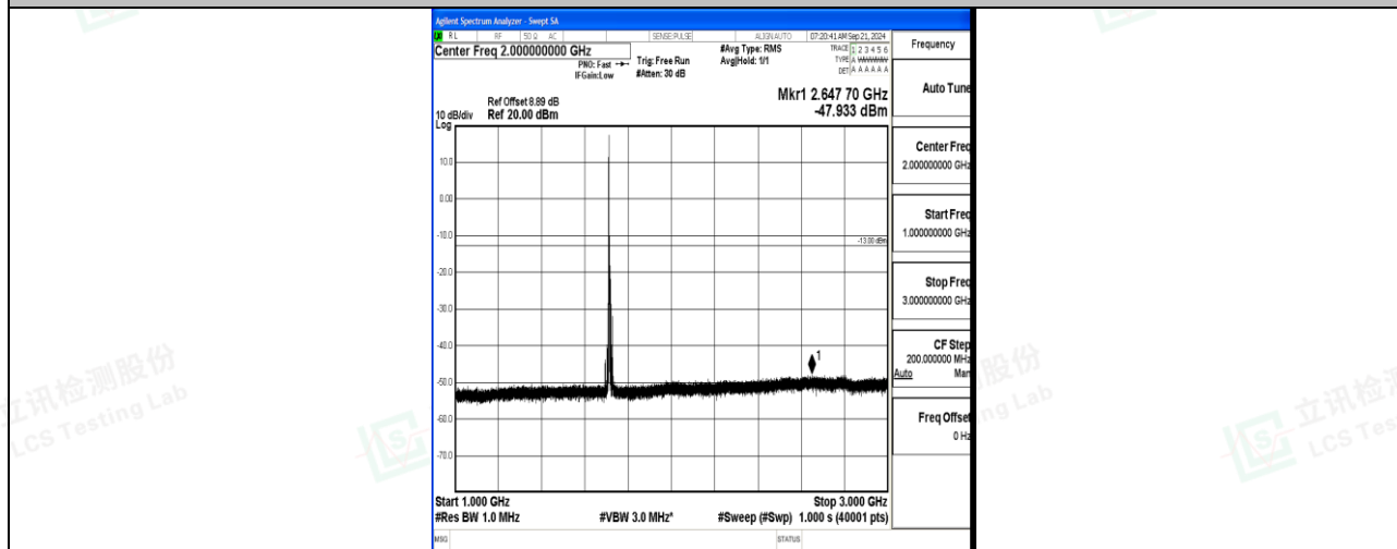
Band66_10MHz_16QAM_132022_1RB#0_1000~3000_1000~3000
