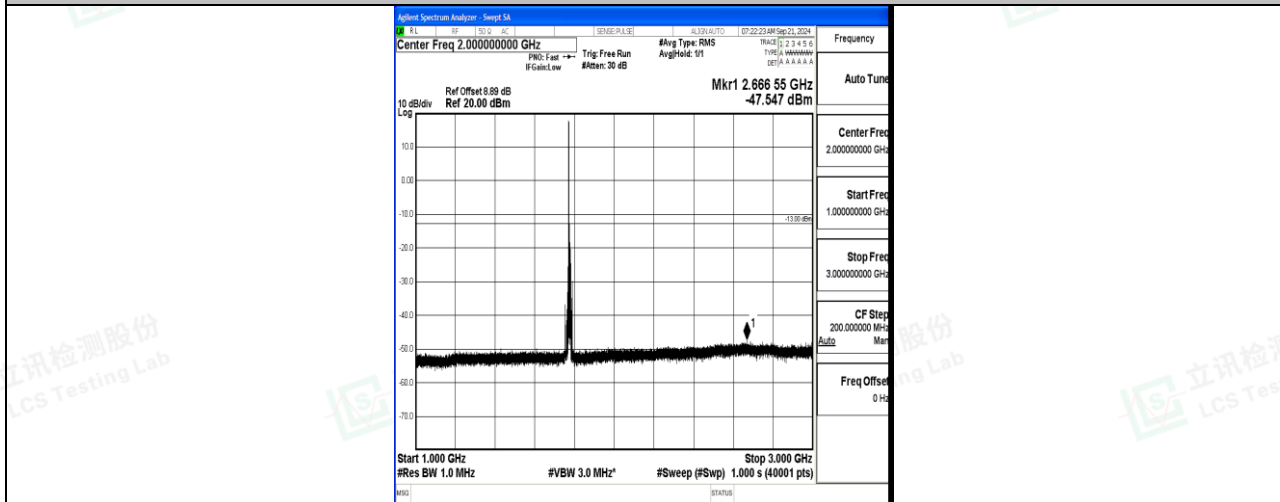
Band66_10MHz_QPSK_132622_1RB#0_1000~3000_1000~3000
