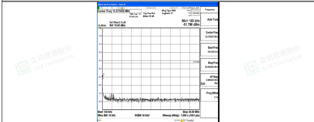
Band66_10MHz_QPSK_132622_1RB#0_0.15~30_0.15~30
