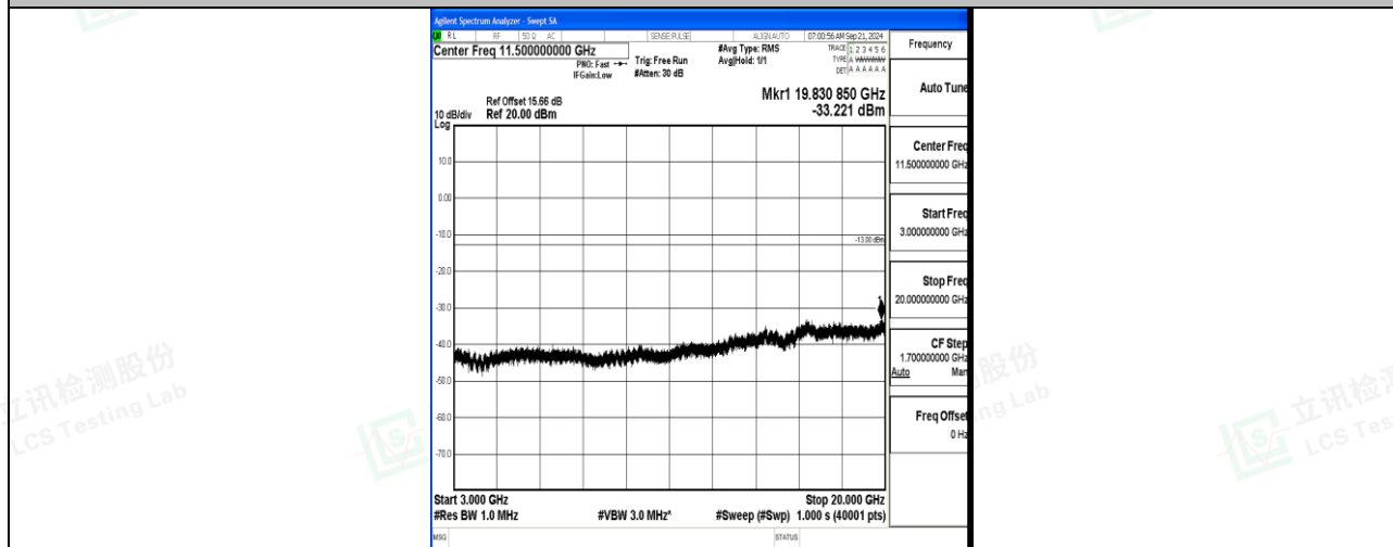
Band66_5MHz_QPSK_132322_1RB#0_3000~20000_3000~20000
