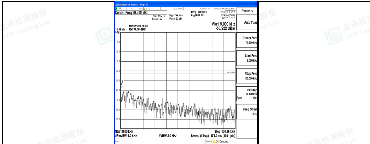
Band66_5MHz_QPSK_132322_1RB#0_0.009~0.15_0.009~0.15
