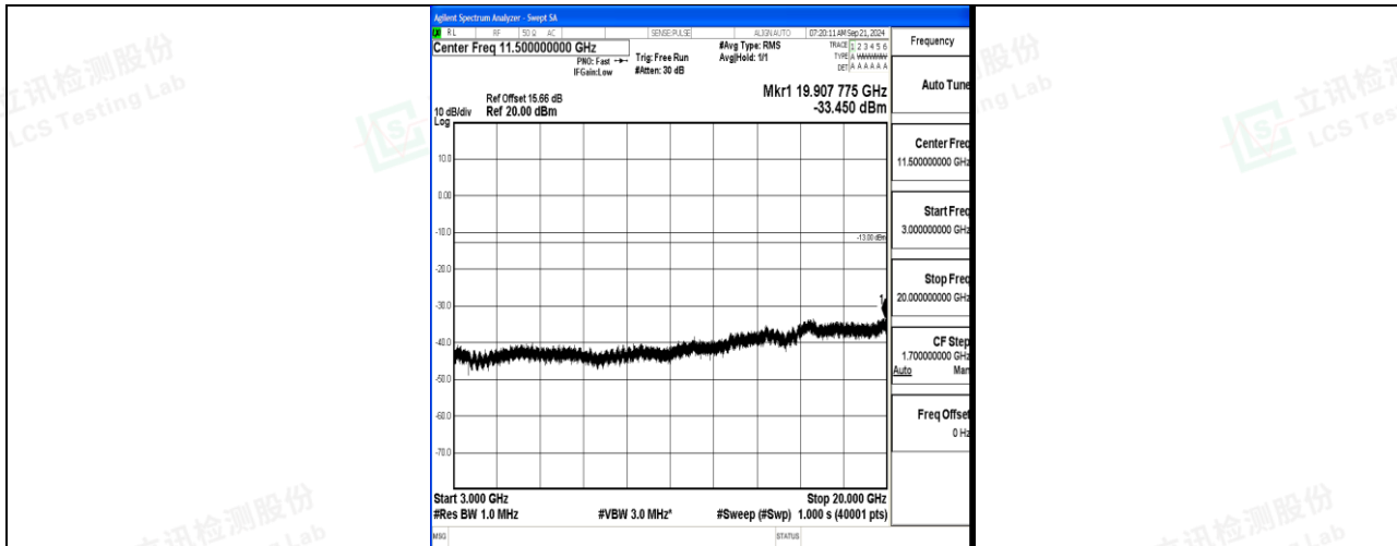
Band66_10MHz_QPSK_132022_1RB#0_3000~20000_3000~20000
