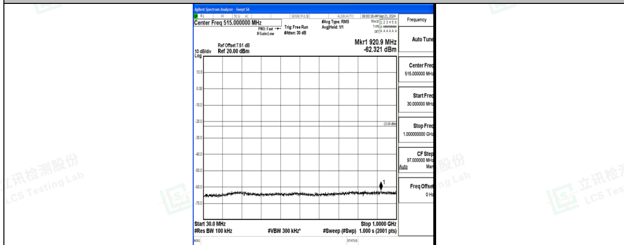
Band66_20MHz_16QAM_132322_1RB#0_30~1000_30~1000
