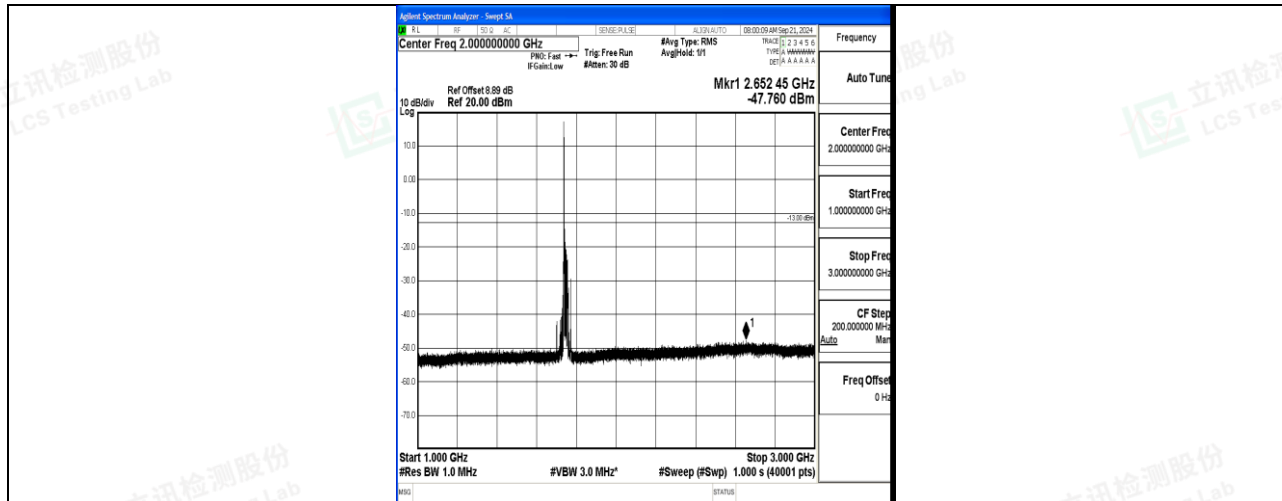
Band66_20MHz_QPSK_132322_1RB#0_1000~3000_1000~3000
