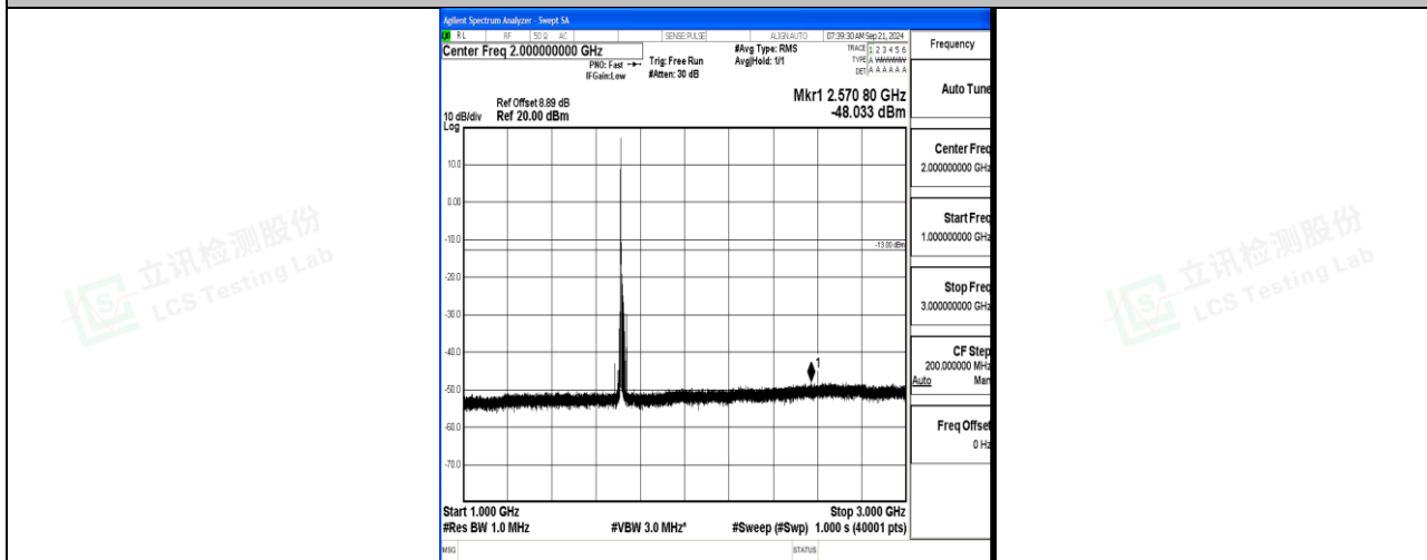
Band66_15MHz_QPSK_132047_1RB#0_1000~3000_1000~3000
