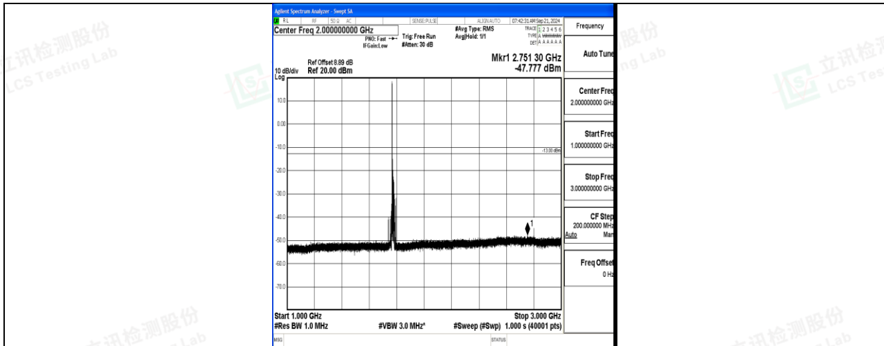
Band66_15MHz_16QAM_132597_1RB#0_1000~3000_1000~3000
