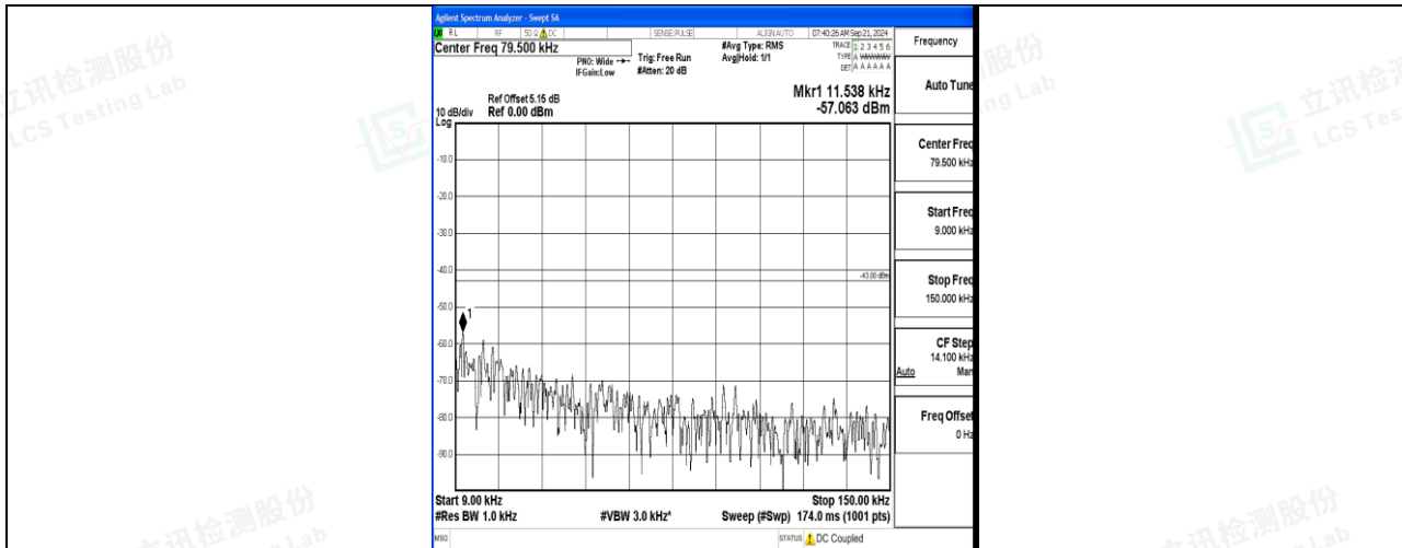
Band66_15MHz_QPSK_132322_1RB#0_0.009~0.15_0.009~0.15
