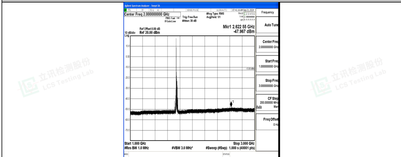
Band66_15MHz_16QAM_132322_1RB#0_1000~3000_1000~3000
