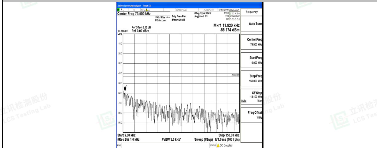
Band66_20MHz_16QAM_132072_1RB#0_0.009~0.15_0.009~0.15
