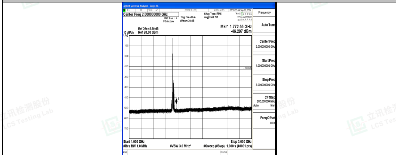
Band66_20MHz_16QAM_132072_1RB#0_1000~3000_1000~3000
