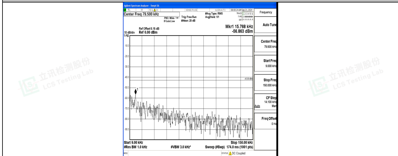
Band66_20MHz_16QAM_132322_1RB#0_0.009~0.15_0.009~0.15
