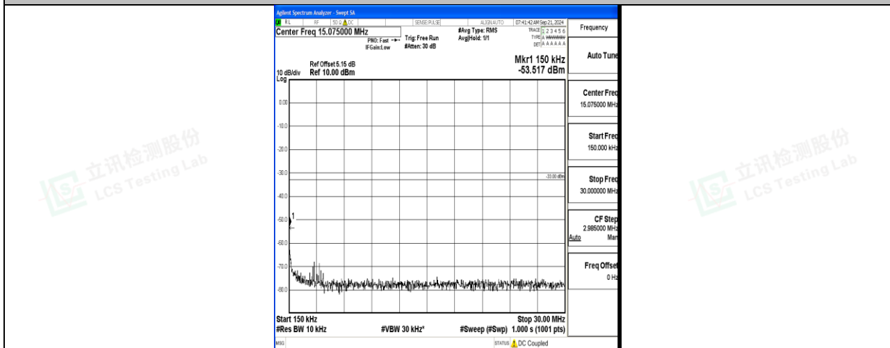
Band66_15MHz_QPSK_132597_1RB#0_0.15~30_0.15~30
