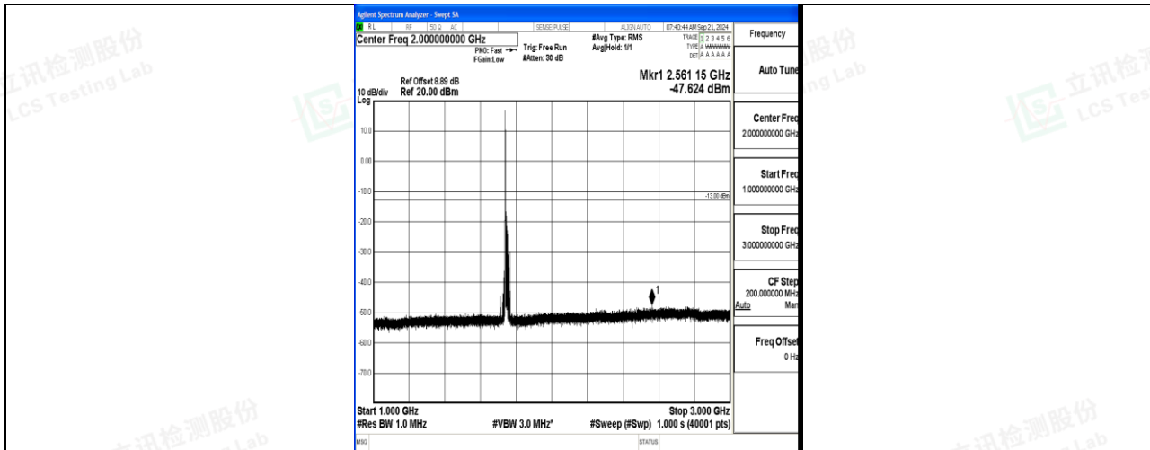
Band66_15MHz_QPSK_132322_1RB#0_1000~3000_1000~3000
