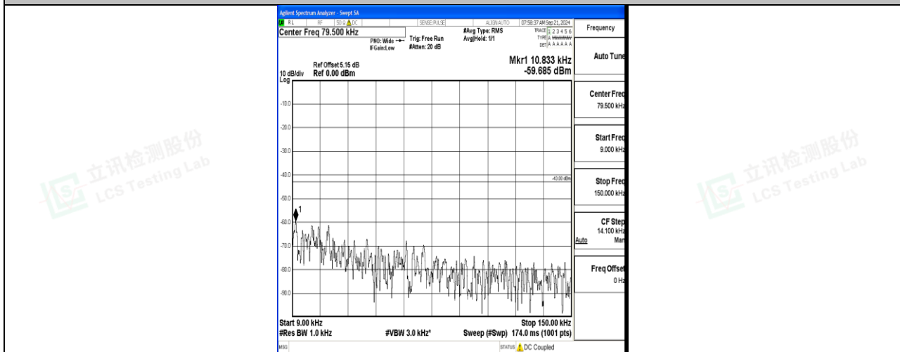
Band66_20MHz_QPSK_132072_1RB#0_0.009~0.15_0.009~0.15
