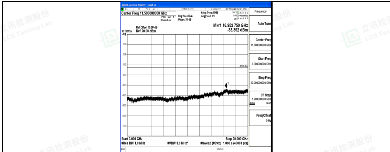
Band66_20MHz_QPSK_132072_1RB#0_3000~20000_3000~20000
