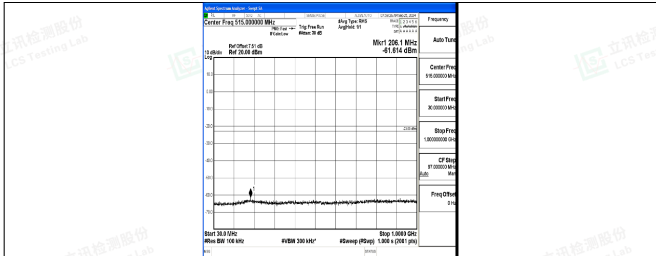
Band66_20MHz_16QAM_132072_1RB#0_30~1000_30~1000
