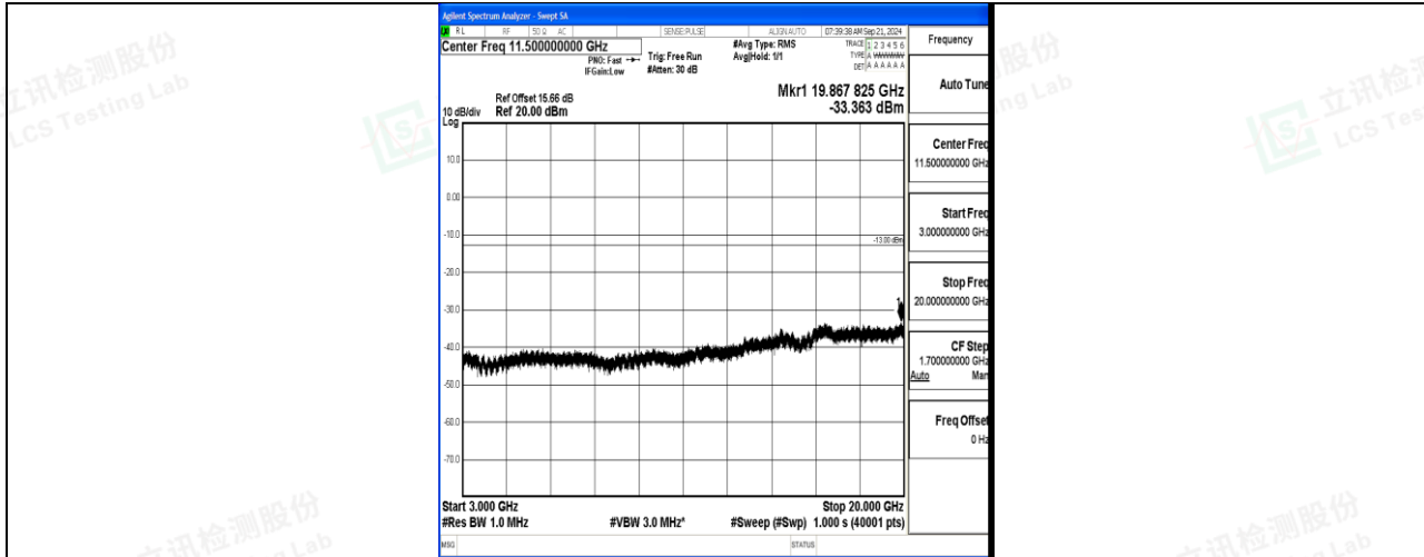
Band66_15MHz_QPSK_132047_1RB#0_3000~20000_3000~20000
