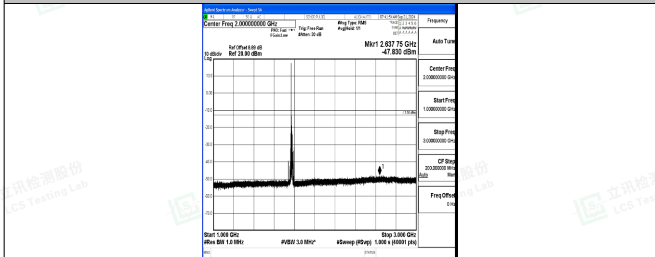
Band66_15MHz_QPSK_132597_1RB#0_1000~3000_1000~3000
