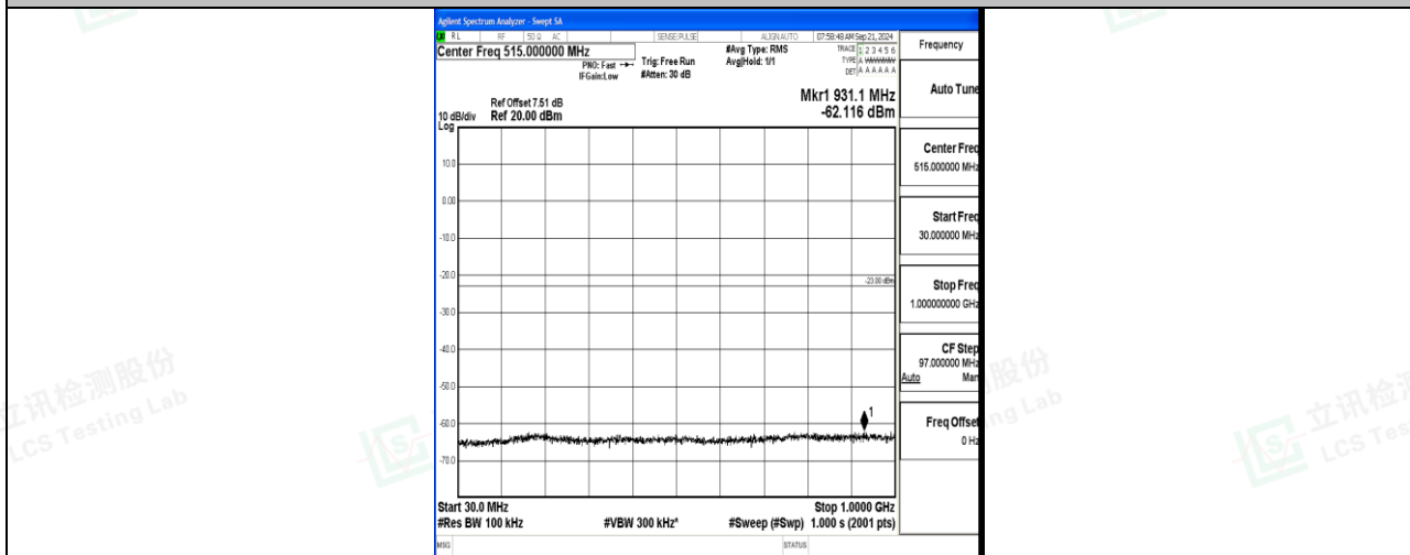
Band66_20MHz_QPSK_132072_1RB#0_30~1000_30~1000
