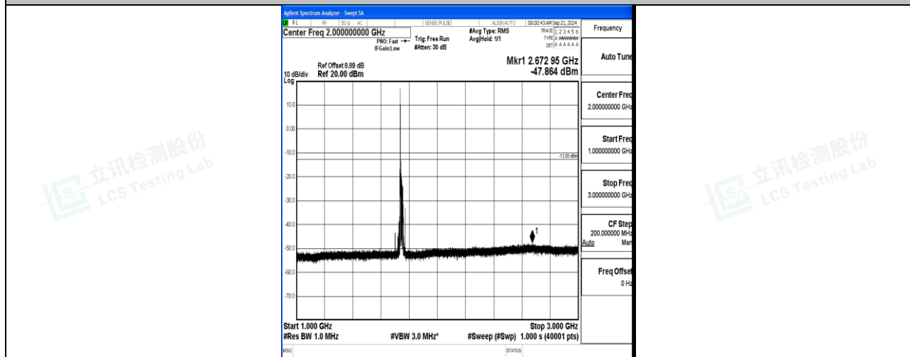
Band66_20MHz_16QAM_132322_1RB#0_1000~3000_1000~3000
