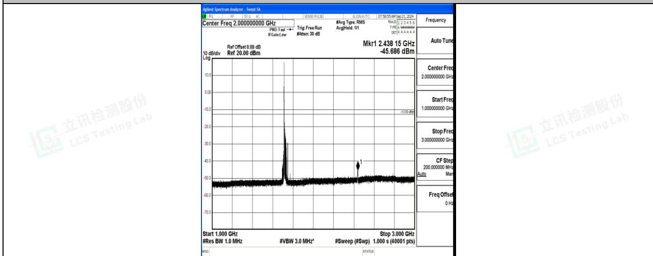
Band66_20MHz_QPSK_132072_1RB#0_1000~3000_1000~3000
