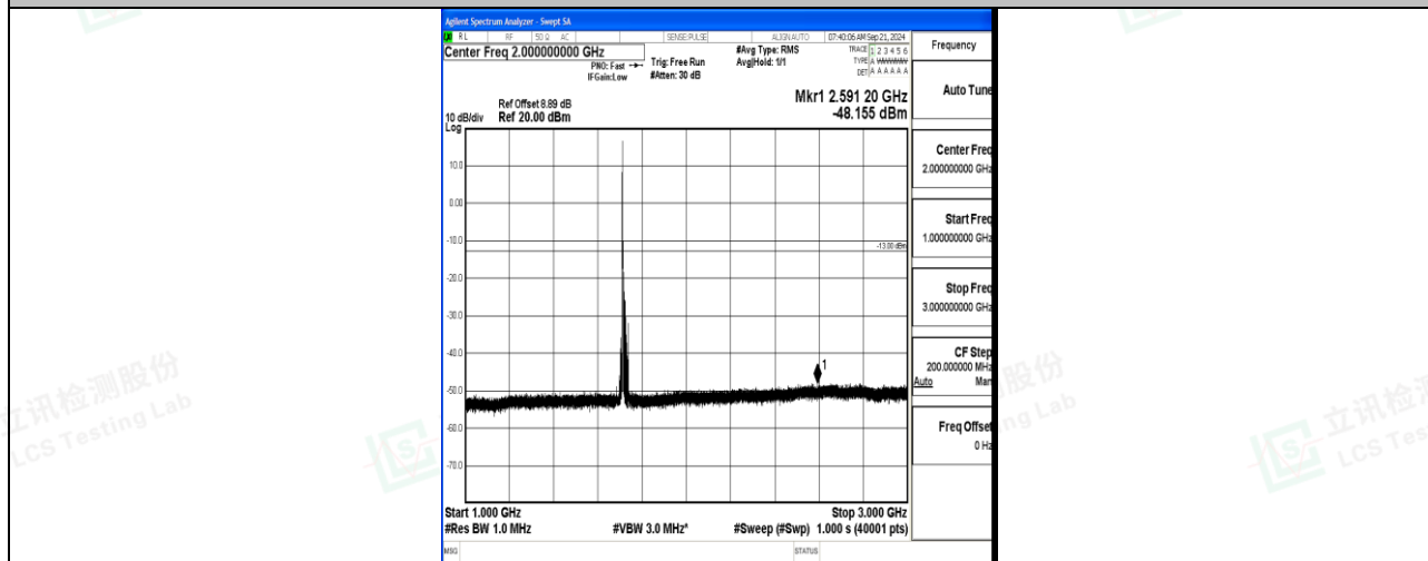
Band66_15MHz_16QAM_132047_1RB#0_1000~3000_1000~3000
