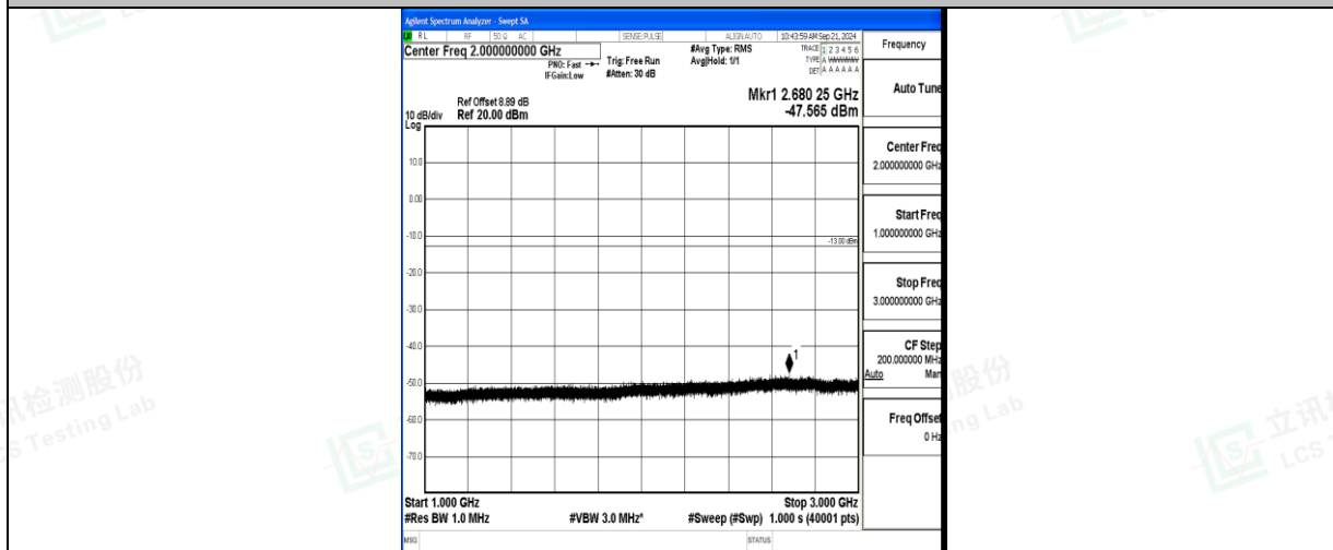
Band71_20MHz_16QAM_133222_1RB#0_1000~3000_1000~3000
