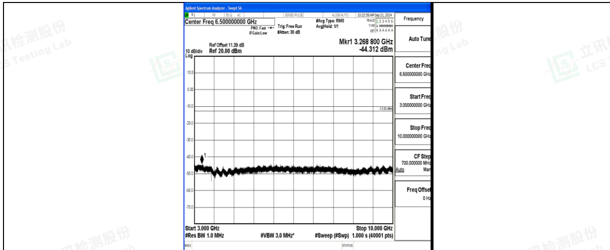
Band71_15MHz_QPSK_133397_1RB#0_3000~10000_3000~10000
