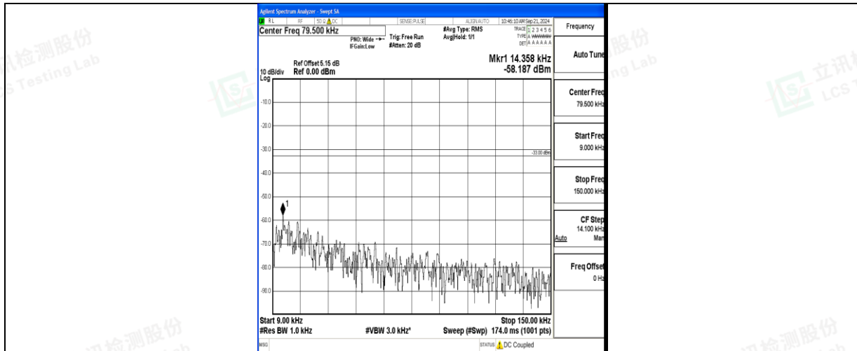
Band71_20MHz_16QAM_133322_1RB#0_0.009~0.15_0.009~0.15
