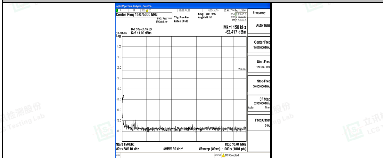
Band71_20MHz_16QAM_133322_1RB#0_0.15~30_0.15~30
