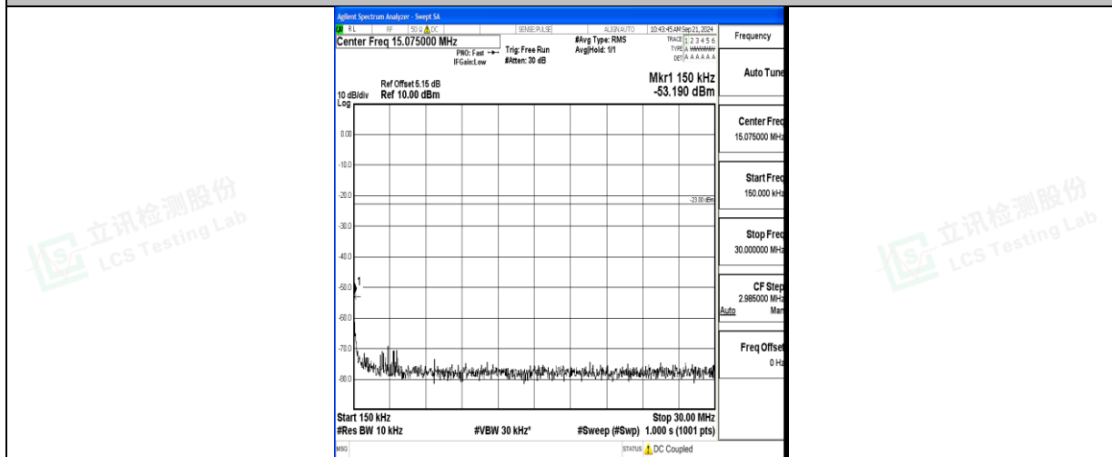
Band71_20MHz_16QAM_133222_1RB#0_0.15~30_0.15~30
