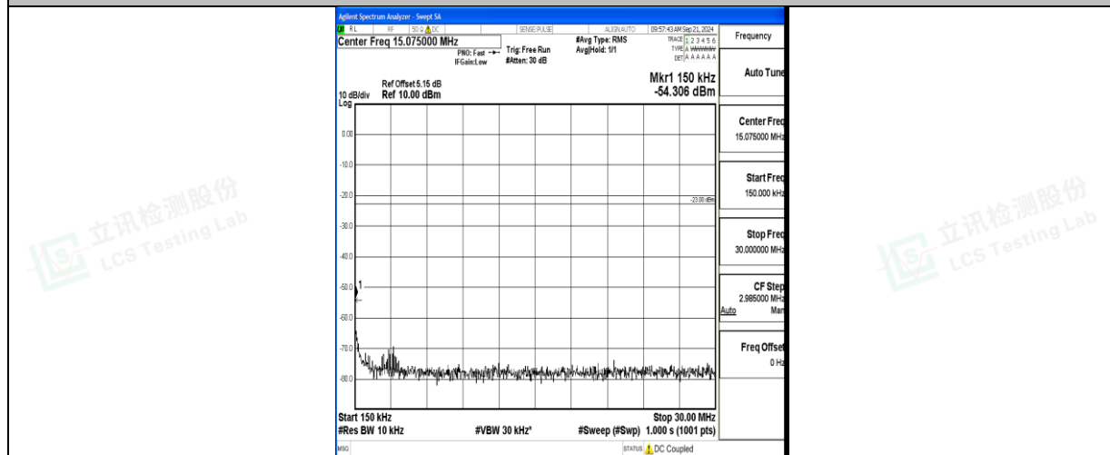
Band71_10MHz_16QAM_133422_1RB#0_0.15~30_0.15~30
