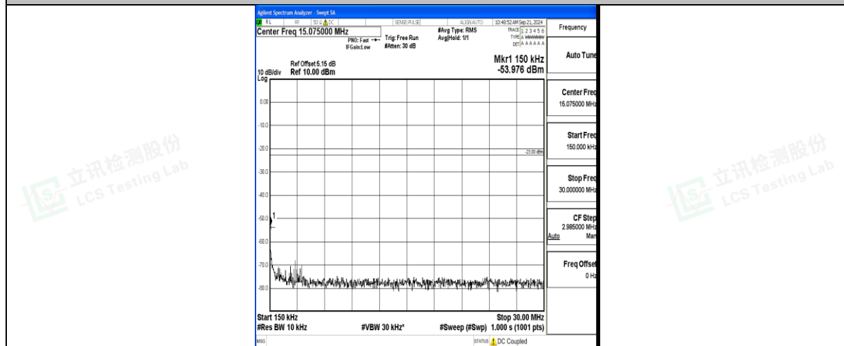
Band71_20MHz_16QAM_133372_1RB#0_0.15~30_0.15~30
