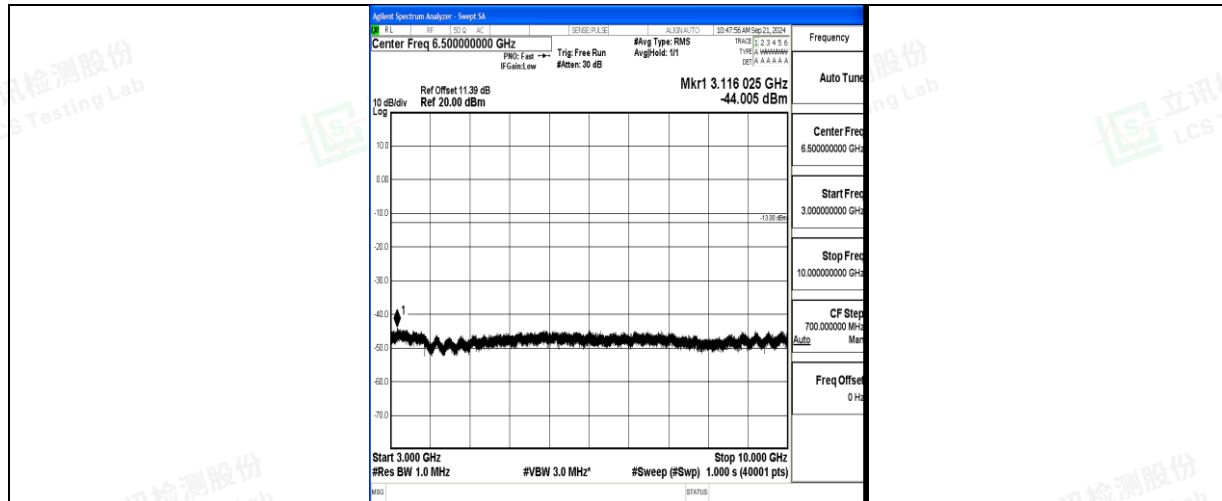
Band71_20MHz_QPSK_133372_1RB#0_3000~10000_3000~10000
