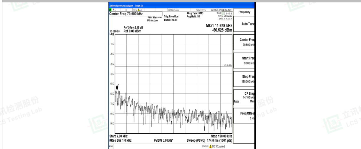
Band71_20MHz_16QAM_133222_1RB#0_0.009~0.15_0.009~0.15
