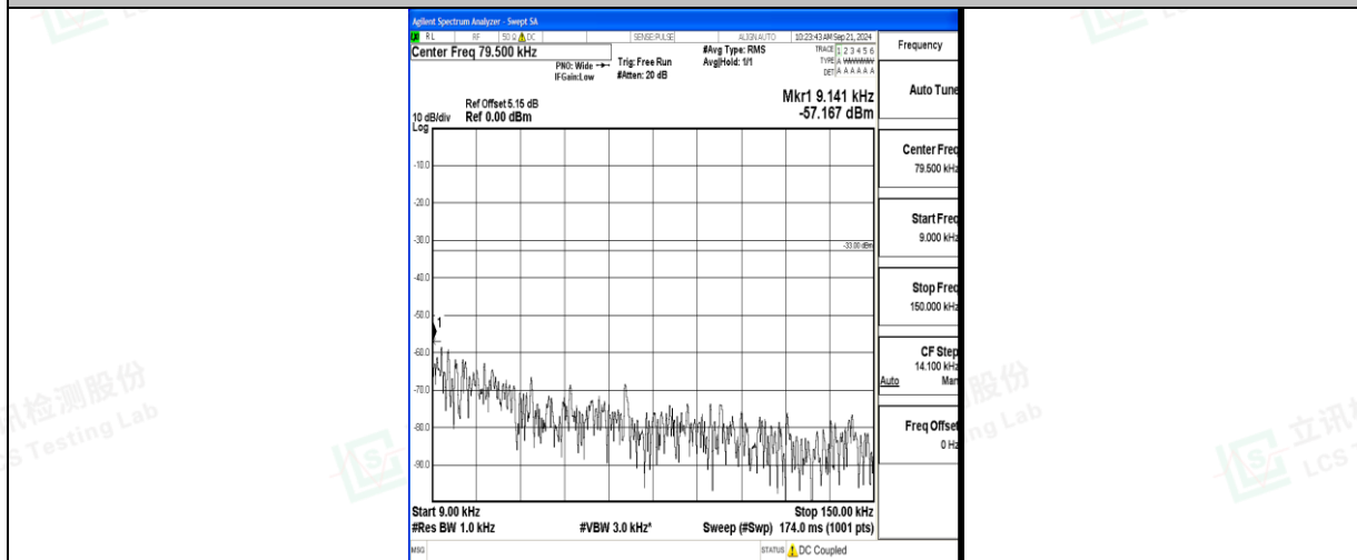
Band71_15MHz_16QAM_133397_1RB#0_0.009~0.15_0.009~0.15
