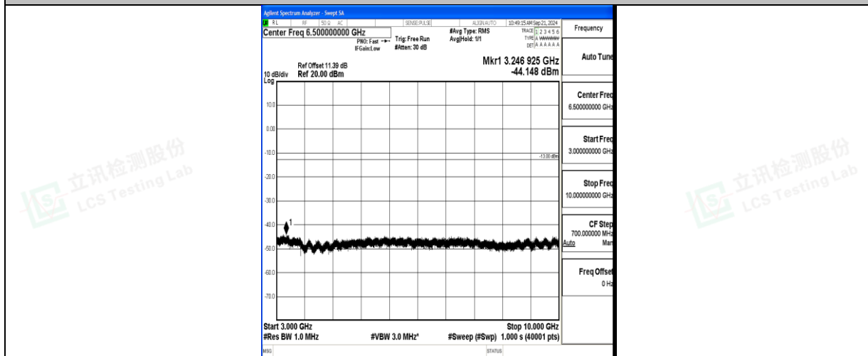
Band71_20MHz_16QAM_133372_1RB#0_3000~10000_3000~10000
