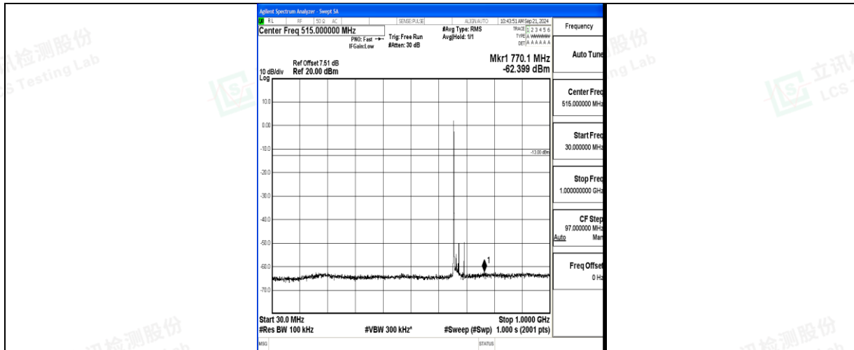
Band71_20MHz_16QAM_133222_1RB#0_30~1000_30~1000
