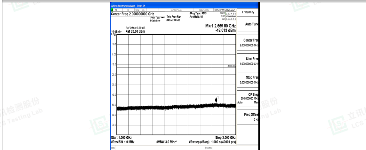
Band71_20MHz_16QAM_133372_1RB#0_1000~3000_1000~3000
