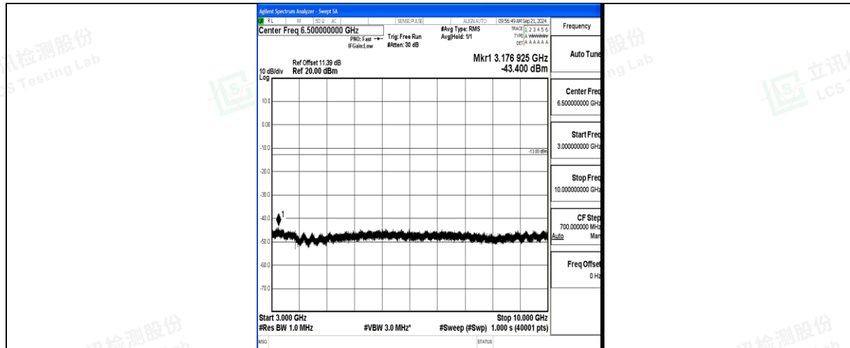
Band71_10MHz_QPSK_133422_1RB#0_3000~10000_3000~10000
