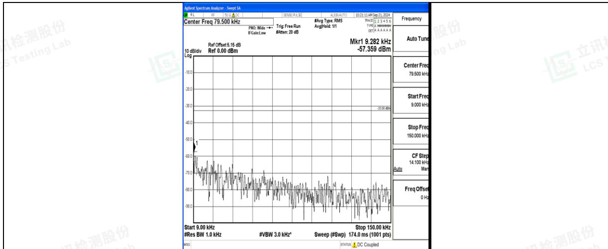
Band71_15MHz_16QAM_133297_1RB#0_0.009~0.15_0.009~0.15
