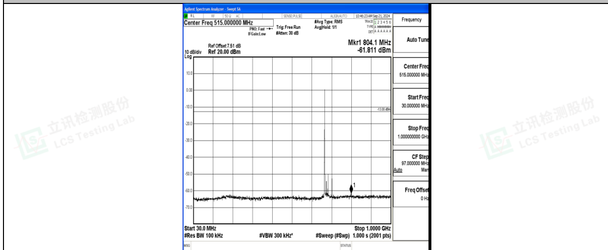
Band71_20MHz_16QAM_133322_1RB#0_30~1000_30~1000
