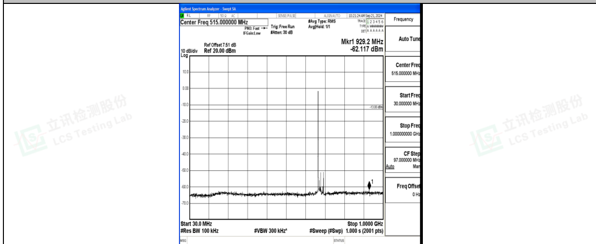
Band71_15MHz_16QAM_133297_1RB#0_30~1000_30~1000
