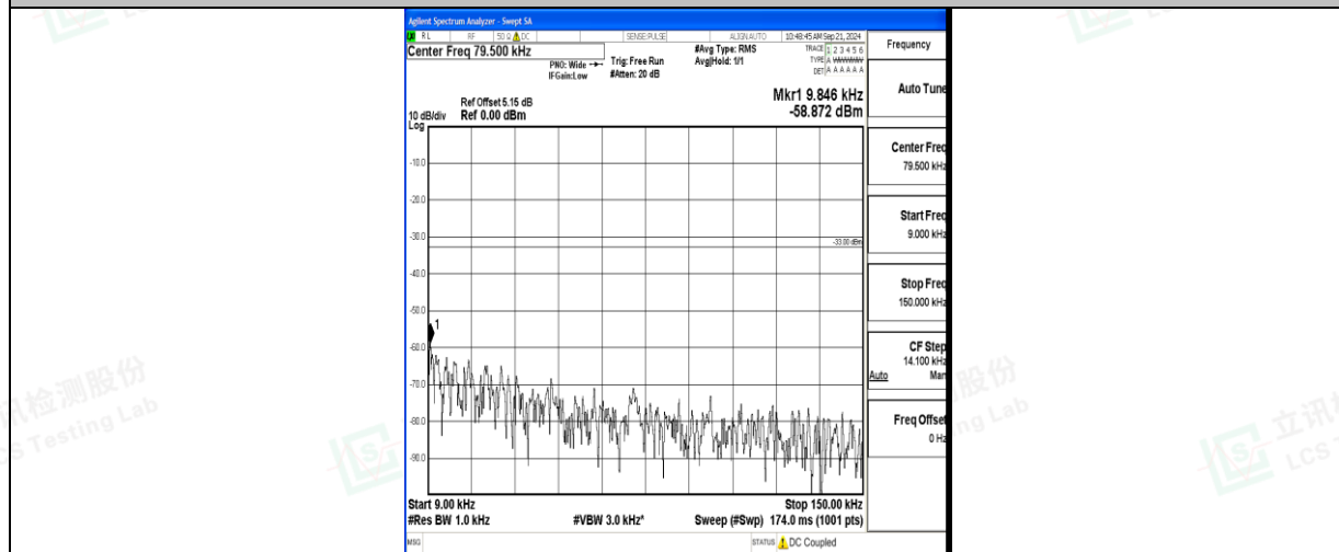
Band71_20MHz_16QAM_133372_1RB#0_0.009~0.15_0.009~0.15
